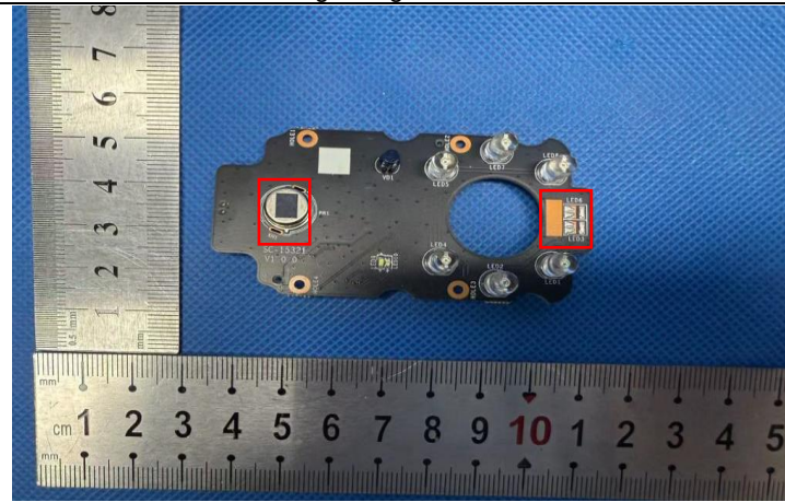
The original light board back side
