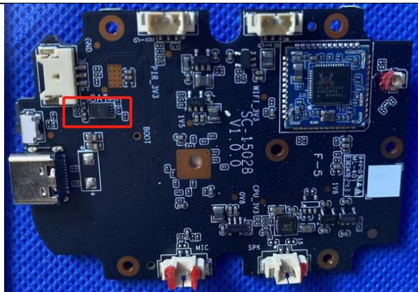
The original main board back side (without battery monitoring circuit)
