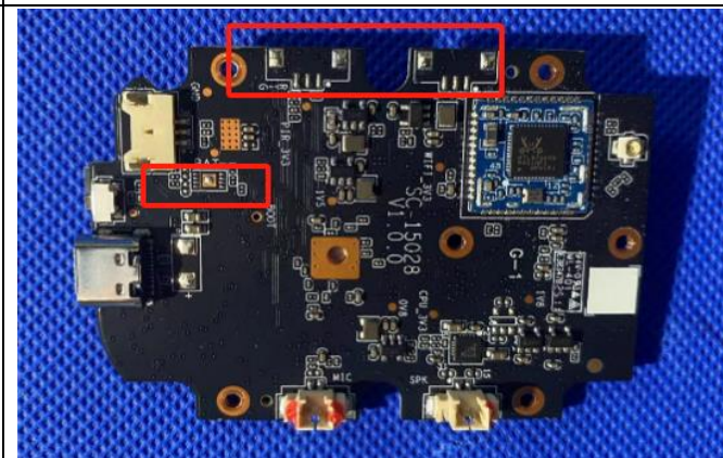
The new main board for model SC155-WQ3C back side (with battery monitoring circuit)
