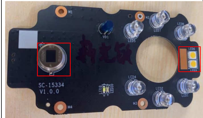
The new light board back side for model SC155 WQ3C front side
