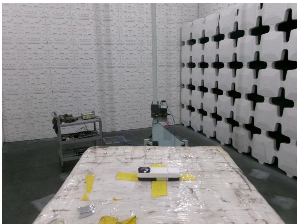
Radiated Setup for Above 1 GHz (433.92MHz)
