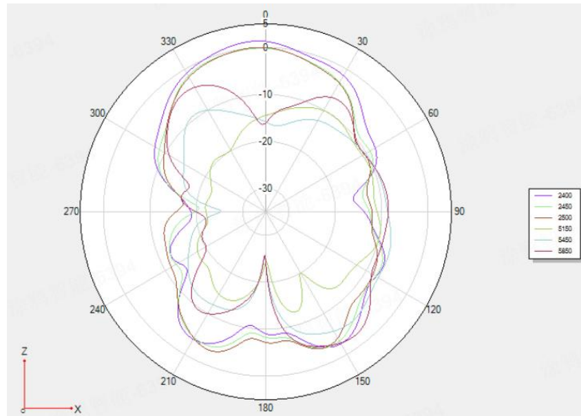
Phi 0 2D
