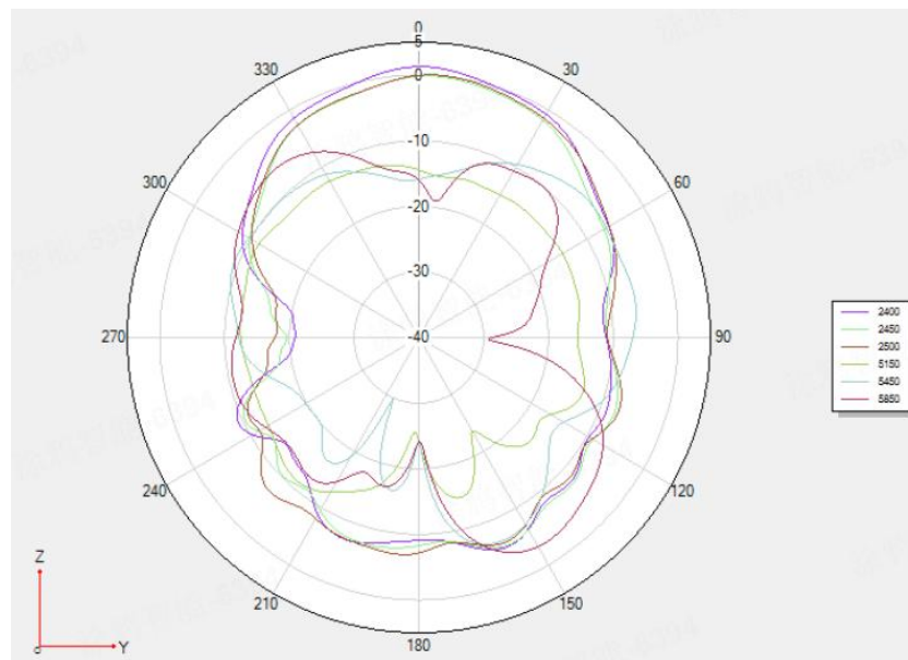
Theta 90 2D
