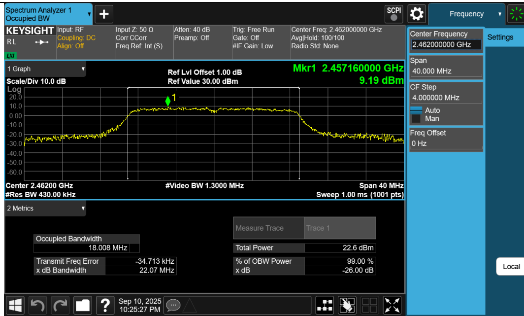
11N20SISO-Ant1-2462
