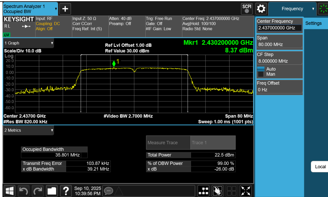
11N40SISO-Ant1-2437
