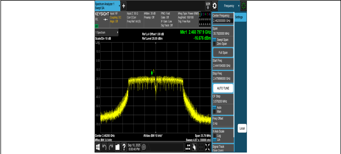
11N20SISO-Ant1-2462-PASS
