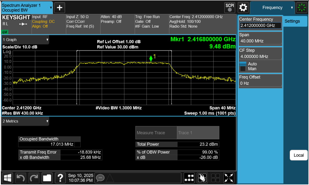
11G-Ant1-2412
