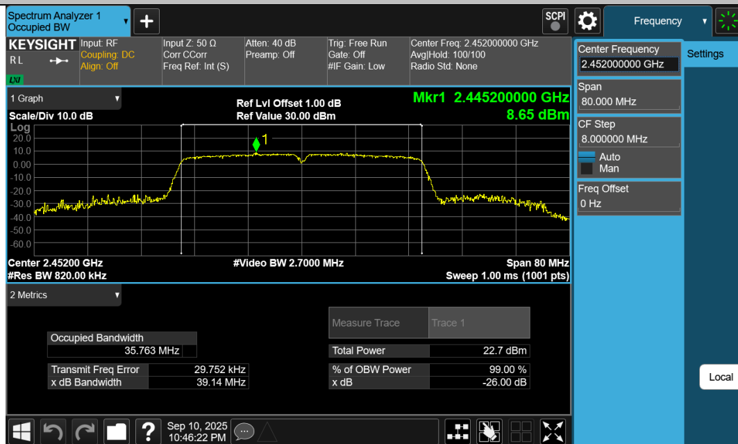
11N40SISO-Ant1-2452
