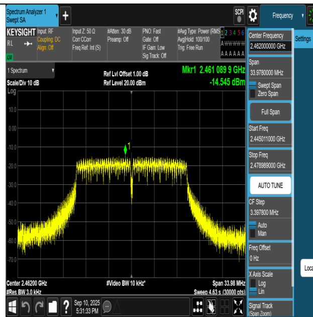
11G-Ant1-2462-PASS
