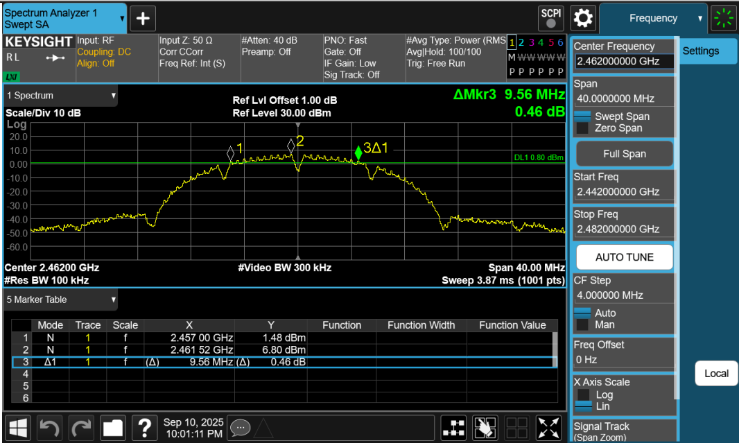
11B-Ant1-2462-PASS
