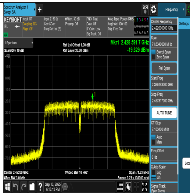
11N40SISO-Ant1-2422-PASS
