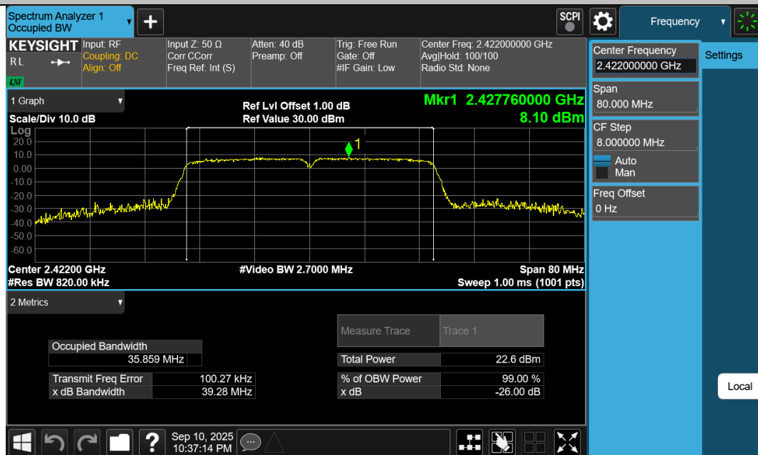
11N40SISO-Ant1-2422
