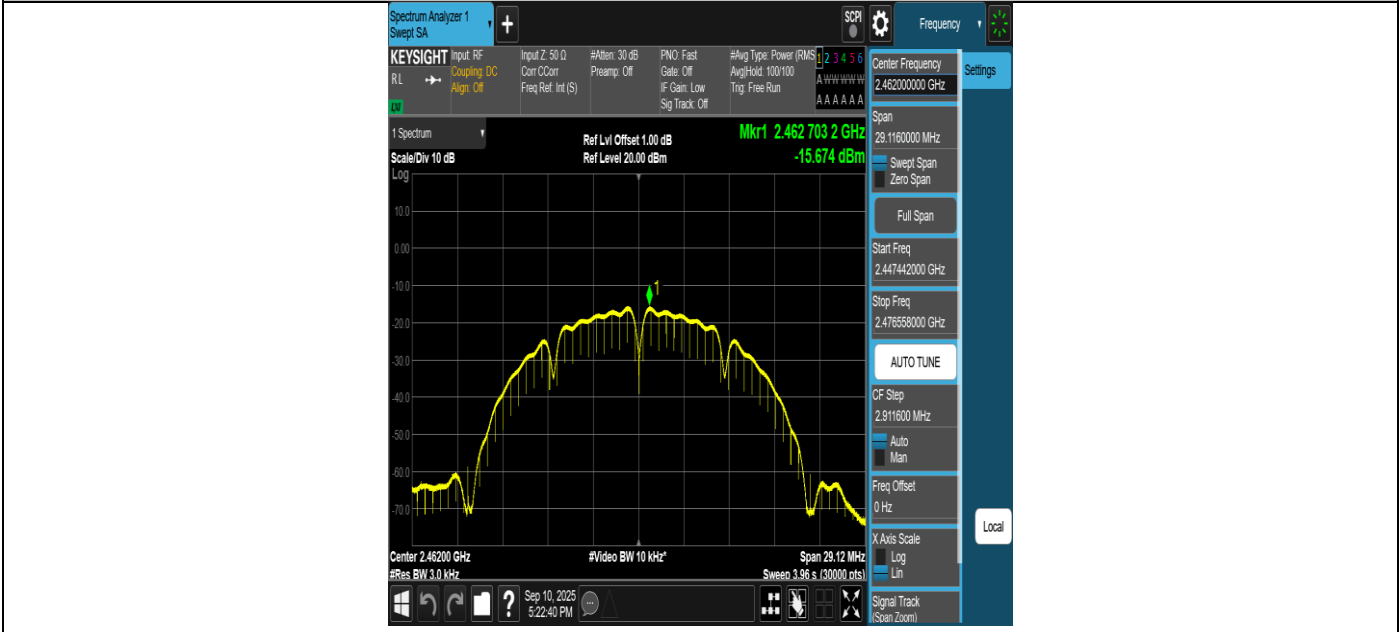
11B-Ant1-2462-PASS
