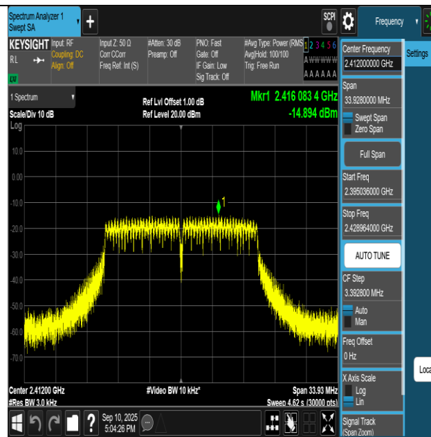
11G-Ant1-2412-PASS
