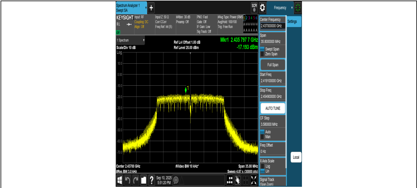
11N20SISO-Ant1-2437-PASS
