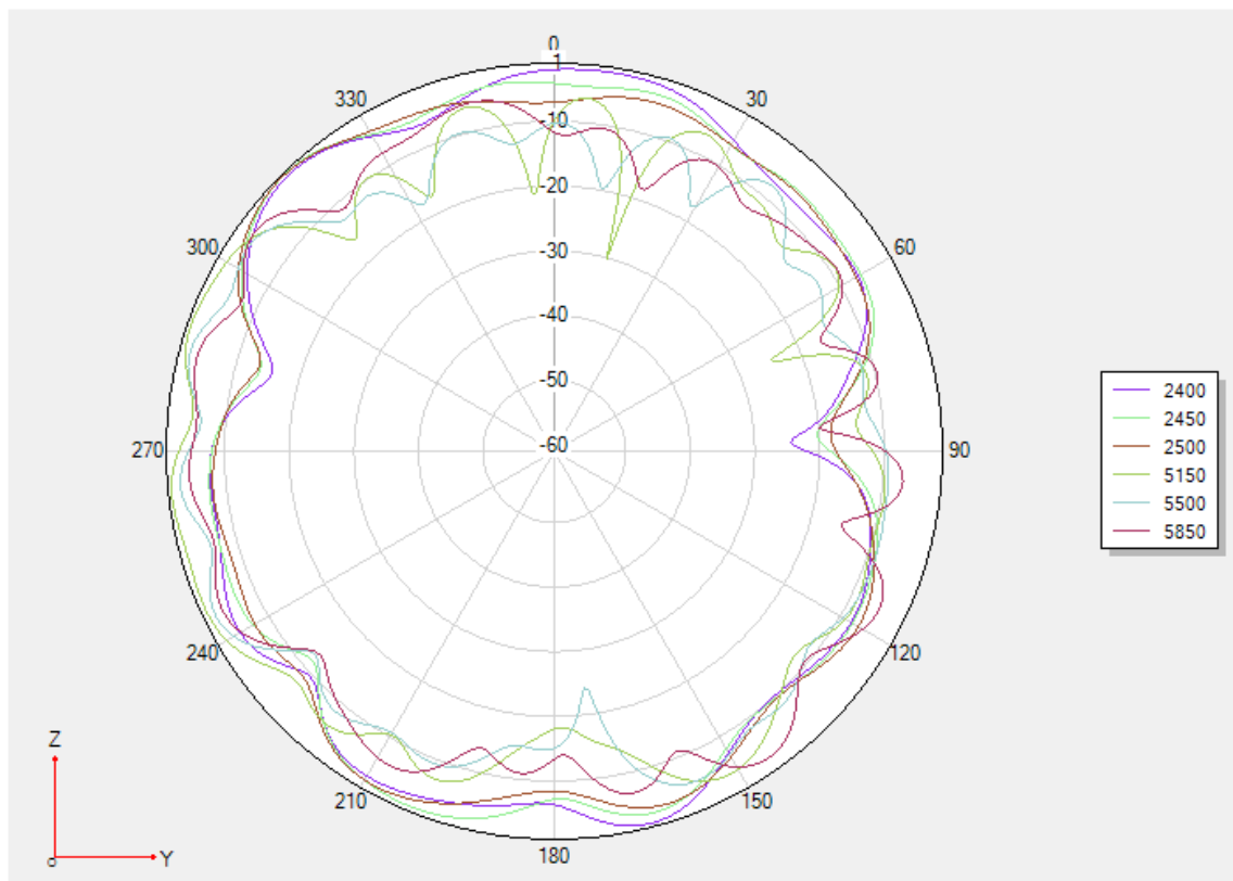
Phi 90 2D
