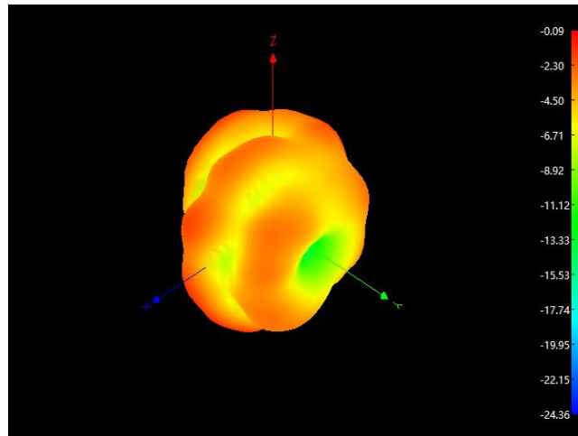
5150MHz 3D
