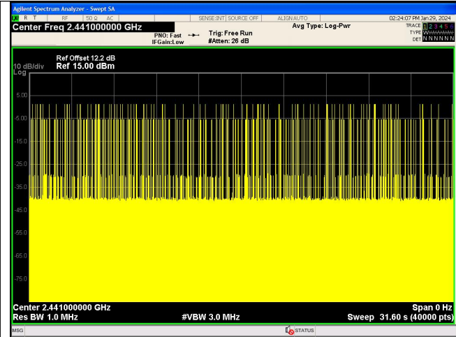
Number of Pulses in 31.6 seconds 8DPSPK_3-DH5
