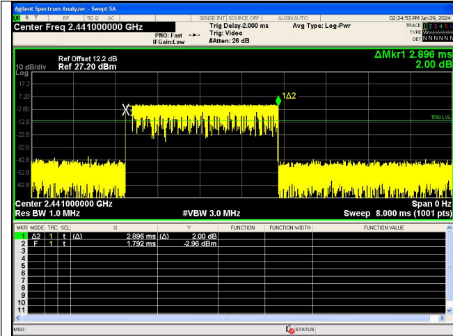
Pulse Width 8DPSPK_3-DH5
