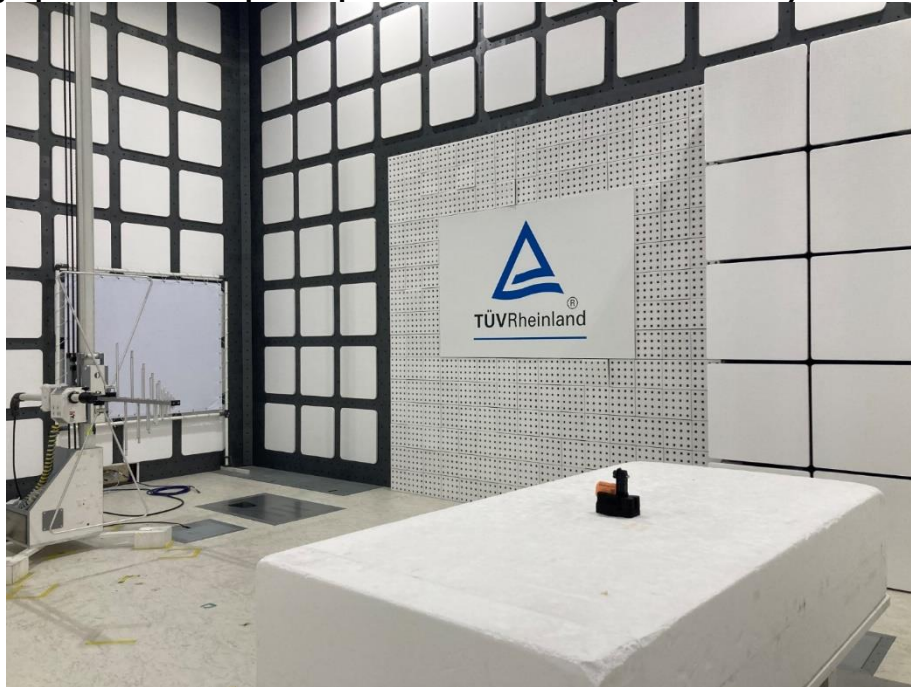
Photograph 3: Test Setup for Spurious Emissions (Back View 2)
