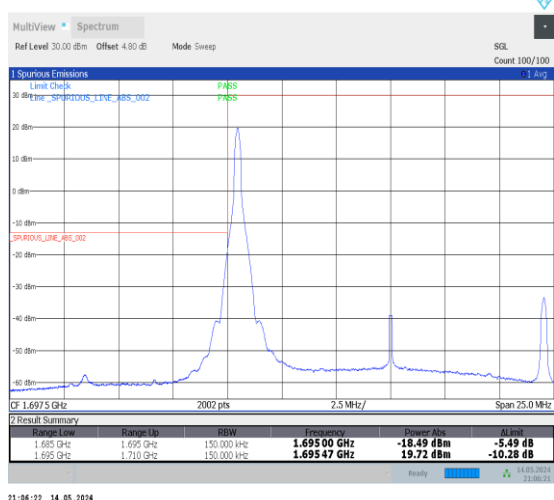
1-N70-PC3-15-15-L-4-CP-QPSK-Edge_1RB_Left-1@0-Ant2-1-seegraph-PASS-see graph
