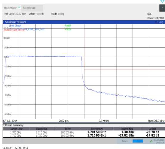
1-N70-PC3-15-10-H-6-CP-QPSK-Outer_Full-52@0-Ant2-1-seegraph-PASS-see graph
