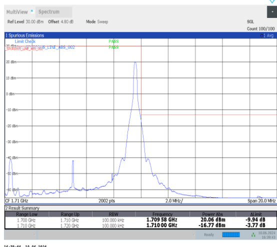
1-N70-PC3-15-10-H-2-DFT-PI2BPSK-Edge_1RB_Right-t1@51-Ant2-1-seegraph-PASS-see graph
