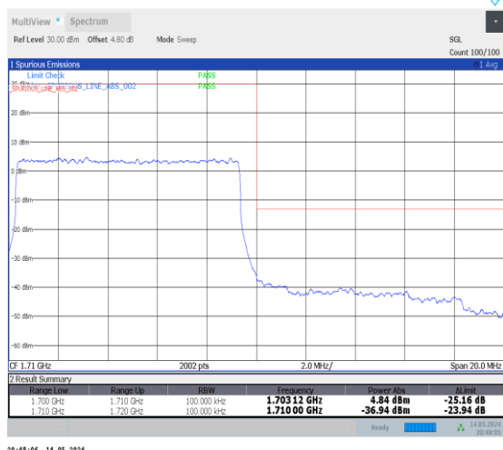
1-N70-PC3-15-10-H-3-DFT-PI2BPSK-Outer_Full-50@0-Ant2-1-seegraph-PASS-see graph
