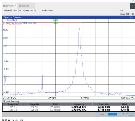
1-N70-PC3-15-15-H-2-DFT-PI2BPSK-Edge_1RB_Right-t1@78-Ant2-1-seegraph-PASS-see graph
