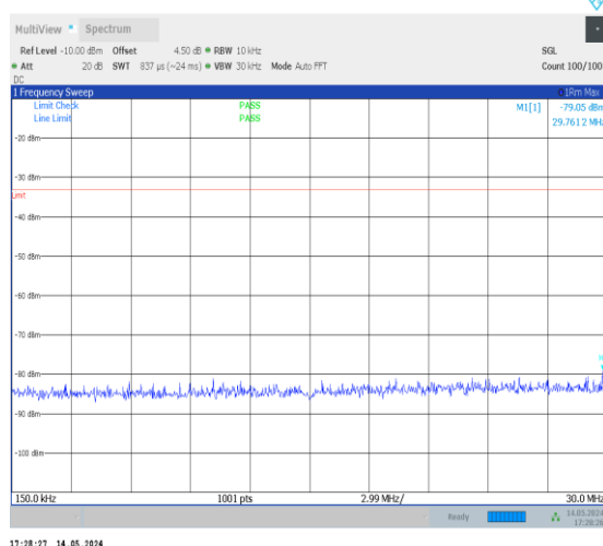
1-N70-PC3-15-15-H-1-DFT-PI2BPSK-Inner_1RB_Le ft-1@1-0.15-30-Ant2-29.76--79.05--33-PASS
