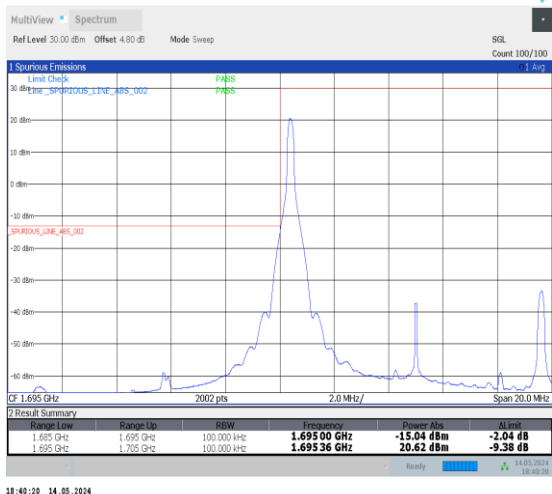
1-N70-PC3-15-10-L-1-DFT-PI2BPSK-Edge_1RB_Left-1@0-Ant2-1-seegraph-PASS-see graph
