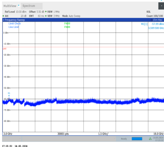
1-N70-PC3-15-15-L-1-DFT-PI2BPSK-Inner_1RB_Lef t-1@1-3000-18000-Ant2-3589.50--57.99--13-PASS
