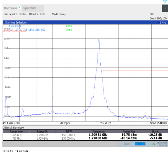
1-N70-PC3-15-15-H-5-CP-QPSK-Edge_1RB_Right-1@78-Ant2-1-seegraph-PASS-see graph
