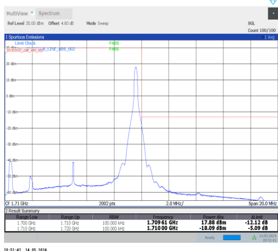
1-N70-PC3-15-10-H-5-CP-QPSK-Edge_1RB_Right-1@51-Ant2-1-seegraph-PASS-see graph
