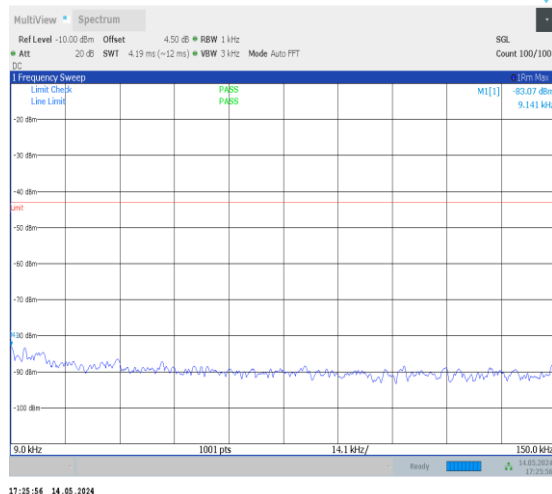
1-N70-PC3-15-15-M-1-DFT-PI2BPSK-Inner_1RB_Le ft-1@1-0.009-0.15-Ant2-0.01--83.07--43-PASS
