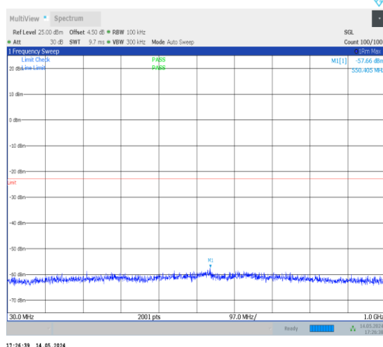
1-N70-PC3-15-15-M-1-DFT-PI2BPSK-Inner_1RB_Le ft-1@1-30-1000-Ant2-550.41--57.66--23-PASS
