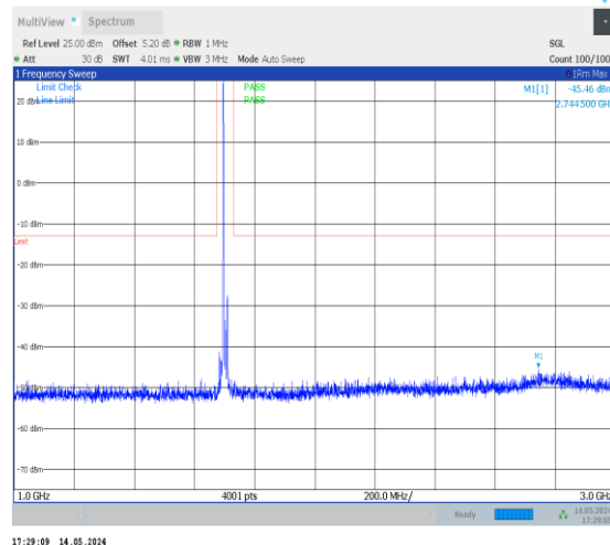
1-N70-PC3-15-15-H-1-DFT-PI2BPSK-Inner_1RB_Le ft-1@1-1000-3000-Ant2-2744.50--45.46--13-PASS
