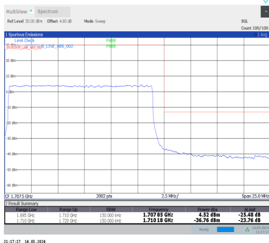
1-N70-PC3-15-15-H-3-DFT-PI2BPSK-Outer_Full-75@0-Ant2-1-seegraph-PASS-see graph
