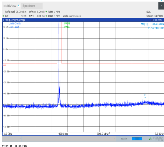
1-N70-PC3-15-15-M-1-DFT-PI2BPSK-Inner_1RB_Le ft-1@1-1000-3000-Ant2-2762.50--44.74--13-PASS
