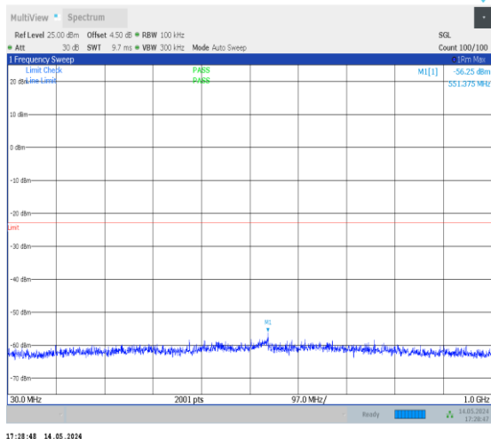
1-N70-PC3-15-15-H-1-DFT-PI2BPSK-Inner_1RB_Le ft-1@1-30-1000-Ant2-551.38--56.25--23-PASS
