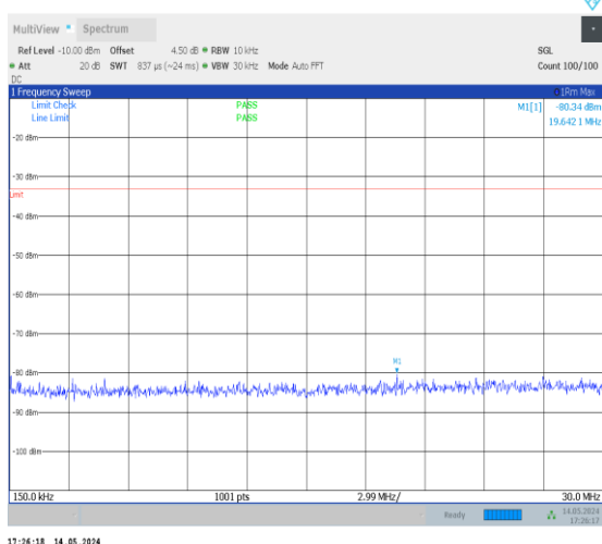
1-N70-PC3-15-15-M-1-DFT-PI2BPSK-Inner_1RB_Le ft-1@1-0.15-30-Ant2-19.64--80.34--33-PASS
