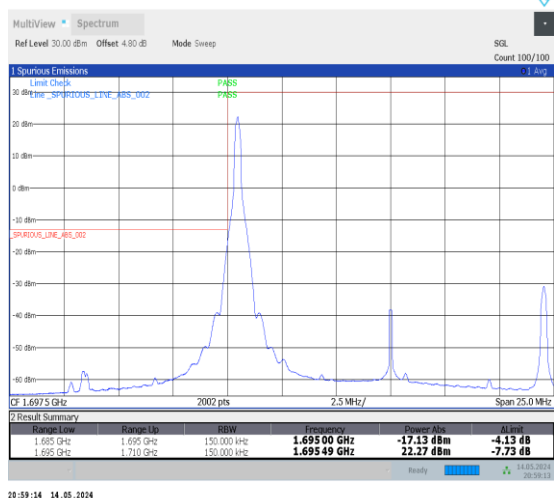
1-N70-PC3-15-15-L-1-DFT-PI2BPSK-Edge_1RB_Left-1@0-Ant2-1-seegraph-PASS-see graph
