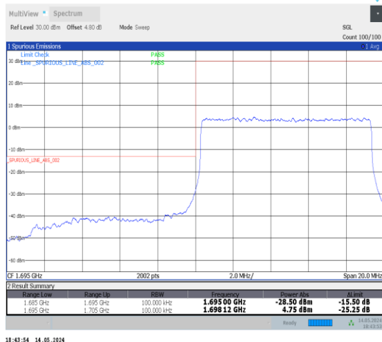
1-N70-PC3-15-10-L-3-DFT-PI2BPSK-Outer_Full-50@0-Ant2-1-seegraph-PASS-see graph
