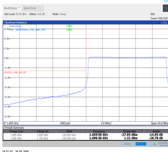
1-N70-PC3-15-10-L-6-CP-QPSK-Outer_Full-52@0-Ant2-1-seegraph-PASS-see graph
