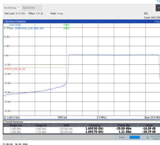
1-N70-PC3-15-15-L-6-CP-QPSK-Outer_Full-79@0-Ant2-1-seegraph-PASS-see graph
