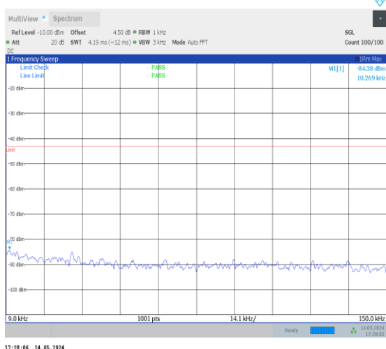
1-N70-PC3-15-15-H-1-DFT-PI2BPSK-Inner_1RB_Le ft-1@1-0.009-0.15-Ant2-0.01--84.38--43-PASS
