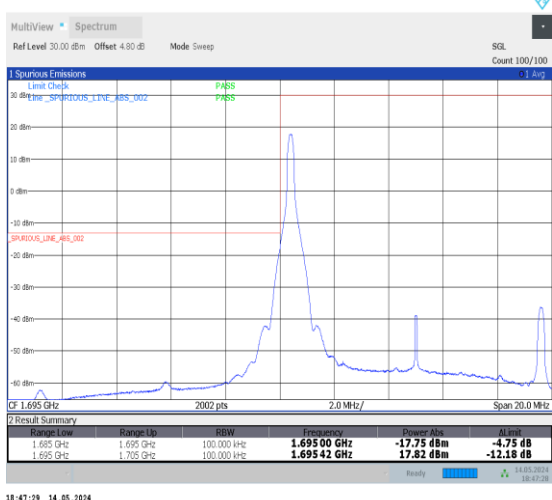
1-N70-PC3-15-10-L-4-CP-QPSK-Edge_1RB_Left-1@0-Ant2-1-seegraph-PASS-see graph
