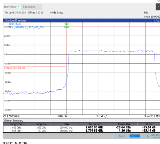
1-N70-PC3-15-15-L-3-DFT-PI2BPSK-Outer_Full-75@0-Ant2-1-seegraph-PASS-see graph
