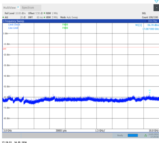
1-N70-PC3-15-15-H-1-DFT-PI2BPSK-Inner_1RB_Le ft-1@1-3000-18000-Ant2-17087.00--56.78--13-PASS
