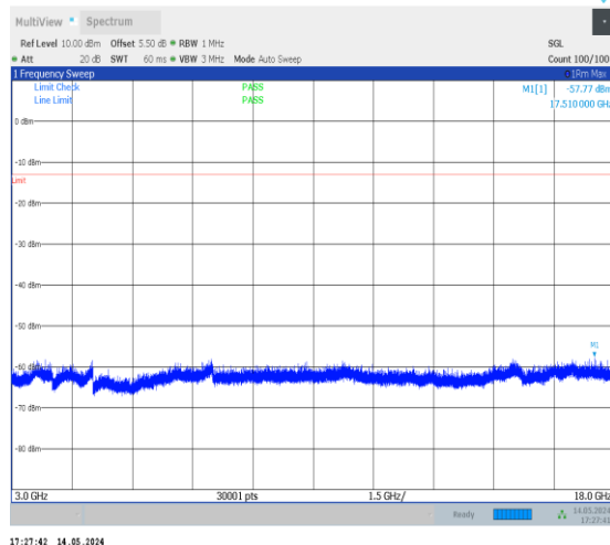
1-N70-PC3-15-15-M-1-DFT-PI2BPSK-Inner_1RB_Le ft-1@1-3000-18000-Ant2-17510.00--57.77--13-PASS
