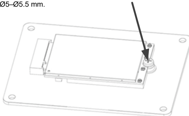
Figure 34: Installation Schematic
