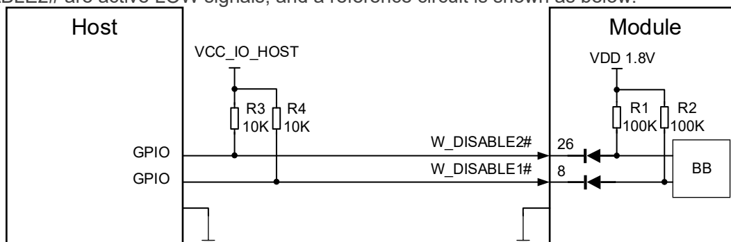
Figure 17: W_DISABLE1# and W_DISABLE2# Reference Circuit
