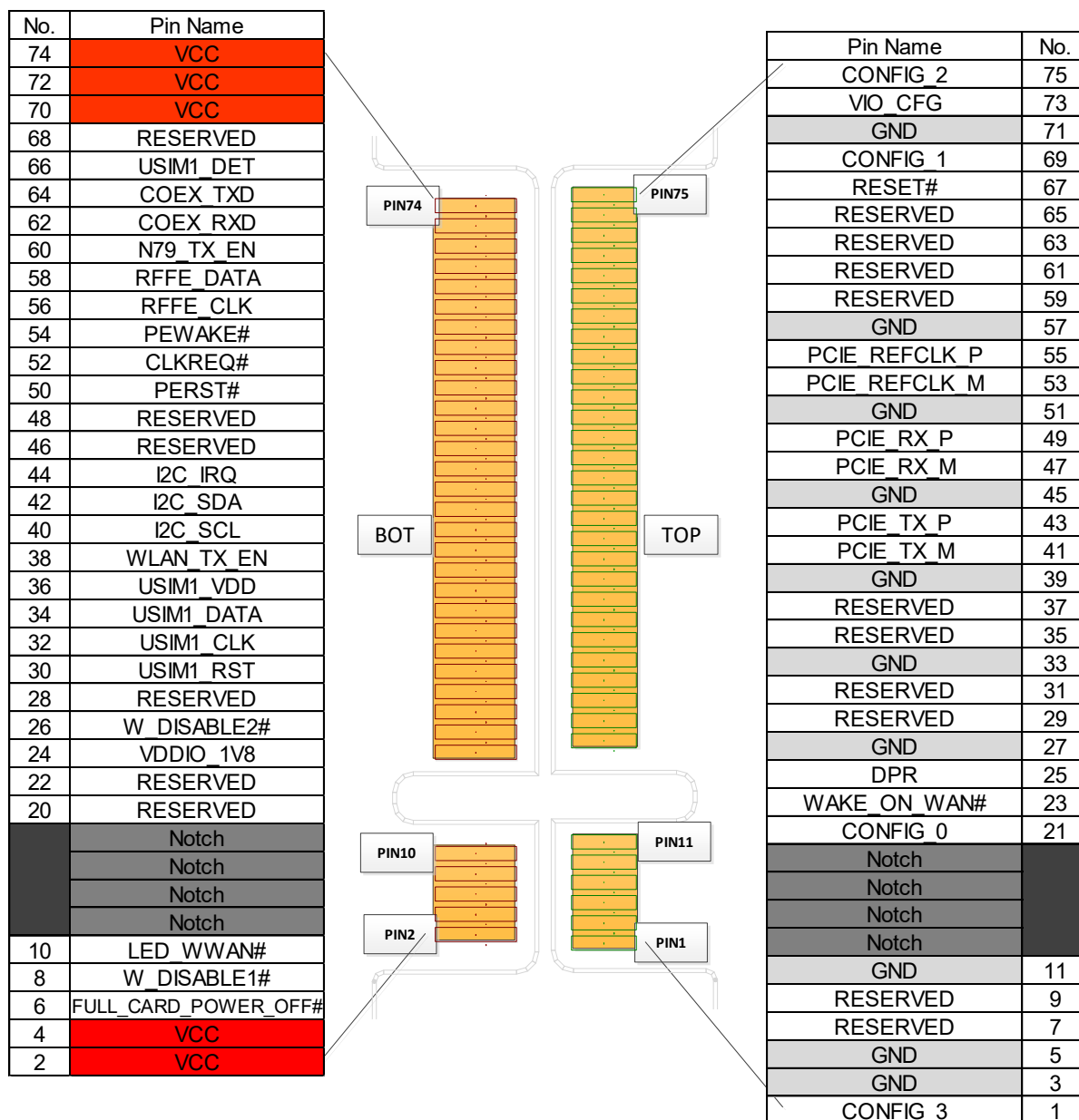
Figure 2: Pin Assignment
