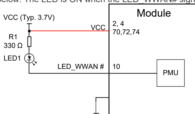
Figure 18: LED_WWAN# Reference Circuit
