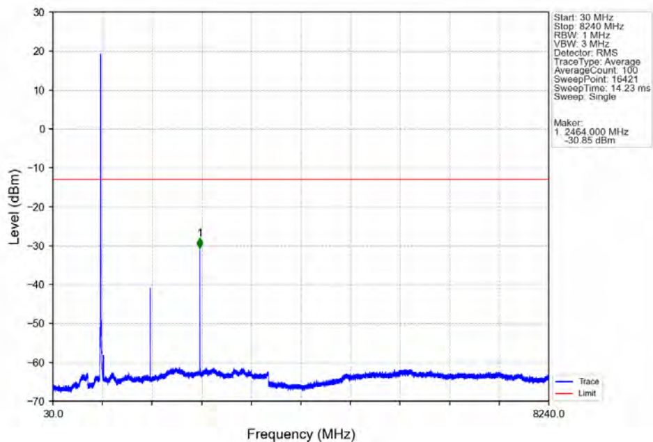
Band26a 3MHz QPSK HCH 822.5MHz RB 1 14 NTV
