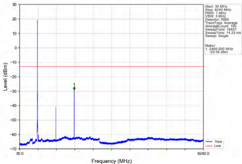
Band26a 1.4MHz 64QAM HCH 823.3MHz RB 1 5 NTNV
