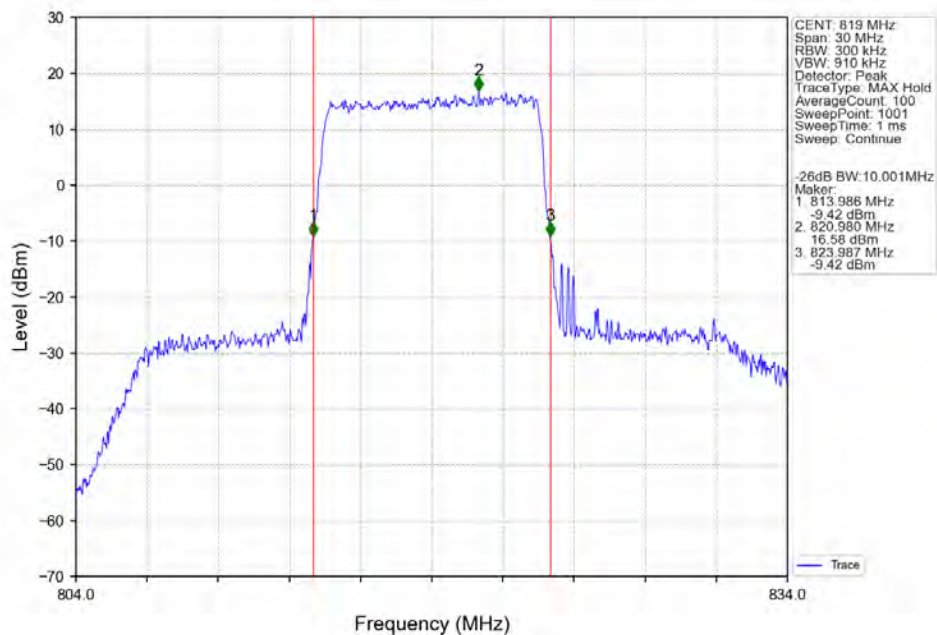
Band26a 10MHz 256QAM MCH 819MHz RB 50 0 NTN
