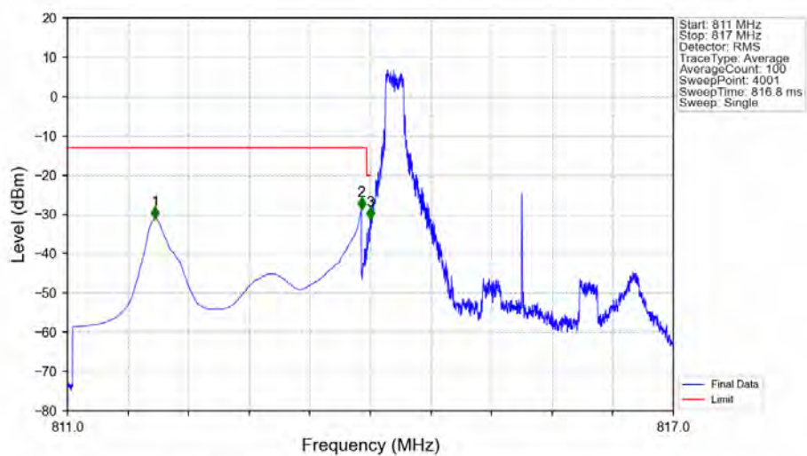
Band26a 3MHz 64QAM LCH 815.5MHz RB 1 0 NTNV
