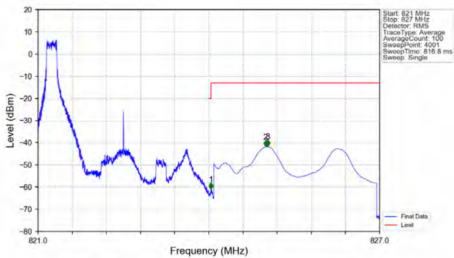
Band26a 3MHz 64QAM HCH 822.5MHz RB 1 14 NTNV
