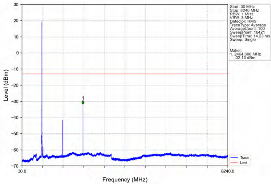
Band26a 3MHz 64QAM HCH 822.5MHz RB 1 14 NTNV
