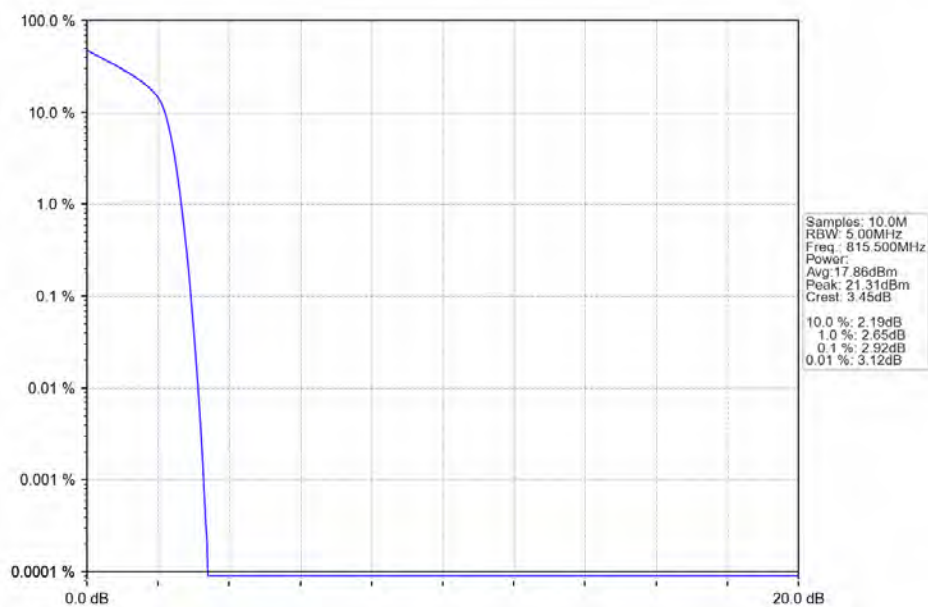
Band26a_3MHz_QPSK_LCH_815.5MHz_RB_15_0_NTNV
