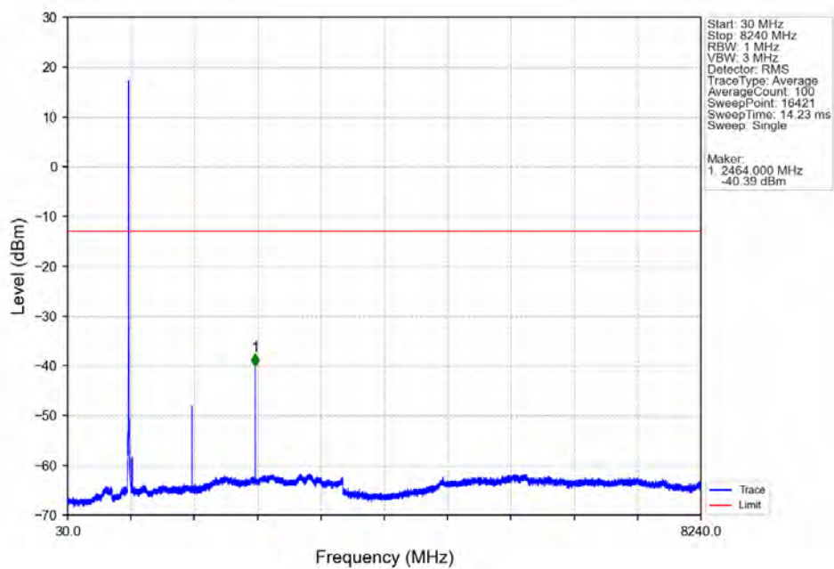
Band26a 3MHz 256QAM HCH 822.5MHz RB 1 0 NTNV
