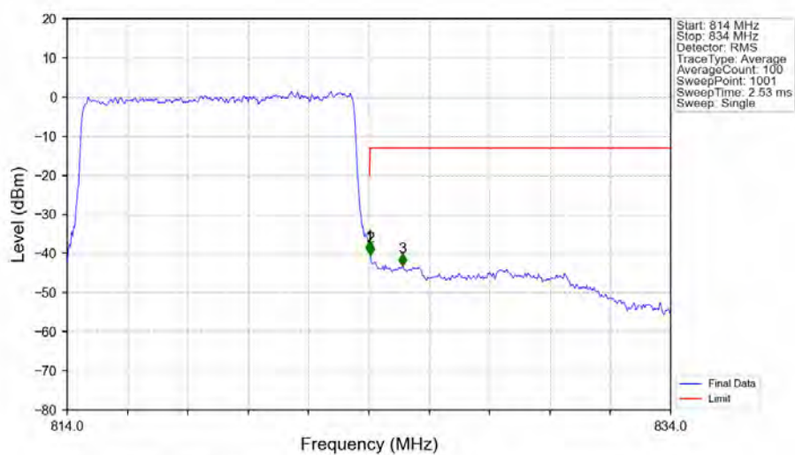
Band26a 10MHz 256QAM HCH 819MHz RB 50 0 NTNV
