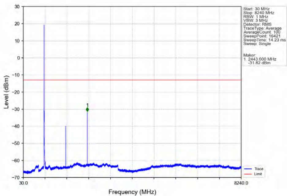
Band26a 3MHz 64QAM LCH 815.5MHz RB 1 0 NTNV
