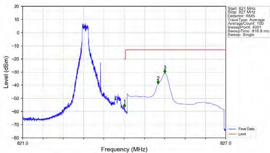
Band26a 1.4MHz 64QAM HCH 823.3MHz RB 1 5 NTNV
