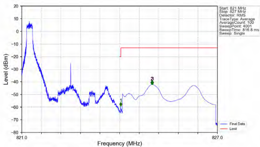
Band26a 3MHz QPSK HCH 822.5MHz RB 1 14 NTV
