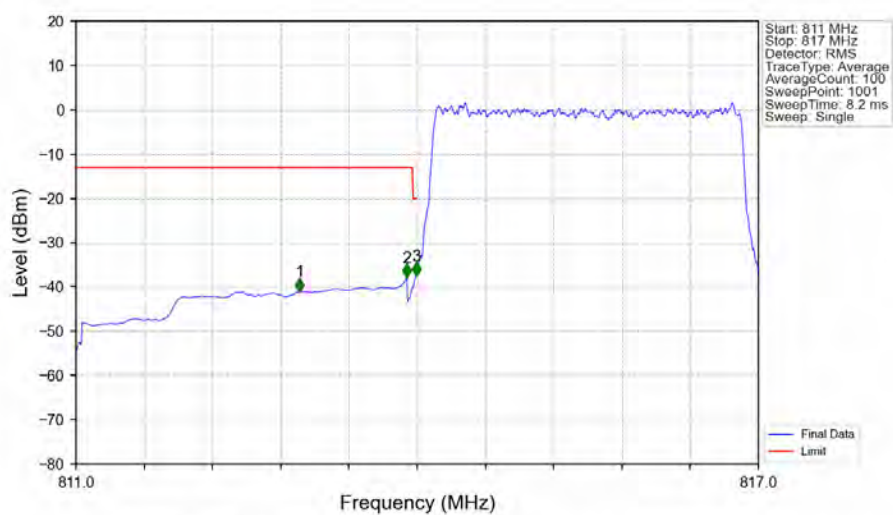
Band26a 3MHz 256QAM LCH 815.5MHz RB 15 0 NTNV
