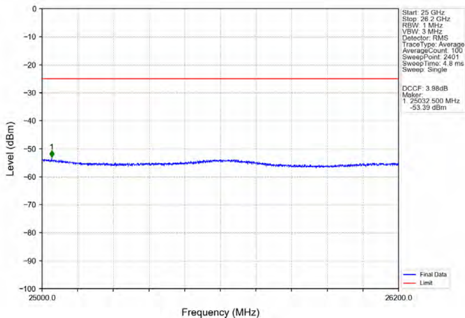
Band38 5MHz 64QAM HCH 2617.5MHz RB 1 24 NTNV
