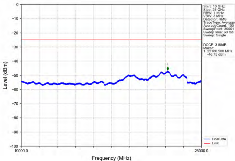
Band38 5MHz 64QAM MCH 2595MHz RB 1 0 NTNV
