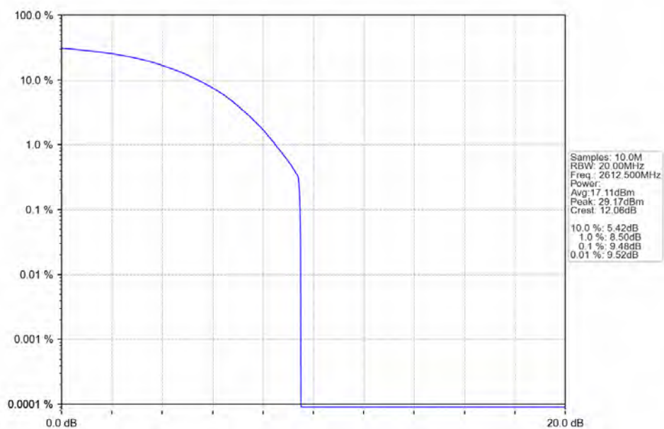
Band38 15MHz 256QAM HCH 2612.5MHz RB 75 0 NTV
