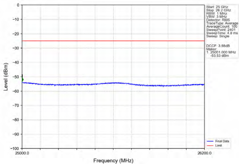
Band38 5MHz QPSK MCH 2595MHz RB 1 0 NTNV
