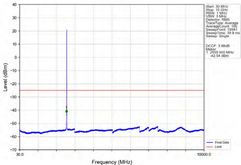
Band38 5MHz 16QAM LCH 2572.5MHz RB 1 0 NTNV
