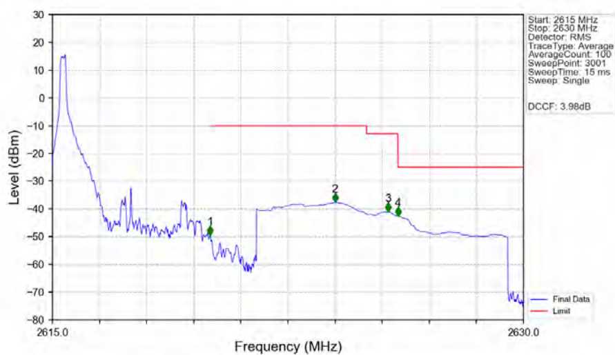
Band38 5MHz 64QAM HCH 2617.5MHz RB 1 24 NTNV
