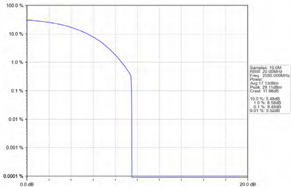
Band38 15MHz 256QAM MCH 2595MHz RB 75 0 NTV
