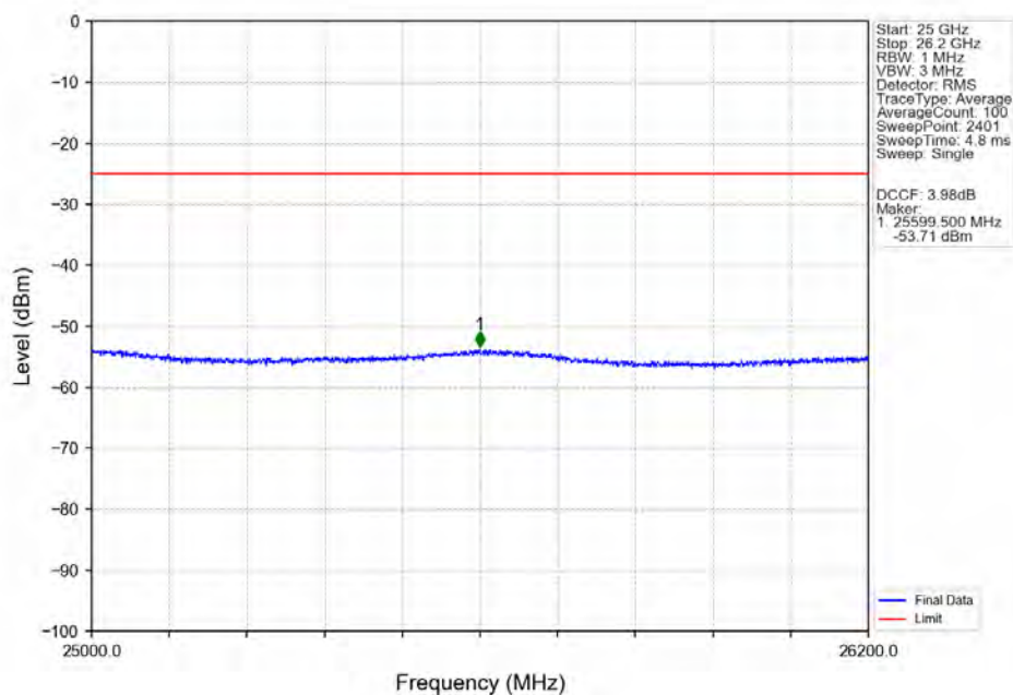
Band38 5MHz 64QAM LCH 2572.5MHz RB 1 0 NTNV
