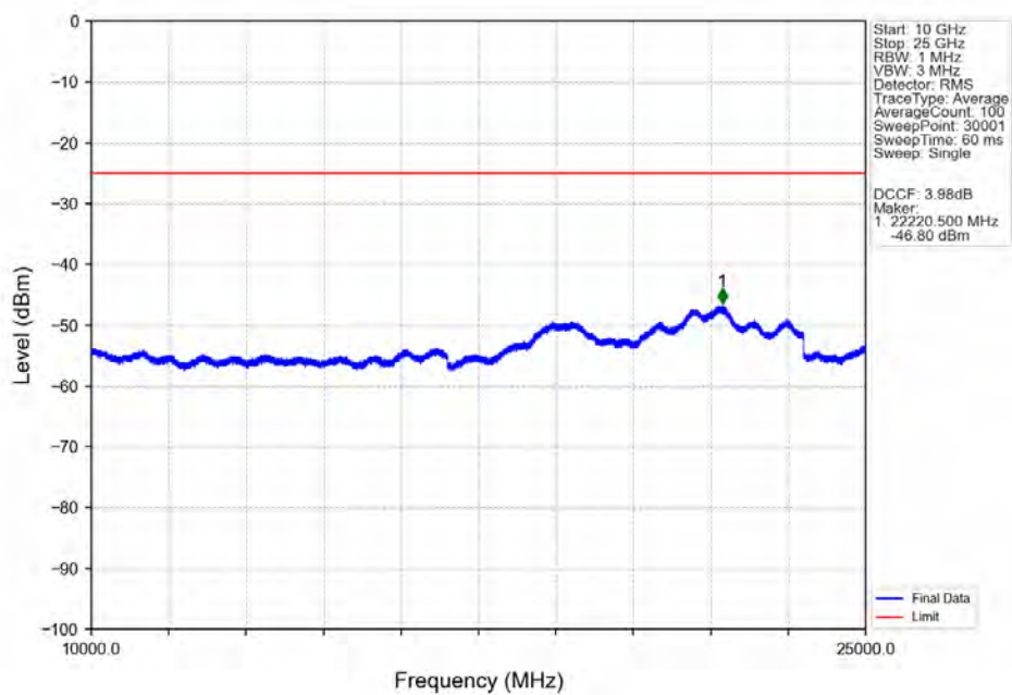
Band38 5MHz 16QAM MCH 2595MHz RB 1 0 NTNV
