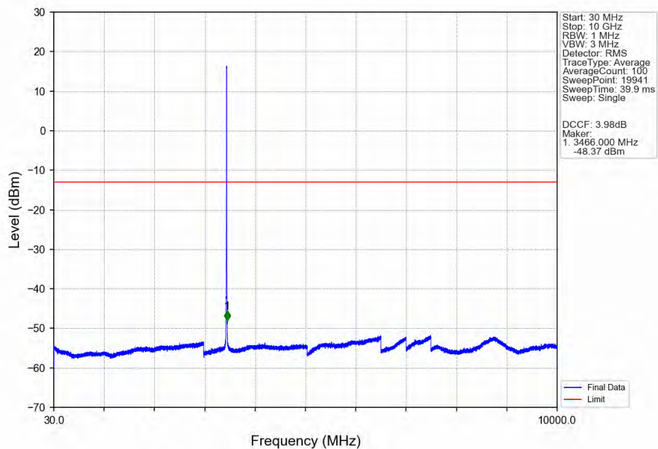
Band42a 5MHz 16QAM LCH 3452.5MHz RB 1 0 NTNV
