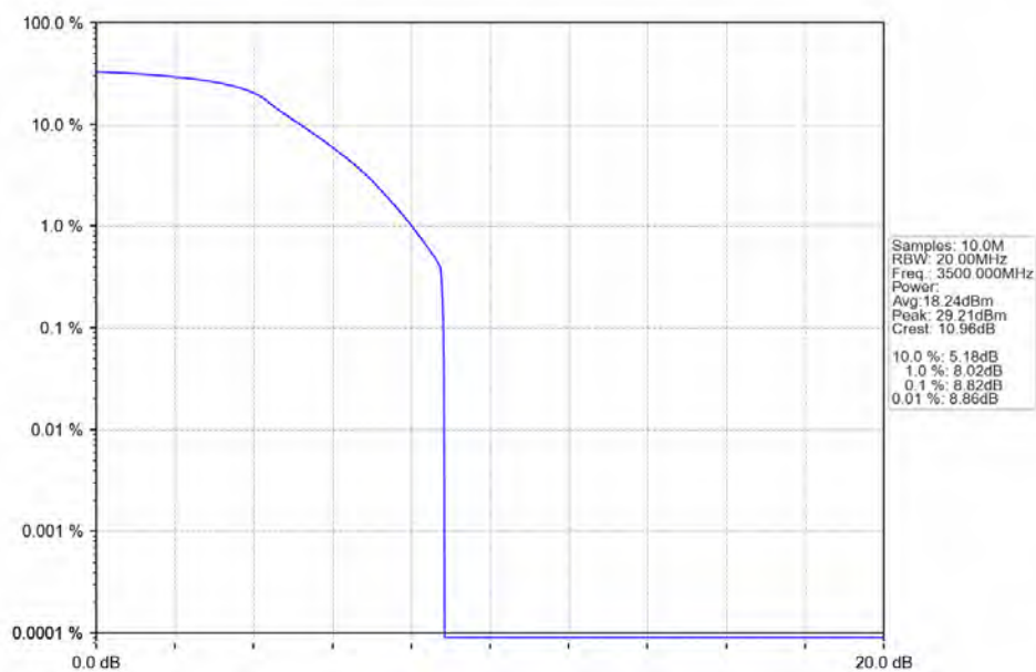
Band42a_15MHz_QPSK_MCH_3500MHz_RB_75_0_NTNV
