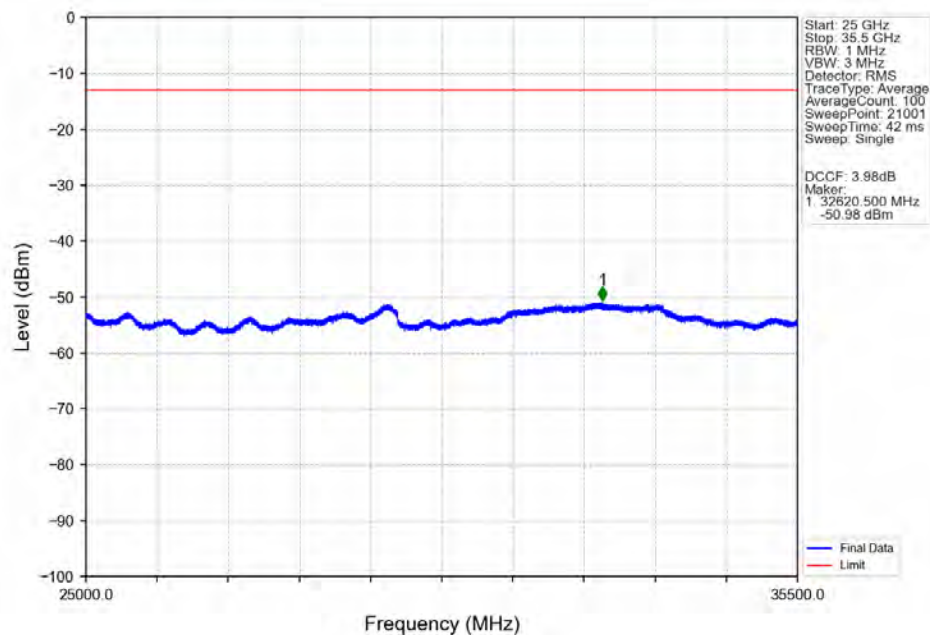
Band42a 5MHz 16QAM LCH 3452.5MHz RB 25 0 NTNV
