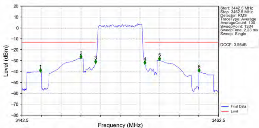
Band42a 5MHz 16QAM LCH 3452.5MHz RB 25 0 NTNV
