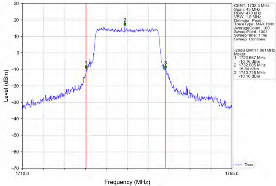
Band4_15MHz_64QAM_MCH_1732.5MHz_RB_75_0_NTNV
