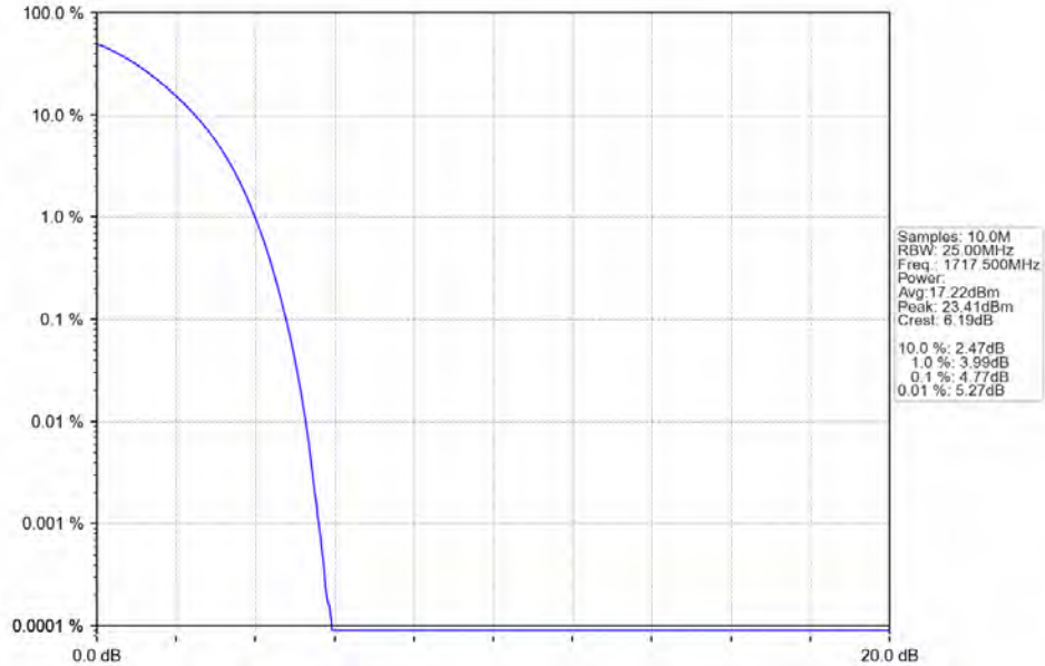
Band4_15MHz_256QAM_LCH_1717.5MHz_RB_75_0_NTNV
