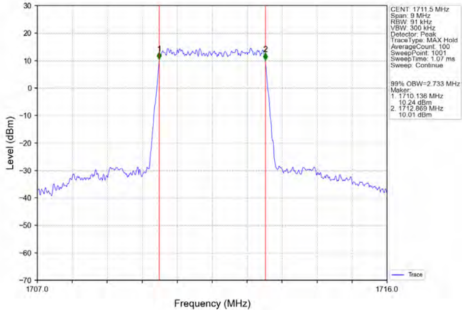
Band4_3MHz_256QAM_LCH_1711.5MHz_RB_15_0_NTNV
