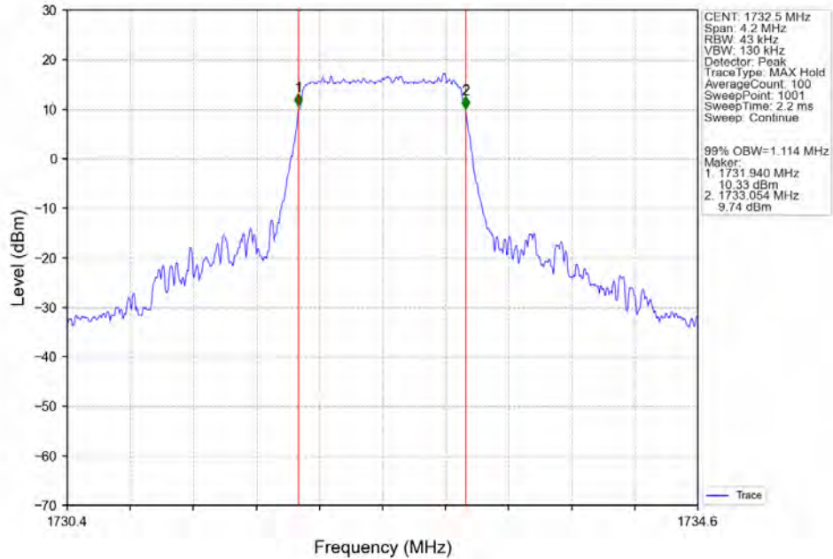
Band4_1.4MHz_64QAM_MCH_1732.5MHz_RB_6_0_NTNV
