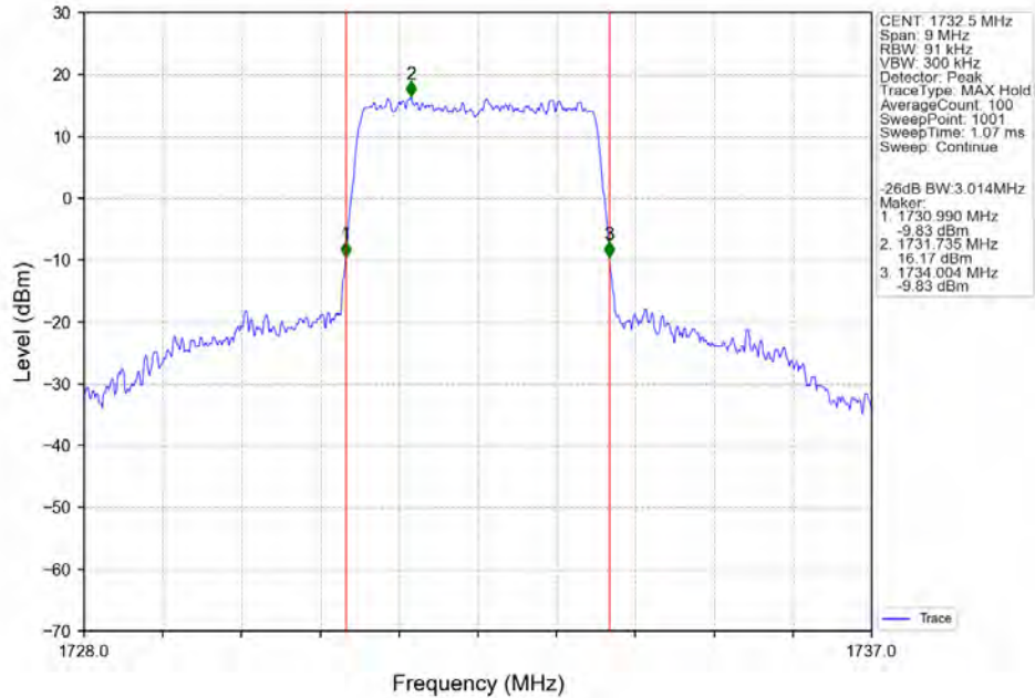
Band4_3MHz_QPSK_MCH_1732.5MHz_RB_15_0_NTNV
