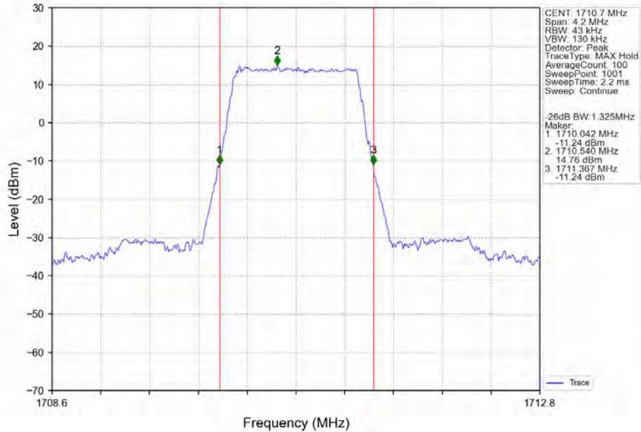
Band4_1.4MHz_256QAM_LCH_1710.7MHz_RB_6_0_NTNV
