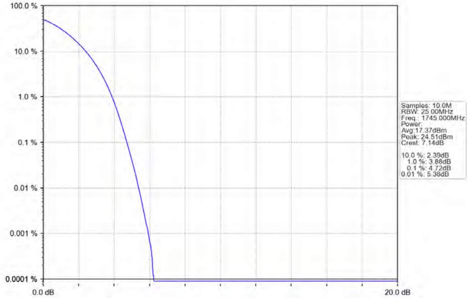
Band4_20MHz_256QAM_HCH_1745MHz_RB_100_0_NTNV
