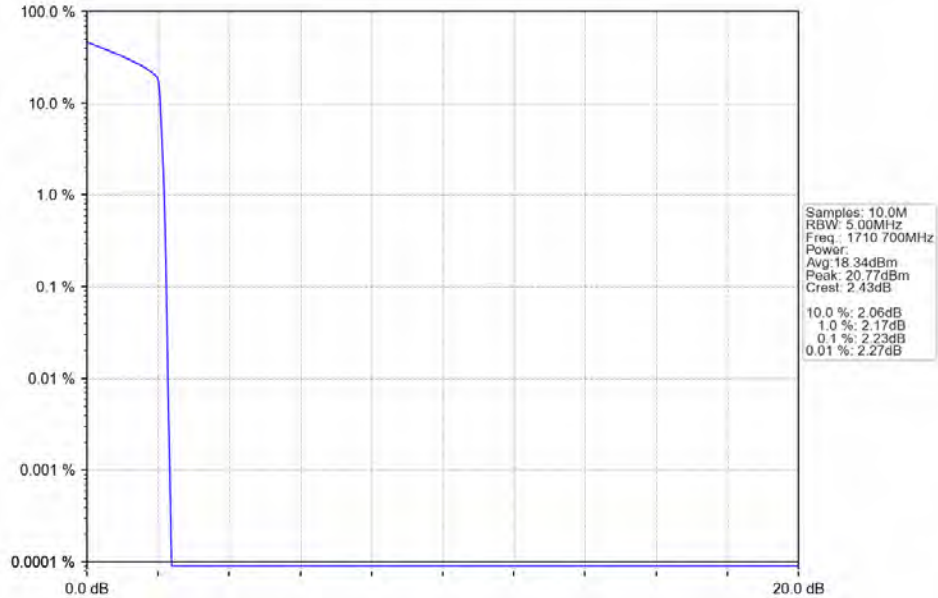
Band4_1.4MHz_16QAM_LCH_1710.7MHz_RB_6_0_NTNV
