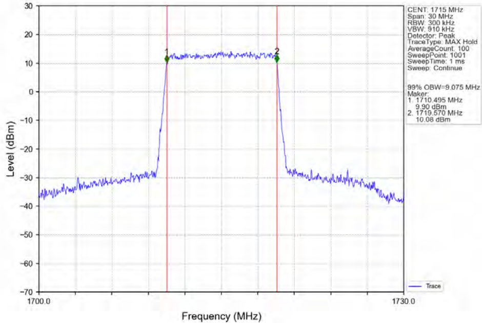
Band4_10MHz_256QAM_LCH_1715MHz_RB_50_0_NTNV
