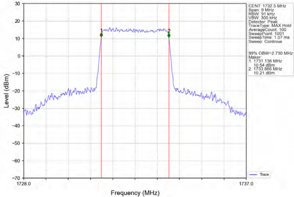
Band4_3MHz_64QAM_MCH_1732.5MHz_RB_15_0_NTNV
