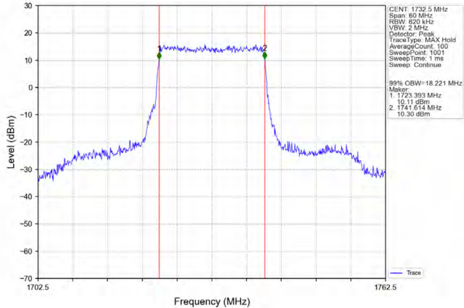
Band4_20MHz_64QAM_MCH_1732.5MHz_RB_100_0_NTNV
