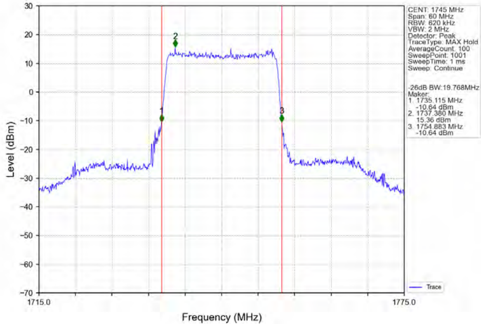
Band4_20MHz_256QAM_HCH_1745MHz_RB_100_0_NTNV
