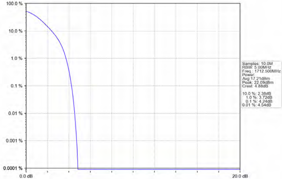
Band4_5MHz_256QAM_LCH_1712.5MHz_RB_25_0_NTNV
