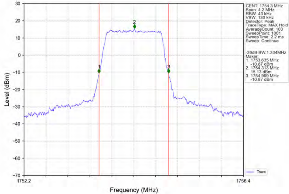
Band4_1.4MHz_256QAM_HCH_1754.3MHz_RB_6_0_NTNV
