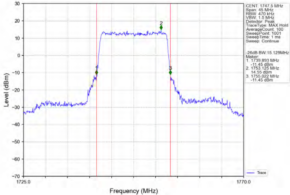
Band4_15MHz_256QAM_HCH_1747.5MHz_RB_75_0_NTNV
