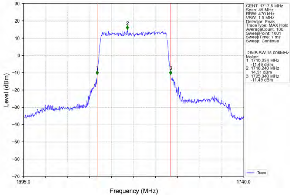
Band4_15MHz_256QAM_LCH_1717.5MHz_RB_75_0_NTNV
