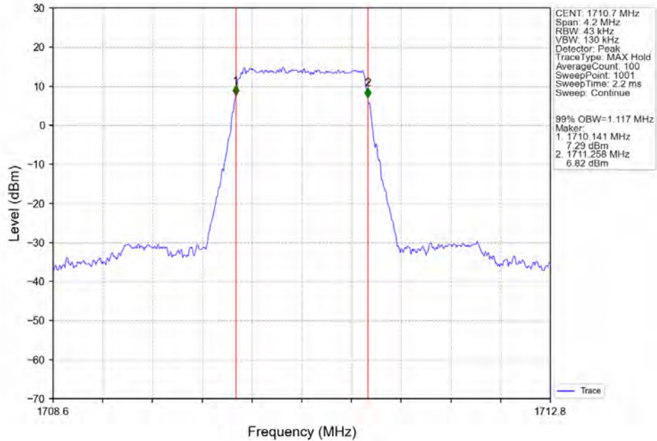
Band4_1.4MHz_256QAM_LCH_1710.7MHz_RB_6_0_NTNV
