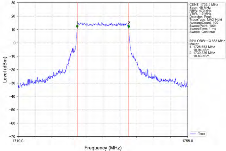
Band4_15MHz_QPSK_MCH_1732.5MHz_RB_75_0_NTNV
