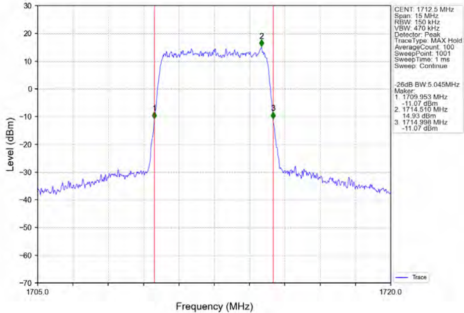
Band4_5MHz_256QAM_LCH_1712.5MHz_RB_25_0_NTNV
