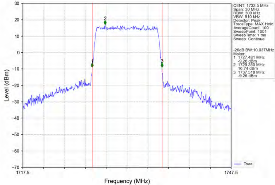
Band4_10MHz_64QAM_MCH_1732.5MHz_RB_50_0_NTNV
