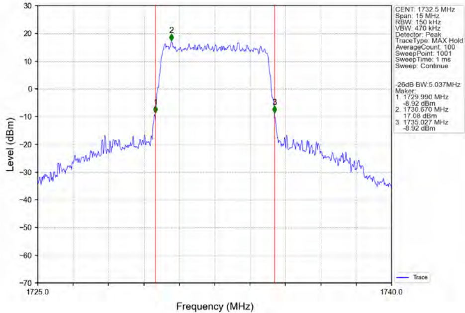
Band4_5MHz_64QAM_MCH_1732.5MHz_RB_25_0_NTNV
