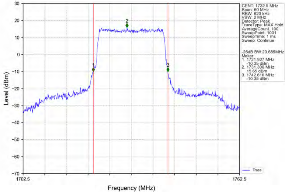
Band4_20MHz_64QAM_MCH_1732.5MHz_RB_100_0_NTNV
