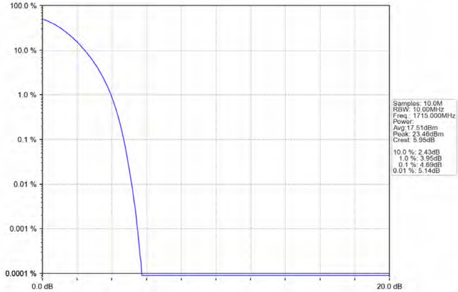
Band4_10MHz_256QAM_LCH_1715MHz_RB_50_0_NTNV
