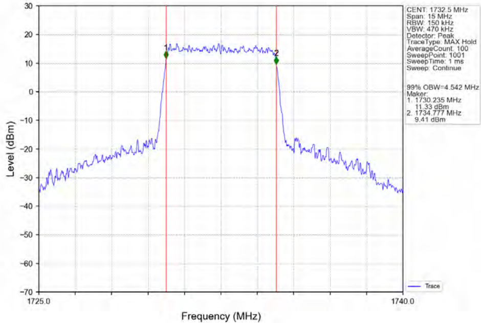
Band4_5MHz_QPSK_MCH_1732.5MHz_RB_25_0_NTNV
