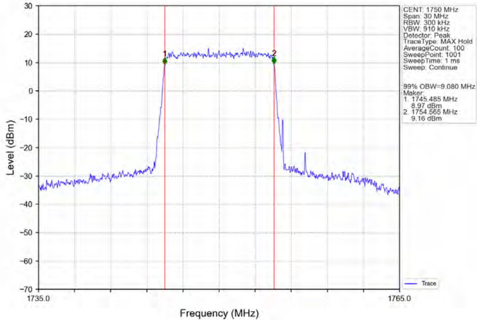
Band4_10MHz_256QAM_HCH_1750MHz_RB_50_0_NTNV
