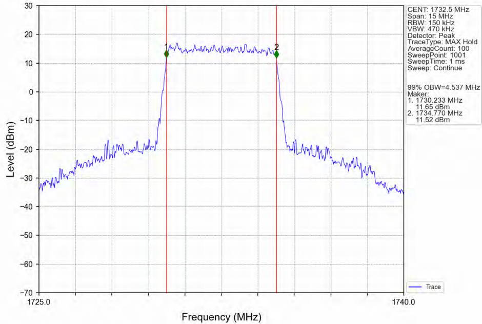
Band4_5MHz_64QAM_MCH_1732.5MHz_RB_25_0_NTNV
