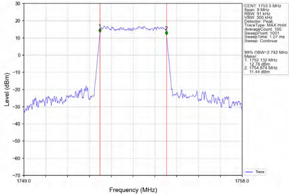
Band4_3MHz_16QAM_HCH_1753.5MHz_RB_15_0_NTNV
