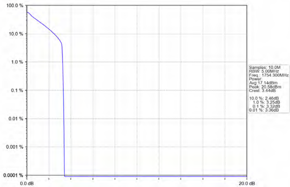
Band4_1.4MHz_256QAM_HCH_1754.3MHz_RB_6_0_NTNV
