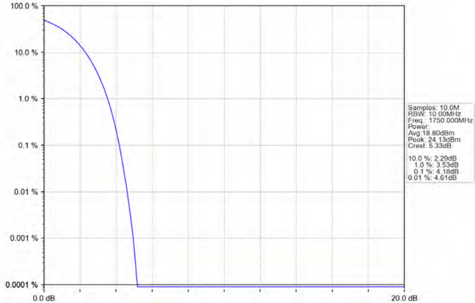
Band4_10MHz_16QAM_HCH_1750MHz_RB_50_0_NTNV
