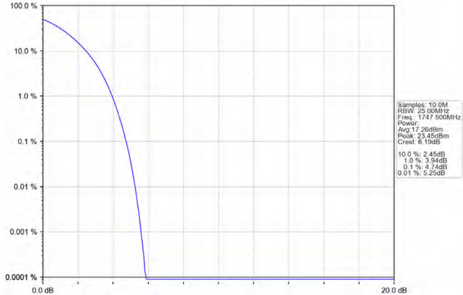
Band4_15MHz_256QAM_HCH_1747.5MHz_RB_75_0_NTNV
