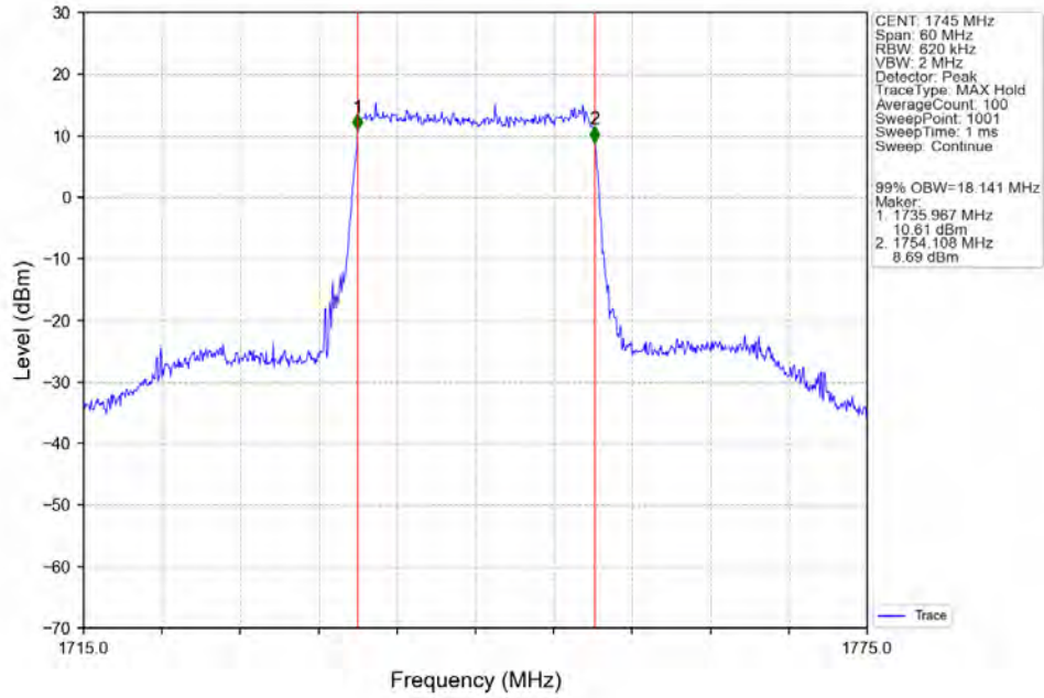
Band4_20MHz_256QAM_HCH_1745MHz_RB_100_0_NTNV
