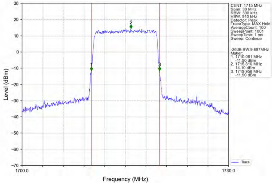
Band4_10MHz_256QAM_LCH_1715MHz_RB_50_0_NTNV
