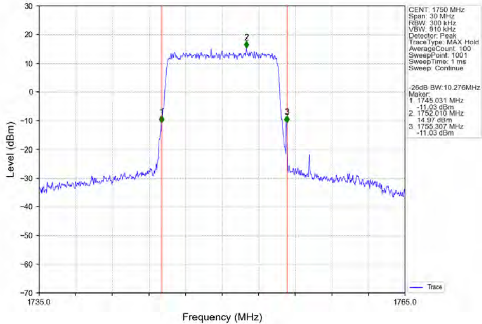
Band4_10MHz_256QAM_HCH_1750MHz_RB_50_0_NTNV
