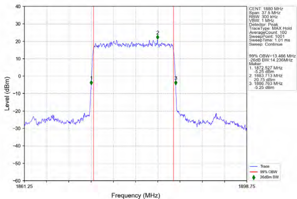
n2_15kHz_SISO_NTNV_15MHz_DFT-s-OFDM PI/2 BPSK_1880MHz_Outer_Full_Ant1
