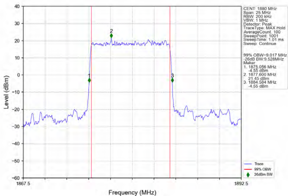
n2_15kHz_SISO_NTNV_10MHz_DFT-s-OFDM PI/2 BPSK_1880MHz_Outer_Full_Ant1
