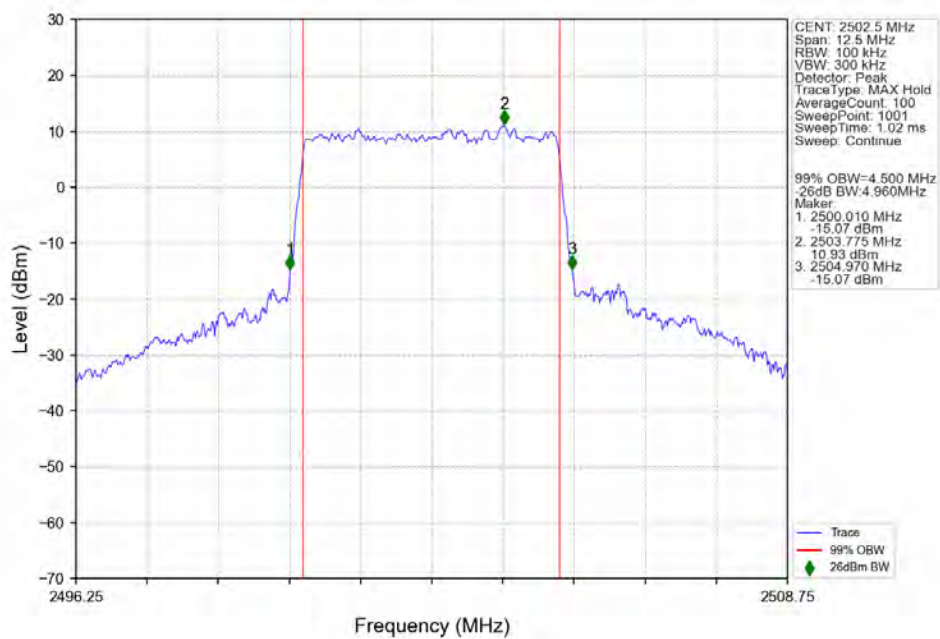
n7_15kHz_SISO_NTNV_5MHz_CP-OFDM_QPSK_2502.5MHz_Outer_Full_Ant1
