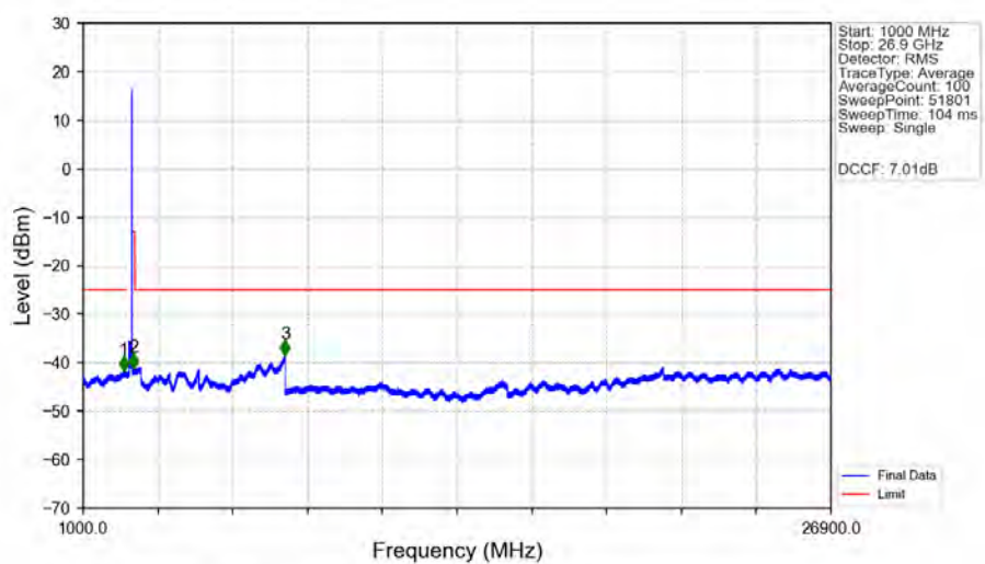
n41_30kHz_MIMO_NTNV_100MHz_DFT-s-OFDM_QPSK_2640MHz_Edge_1RB_Right_Ant1
