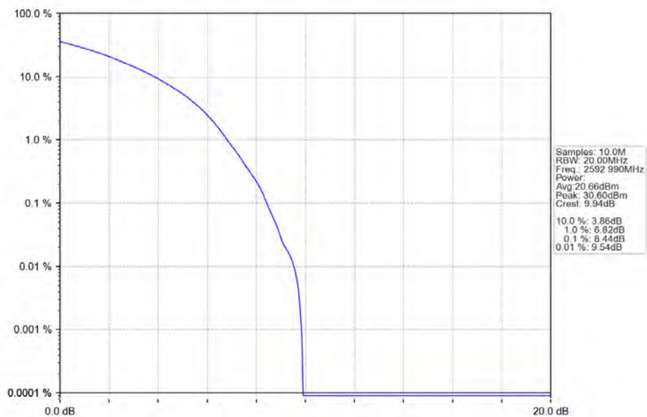
n41_30kHz_SISO_NTNV_20MHz_CP-OFDM_16_QAM_2592.99MHz_Outer_Full_Ant1
