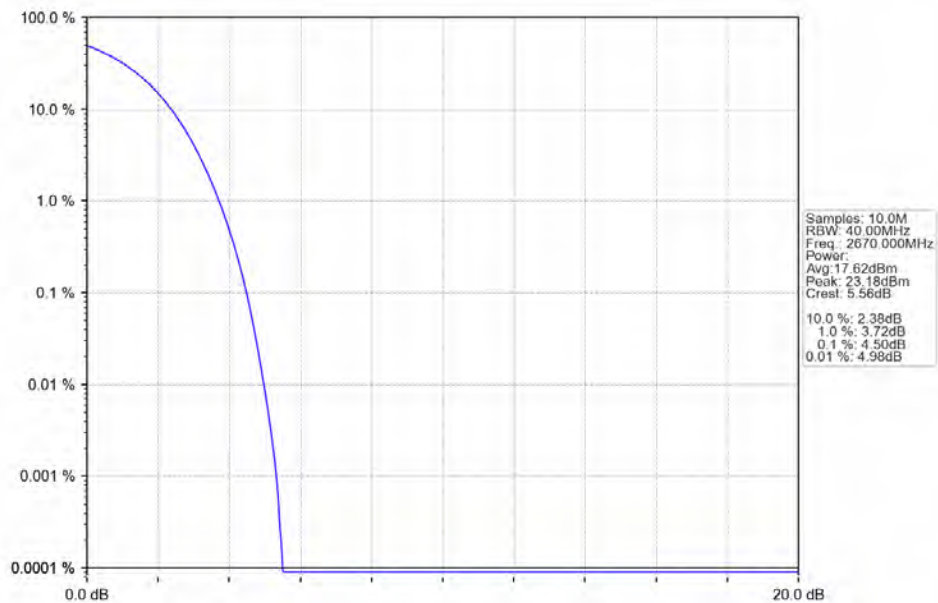
n41_30kHz_SISO_NTNV_40MHz_DFT-s-OFDM_256_QAM_2670MHz_Outer_Full_Ant1
