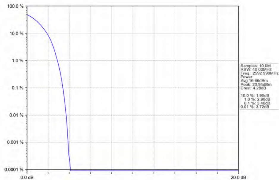
n41_30kHz_SISO_NTNV_30MHz_DFT-s-OFDM PI/2 BPSK_2592.99MHz_Outer_Full_Ant1
