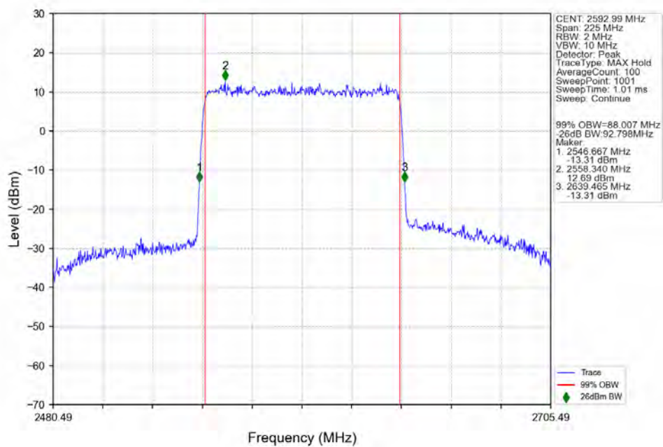
n41_30kHz_SISO_NTNV_90MHz_CP-OFDM_256_QAM_2592.99MHz_Outer_Full_Ant1
