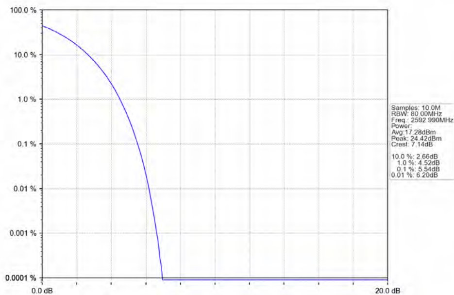
n41_30kHz_SISO_NTNV_80MHz_DFT-s-OFDM PI/2 BPSK_2592.99MHz_Outer_Full_Ant1
