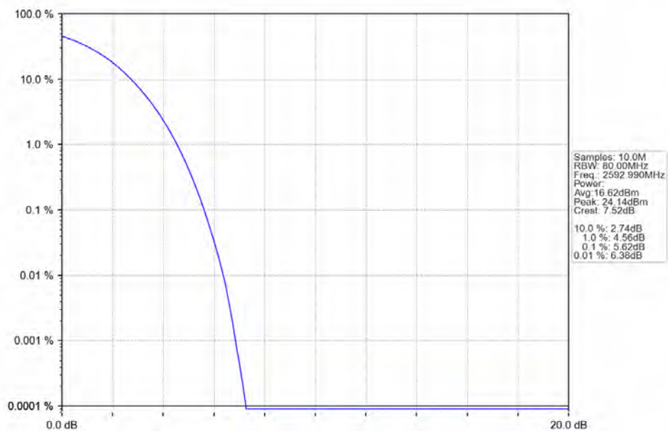
n41_30kHz_SISO_NTNV_60MHz_DFT-s-OFDM_16_QAM_2592.99MHz_Outer_Full_Ant1
