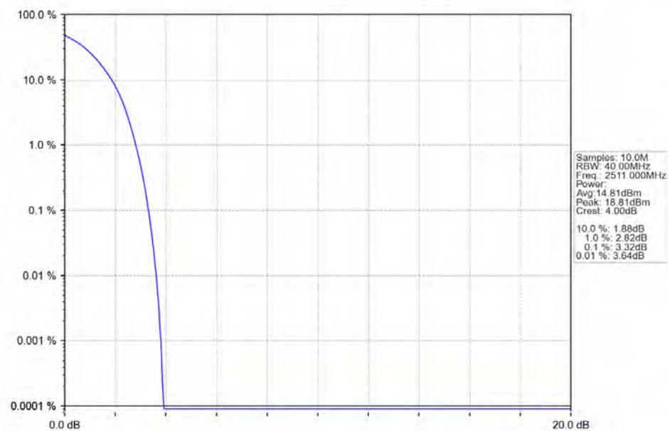
n41_30kHz_SISO_NTNV_30MHz_DFT-s-OFDM PI/2 BPSK_2511MHz_Outer_Full_Ant1
