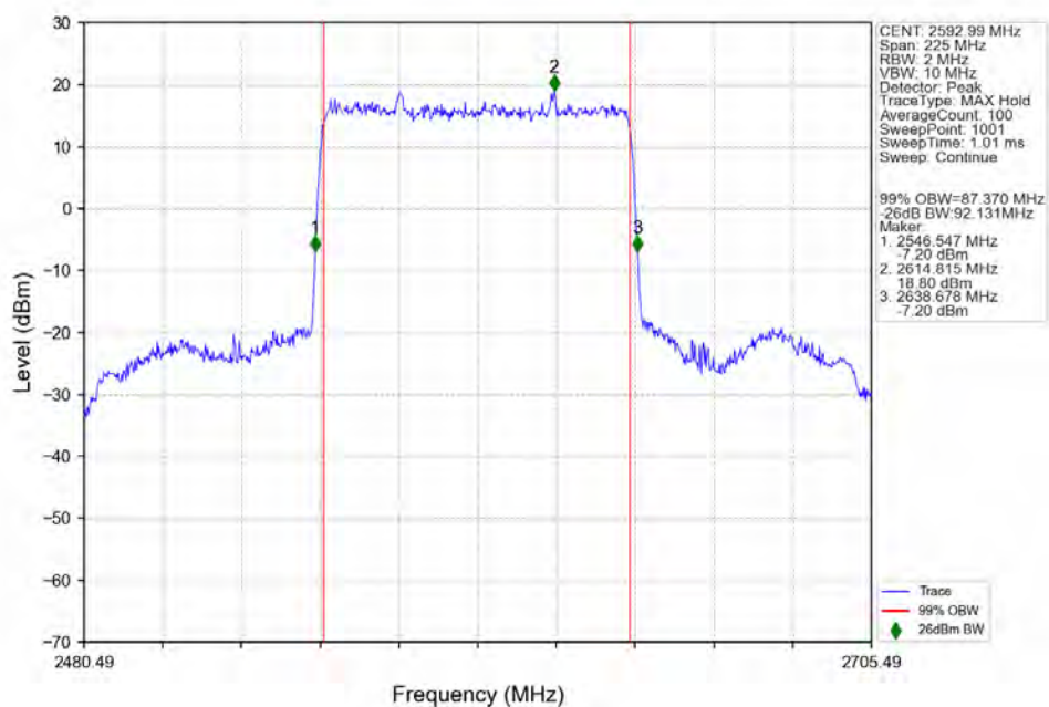
n41_30kHz_SISO_NTNV_90MHz_DFT-s-OFDM PI/2 BPSK_2592.99MHz_Outer_Full_Ant1
