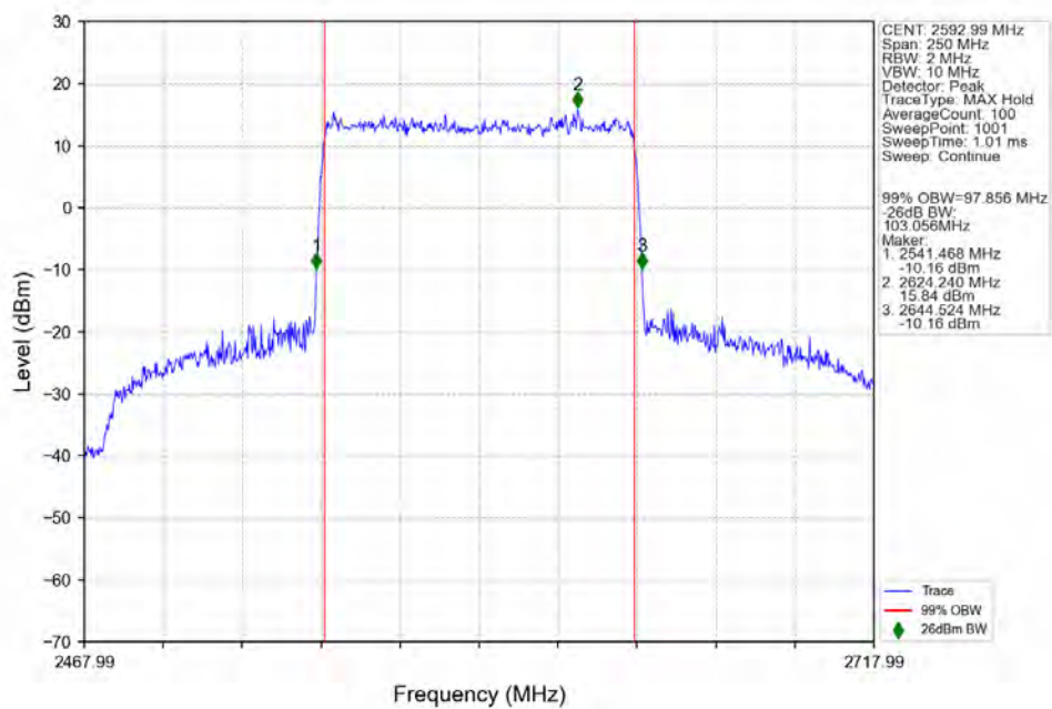
n41_30kHz_SISO_NTNV_100MHz_CP-OFDM_16_QAM_2592.99MHz_Outer_Full_Ant1
