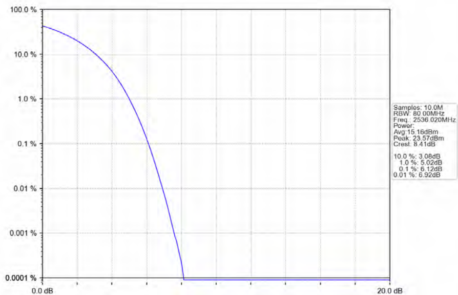
n41_30kHz_SISO_NTNV_80MHz_DFT-s-OFDM_64_QAM_2536.02MHz_Outer_Full_Ant1
