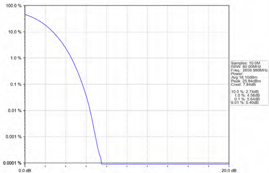
n41_30kHz_SISO_NTNV_60MHz_DFT-s-OFDM_64_QAM_2659.98MHz_Outer_Full_Ant1
