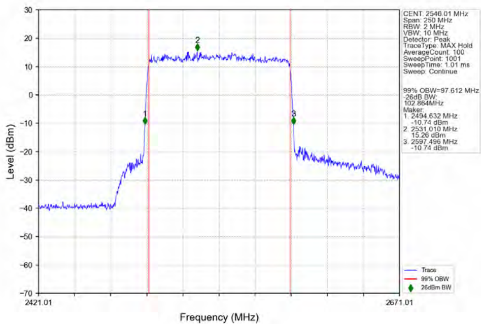
n41_30kHz_SISO_NTNV_100MHz_CP-OFDM_64_QAM_2546.01MHz_Outer_Full_Ant1
