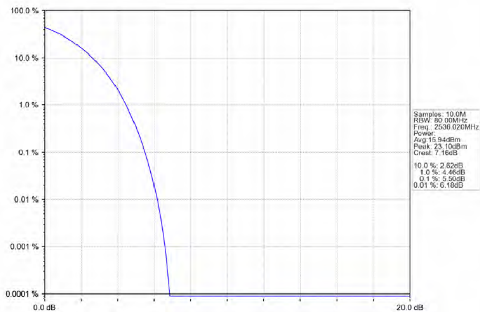
n41_30kHz_SISO_NTNV_80MHz_DFT-s-OFDM PI/2 BPSK_2536.02MHz_Outer_Full_Ant1
