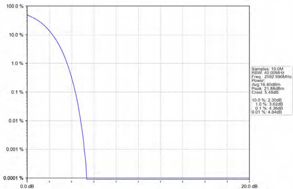
n41_30kHz_SISO_NTNV_40MHz_DFT-s-OFDM_16_QAM_2592.99MHz_Outer_Full_Ant1
