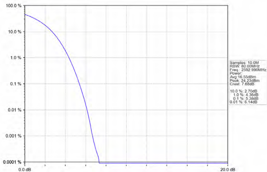
n41_30kHz_SISO_NTNV_50MHz_DFT-s-OFDM_16_QAM_2592.99MHz_Outer_Full_Ant1
