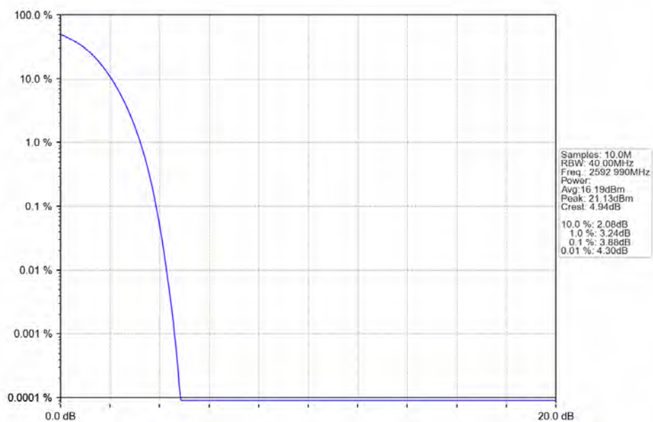
n41_30kHz_SISO_NTNV_30MHz_DFT-s-OFDM_16_QAM_2592.99MHz_Outer_Full_Ant1
