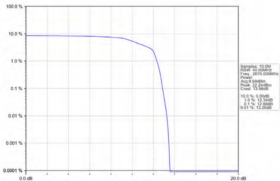
n41_30kHz_SISO_NTNV_40MHz_DFT-s-OFDM_QPSK_2670MHz_Outer_Full_Ant1
