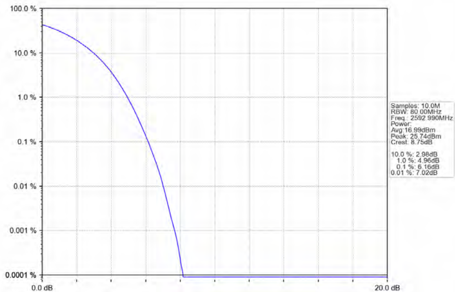
n41_30kHz_SISO_NTNV_80MHz_DFT-s-OFDM_QPSK_2592.99MHz_Outer_Full_Ant1
