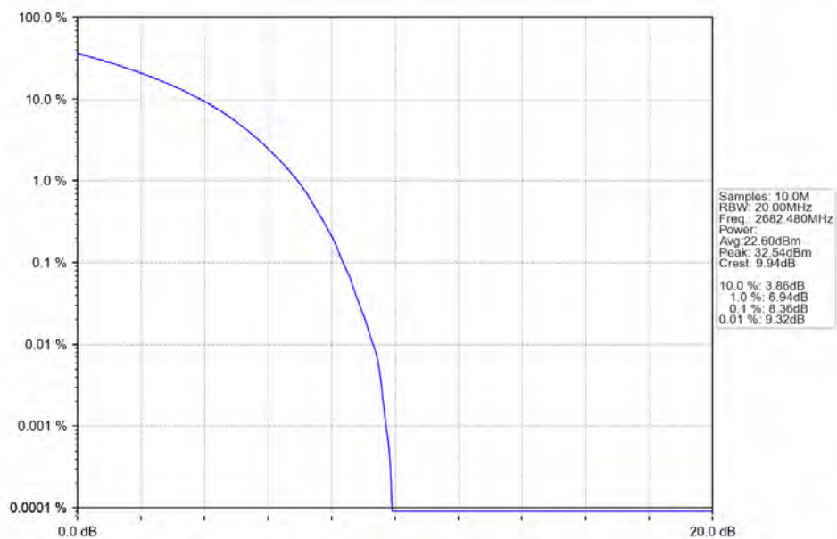
n41_30kHz_SISO_NTNV_15MHz_CP-OFDM_64_QAM_2682.48MHz_Outer_Full_Ant1
