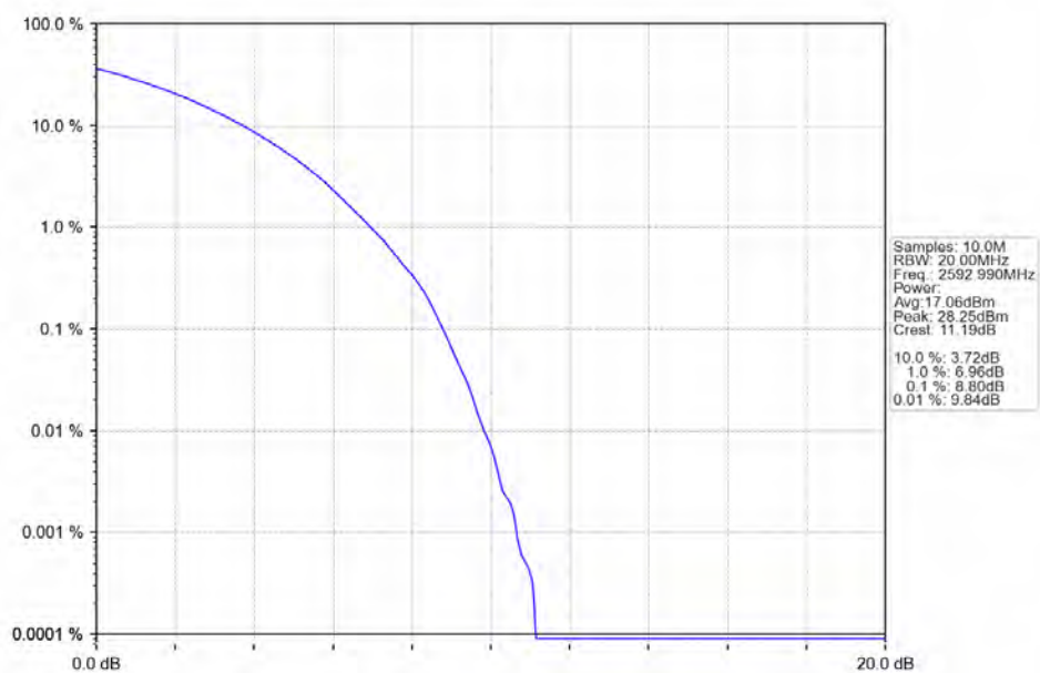
n41_30kHz_SISO_NTNV_20MHz_CP-OFDM_256_QAM_2592.99MHz_Outer_Full_Ant1
