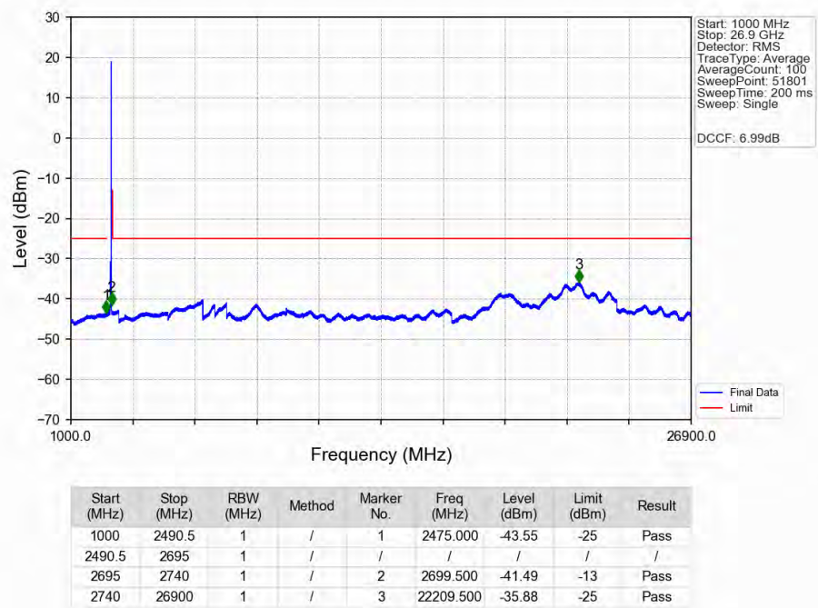
n41_30kHz_SISO_NTNV_50MHz_DFT-s-OFDM_PI/2_BPSK_2664.99MHz_Edge_1RB_Right_Ant1
