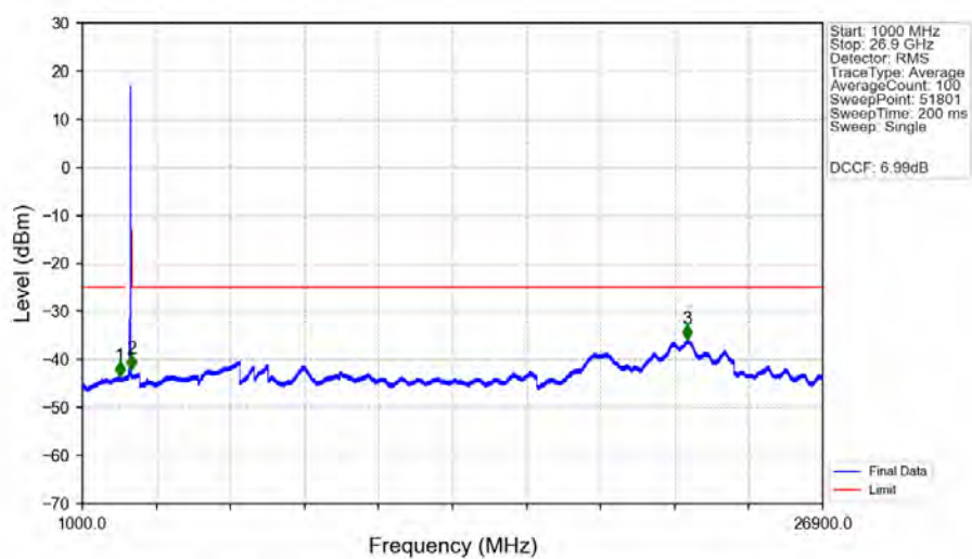
n41_30kHz_SISO_NTNV_40MHz_CP-OFDM_QPSK_2670MHz_Edge_1RB_Right_Ant1
