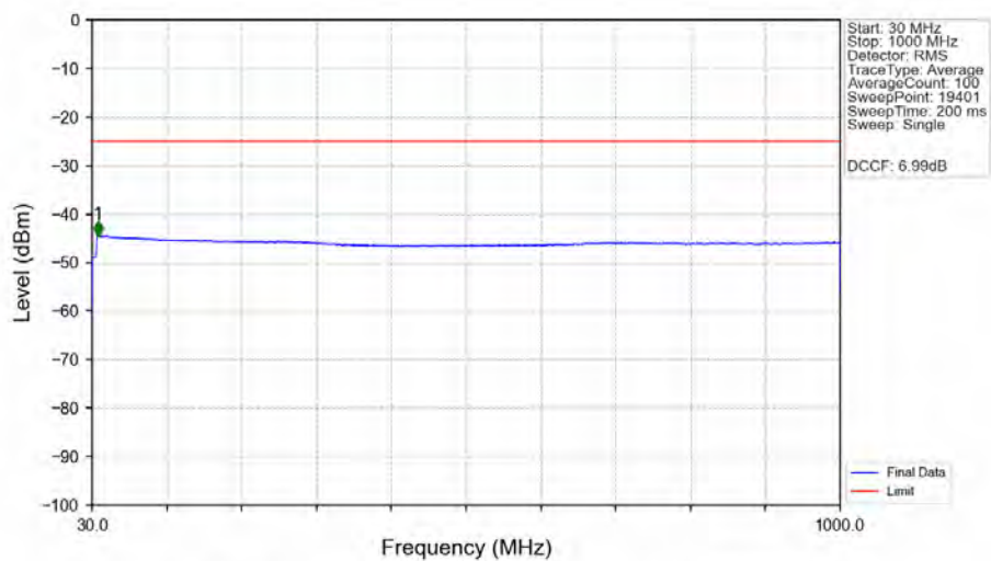
n41_30kHz_SISO_NTNV_40MHz_CP-OFDM_QPSK_2670MHz_Edge_1RB_Right_Ant1
