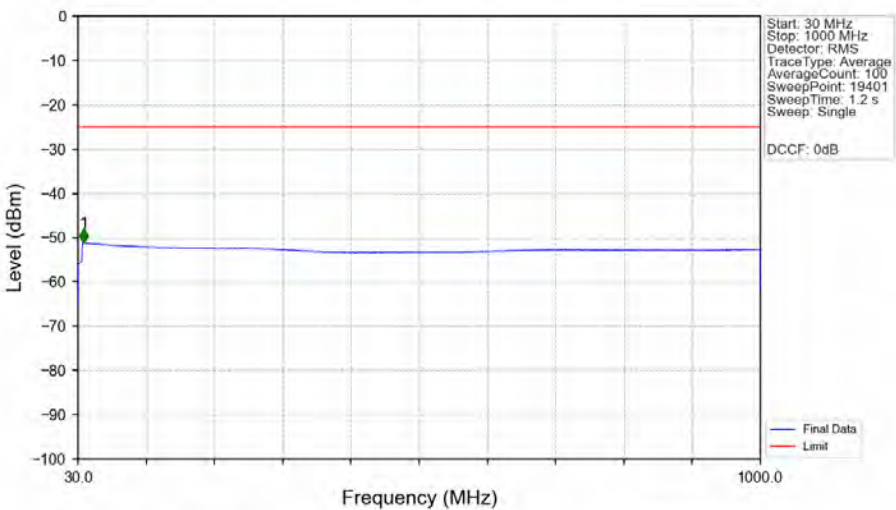
n41_30kHz_SISO_NTNV_80MHz_DFT-s-OFDM_QPSK_2536.02MHz_Edge_1RB_Left_Ant1
