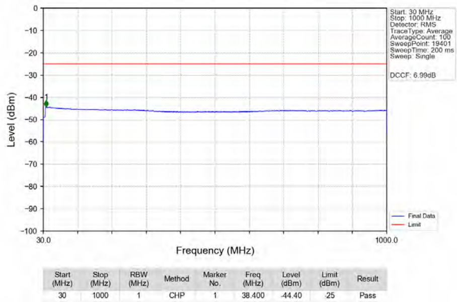
n41_30kHz_SISO_NTNV_50MHz_DFT-s-OFDM_PI/2_BPSK_2664.99MHz_Edge_1RB_Right_Ant1
