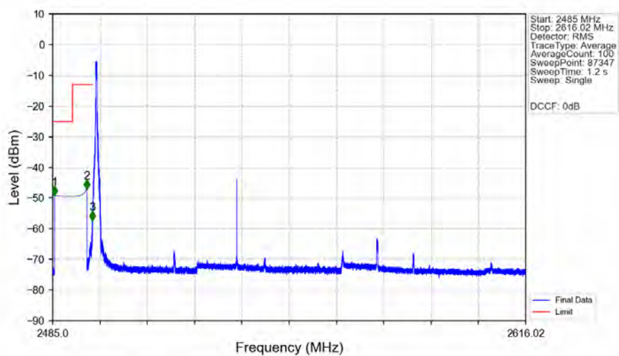
n41_30kHz_SISO_NTNV_80MHz_CP-OFDM_QPSK_2536.02MHz_Edge_1RB_Left_Ant1
