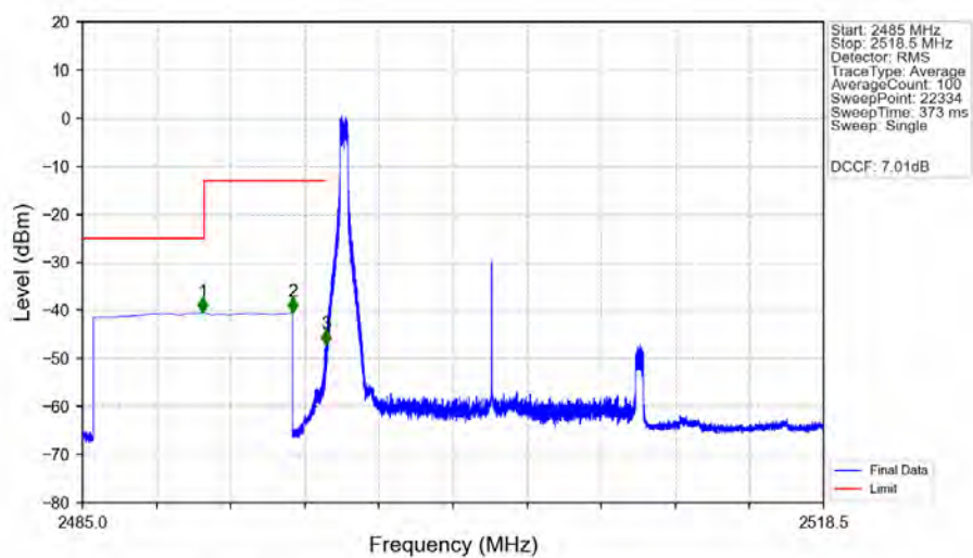
n41_30kHz_MIMO_NTNV_15MHz_CP-OFDM_QPSK_2503.5MHz_Edge_1RB_Left_Ant1
