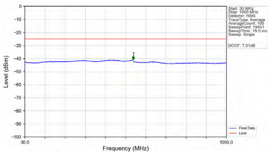
n41_30kHz_MIMO_NTNV_15MHz_CP-OFDM_QPSK_2503.5MHz_Edge_1RB_Left_Ant1
