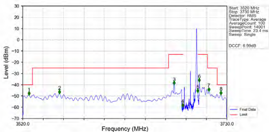
n48_30kHz_SISO_NTNV_15MHz_CP-OFDM_QPSK_3692.49MHz_Inner_1RB_Right_Ant1
