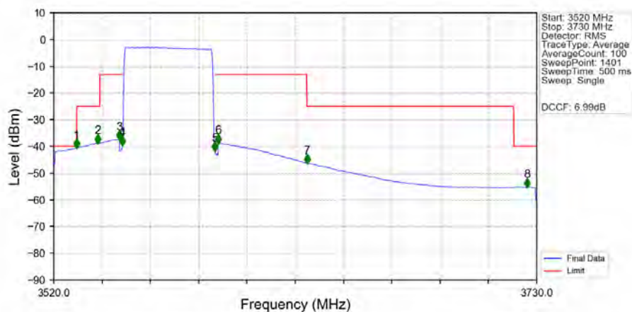
n48_30kHz_SISO_NTNV_40MHz_CP-OFDM_QPSK_3570MHz_Outer_Full_Ant1
