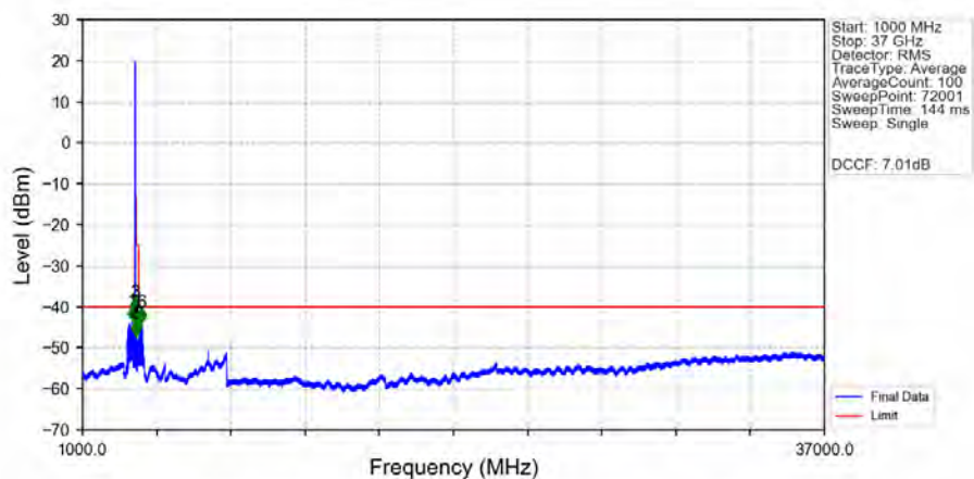
n48_30kHz_SISO_NTNV_20MHz_DFT-s-OFDM PI/2 BPSK_3560.01MHz_Edge_1RB_Left_Ant1
