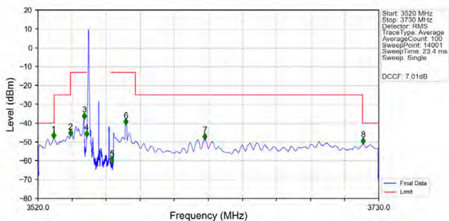
n48_30kHz_SISO_NTNV_15MHz_CP-OFDM_QPSK_3557.52MHz_Inner_1RB_Left Ant1
