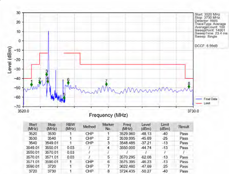
n48_30kHz_SISO_NTNV_20MHz_DFT-s-OFDM_QPSK_3560.01MHz_Edge_1RB_Left_Ant1
