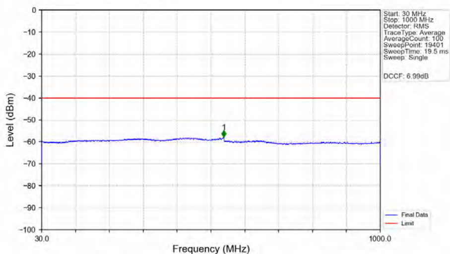
n48_30kHz_SISO_NTNV_20MHz_CP-OFDM_QPSK_3690MHz_Edge_1RB_Right_Ant1
