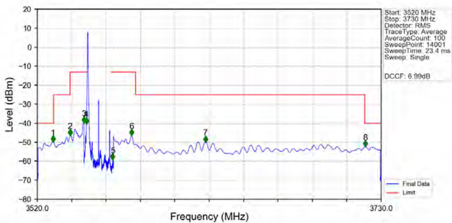
n48_30kHz_SISO_NTNV_15MHz_CP-OFDM_QPSK_3557.52MHz_Edge_1RB_Left_Ant1
