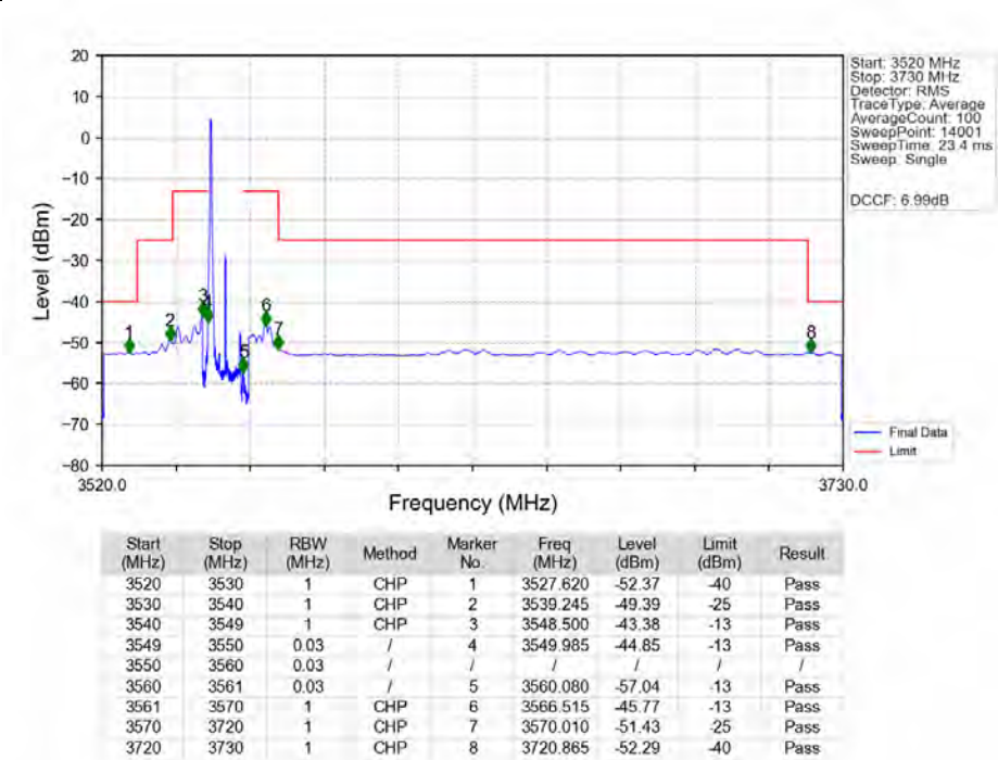
n48_30kHz_MIMO_NTNV_10MHz_CP-OFDM_QPSK_3555MHz_Edge_1RB_Left_Ant1
