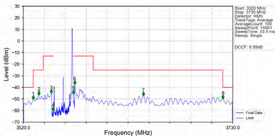
n48_30kHz_SISO_NTNV_20MHz_DFT-s-OFDM PI/2 BPSK_3560.01MHz_Edge_1RB_Right_Ant1
