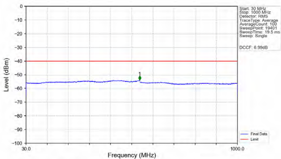
n48_30kHz_SISO_NTNV_15MHz_CP-OFDM_QPSK_3557.52MHz_Edge_1RB_Left_Ant1
