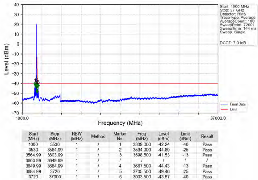
n48_30kHz_SISO_NTNV_40MHz_DFT-s-OFDM_QPSK_3624.99MHz_Edge_1RB_Left_Ant1
