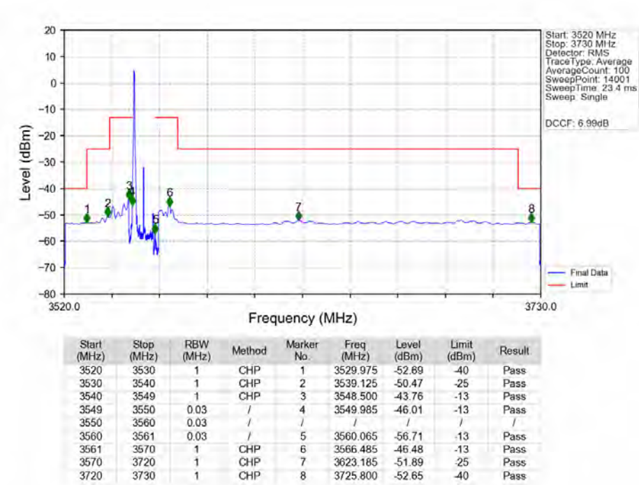
n48_30kHz_MIMO_NTNV_10MHz_CP-OFDM_QPSK_3555MHz_Edge_1RB_Left_Ant2
