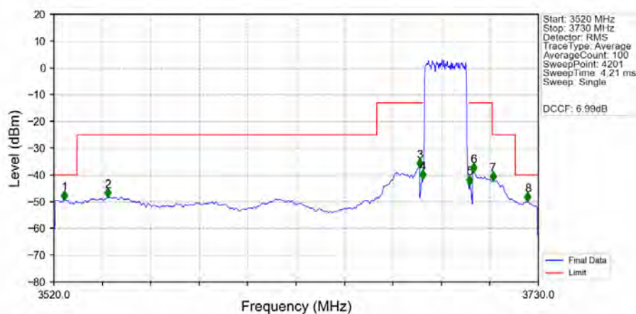
n48_30kHz_SISO_NTNV_20MHz_DFT-s-OFDM_PI/2_BPSK_3690MHz_Outer_Full_Ant1
