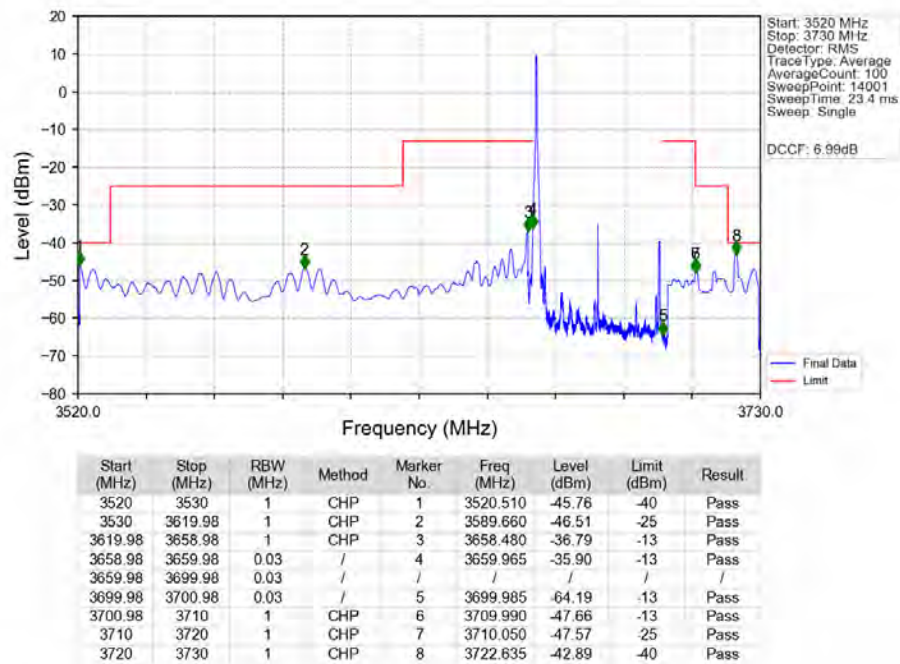
n48_30kHz_SISO_NTNV_40MHz_DFT-s-OFDM_QPSK_3679.98MHz_Edge_1RB_Left_Ant1
