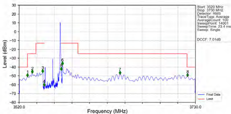
n48_30kHz_SISO_NTNV_20MHz_DFT-s-OFDM_QPSK_3560.01MHz_Edge_1RB_Right_Ant1
