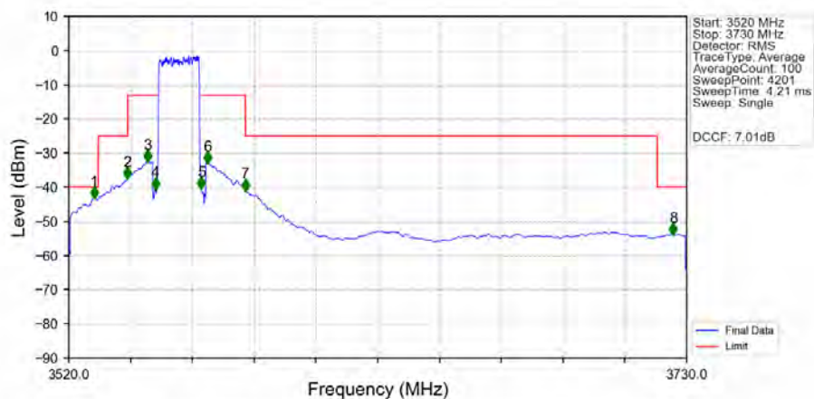
n48_30kHz_SISO_NTNV_15MHz_CP-OFDM_QPSK_3557.52MHz_Outer_Full_Ant1
