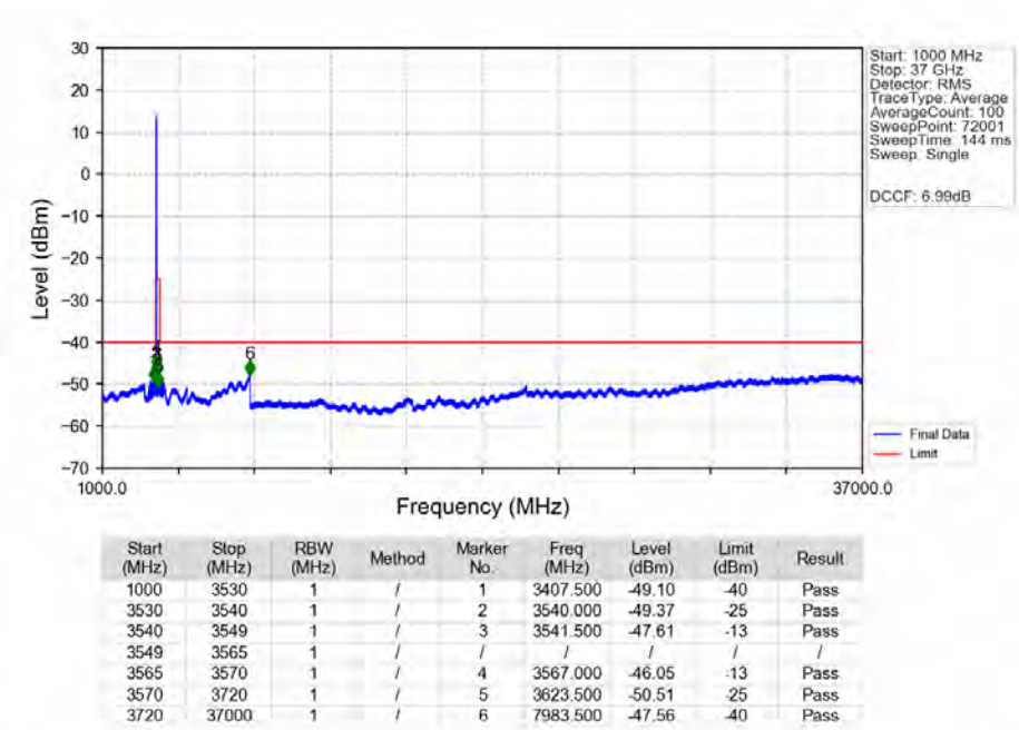
n48_30kHz_MIMO_NTNV_10MHz_CP-OFDM_QPSK_3555MHz_Edge_1RB_Left_Ant1
