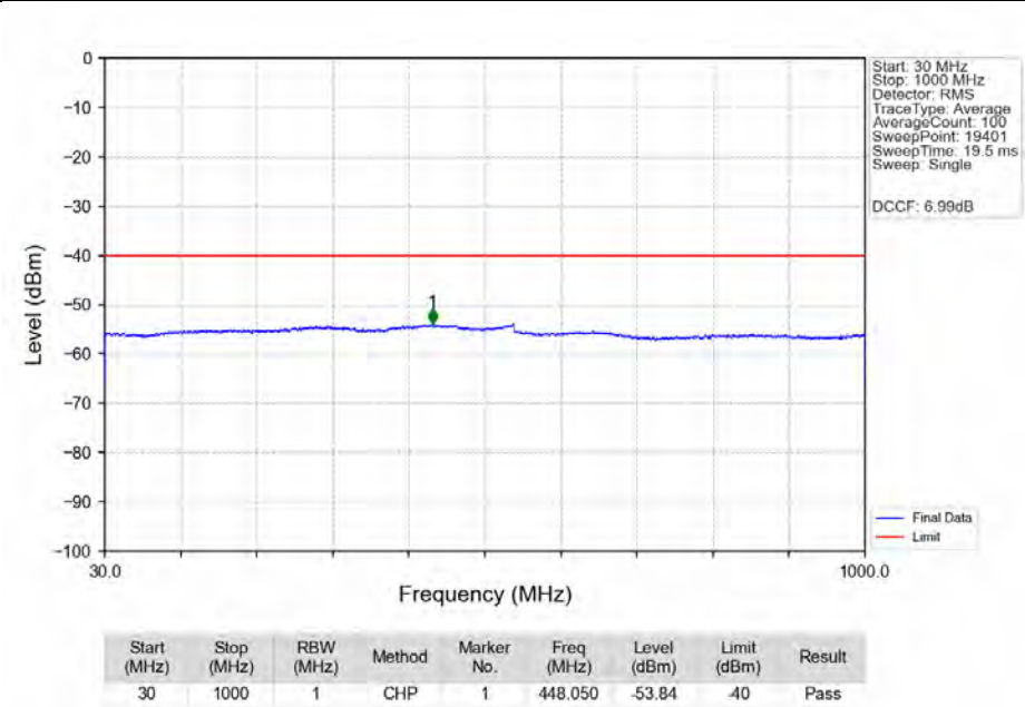
n48_30kHz_SISO_NTNV_20MHz_DFT-s-OFDM_QPSK_3560.01MHz_Edge_1RB_Left_Ant1
