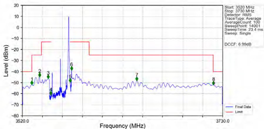
n48_30kHz_SISO_NTNV_20MHz_CP-OFDM_QPSK_3560.01MHz_Inner_1RB_Right_Ant1
