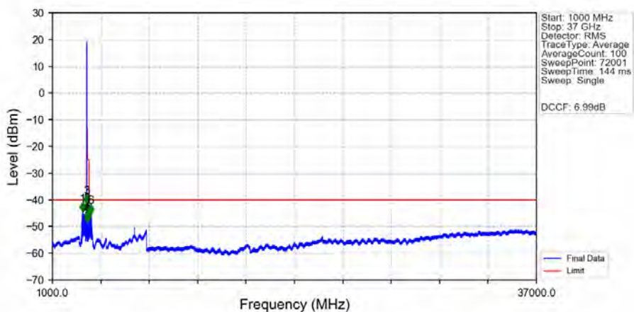
n48_30kHz_SISO_NTNV_20MHz_DFT-s-OFDM_QPSK_3560.01MHz_Edge_1RB_Left_Ant1
