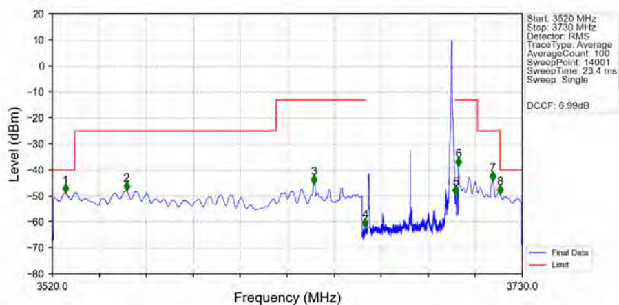
n48_30kHz_SISO_NTNV_40MHz_CP-OFDM_QPSK_3679.98MHz_Inner_1RB_Right_Ant1
