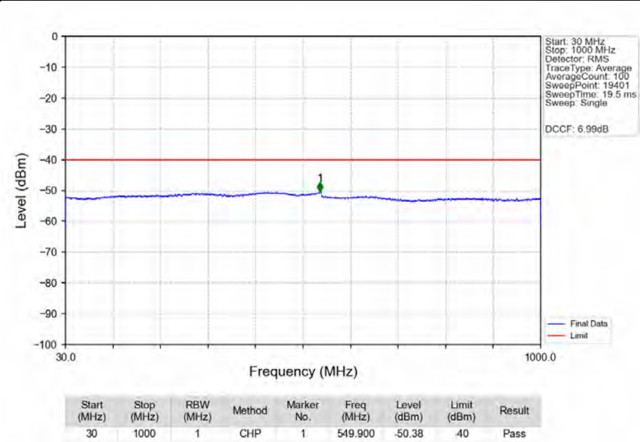
n48_30kHz_MIMO_NTNV_10MHz_CP-OFDM_QPSK_3555MHz_Edge_1RB_Left_Ant1
