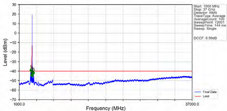
n48_30kHz_SISO_NTNV_20MHz_DFT-s-OFDM_PI/2_BPSK_3690MHz_Edge_1RB_Right_Ant1
