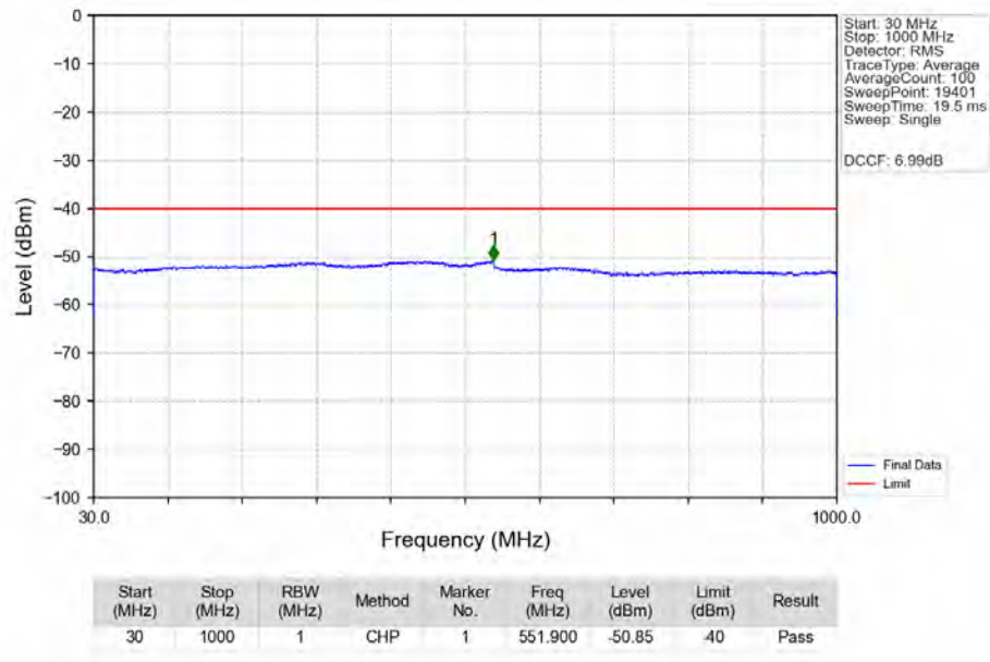
n48_30kHz_MIMO_NTNV_15MHz_DFT-s-OFDM_PI/2_BPSK_3557.52MHz_Edge_1RB_Left_Ant2
