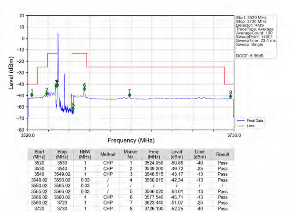
n48_30kHz_MIMO_NTNV_15MHz_CP-OFDM_QPSK_3557.52MHz_Edge_1RB_Left_Ant1
