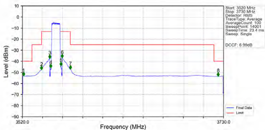
n48_30kHz_MIMO_NTNV_10MHz_CP-OFDM_QPSK_3555MHz_Outer_Full_Ant2
