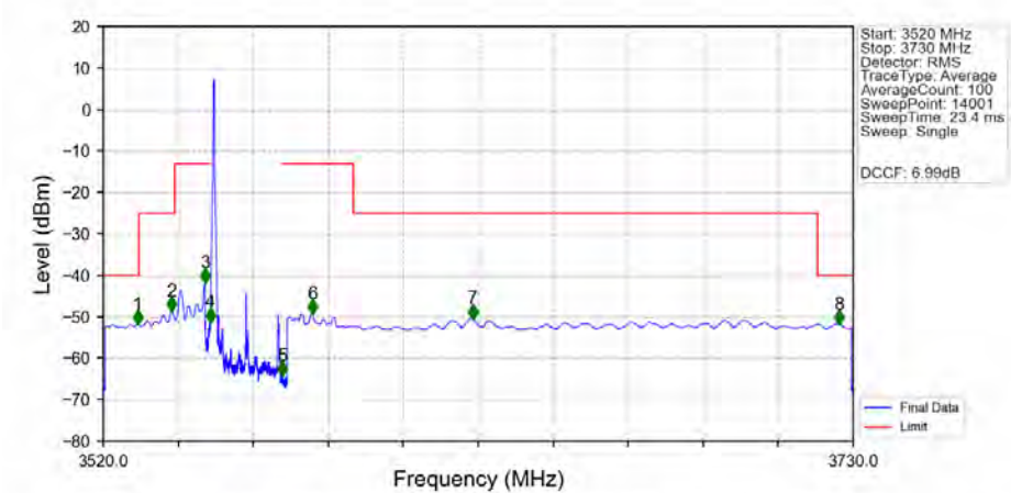
n48_30kHz_MIMO_NTNV_20MHz_DFT-s-OFDM_QPSK_3560.01MHz_Edge_1RB_Left_Ant1
