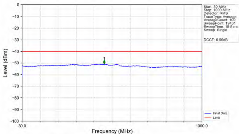
n48_30kHz_MIMO_NTNV_20MHz_DFT-s-OFDM_PI/2_BPSK_3560.01MHz_Edge_1RB_Left_Ant2
