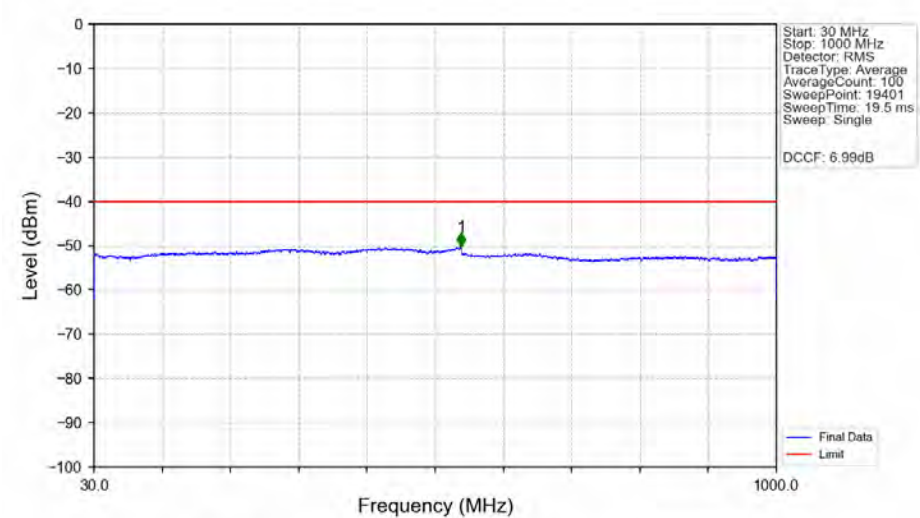
n48_30kHz_MIMO_NTNV_20MHz_DFT-s-OFDM_QPSK_3560.01MHz_Edge_1RB_Left_Ant1
