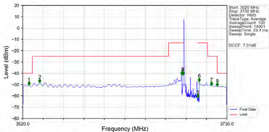
n48_30kHz_MIMO_NTNV_15MHz_DFT-s-OFDM_PI/2_BPSK_3692.49MHz_Edge_1RB_Left_Ant2
