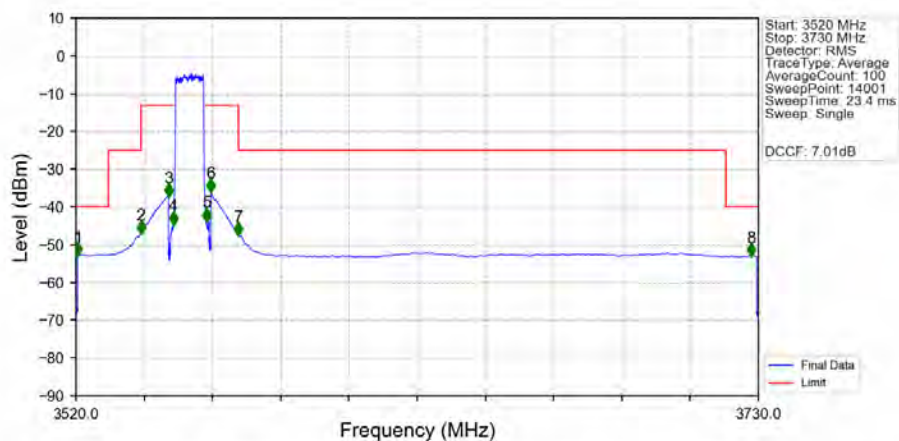
n48_30kHz_MIMO_NTNV_10MHz_CP-OFDM_QPSK_3555MHz_Outer_Full_Ant1
