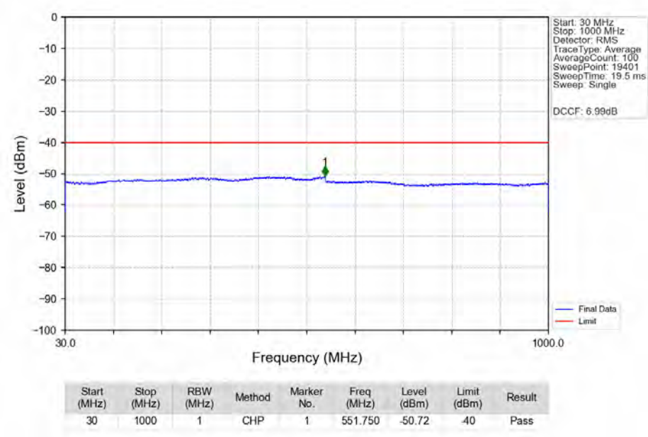
n48_30kHz_MIMO_NTNV_15MHz_CP-OFDM_QPSK_3557.52MHz_Edge_1RB_Left_Ant2
