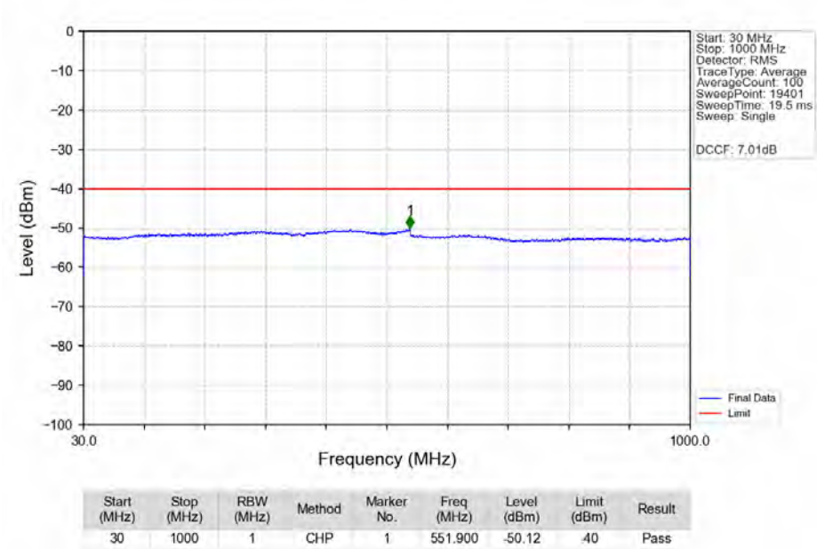
n48_30kHz_MIMO_NTNV_15MHz_DFT-s-OFDM_QPSK_3557.52MHz_Edge_1RB_Left_Ant1
