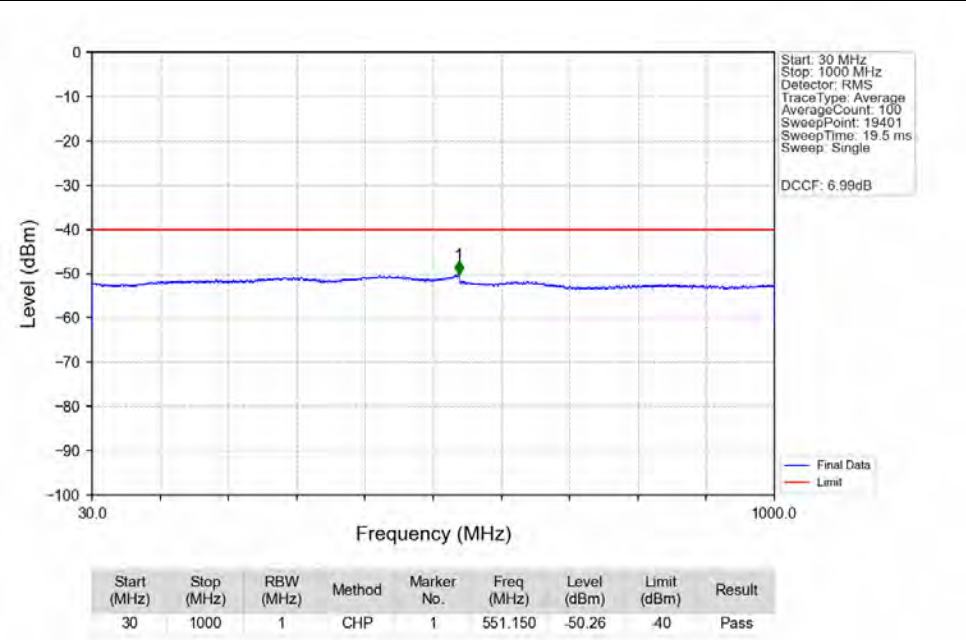
n48_30kHz_MIMO_NTNV_15MHz_CP-OFDM_QPSK_3557.52MHz_Edge_1RB_Left_Ant1
