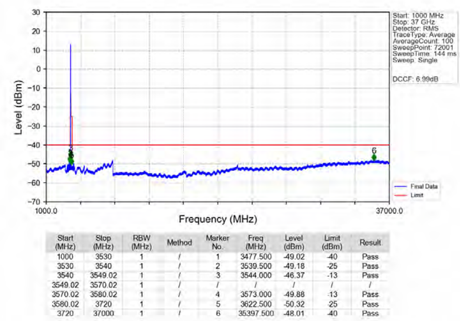
n48_30kHz_MIMO_NTNV_15MHz_CP-OFDM_QPSK_3557.52MHz_Edge_1RB_Left_Ant2
