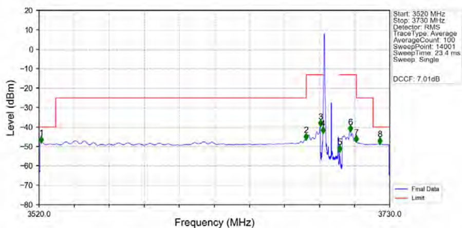
n48_30kHz_MIMO_NTNV_10MHz_CP-OFDM_QPSK_3694.98MHz_Edge_1RB_Left_MIMO
