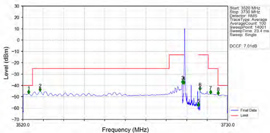
n48_30kHz_MIMO_NTNV_15MHz_DFT-s-OFDM_PI/2_BPSK_3692.49MHz_Edge_1RB_Left_MIMO
