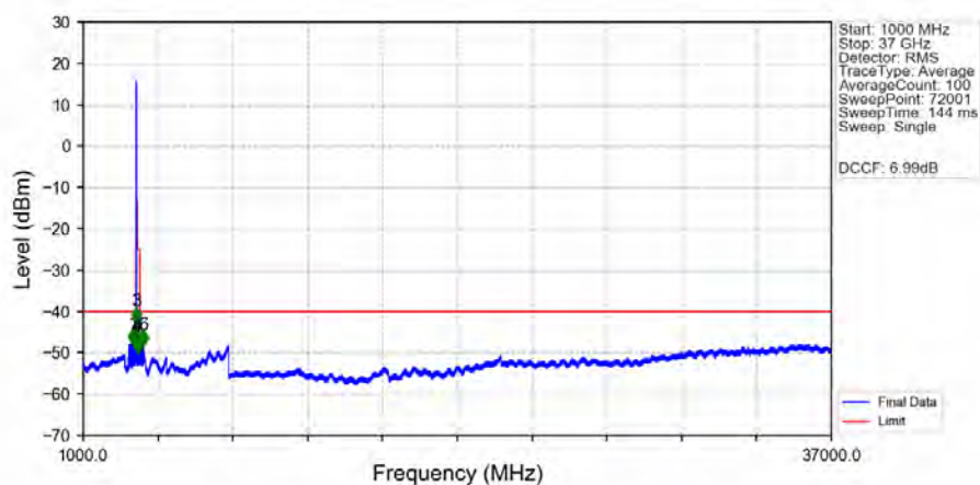
n48_30kHz_MIMO_NTNV_20MHz_DFT-s-OFDM_PI/2_BPSK_3560.01MHz_Edge_1RB_Left_Ant2
