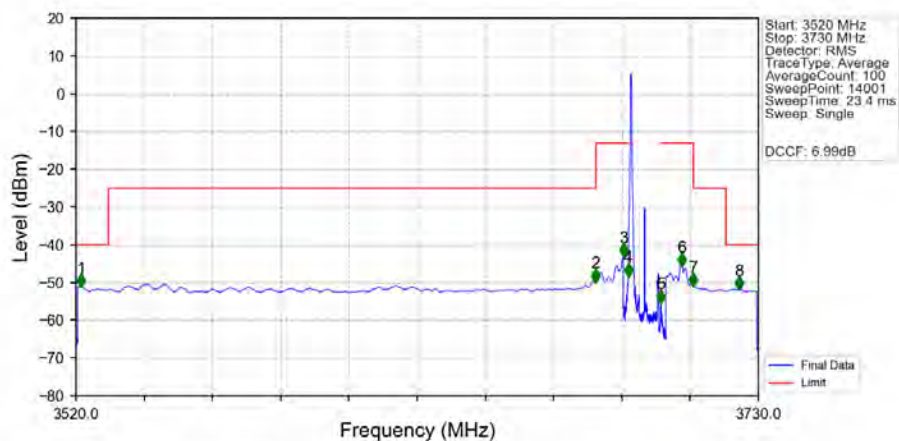
n48_30kHz_MIMO_NTNV_10MHz_CP-OFDM_QPSK_3694.98MHz_Edge_1RB_Left_Ant2
