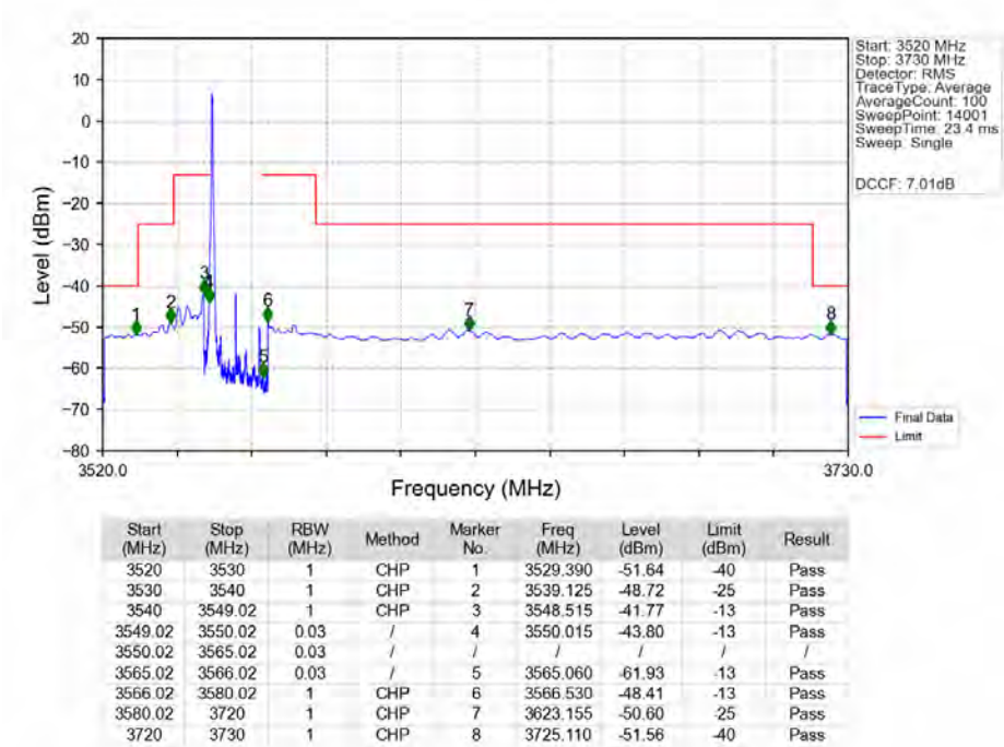
n48_30kHz_MIMO_NTNV_15MHz_DFT-s-OFDM_QPSK_3557.52MHz_Edge_1RB_Left_Ant1
