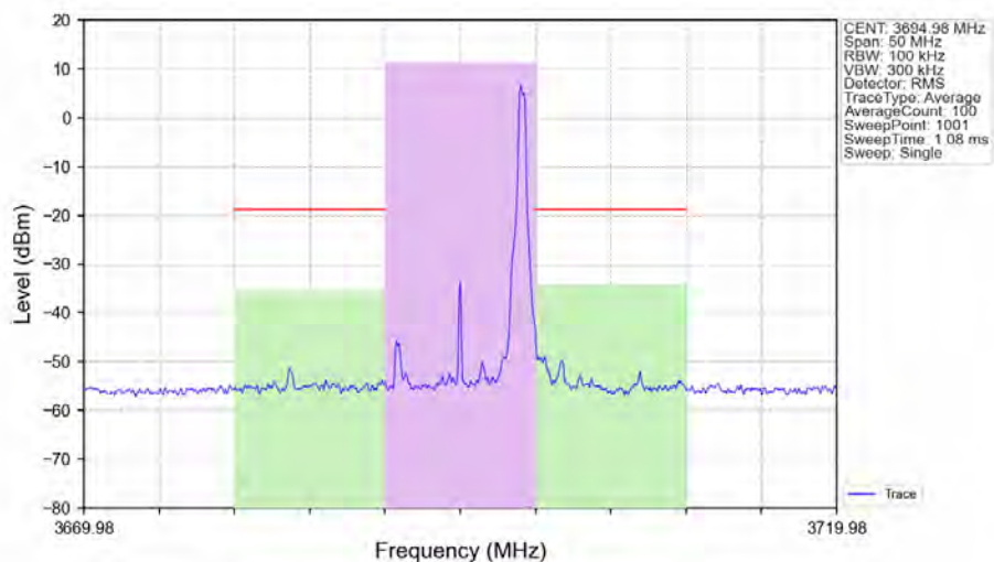
n48_30kHz_SISO_NTNV_10MHz_DFT-s-OFDM 256 QAM 3694.98MHz_Edge_1RB_Right_Ant1
