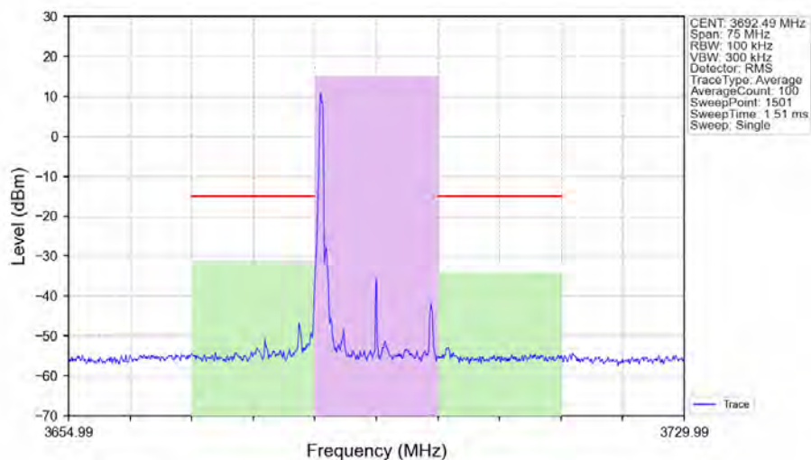
n48_30kHz_SISO_NTNV_15MHz_DFT-s-OFDM_64_QAM_3692.49MHz_Edge_1RB_Left_Ant1
