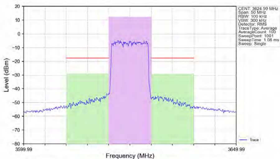
n48_30kHz_SISO_NTNV_10MHz_CP-OFDM 16 QAM 3624.99MHz_Outer_Full_Ant1
