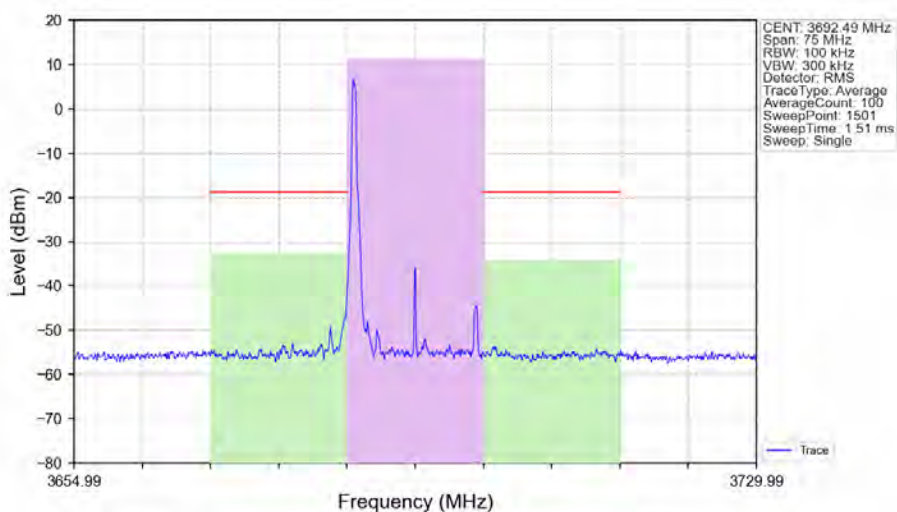
n48_30kHz_SISO_NTNV_15MHz_DFT-s-OFDM_256_QAM_3692.49MHz_Edge_1RB_Left_Ant1
