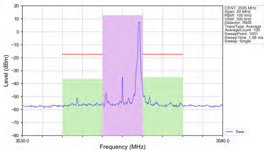
n48_30kHz_SISO_NTNV_10MHz_CP-OFDM 64 QAM 3555MHz_Edge_1RB_Right_Ant1
