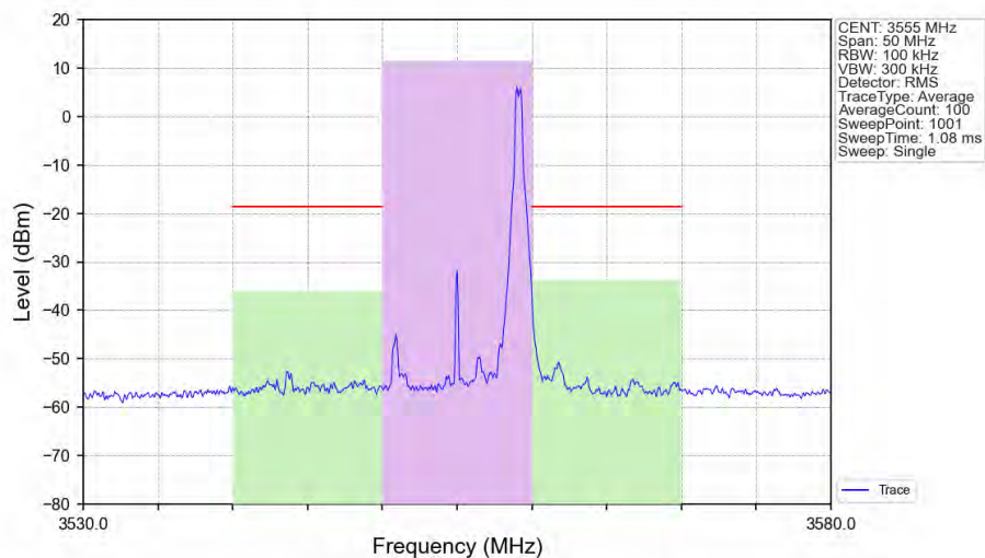
n48_30kHz_SISO_NTNV_10MHz_CP-OFDM 16 QAM 3555MHz_Edge_1RB_Right_Ant1
