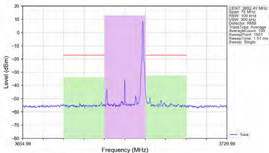
n48_30kHz_SISO_NTNV_15MHz_DFT-s-OFDM_64_QAM_3692.49MHz_Edge_1RB_Right_Ant1
