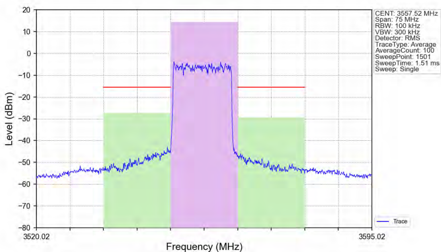
n48_30kHz_SISO_NTNV_15MHz_DFT-s-OFDM QPSK 3557.52MHz_Outer_Full_Ant1
