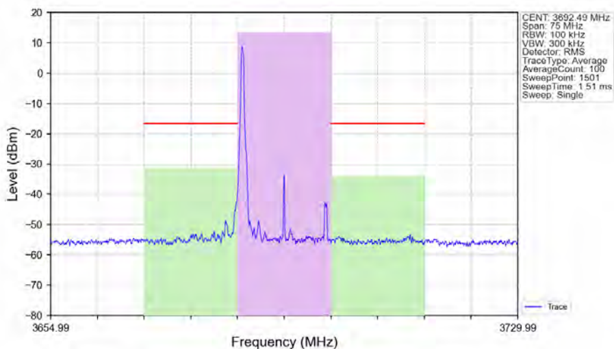
n48_30kHz_SISO_NTNV_15MHz_CP-OFDM_QPSK_3692.49MHz_Edge_1RB_Left_Ant1
