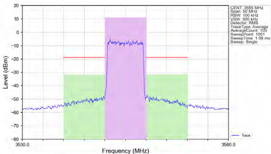
n48_30kHz_SISO_NTNV_10MHz_DFT-s-OFDM 256 QAM 3555MHz_Outer_Full_Ant1
