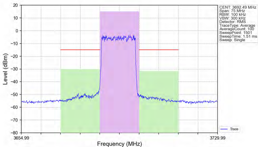
n48_30kHz_SISO_NTNV_15MHz_DFT-s-OFDM_PI/2_BPSK_3692.49MHz_Outer_Full_Ant1
