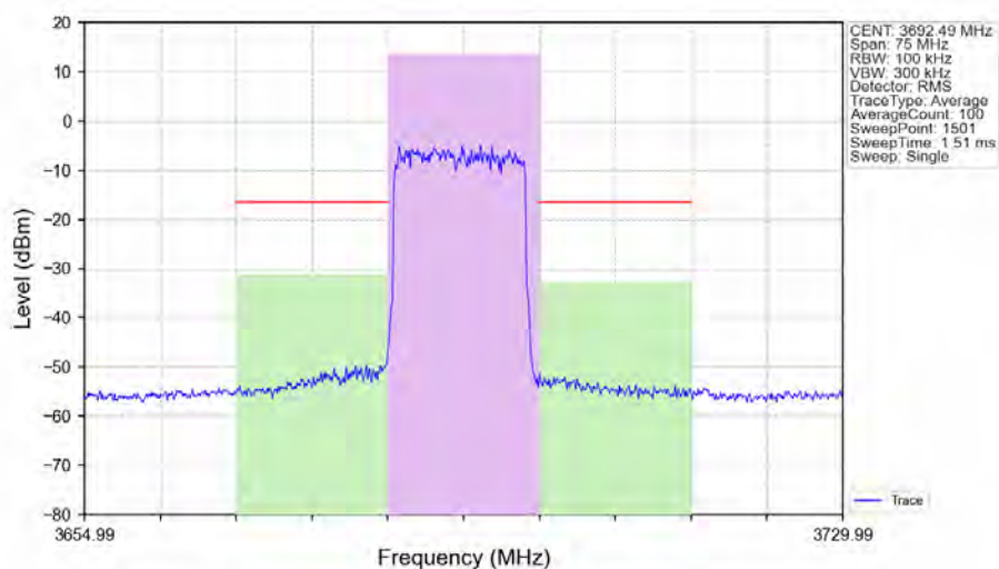
n48_30kHz_SISO_NTNV_15MHz_DFT-s-OFDM 64 QAM_3692.49MHz_Outer_Full_Ant1
