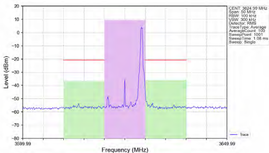
n48_30kHz_SISO_NTNV_10MHz_CP-OFDM 256 QAM 3624.99MHz_Edge_1RB_Right_Ant1
