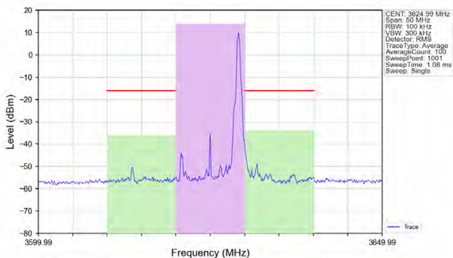
n48_30kHz_SISO_NTNV_10MHz_DFT-s-OFDM_16_QAM_3624.99MHz_Edge_1RB_Right_Ant1
