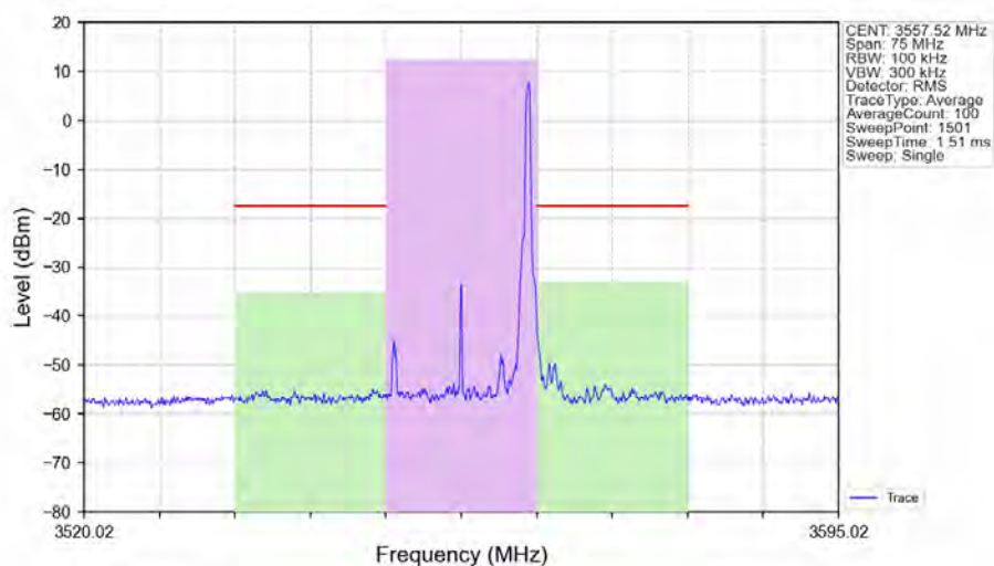
n48_30kHz_SISO_NTNV_15MHz_CP-OFDM_QPSK_3557.52MHz_Edge_1RB_Right_Ant1
