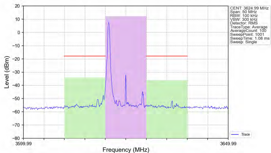
n48_30kHz_SISO_NTNV_10MHz_CP-OFDM_64_QAM_3624.99MHz_Edge_1RB_Left_Ant1
