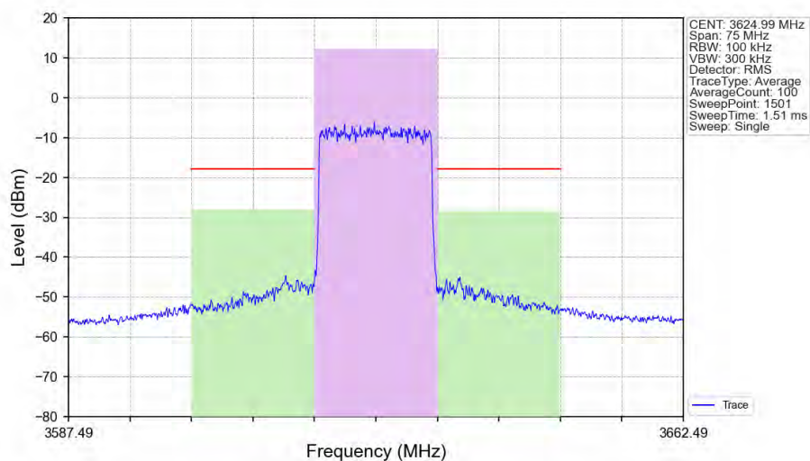
n48_30kHz_SISO_NTNV_15MHz_CP-OFDM 16 QAM 3624.99MHz_Outer_Full_Ant1
