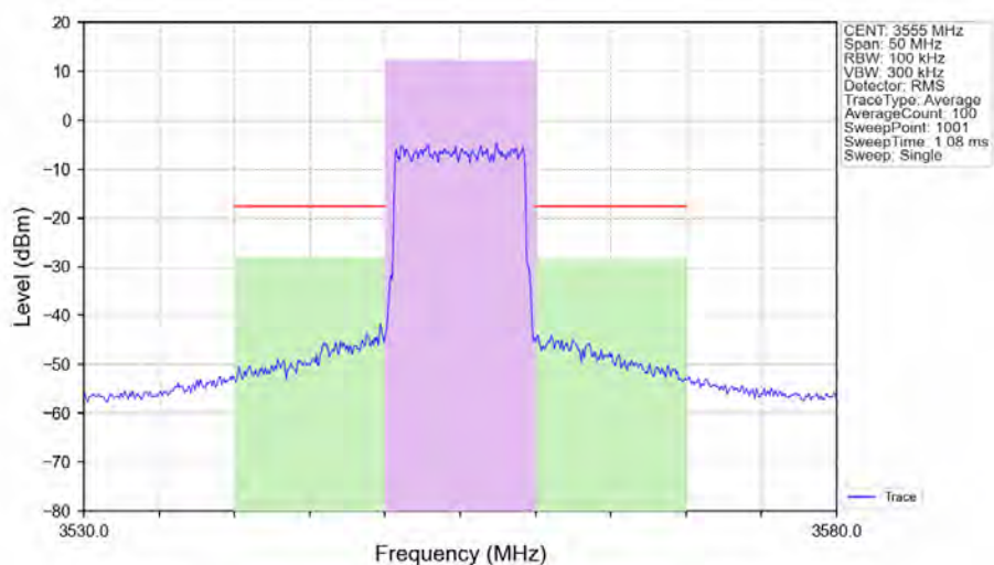
n48_30kHz_SISO_NTNV_10MHz_CP-OFDM QPSK 3555MHz_Outer_Full_Ant1
