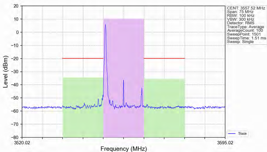
n48_30kHz_SISO_NTNV_15MHz_DFT-s-OFDM_256_QAM_3557.52MHz_Edge_1RB_Left_Ant1
