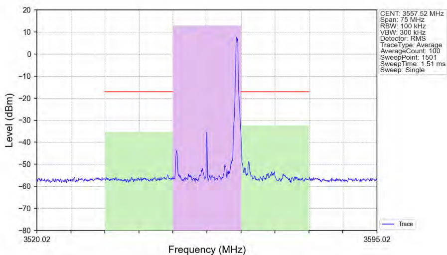
n48_30kHz_SISO_NTNV_15MHz_DFT-s-OFDM_64_QAM_3557.52MHz_Edge_1RB_Right_Ant1
