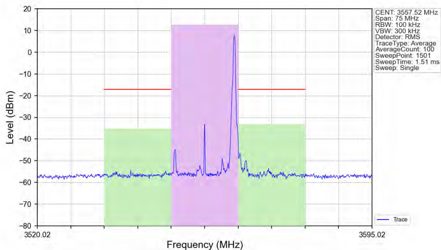
n48_30kHz_SISO_NTNV_15MHz_CP-OFDM 16 QAM 3557.52MHz_Edge_1RB_Right_Ant1
