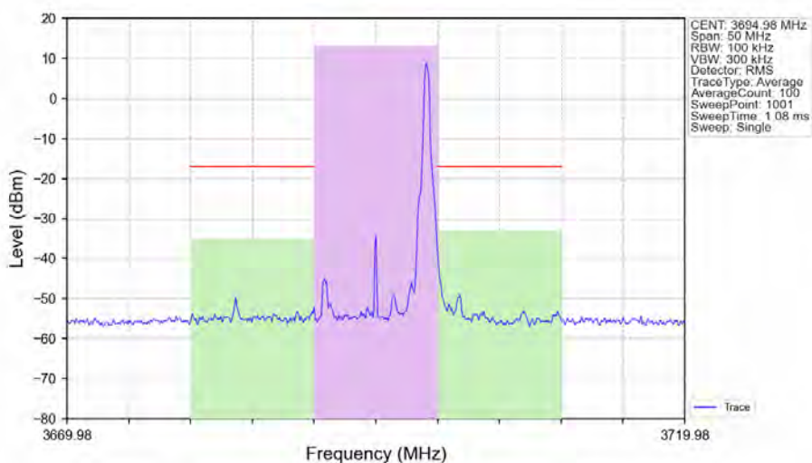
n48_30kHz_SISO_NTNV_10MHz_DFT-s-OFDM_64_QAM_3694.98MHz_Edge_1RB_Right_Ant1
