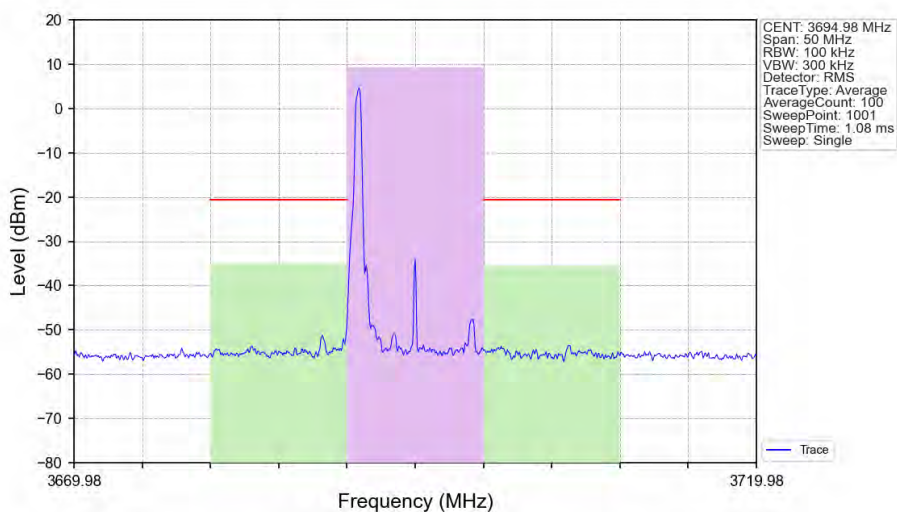
n48_30kHz_SISO_NTNV_10MHz_CP-OFDM 256 QAM 3694.98MHz_Edge_1RB_Left_Ant1
