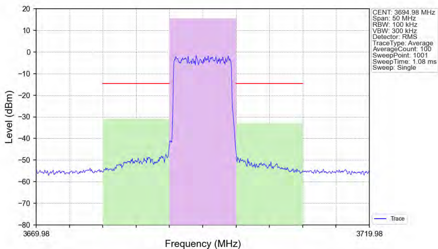
n48_30kHz_SISO_NTNV_10MHz_DFT-s-OFDM_PI/2_BPSK_3694.98MHz_Outer_Full_Ant1
