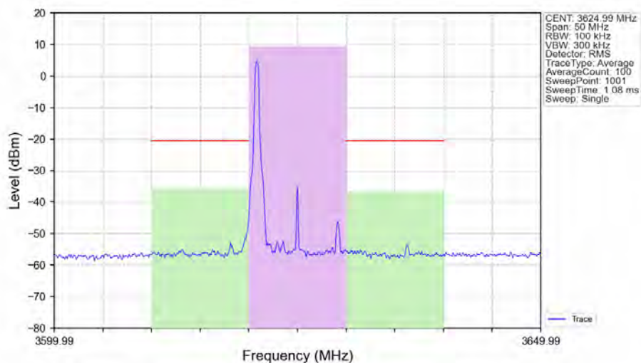
n48_30kHz_SISO_NTNV_10MHz_CP-OFDM 256 QAM 3624.99MHz_Edge_1RB_Left_Ant1
