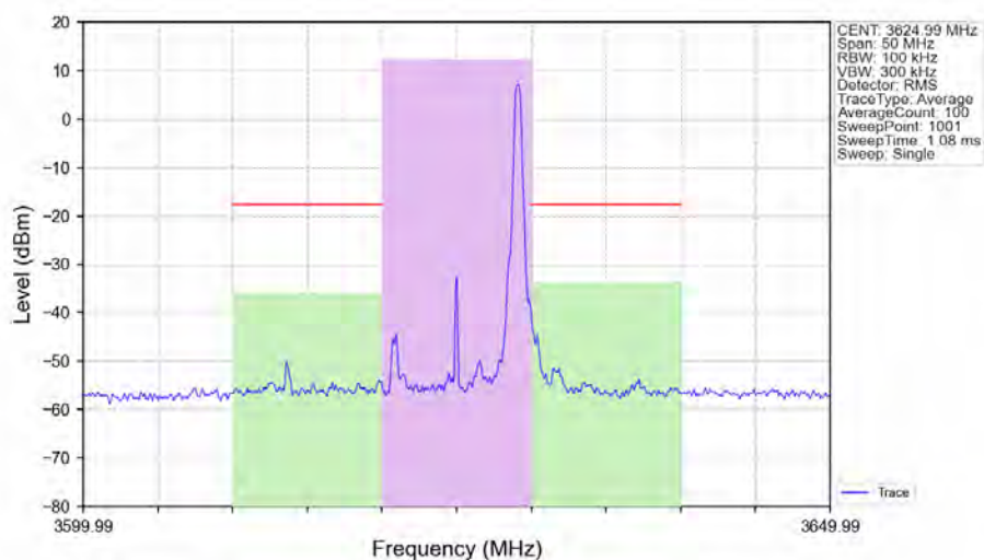
n48_30kHz_SISO_NTNV_10MHz_CP-OFDM_16_QAM_3624.99MHz_Edge_1RB_Right_Ant1
