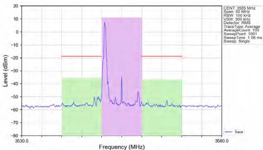
n48_30kHz_SISO_NTNV_10MHz_DFT-s-OFDM 256 QAM 3555MHz_Edge_1RB_Left_Ant1
