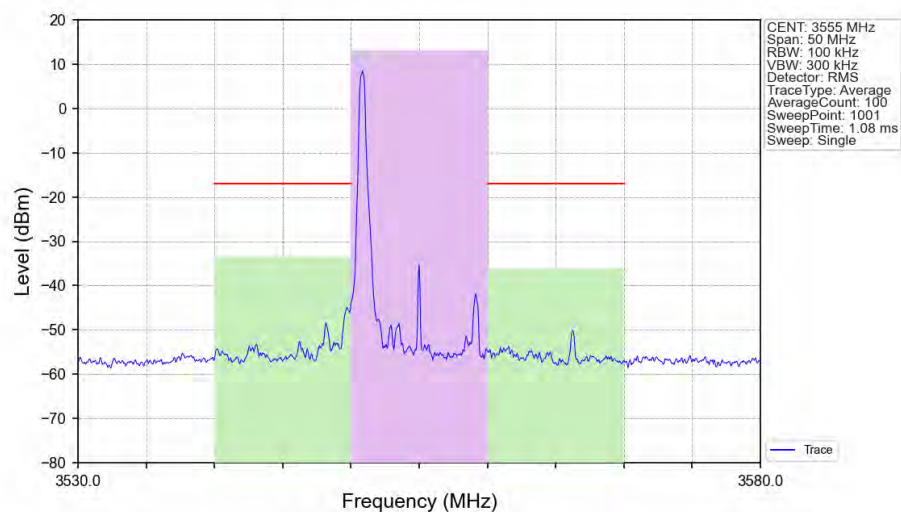
n48_30kHz_SISO_NTNV_10MHz_DFT-s-OFDM_16_QAM_3555MHz_Edge_1RB_Left_Ant1
