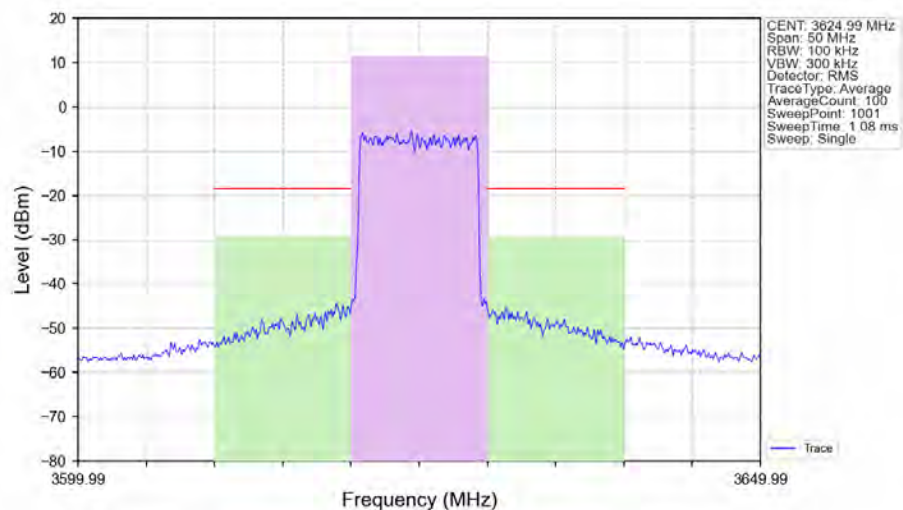
n48_30kHz_SISO_NTNV_10MHz_CP-OFDM_64_QAM_3624.99MHz_Outer_Full_Ant1
