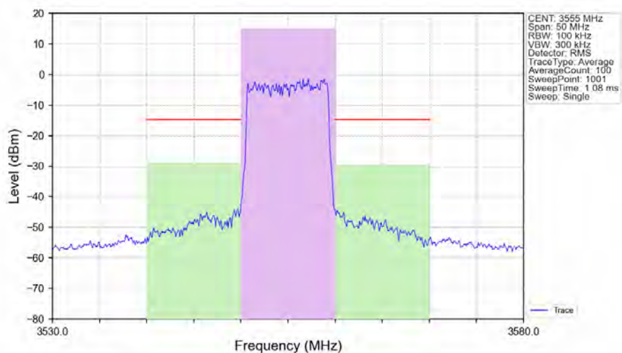
n48_30kHz_SISO_NTNV_10MHz_DFT-s-OFDM PI/2 BPSK_3555MHz_Outer_Full_Ant1
