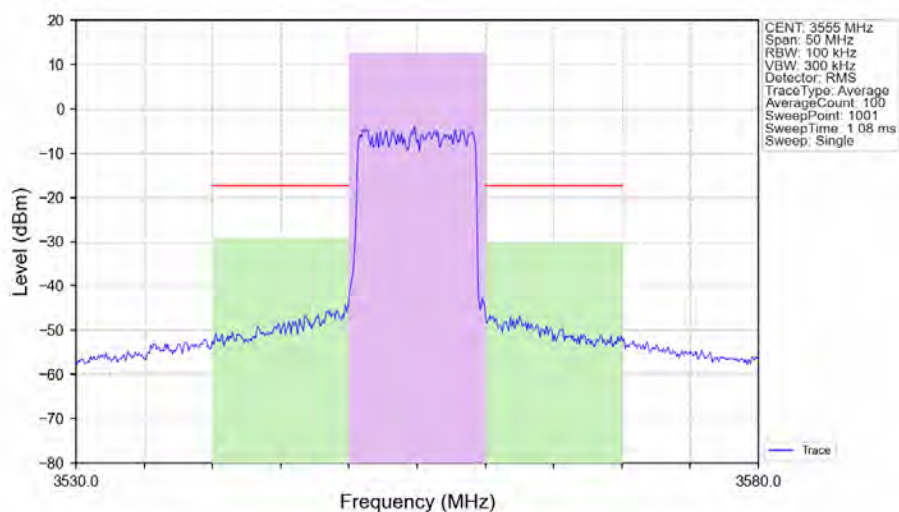
n48_30kHz_SISO_NTNV_10MHz_DFT-s-OFDM 64 QAM_3555MHz_Outer_Full_Ant1
