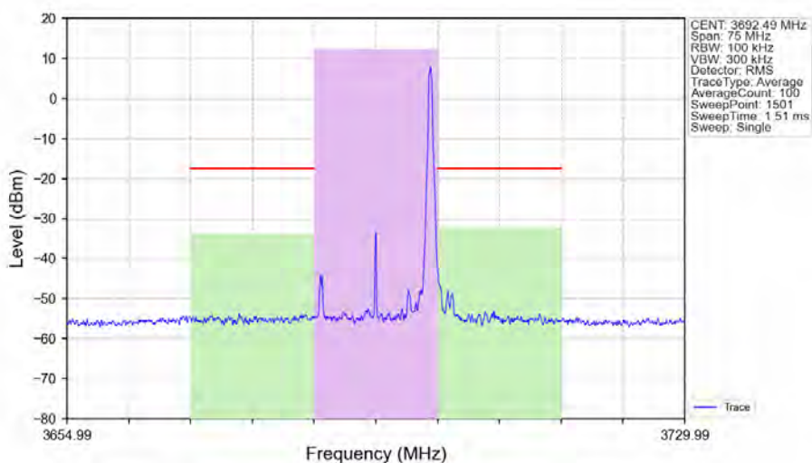
n48_30kHz_SISO_NTNV_15MHz_CP-OFDM_QPSK_3692.49MHz_Edge_1RB_Right_Ant1
