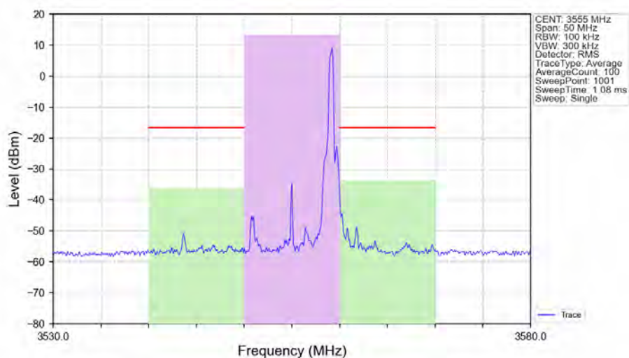
n48_30kHz_SISO_NTNV_10MHz_DFT-s-OFDM_64_QAM_3555MHz_Edge_1RB_Right_Ant1
