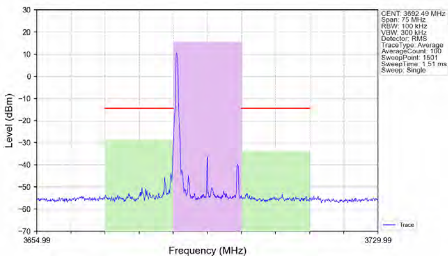
n48_30kHz_SISO_NTNV_15MHz_DFT-s-OFDM_PI/2_BPSK_3692.49MHz_Edge_1RB_Left_Ant1
