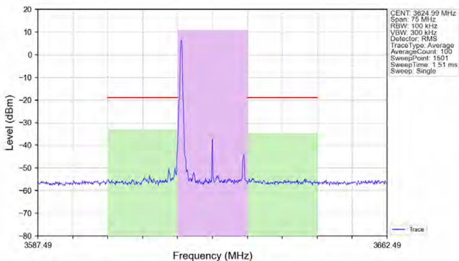
n48_30kHz_SISO_NTNV_15MHz_DFT-s-OFDM_256_QAM_3624.99MHz_Edge_1RB_Left_Ant1
