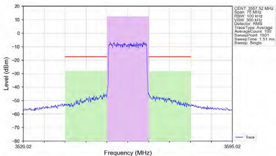
n48_30kHz_SISO_NTNV_15MHz_CP-OFDM QPSK 3557.52MHz_Outer_Full_Ant1
