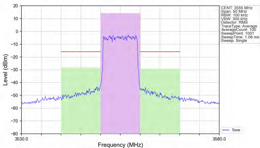
n48_30kHz_SISO_NTNV_10MHz_DFT-s-OFDM QPSK 3555MHz_Outer_Full_Ant1
