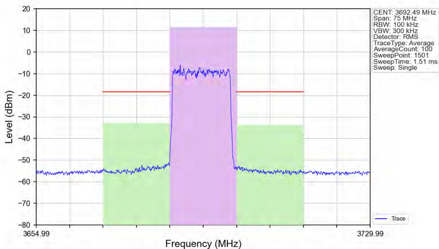
n48_30kHz_SISO_NTNV_15MHz_DFT-s-OFDM_256_QAM_3692.49MHz_Outer_Full_Ant1
