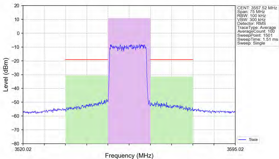
n48_30kHz_SISO_NTNV_15MHz_DFT-s-OFDM_256_QAM_3557.52MHz_Outer_Full_Ant1
