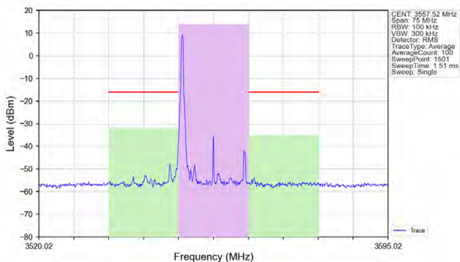
n48_30kHz_SISO_NTNV_15MHz_DFT-s-OFDM_16_QAM_3557.52MHz_Edge_1RB_Left_Ant1
