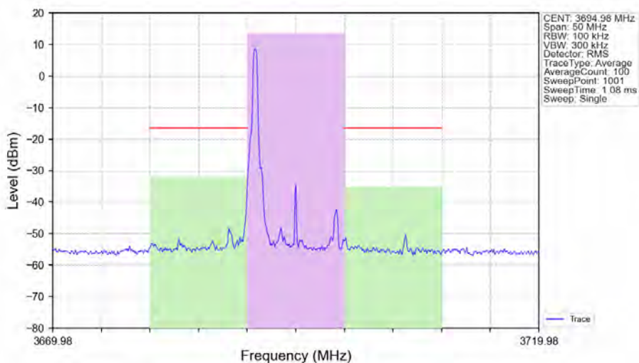
n48_30kHz_SISO_NTNV_10MHz_DFT-s-OFDM_64_QAM_3694.98MHz_Edge_1RB_Left_Ant1
