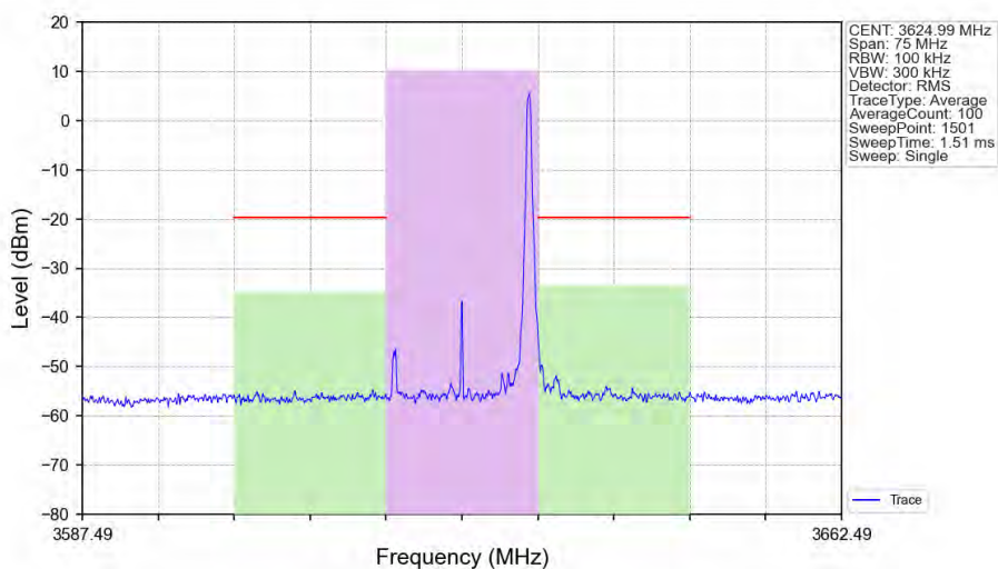
n48_30kHz_SISO_NTNV_15MHz_DFT-s-OFDM_256_QAM_3624.99MHz_Edge_1RB_Right_Ant1
