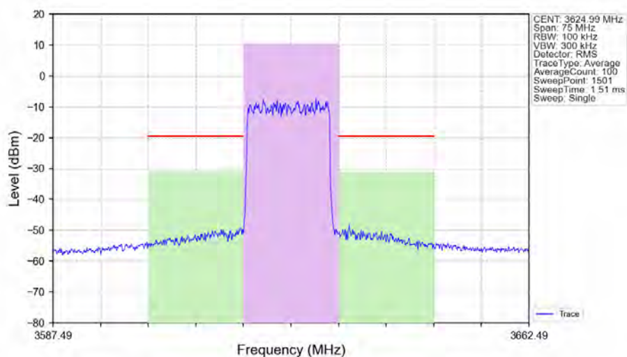
n48_30kHz_SISO_NTNV_15MHz_DFT-s-OFDM_256_QAM_3624.99MHz_Outer_Full_Ant1
