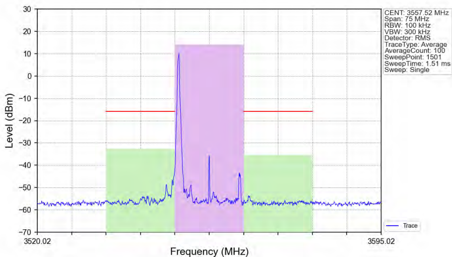
n48_30kHz_SISO_NTNV_15MHz_DFT-s-OFDM_64_QAM_3557.52MHz_Edge_1RB_Left_Ant1
