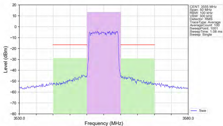
n48_30kHz_SISO_NTNV_10MHz_DFT-s-OFDM_16_QAM_3555MHz_Outer_Full_Ant1
