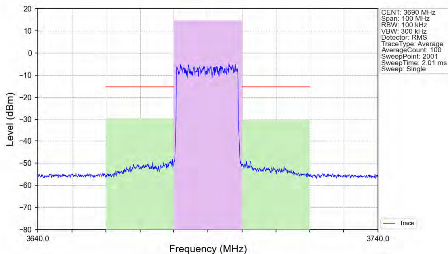
n48_30kHz_SISO_NTNV_20MHz_DFT-s-OFDM_PI/2_BPSK_3690MHz_Outer_Full_Ant1
