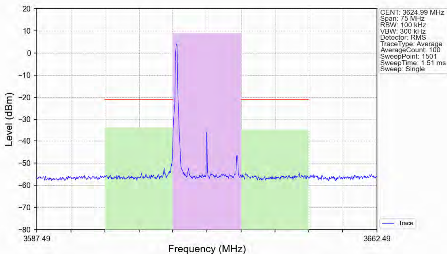
n48_30kHz_SISO_NTNV_15MHz_CP-OFDM 256 QAM 3624.99MHz_Edge_1RB_Left_Ant1
