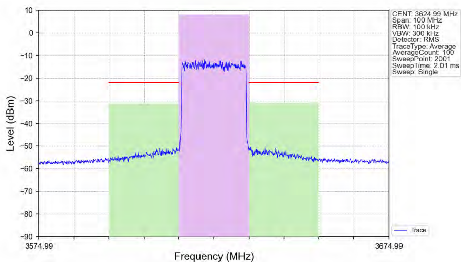
n48_30kHz_SISO_NTNV_20MHz_CP-OFDM 256 QAM 3624.99MHz_Outer_Full_Ant1
