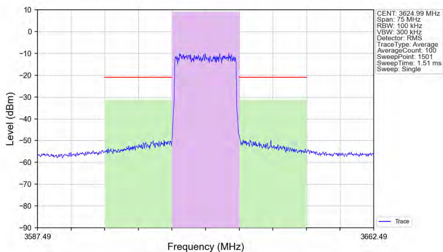
n48_30kHz_SISO_NTNV_15MHz_CP-OFDM 256 QAM 3624.99MHz_Outer_Full_Ant1
