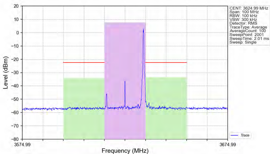
n48_30kHz_SISO_NTNV_20MHz_CP-OFDM 256 QAM 3624.99MHz_Edge_1RB_Right_Ant1
