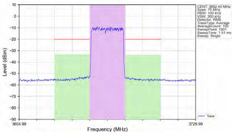
n48_30kHz_SISO_NTNV_15MHz_CP-OFDM 256 QAM 3692.49MHz_Outer_Full_Ant1
