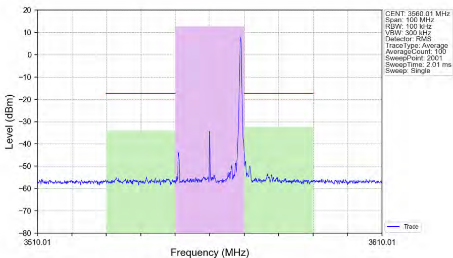
n48_30kHz_SISO_NTNV_20MHz_CP-OFDM_QPSK_3560.01MHz_Edge_1RB_Right_Ant1
