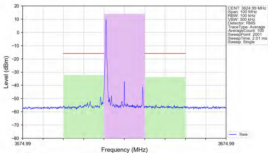
n48_30kHz_SISO_NTNV_20MHz_DFT-s-OFDM_QPSK_3624.99MHz_Edge_1RB_Left_Ant1
