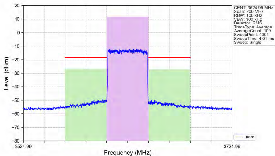
n48_30kHz_SISO_NTNV_40MHz_CP-OFDM_QPSK_3624.99MHz_Outer_Full_Ant1
