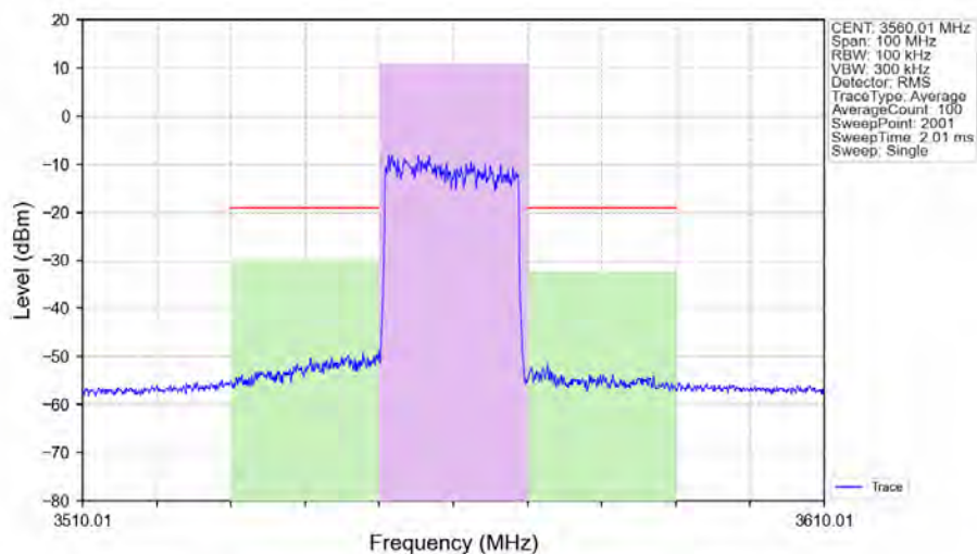
n48_30kHz_SISO_NTNV_20MHz_DFT-s-OFDM 256 QAM 3560.01MHz_Outer_Full_Ant1
