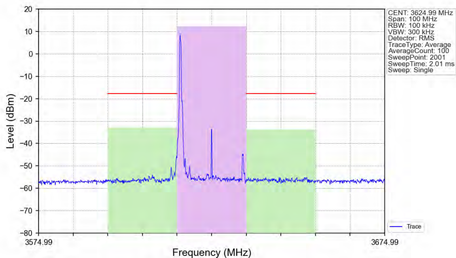
n48_30kHz_SISO_NTNV_20MHz_CP-OFDM_16_QAM_3624.99MHz_Edge_1RB_Left_Ant1
