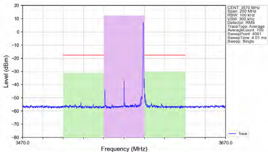
n48_30kHz_SISO_NTNV_40MHz_CP-OFDM_16_QAM_3570MHz_Edge_1RB_Right_Ant1
