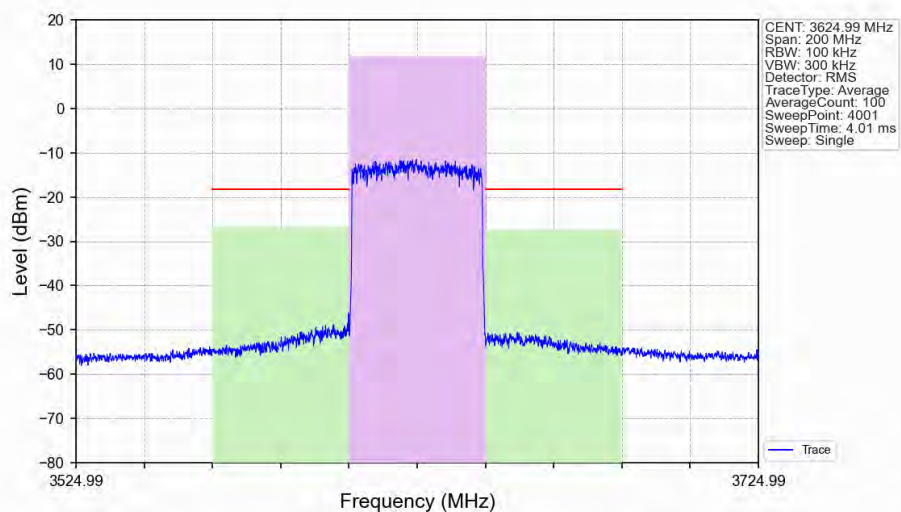
n48_30kHz_SISO_NTNV_40MHz_CP-OFDM_16_QAM_3624.99MHz_Outer_Full_Ant1
