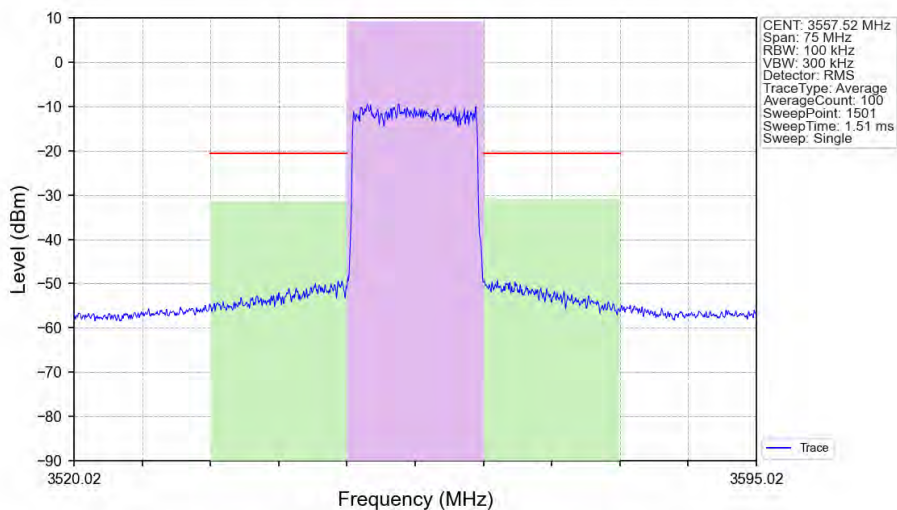
n48_30kHz_SISO_NTNV_15MHz_CP-OFDM 256 QAM 3557.52MHz_Outer_Full_Ant1
