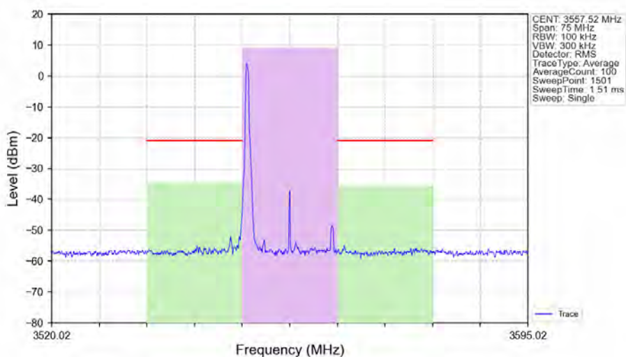
n48_30kHz_SISO_NTNV_15MHz_CP-OFDM 256 QAM 3557.52MHz_Edge_1RB_Left_Ant1
