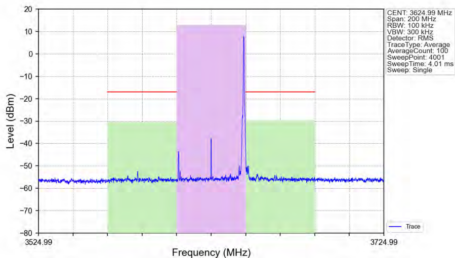
n48_30kHz_SISO_NTNV_40MHz_CP-OFDM_QPSK_3624.99MHz_Edge_1RB_Right_Ant1
