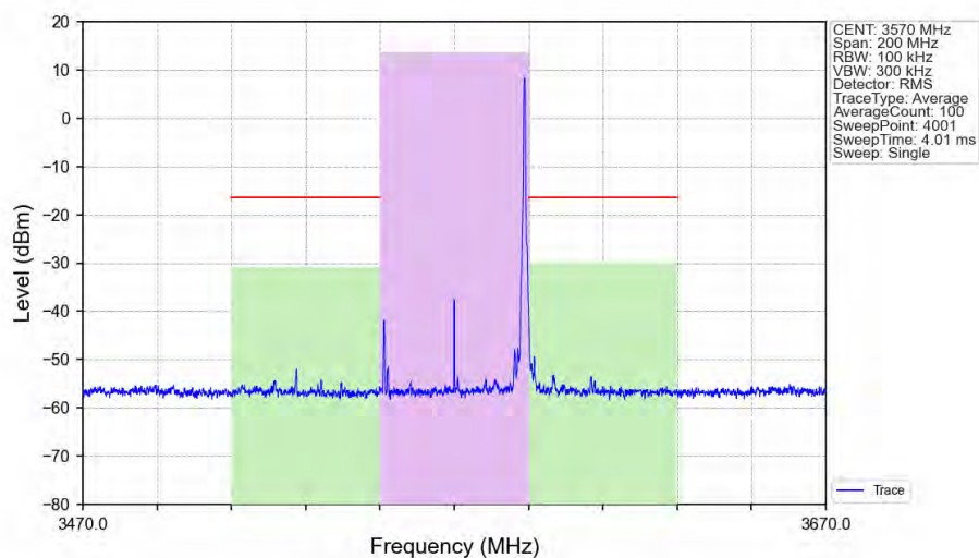
n48_30kHz_SISO_NTNV_40MHz_DFT-s-OFDM_16_QAM_3570MHz_Edge_1RB_Right_Ant1
