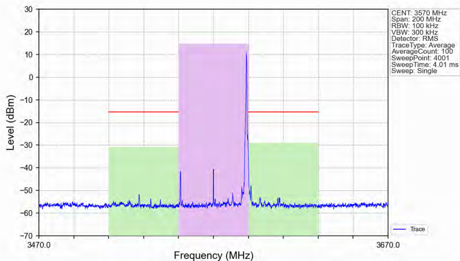
n48_30kHz_SISO_NTNV_40MHz_DFT-s-OFDM_PI/2_BPSK_3570MHz_Edge_1RB_Right_Ant1
