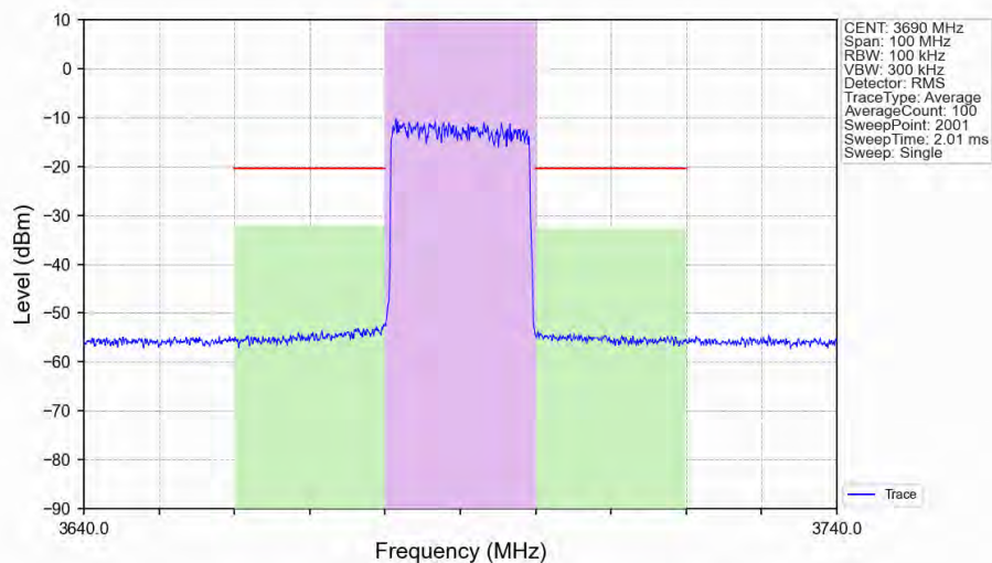
n48_30kHz_SISO_NTNV_20MHz_CP-OFDM 256 QAM 3690MHz_Outer_Full_Ant1
