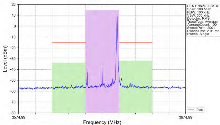
n48_30kHz_SISO_NTNV_20MHz_DFT-s-OFDM QPSK_3624.99MHz_Edge_1RB_Right_Ant1
