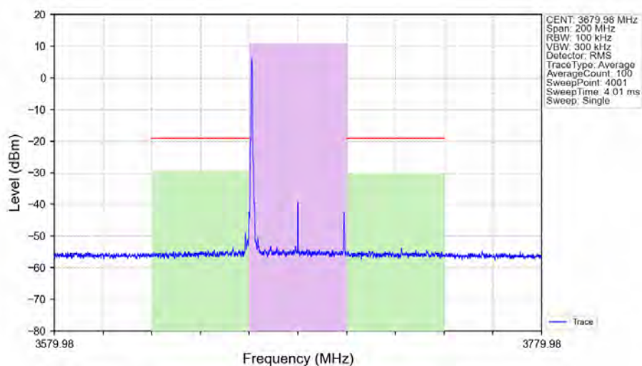
n48_30kHz_SISO_NTNV_40MHz_DFT-s-OFDM_256_QAM_3679.98MHz_Edge_1RB_Left_Ant1
