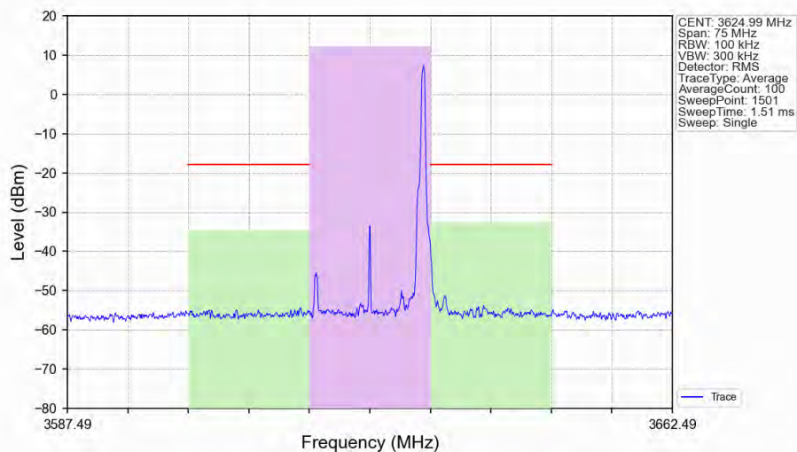
n48_30kHz_SISO_NTNV_15MHz_CP-OFDM 64 QAM_3624.99MHz_Edge_1RB_Right_Ant1
