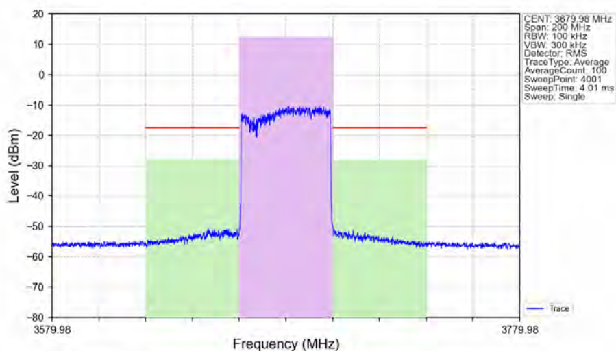
n48_30kHz_SISO_NTNV_40MHz_CP-OFDM_QPSK_3679.98MHz_Outer_Full_Ant1
