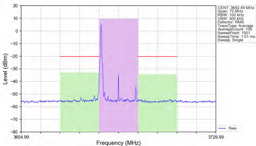
n48_30kHz_SISO_NTNV_15MHz_CP-OFDM 256 QAM 3692.49MHz_Edge_1RB_Left_Ant1
