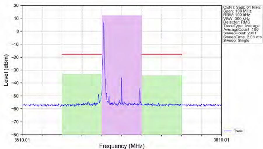
n48_30kHz_SISO_NTNV_20MHz_CP-OFDM_64_QAM_3560.01MHz_Edge_1RB_Left_Ant1
