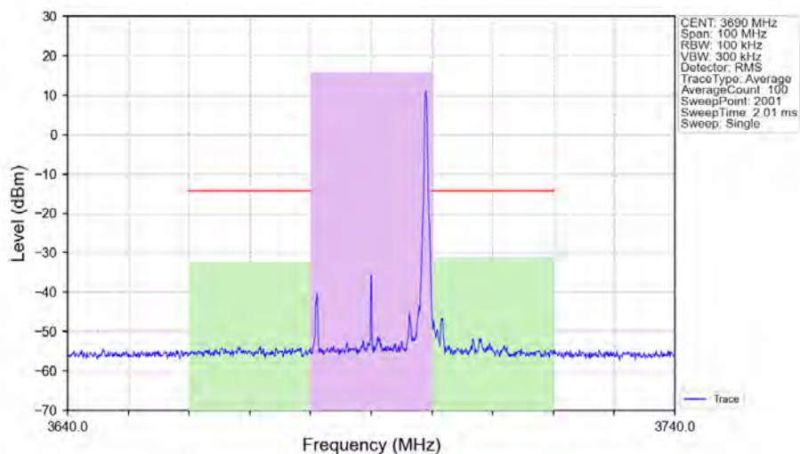
n48_30kHz_SISO_NTNV_20MHz_DFT-s-OFDM PI/2 BPSK 3690MHz_Edge_1RB_Right_Ant1
