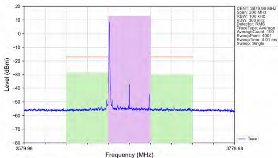
n48_30kHz_SISO_NTNV_40MHz_CP-OFDM_16_QAM_3679.98MHz_Edge_1RB_Left_Ant1
