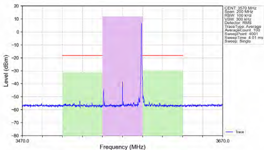
n48_30kHz_SISO_NTNV_40MHz_CP-OFDM_64_QAM_3570MHz_Edge_1RB_Right_Ant1
