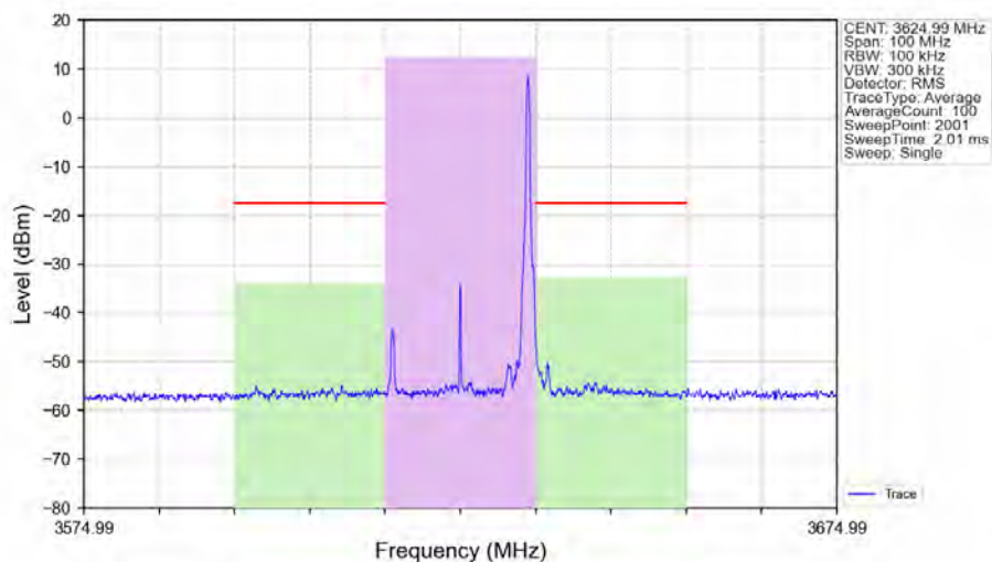
n48_30kHz_SISO_NTNV_20MHz_CP-OFDM QPSK_3624.99MHz_Edge_1RB_Right_Ant1
