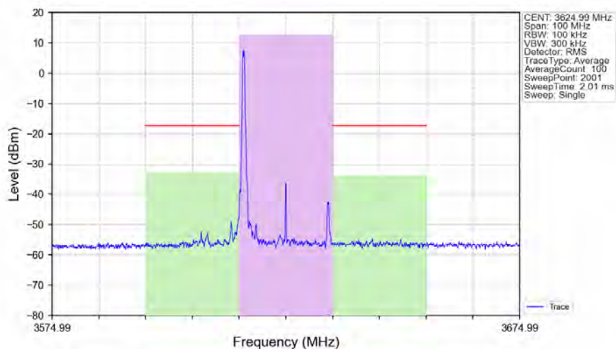
n48_30kHz_SISO_NTNV_20MHz_DFT-s-OFDM_16_QAM_3624.99MHz_Edge_1RB_Left_Ant1
