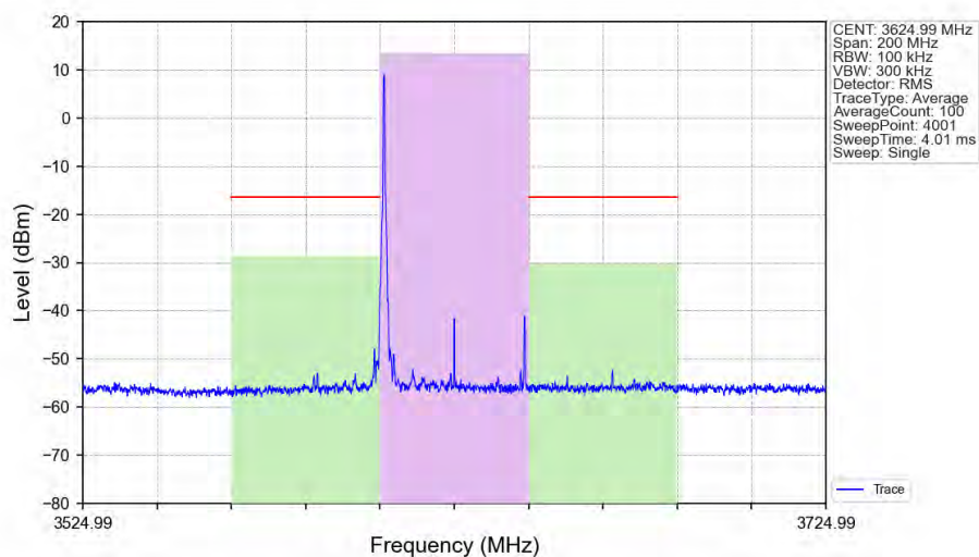
n48_30kHz_SISO_NTNV_40MHz_DFT-s-OFDM_QPSK_3624.99MHz_Edge_1RB_Left_Ant1
