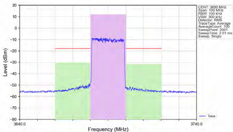
n48_30kHz_SISO_NTNV_20MHz_CP-OFDM 64 QAM_3690MHz_Outer_Full_Ant1
