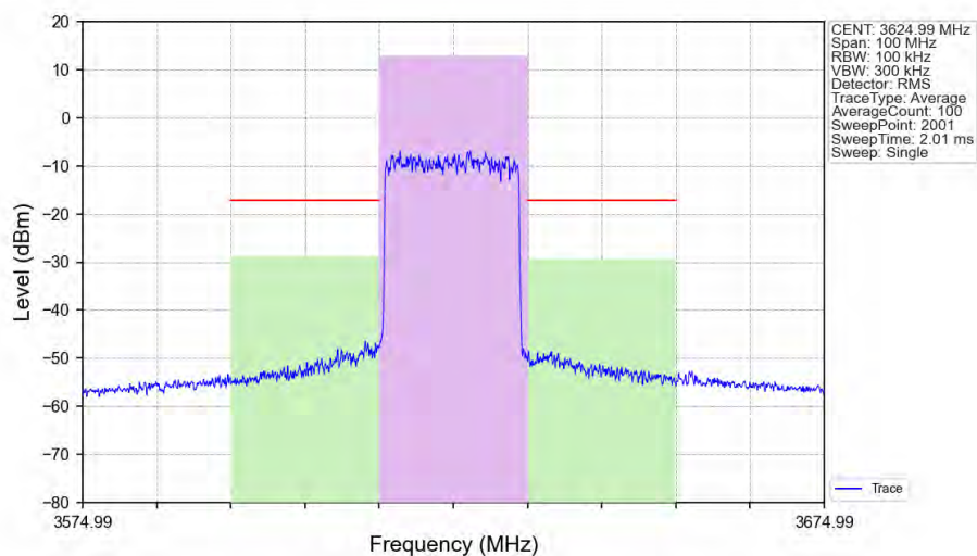
n48_30kHz_SISO_NTNV_20MHz_DFT-s-OFDM 16 QAM_3624.99MHz_Outer_Full_Ant1
