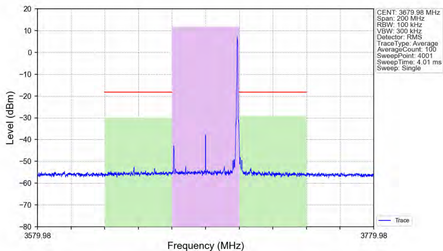
n48_30kHz_SISO_NTNV_40MHz_CP-OFDM 16 QAM_3679.98MHz_Edge_1RB_Right_Ant1
