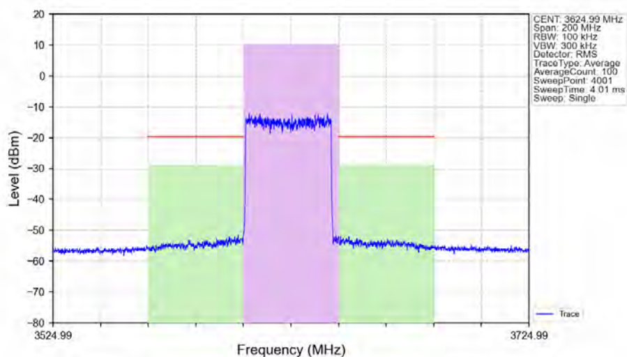
n48_30kHz_SISO_NTNV_40MHz_DFT-s-OFDM_256_QAM_3624.99MHz_Outer_Full_Ant1
