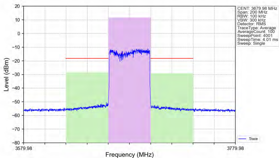
n48_30kHz_SISO_NTNV_40MHz_CP-OFDM 64 QAM_3679.98MHz_Outer_Full_Ant1
