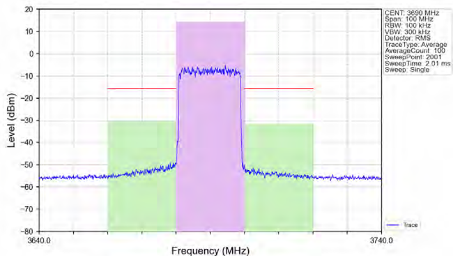
n48_30kHz_SISO_NTNV_20MHz_DFT-s-OFDM_16_QAM_3690MHz_Outer_Full_Ant1
