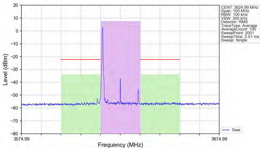
n48_30kHz_SISO_NTNV_20MHz_CP-OFDM 256 QAM 3624.99MHz_Edge_1RB_Left_Ant1
