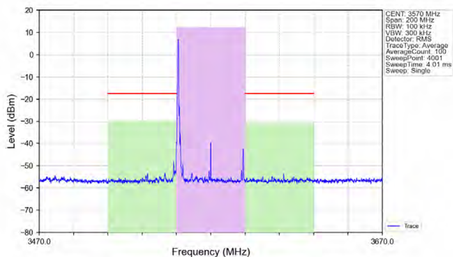
n48_30kHz_SISO_NTNV_40MHz_DFT-s-OFDM_16_QAM_3570MHz_Edge_1RB_Left_Ant1
