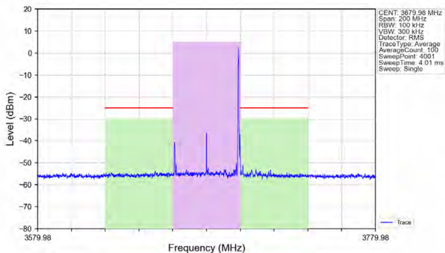
n48_30kHz_SISO_NTNV_40MHz_DFT-s-OFDM 16 QAM_3679.98MHz_Edge_1RB_Right_Ant1
