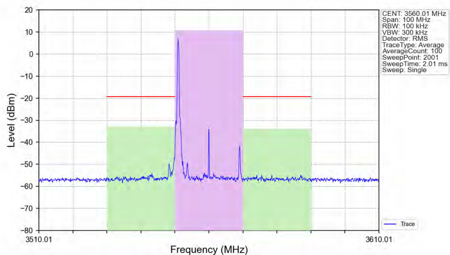
n48_30kHz_SISO_NTNV_20MHz_CP-OFDM_16_QAM_3560.01MHz_Edge_1RB_Left_Ant1
