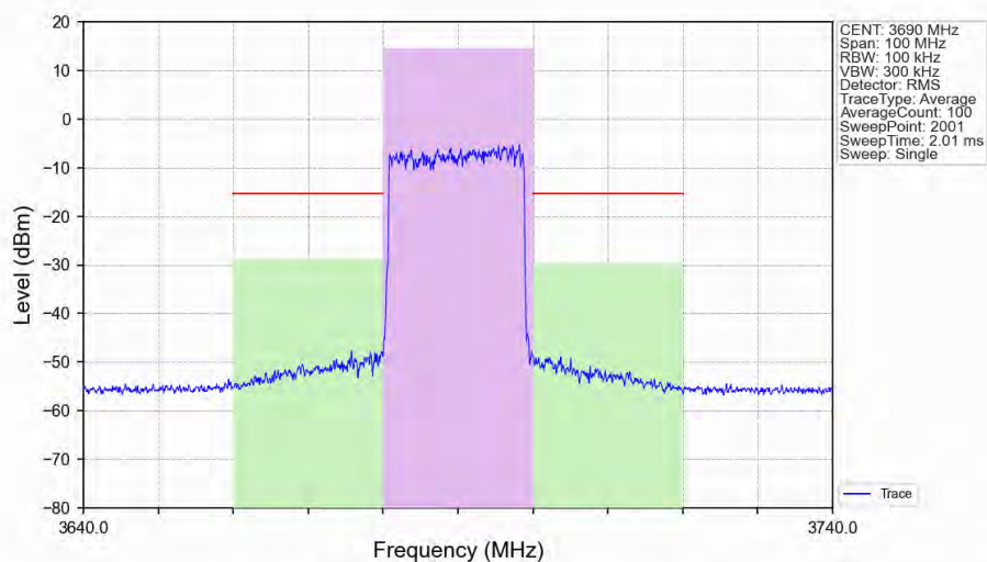
n48_30kHz_SISO_NTNV_20MHz_DFT-s-OFDM QPSK_3690MHz_Outer_Full_Ant1
