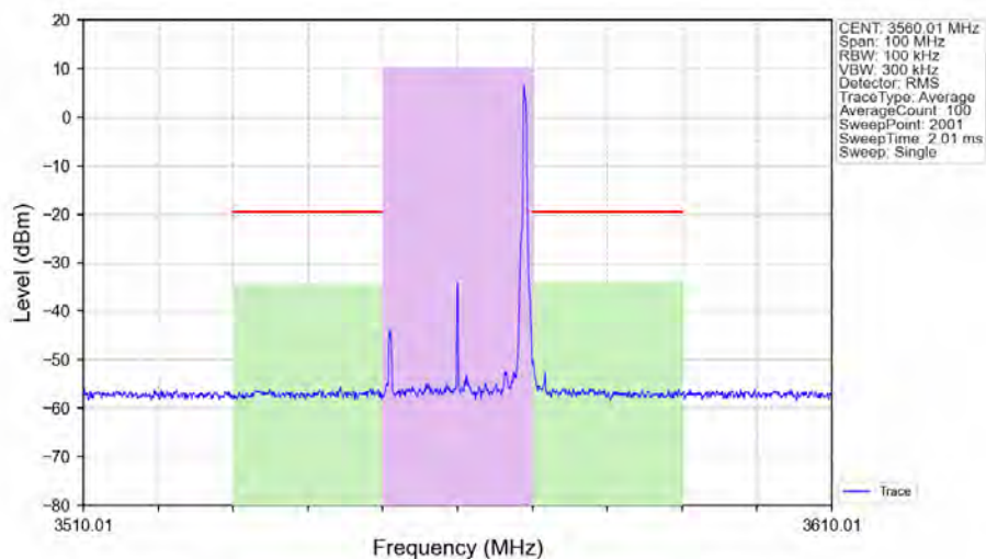
n48_30kHz_SISO_NTNV_20MHz_CP-OFDM 256 QAM 3560.01MHz_Edge_1RB_Right_Ant1
