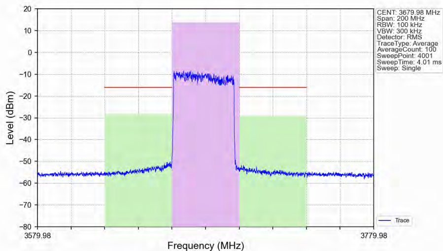
n48_30kHz_SISO_NTNV_40MHz_DFT-s-OFDM_16_QAM_3679.98MHz_Outer_Full_Ant1
