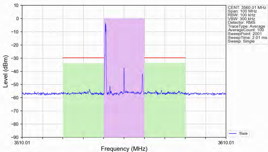
n48_30kHz_SISO_NTNV_20MHz_CP-OFDM_QPSK_3560.01MHz_Edge_1RB_Left_Ant1
