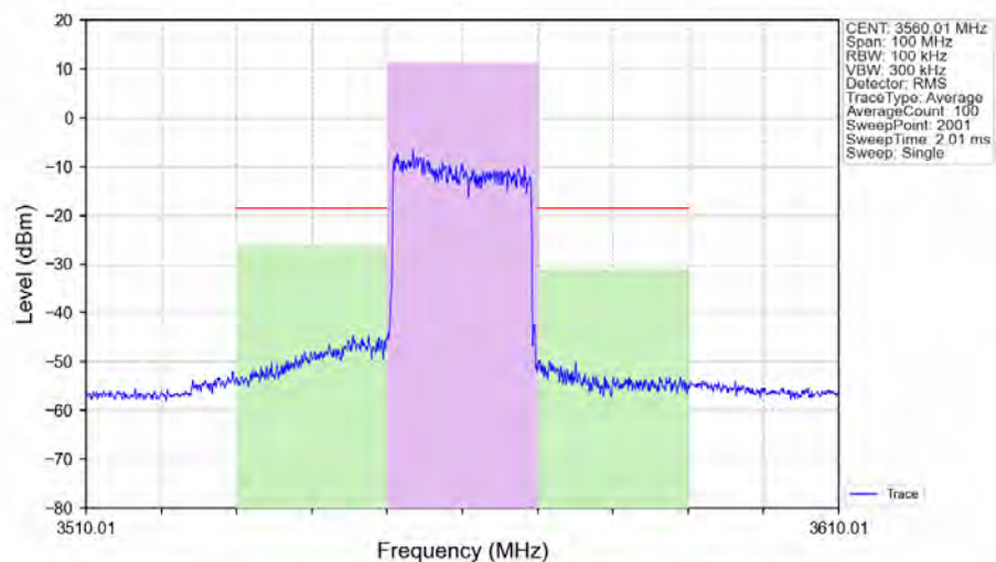
n48_30kHz_SISO_NTNV_20MHz_CP-OFDM_16_QAM_3560.01MHz_Outer_Full_Ant1
