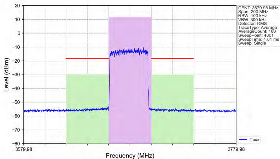
n48_30kHz_SISO_NTNV_40MHz_DFT-s-OFDM_256_QAM_3679.98MHz_Outer_Full_Ant1
