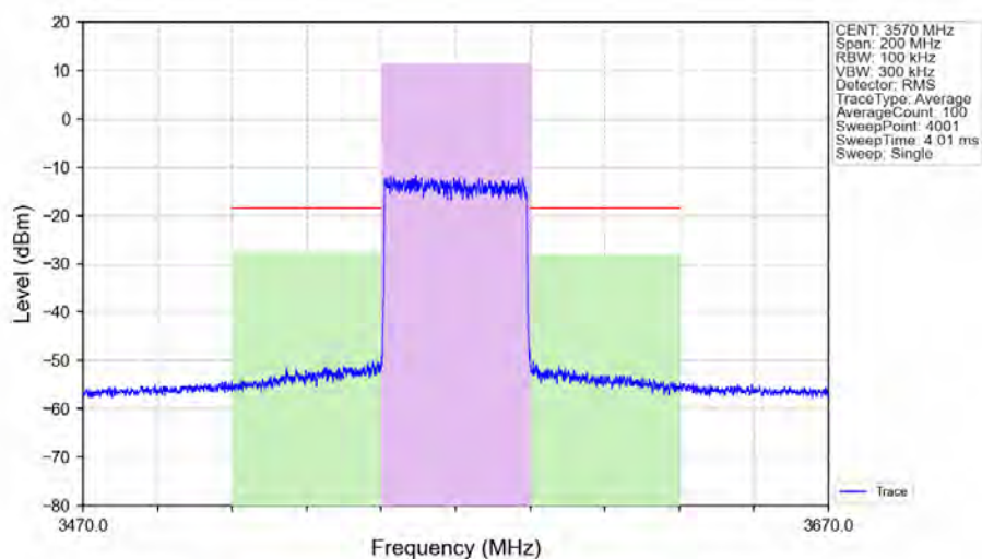
n48_30kHz_SISO_NTNV_40MHz_CP-OFDM 64 QAM_3570MHz_Outer_Full_Ant1
