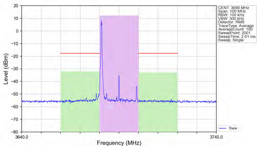
n48_30kHz_SISO_NTNV_20MHz_DFT-s-OFDM 256 QAM 3690MHz_Edge_1RB_Left_Ant1
