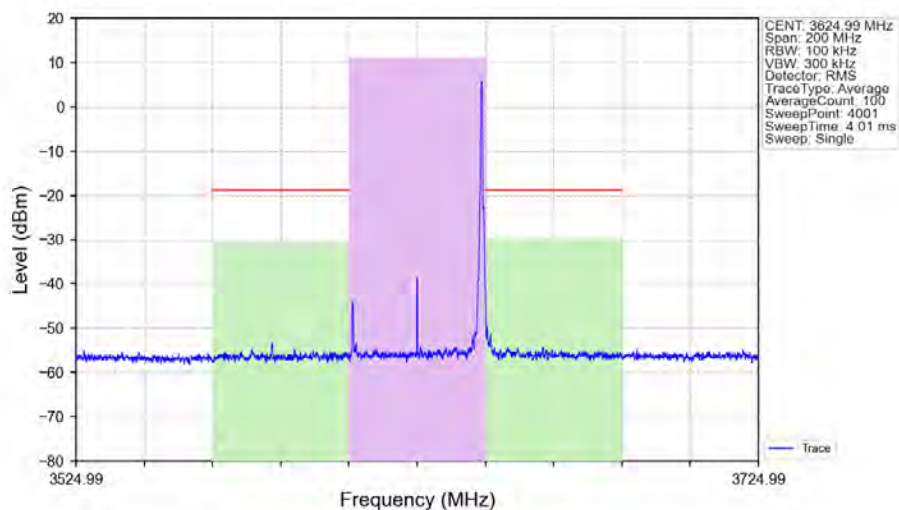
n48_30kHz_SISO_NTNV_40MHz_CP-OFDM 64 QAM_3624.99MHz_Edge_1RB_Right_Ant1
