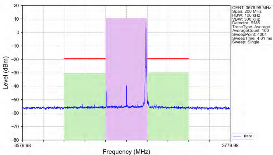
n48_30kHz_SISO_NTNV_40MHz_DFT-s-OFDM_256_QAM_3679.98MHz_Edge_1RB_Right_Ant1
