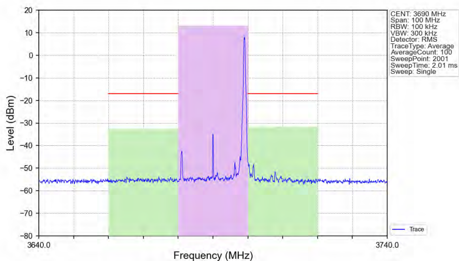
n48_30kHz_SISO_NTNV_20MHz_DFT-s-OFDM_64_QAM_3690MHz_Edge_1RB_Right_Ant1
