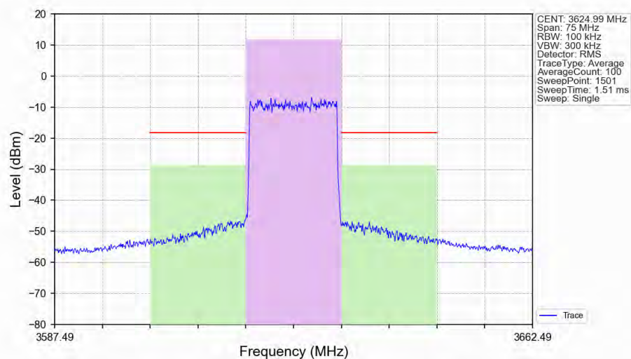
n48_30kHz_SISO_NTNV_15MHz_CP-OFDM_64_QAM_3624.99MHz_Outer_Full_Ant1
