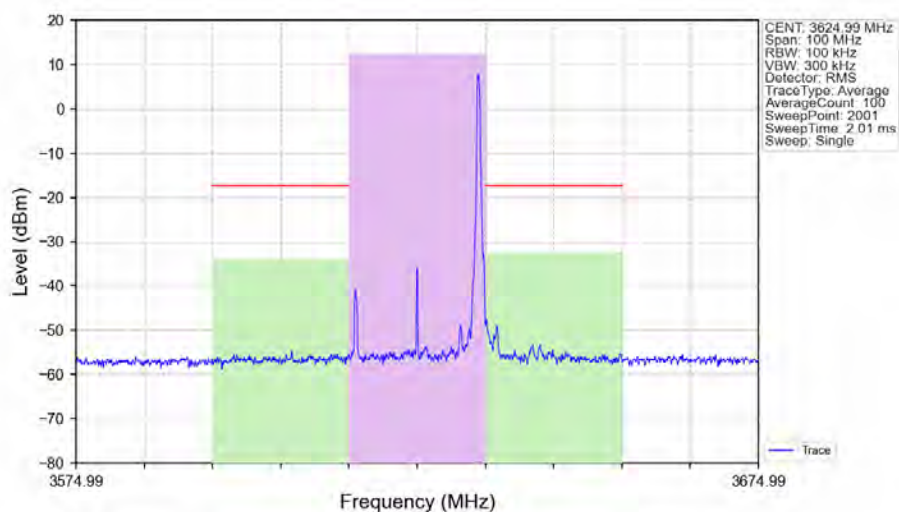
n48_30kHz_SISO_NTNV_20MHz_DFT-s-OFDM_16_QAM_3624.99MHz_Edge_1RB_Right_Ant1
