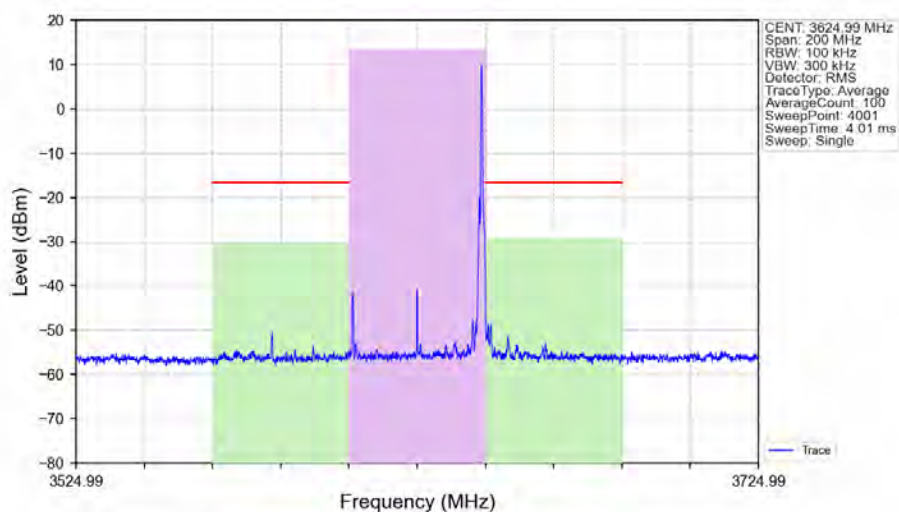
n48_30kHz_SISO_NTNV_40MHz_DFT-s-OFDM PI/2 BPSK_3624.99MHz_Edge_1RB_Right_Ant1
