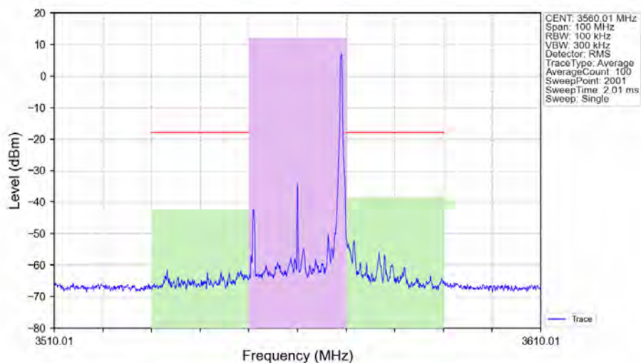
n48_30kHz_SISO_NTNV_20MHz_DFT-s-OFDM_256_QAM_3560.01MHz_Edge_1RB_Right_Ant1
