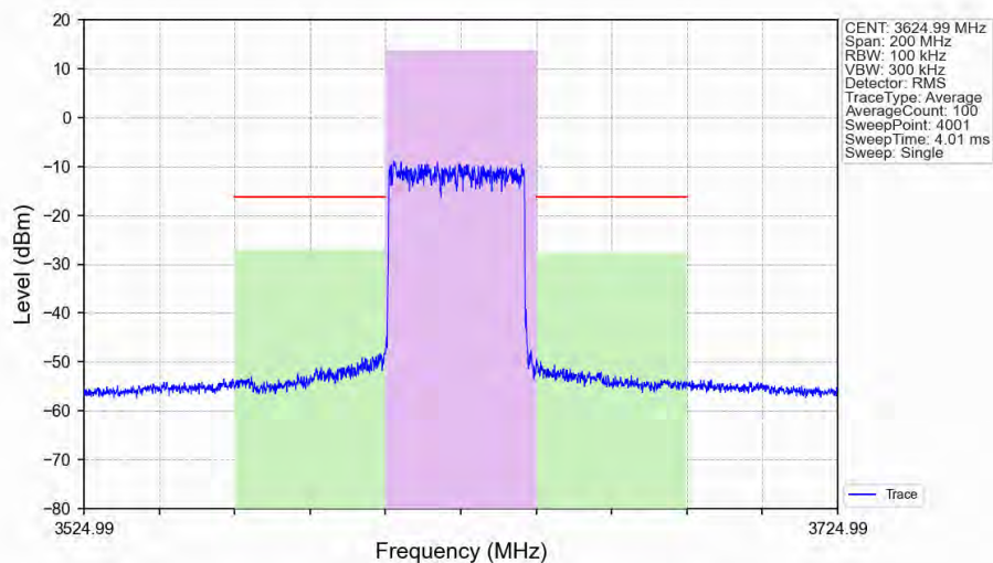
n48_30kHz_SISO_NTNV_40MHz_DFT-s-OFDM_QPSK_3624.99MHz_Outer_Full_Ant1
