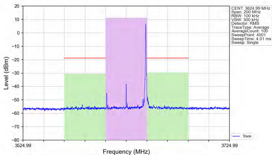
n48_30kHz_SISO_NTNV_40MHz_CP-OFDM_16_QAM_3624.99MHz_Edge_1RB_Right_Ant1
