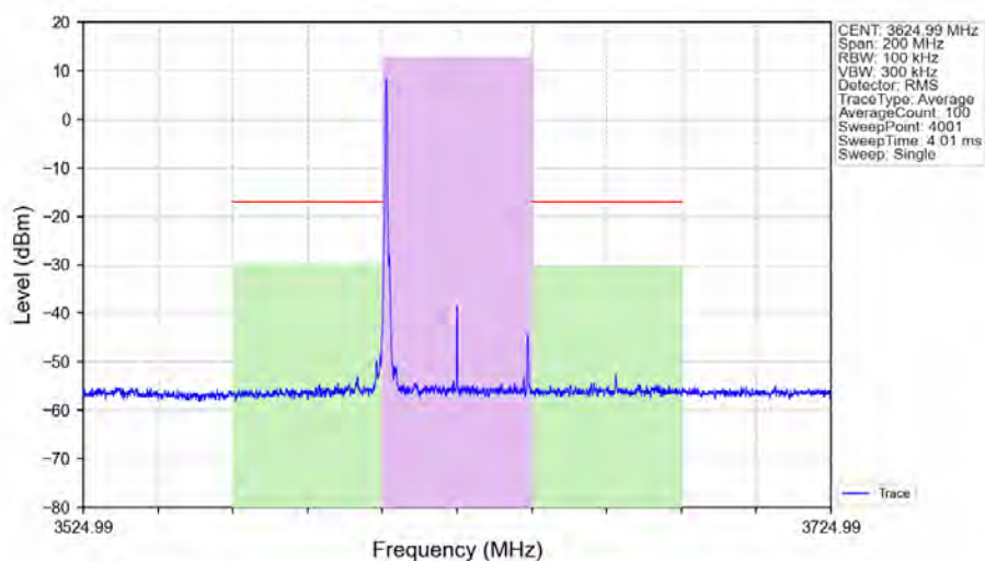
n48_30kHz_SISO_NTNV_40MHz_CP-OFDM_QPSK_3624.99MHz_Edge_1RB_Left_Ant1
