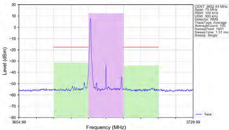
n48_30kHz_SISO_NTNV_15MHz_CP-OFDM_64_QAM_3692.49MHz_Edge_1RB_Left_Ant1
