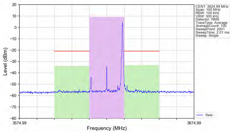
n48_30kHz_SISO_NTNV_20MHz_CP-OFDM 64 QAM_3624.99MHz_Edge_1RB_Right_Ant1
