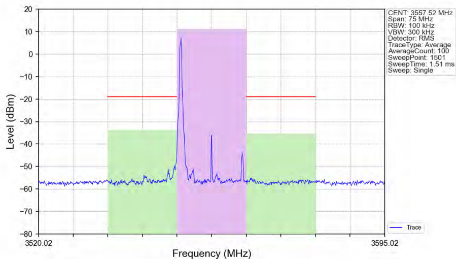
n48_30kHz_SISO_NTNV_15MHz_CP-OFDM_64_QAM_3557.52MHz_Edge_1RB_Left_Ant1
