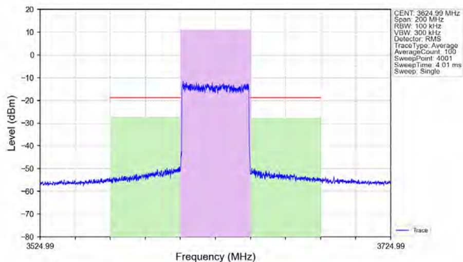
n48_30kHz_SISO_NTNV_40MHz_CP-OFDM_64_QAM_3624.99MHz_Outer_Full_Ant1
