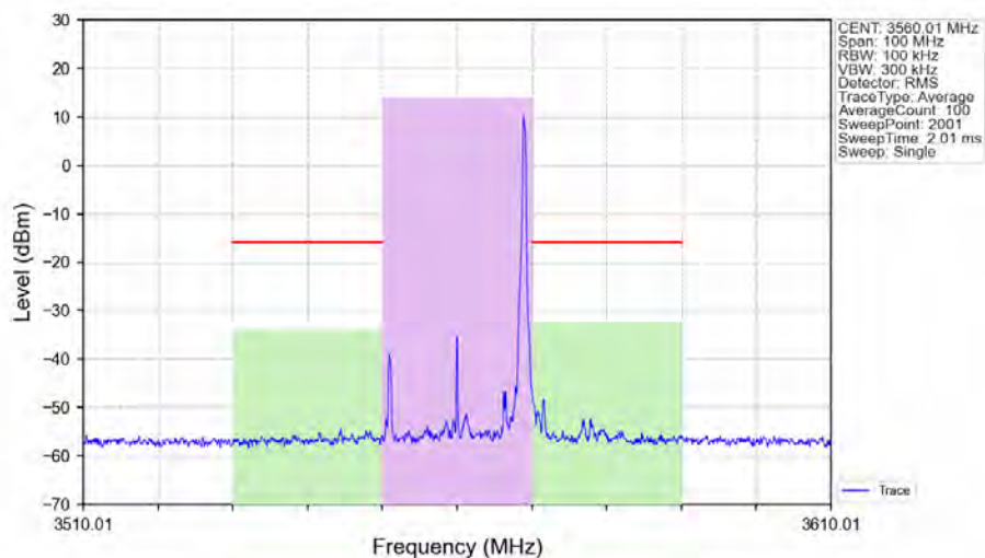
n48_30kHz_SISO_NTNV_20MHz_DFT-s-OFDM_PI/2_BPSK_3560.01MHz_Edge_1RB_Right_Ant1
