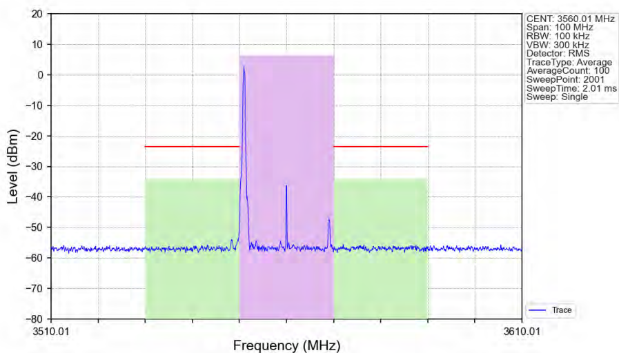
n48_30kHz_SISO_NTNV_20MHz_CP-OFDM 256 QAM 3560.01MHz_Edge_1RB_Left_Ant1
