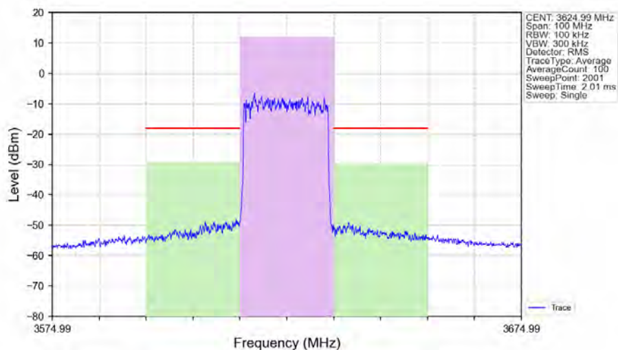
n48_30kHz_SISO_NTNV_20MHz_DFT-s-OFDM_64_QAM_3624.99MHz_Outer_Full_Ant1
