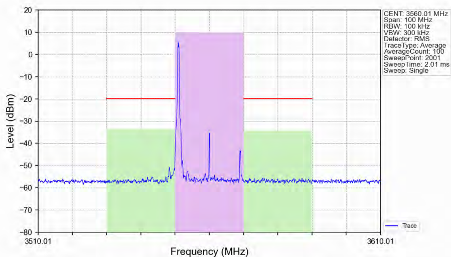
n48_30kHz_SISO_NTNV_20MHz_DFT-s-OFDM 256 QAM 3560.01MHz_Edge_1RB_Left_Ant1
