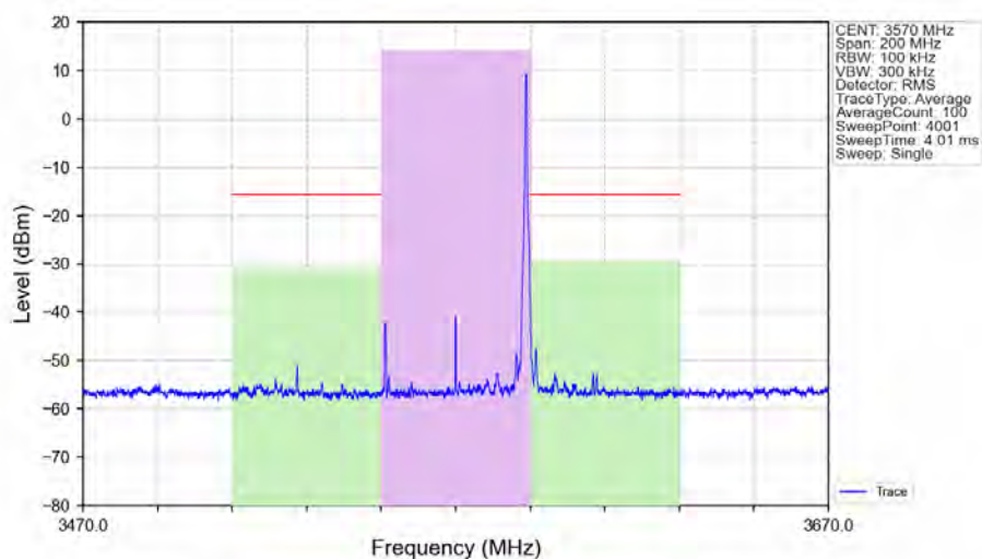
n48_30kHz_SISO_NTNV_40MHz_DFT-s-OFDM_QPSK_3570MHz_Edge_1RB_Right_Ant1
