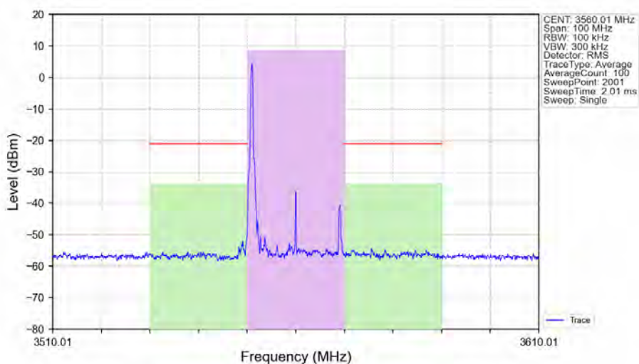
n48_30kHz_SISO_NTNV_20MHz_DFT-s-OFDM_16_QAM_3560.01MHz_Edge_1RB_Left_Ant1
