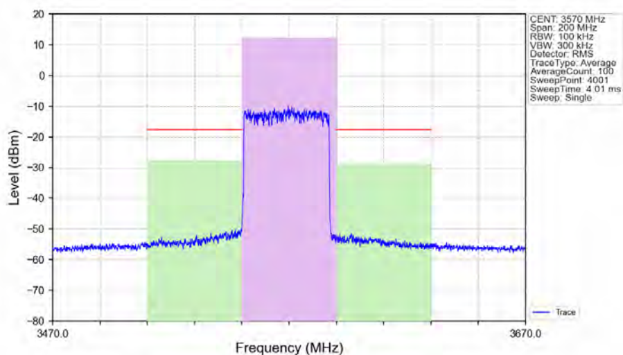
n48_30kHz_SISO_NTNV_40MHz_DFT-s-OFDM 64 QAM_3570MHz_Outer_Full_Ant1
