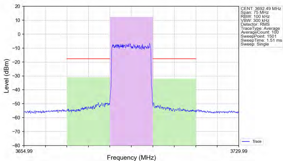
n48_30kHz_SISO_NTNV_15MHz_CP-OFDM 64 QAM_3692.49MHz_Outer_Full_Ant1
