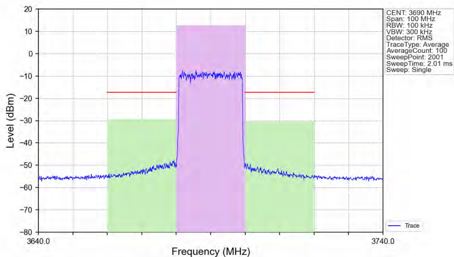
n48_30kHz_SISO_NTNV_20MHz_CP-OFDM_16_QAM_3690MHz_Outer_Full_Ant1
