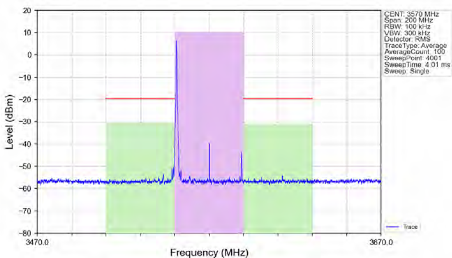
n48_30kHz_SISO_NTNV_40MHz_DFT-s-OFDM 256 QAM 3570MHz_Edge_1RB_Left_Ant1
