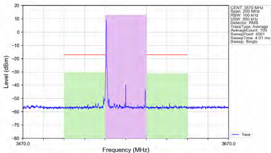
n48_30kHz_SISO_NTNV_40MHz_DFT-s-OFDM_64_QAM_3570MHz_Edge_1RB_Left_Ant1
