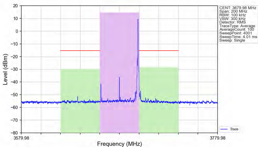
n48_30kHz_SISO_NTNV_40MHz_DFT-s-OFDM_QPSK_3679.98MHz_Edge_1RB_Right_Ant1
