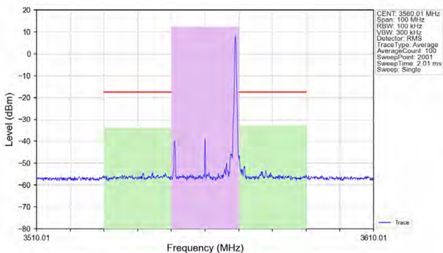
n48_30kHz_SISO_NTNV_20MHz_DFT-s-OFDM_QPSK_3560.01MHz_Edge_1RB_Right_Ant1
