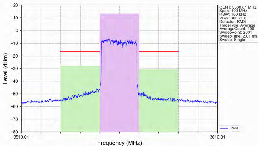
n48_30kHz_SISO_NTNV_20MHz_DFT-s-OFDM_16_QAM_3560.01MHz_Outer_Full_Ant1
