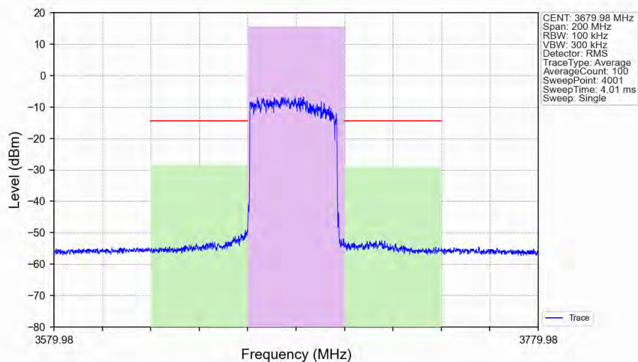
n48_30kHz_SISO_NTNV_40MHz_DFT-s-OFDM_PI/2_BPSK_3679.98MHz_Outer_Full_Ant1
