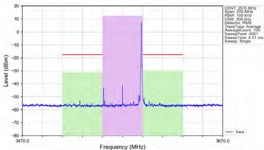
n48_30kHz_SISO_NTNV_40MHz_DFT-s-OFDM_64_QAM_3570MHz_Edge_1RB_Right_Ant1
