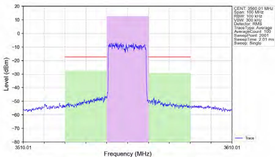
n48_30kHz_SISO_NTNV_20MHz_DFT-s-OFDM QPSK 3560.01MHz_Outer_Full_Ant1
