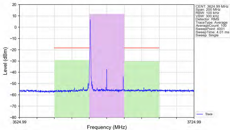
n48_30kHz_SISO_NTNV_40MHz_CP-OFDM_16_QAM_3624.99MHz_Edge_1RB_Left_Ant1
