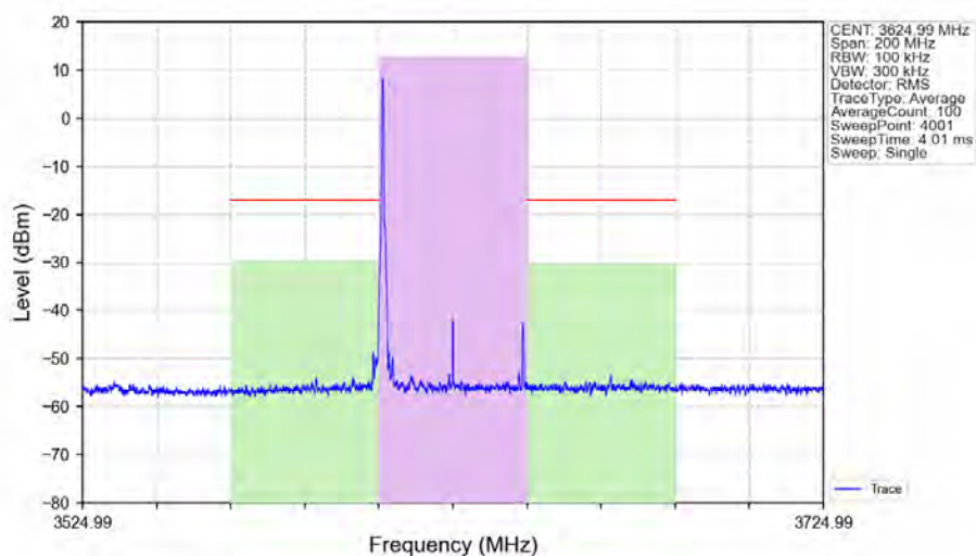
n48_30kHz_SISO_NTNV_40MHz_DFT-s-OFDM_64_QAM_3624.99MHz_Edge_1RB_Left_Ant1
