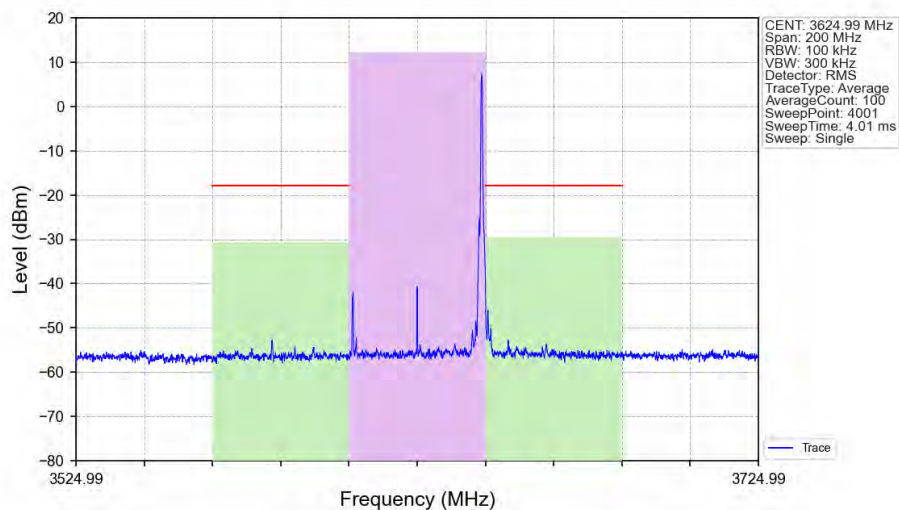
n48_30kHz_SISO_NTNV_40MHz_DFT-s-OFDM 64 QAM_3624.99MHz_Edge_Right_Ant1
