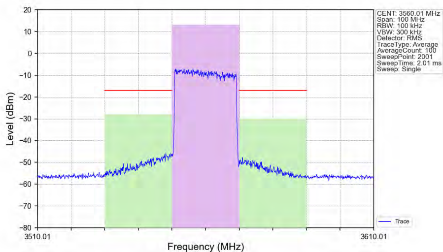
n48_30kHz_SISO_NTNV_20MHz_CP-OFDM 64 QAM_3560.01MHz_Outer_Full_Ant1
