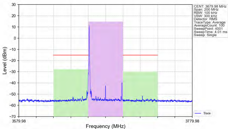
n48_30kHz_SISO_NTNV_40MHz_DFT-s-OFDM_QPSK_3679.98MHz_Edge_1RB_Left_Ant1
