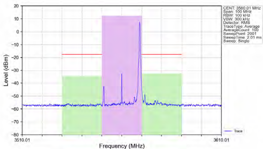
n48_30kHz_SISO_NTNV_20MHz_CP-OFDM_64_QAM_3560.01MHz_Edge_1RB_Right_Ant1
