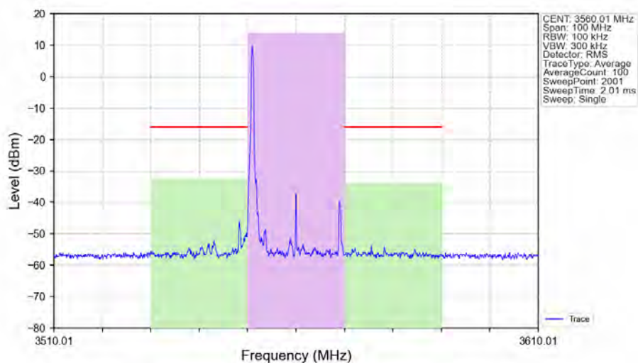
n48_30kHz_SISO_NTNV_20MHz_DFT-s-OFDM PI/2 BPSK_3560.01MHz_Edge_1RB_Left_Ant1
