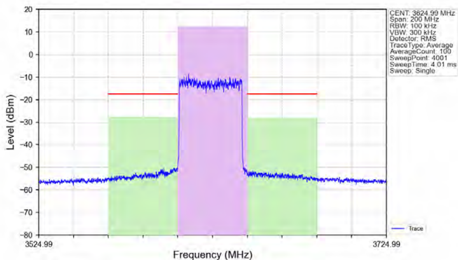
n48_30kHz_SISO_NTNV_40MHz_DFT-s-OFDM_64_QAM_3624.99MHz_Outer_Full_Ant1
