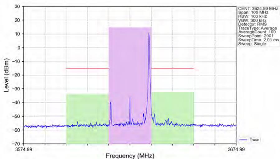
n48_30kHz_SISO_NTNV_20MHz_DFT-s-OFDM PI/2 BPSK_3624.99MHz_Edge_1RB_Right_Ant1
