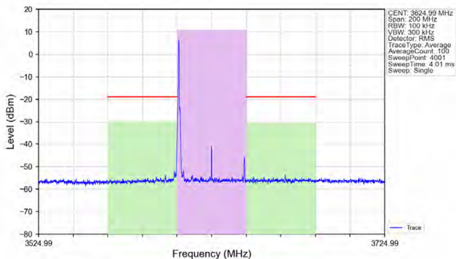
n48_30kHz_SISO_NTNV_40MHz_DFT-s-OFDM_256_QAM_3624.99MHz_Edge_1RB_Left_Ant1
