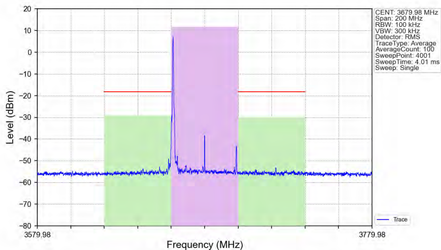
n48_30kHz_SISO_NTNV_40MHz_DFT-s-OFDM_64_QAM_3679.98MHz_Edge_1RB_Left_Ant1
