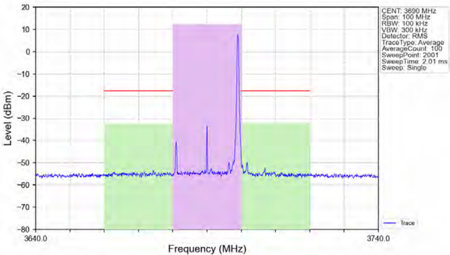
n48_30kHz_SISO_NTNV_20MHz_CP-OFDM_QPSK_3690MHz_Edge_1RB_Right_Ant1
