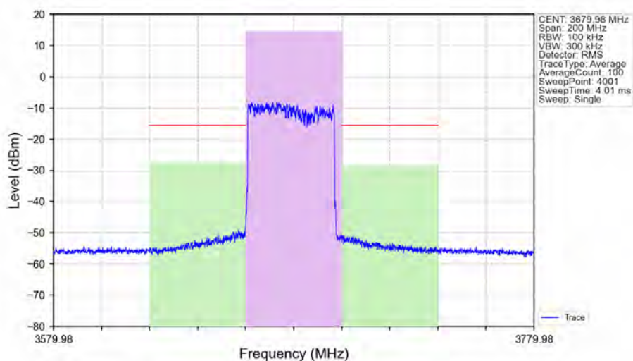
n48_30kHz_SISO_NTNV_40MHz_DFT-s-OFDM_QPSK_3679.98MHz_Outer_Full_Ant1
