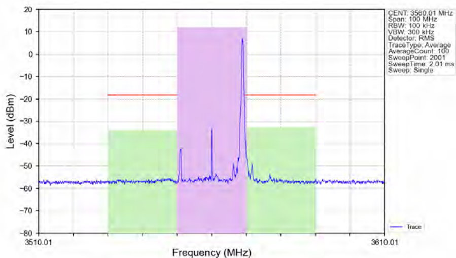
n48_30kHz_SISO_NTNV_20MHz_CP-OFDM_16 QAM_3560.01MHz_Edge_1RB_Right_Ant1
