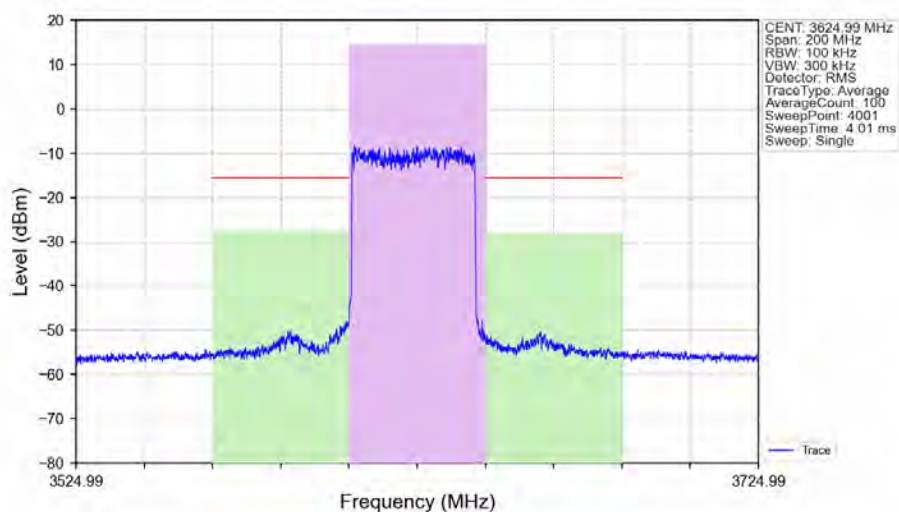
n48_30kHz_SISO_NTNV_40MHz_DFT-s-OFDM_PI/2_BPSK_3624.99MHz_Outer_Full_Ant1
