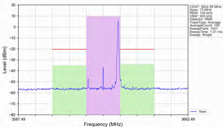
n48_30kHz_SISO_NTNV_15MHz_CP-OFDM 256 QAM 3624.99MHz_Edge_1RB_Right_Ant1
