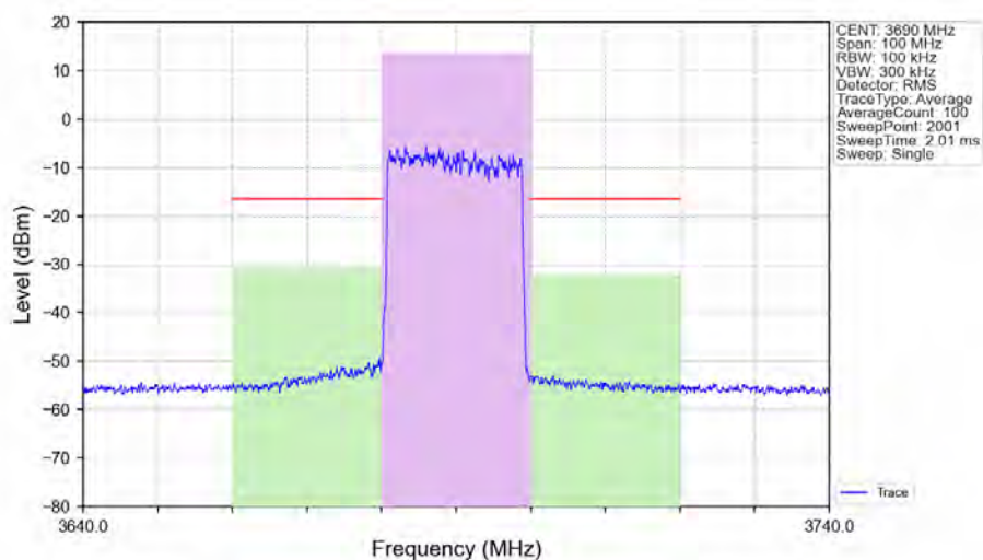
n48_30kHz_SISO_NTNV_20MHz_DFT-s-OFDM 64 QAM_3690MHz_Outer_Full_Ant1
