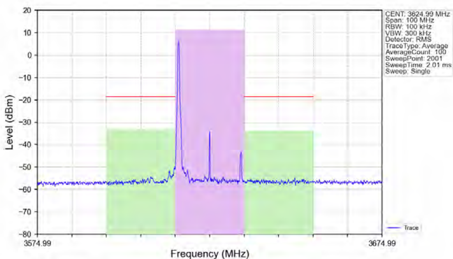
n48_30kHz_SISO_NTNV_20MHz_CP-OFDM_64_QAM_3624.99MHz_Edge_1RB_Left_Ant1
