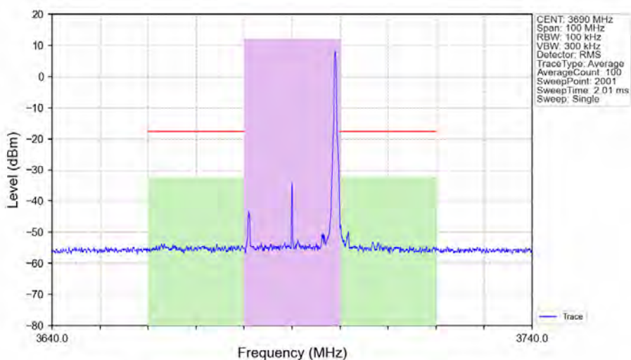
n48_30kHz_SISO_NTNV_20MHz_CP-OFDM 64 QAM 3690MHz_Edge_1RB_Right_Ant1
