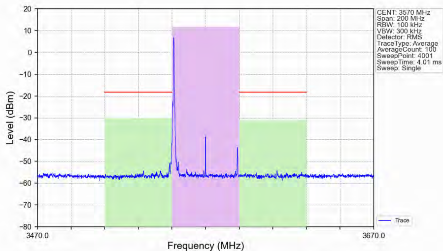
n48_30kHz_SISO_NTNV_40MHz_CP-OFDM_64_QAM_3570MHz_Edge_1RB_Left_Ant1
