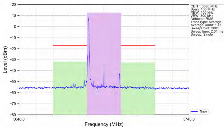
n48_30kHz_SISO_NTNV_20MHz_DFT-s-OFDM_64_QAM_3690MHz_Edge_1RB_Left_Ant1
