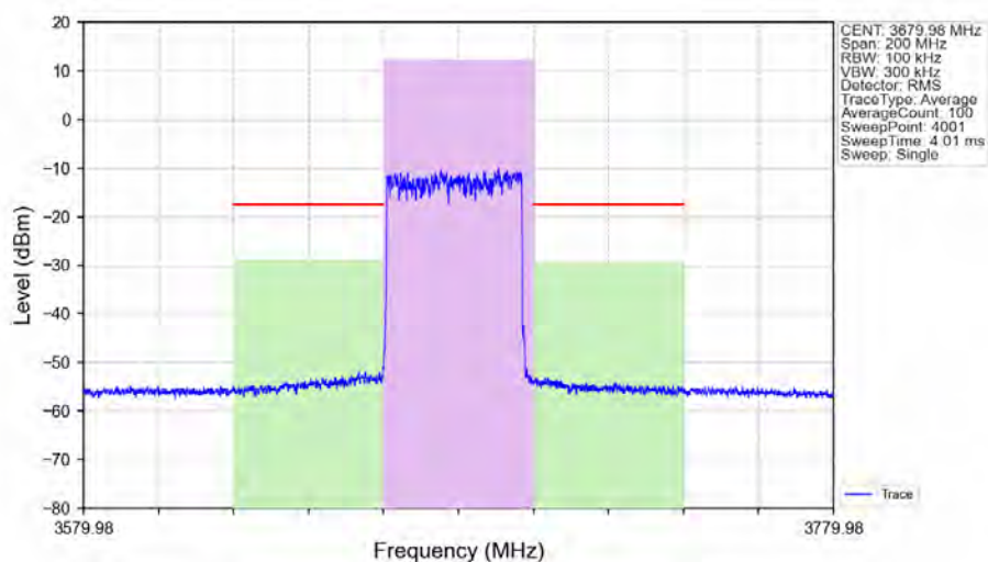
n48_30kHz_SISO_NTNV_40MHz_DFT-s-OFDM 64 QAM_3679.98MHz_Outer_Full_Ant1
