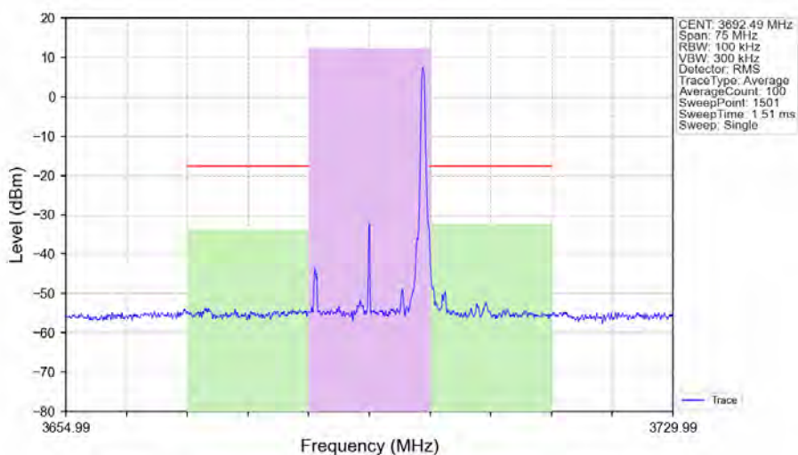
n48_30kHz_SISO_NTNV_15MHz_CP-OFDM_64_QAM_3692.49MHz_Edge_1RB_Right_Ant1
