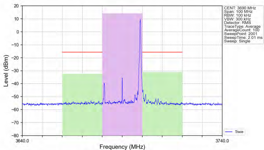
n48_30kHz_SISO_NTNV_20MHz_DFT-s-OFDM_QPSK_3690MHz_Edge_1RB_Right_Ant1
