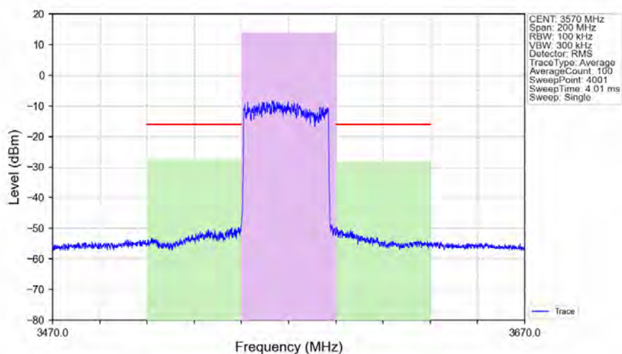
n48_30kHz_SISO_NTNV_40MHz_DFT-s-OFDM QPSK 3570MHz_Outer_Full_Ant1
