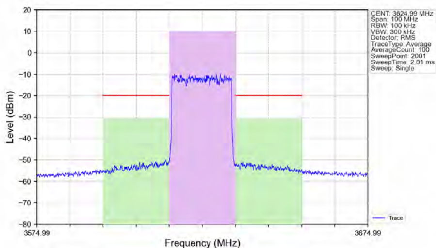
n48_30kHz_SISO_NTNV_20MHz_DFT-s-OFDM_256_QAM_3624.99MHz_Outer_Full_Ant1
