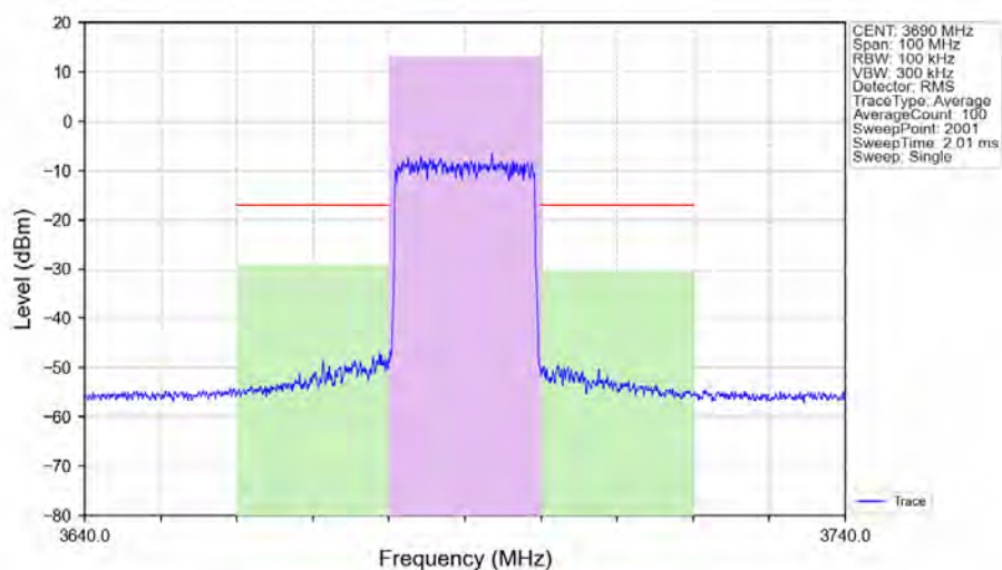
n48_30kHz_SISO_NTNV_20MHz_CP-OFDM QPSK_3690MHz_Outer_Full_Ant1
