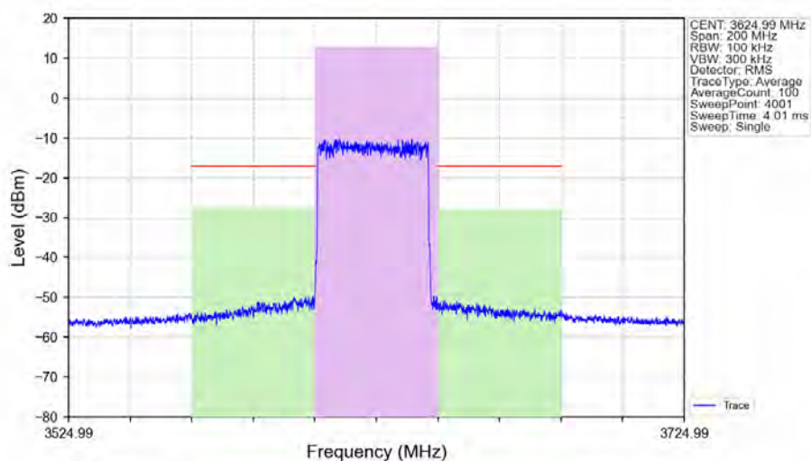
n48_30kHz_SISO_NTNV_40MHz_DFT-s-OFDM_16_QAM_3624.99MHz_Outer_Full_Ant1
