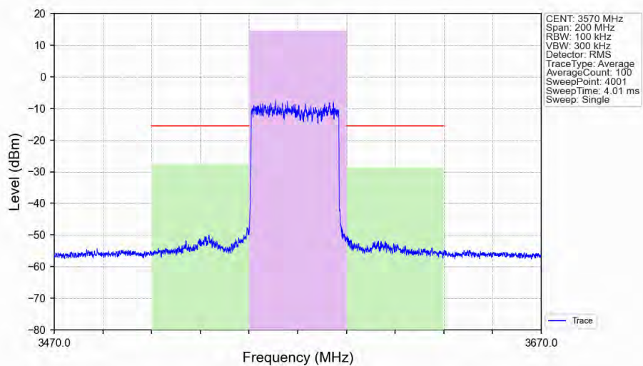
n48_30kHz_SISO_NTNV_40MHz_DFT-s-OFDM PI/2 BPSK_3570MHz_Outer_Full_Ant1
