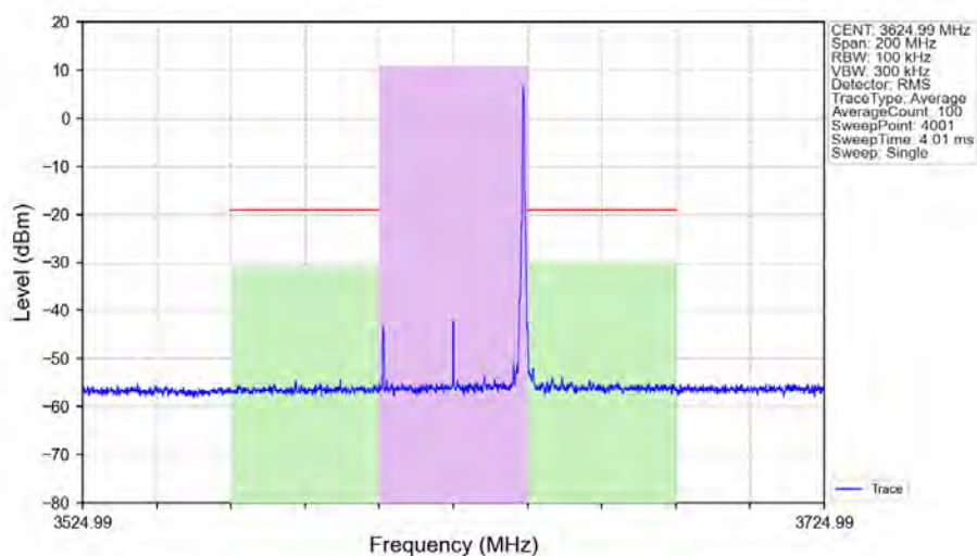
n48_30kHz_SISO_NTNV_40MHz_DFT-s-OFDM_256_QAM_3624.99MHz_Edge_1RB_Right_Ant1
