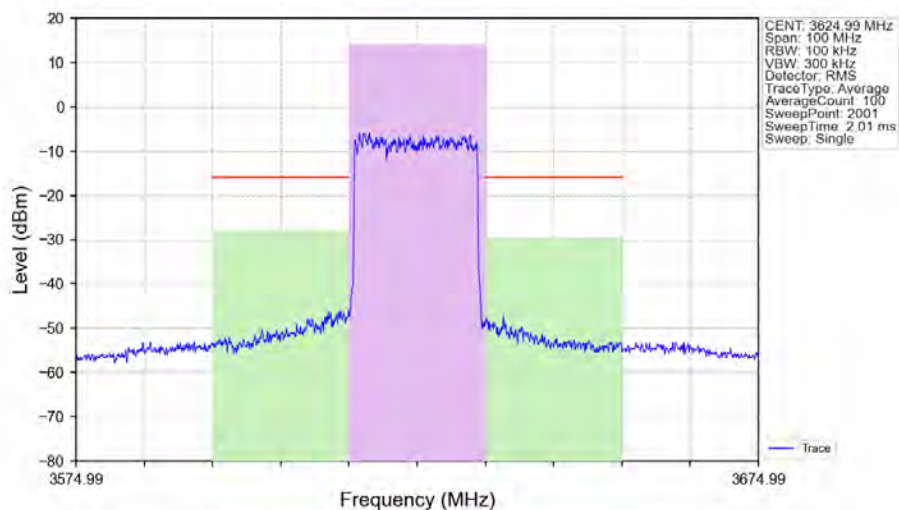
n48_30kHz_SISO_NTNV_20MHz_DFT-s-OFDM_QPSK_3624.99MHz_Outer_Full_Ant1
