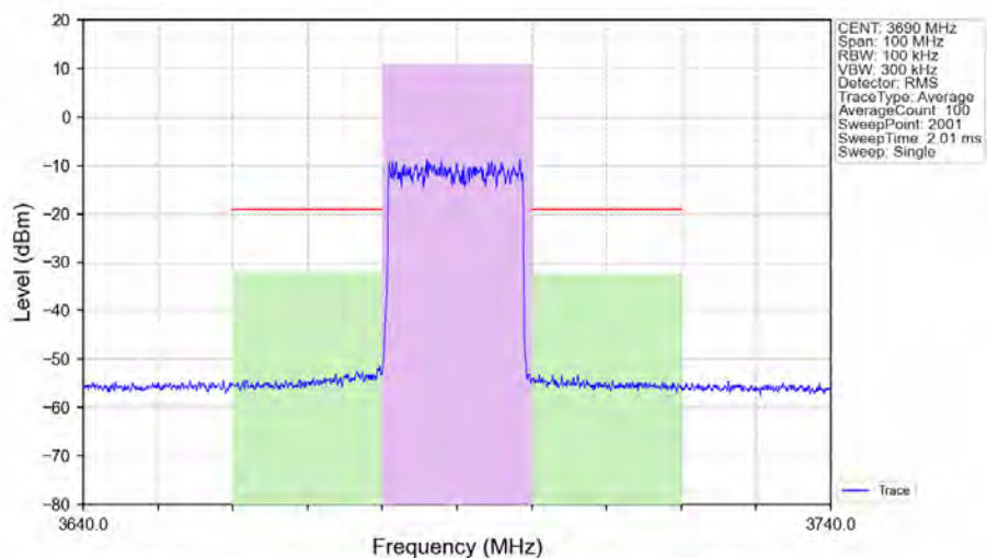
n48_30kHz_SISO_NTNV_20MHz_DFT-s-OFDM 256 QAM 3690MHz_Outer_Full_Ant1
