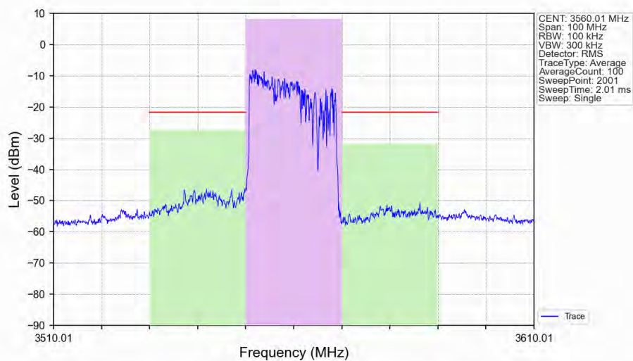
n48_30kHz_SISO_NTNV_20MHz_DFT-s-OFDM PI/2 BPSK_3560.01MHz_Outer_Full_Ant1
