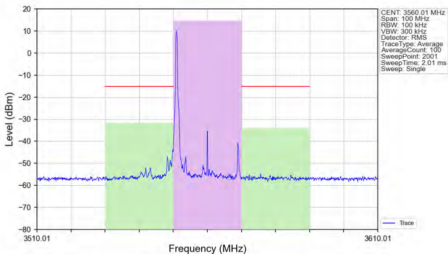
n48_30kHz_SISO_NTNV_20MHz_DFT-s-OFDM_QPSK_3560.01MHz_Edge_1RB_Left_Ant1
