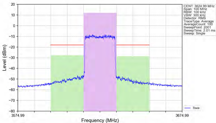
n48_30kHz_SISO_NTNV_20MHz_CP-OFDM_QPSK_3624.99MHz_Outer_Full_Ant1
