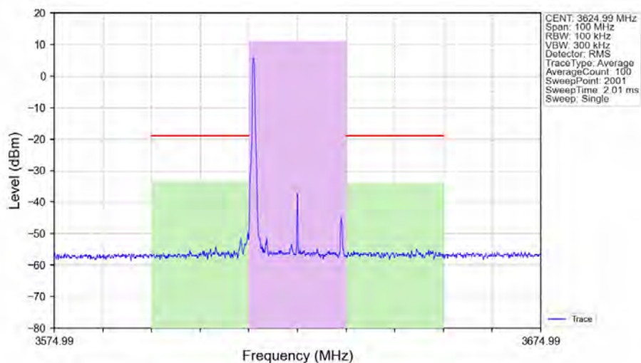
n48_30kHz_SISO_NTNV_20MHz_DFT-s-OFDM_256_QAM_3624.99MHz_Edge_1RB_Left_Ant1
