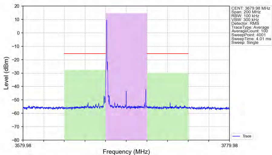
n48_30kHz_SISO_NTNV_40MHz_DFT-s-OFDM_16_QAM_3679.98MHz_Edge_1RB_Left_Ant1
