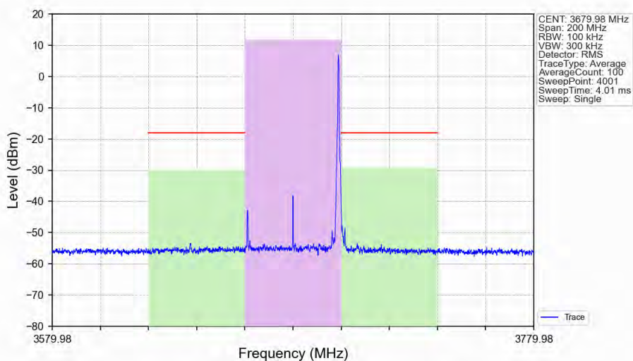
n48_30kHz_SISO_NTNV_40MHz_CP-OFDM_QPSK_3679.98MHz_Edge_1RB_Right_Ant1
