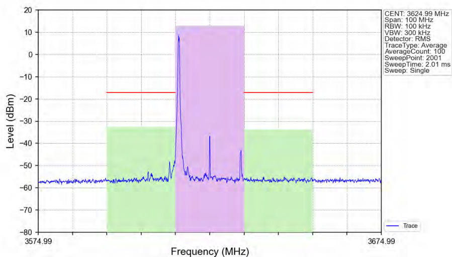
n48_30kHz_SISO_NTNV_20MHz_DFT-s-OFDM_64_QAM_3624.99MHz_Edge_1RB_Left_Ant1
