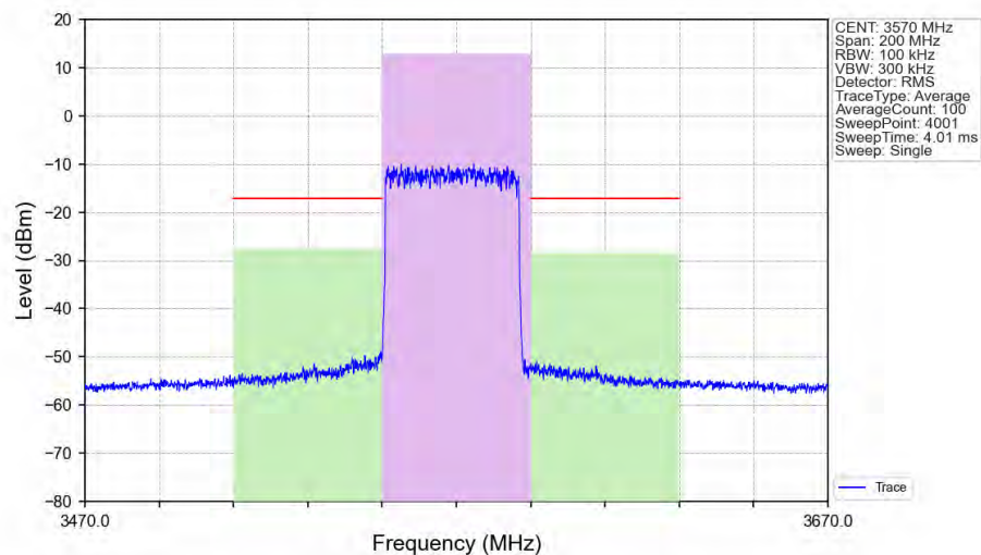
n48_30kHz_SISO_NTNV_40MHz_DFT-s-OFDM_16_QAM_3570MHz_Outer_Full_Ant1
