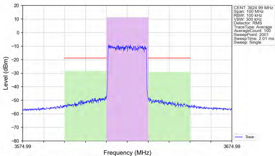
n48_30kHz_SISO_NTNV_20MHz_CP-OFDM_64_QAM_3624.99MHz_Outer_Full_Ant1
