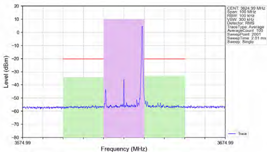
n48_30kHz_SISO_NTNV_20MHz_DFT-s-OFDM_256_QAM_3624.99MHz_Edge_1RB_Right_Ant1
