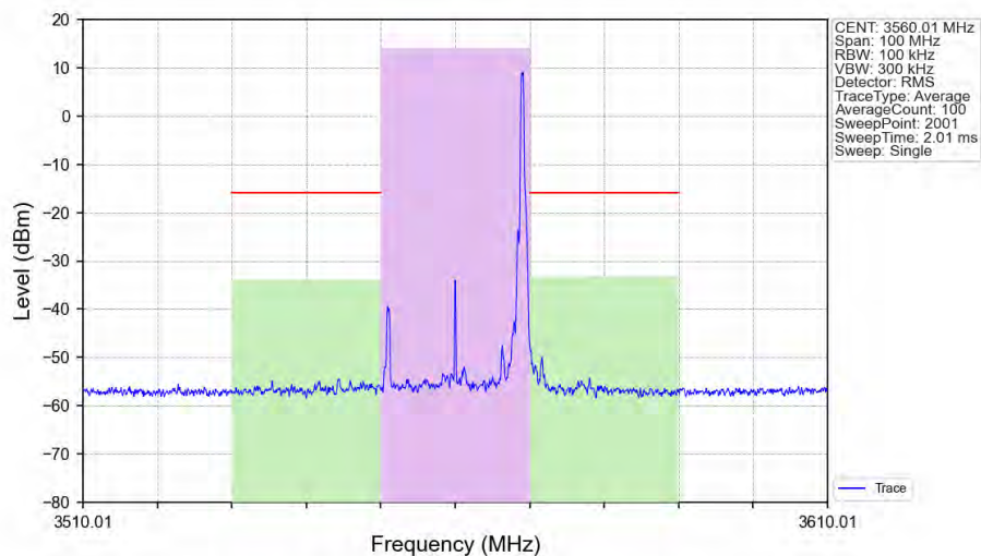
n48_30kHz_SISO_NTNV_20MHz_DFT-s-OFDM 16 QAM_3560.01MHz_Edge_1RB_Right_Ant1
