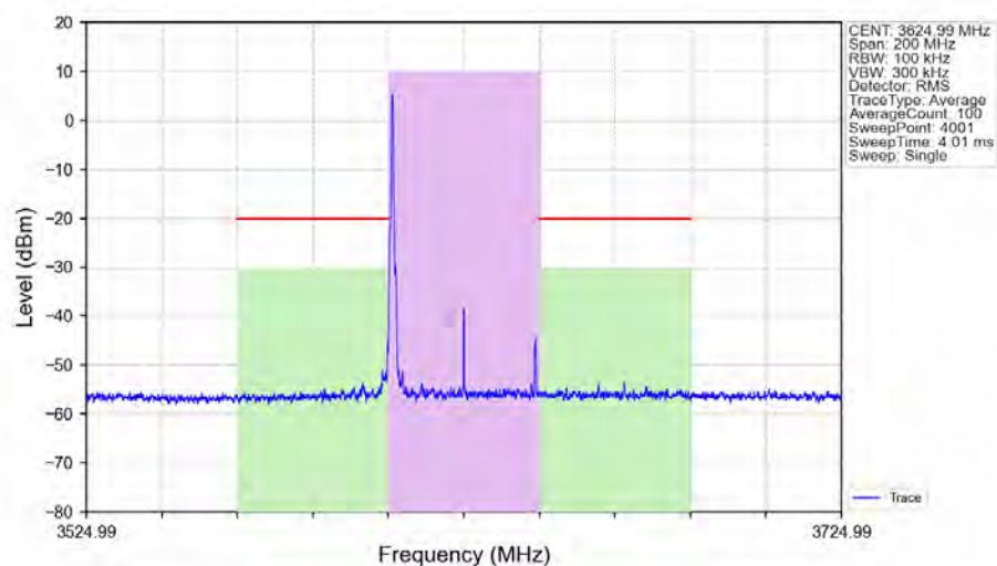
n48_30kHz_SISO_NTNV_40MHz_CP-OFDM_64_QAM_3624.99MHz_Edge_1RB_Left_Ant1
