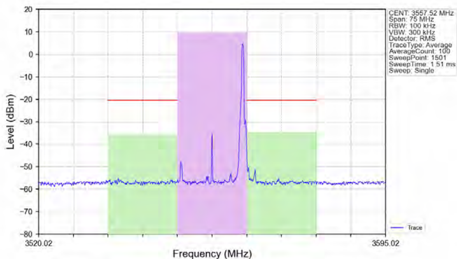
n48_30kHz_SISO_NTNV_15MHz_CP-OFDM 256 QAM 3557.52MHz_Edge_1RB_Right_Ant1
