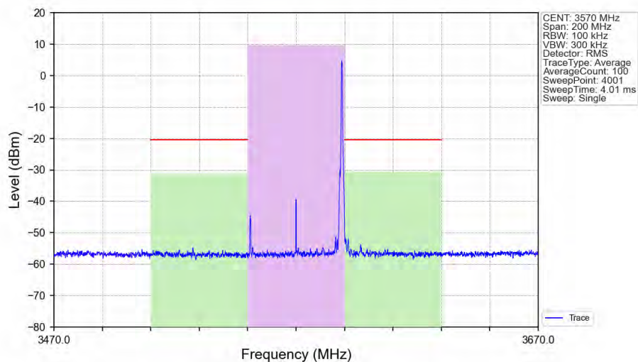
n48_30kHz_SISO_NTNV_40MHz_DFT-s-OFDM_256_QAM_3570MHz_Edge_1RB_Right_Ant1
