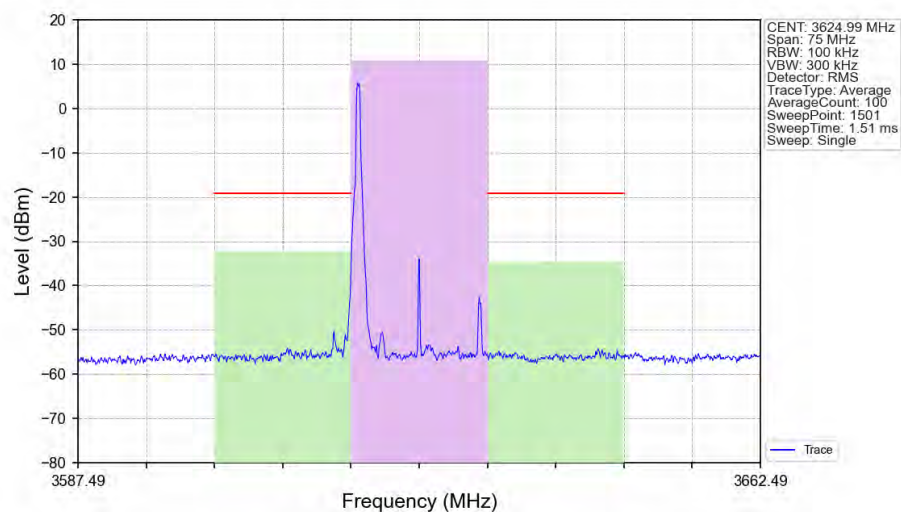
n48_30kHz_SISO_NTNV_15MHz_CP-OFDM_64_QAM_3624.99MHz_Edge_1RB_Left_Ant1
