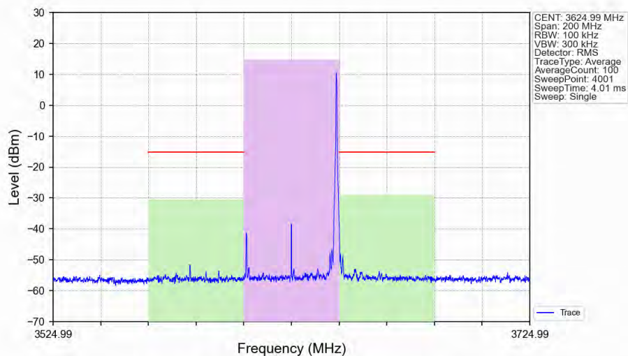
n48_30kHz_SISO_NTNV_40MHz_DFT-s-OFDM_QPSK_3624.99MHz_Edge_1RB_Right_Ant1
