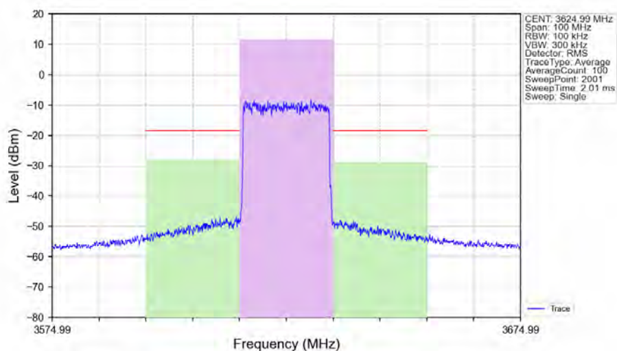
n48_30kHz_SISO_NTNV_20MHz_CP-OFDM_16 QAM_3624.99MHz_Outer_Full_Ant1
