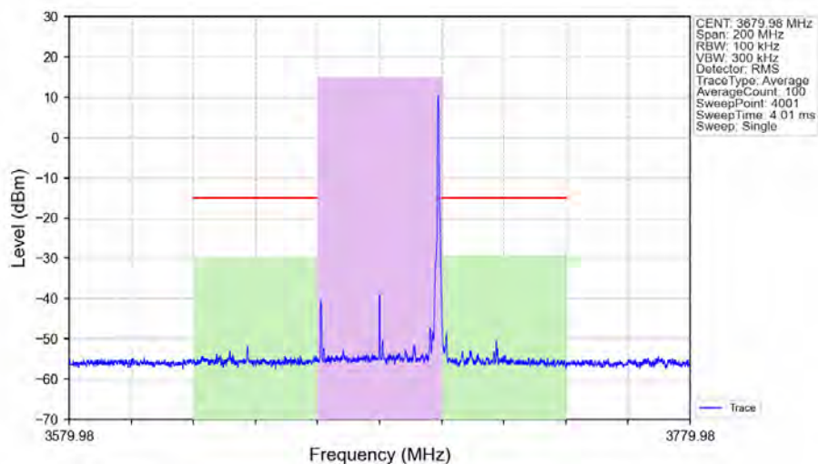
n48_30kHz_SISO_NTNV_40MHz_DFT-s-OFDM PI/2 BPSK 3679.98MHz_Edge_1RB_Right_Ant1
