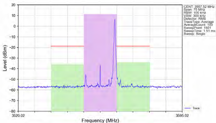
n48_30kHz_SISO_NTNV_15MHz_CP-OFDM_64_QAM_3557.52MHz_Edge_1RB_Right_Ant1
