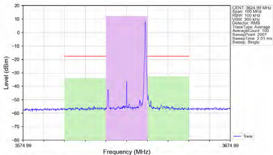
n48_30kHz_SISO_NTNV_20MHz_DFT-s-OFDM 64 QAM_3624.99MHz_Edge_1RB_Right_Ant1
