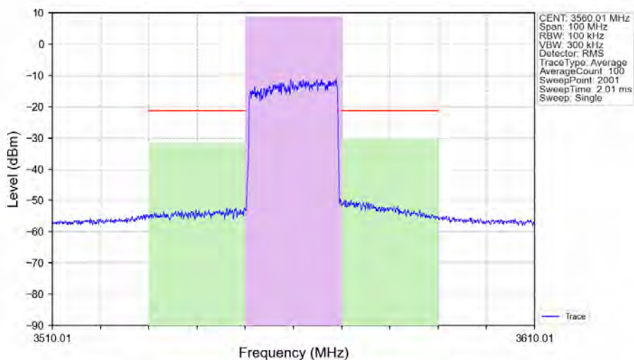
n48_30kHz_SISO_NTNV_20MHz_CP-OFDM 256 QAM 3560.01MHz_Outer_Full_Ant1
