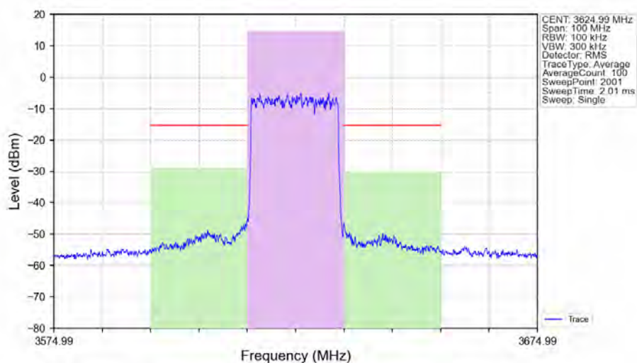
n48_30kHz_SISO_NTNV_20MHz_DFT-s-OFDM_PI/2_BPSK_3624.99MHz_Outer_Full_Ant1
