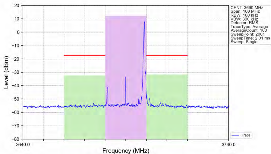
n48_30kHz_SISO_NTNV_20MHz_CP-OFDM 16 QAM_3690MHz_Edge_1RB_Right_Ant1
