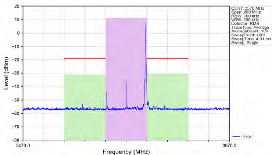
n48_30kHz_SISO_NTNV_40MHz_CP-OFDM_QPSK_3570MHz_Edge_1RB_Right_Ant1
