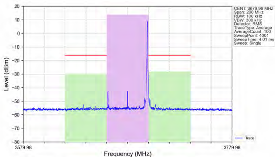
n48_30kHz_SISO_NTNV_40MHz_DFT-s-OFDM_64_QAM_3679.98MHz_Edge_1RB_Right_Ant1
