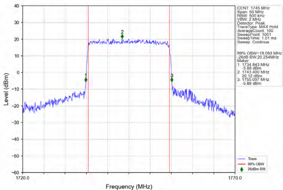
n66 15kHz SISO NTV 20MHz CP-OFDM 16 QAM 1745MHz Outer Full Ant1
