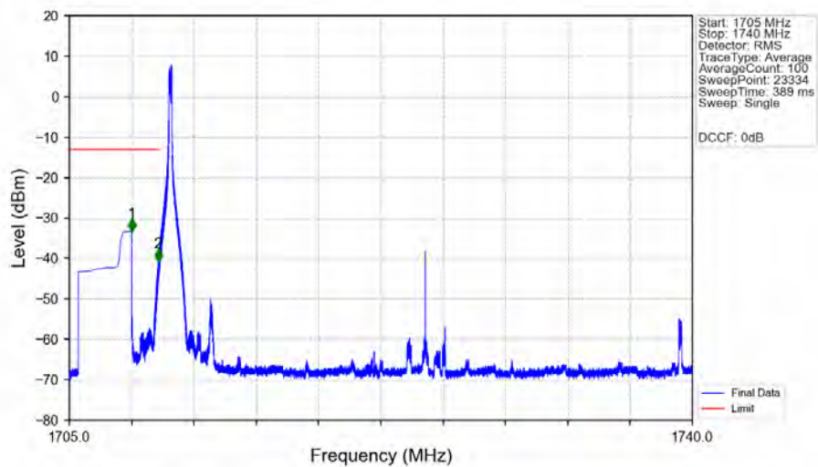
n66_15kHz_MIMO_NTNV_30MHz_DFT-s-OFDM PI/2 BPSK_1725MHz_Edge_1RB_Left_Ant1
