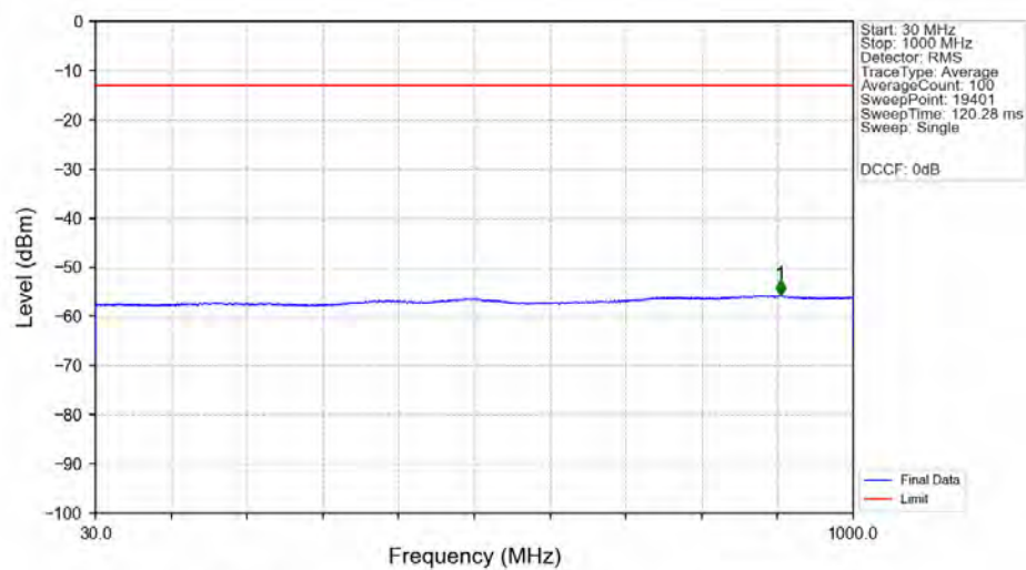
n70_15kHz_SISO_NTNV_10MHz_DFT-s-OFDM PI/2 BPSK_1700MHz_Edge_1RB_Left_Ant1
