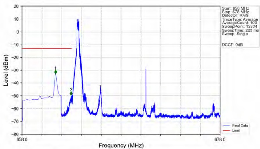
n71 15kHz MIMO NTNV 15MHz DFT-s-OFDM QPSK 670.5MHz Inner 1RB Left Ant2
