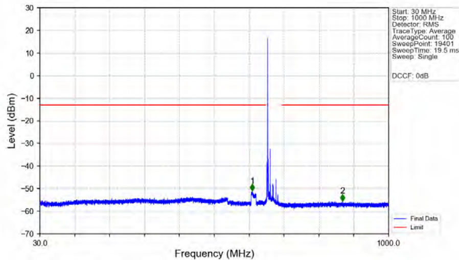
n71_15kHz_MIMO_NTNV_15MHz_DFT-s-OFDM PI/2 BPSK_670.5MHz_Edge_1RB_Left_Ant1
