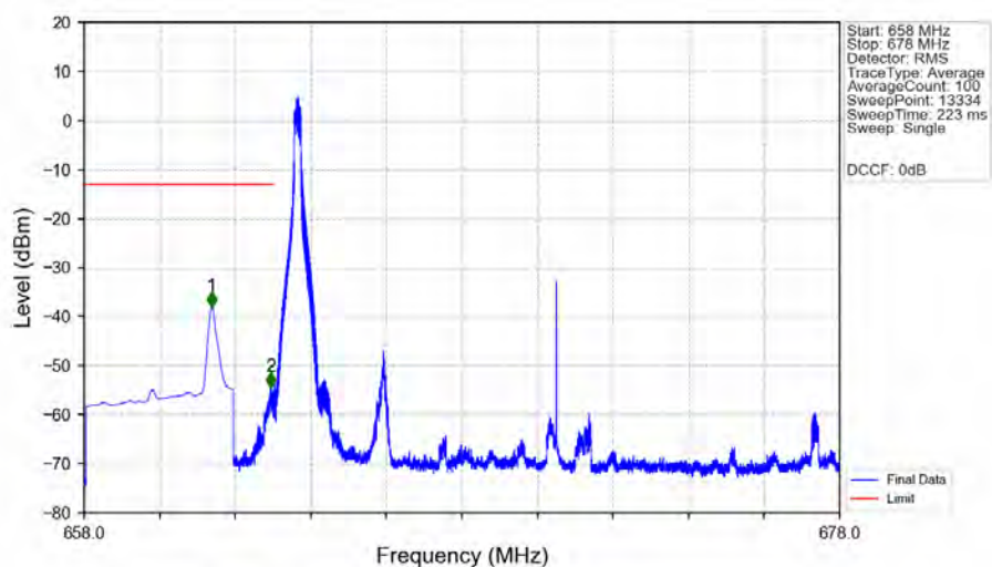
n71 15kHz MIMO NTNV 15MHz DFT-s-OFDM QPSK 670.5MHz Inner 1RB Left Ant1
