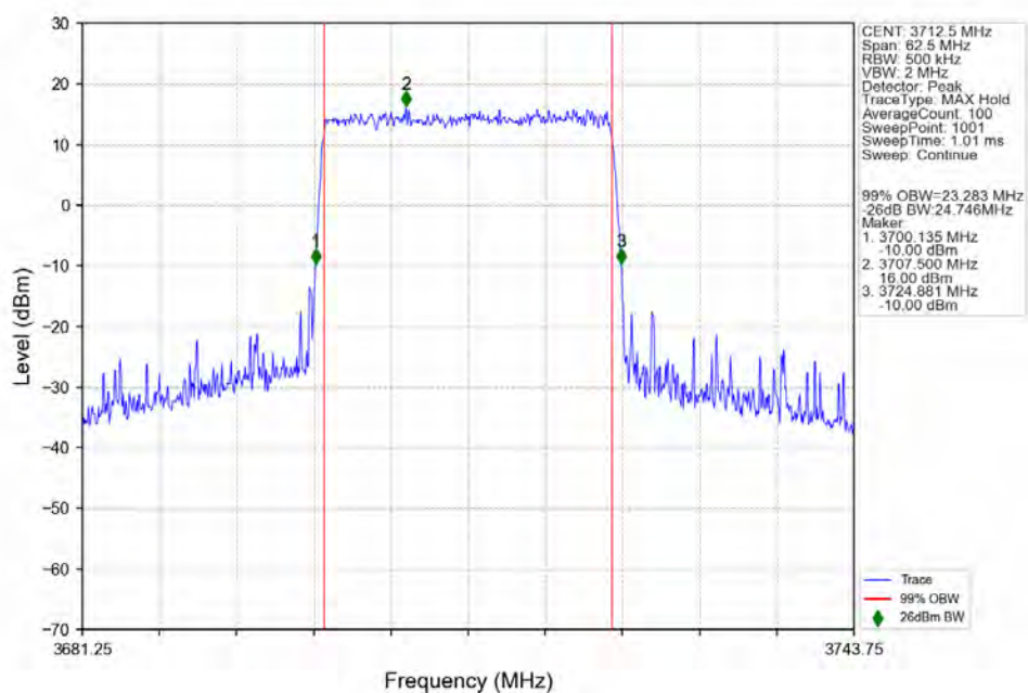
n77a_30kHz_SISO_NTNV_25MHz_CP-OFDM_QPSK_3712.5MHz_Outer_Full_Ant1
