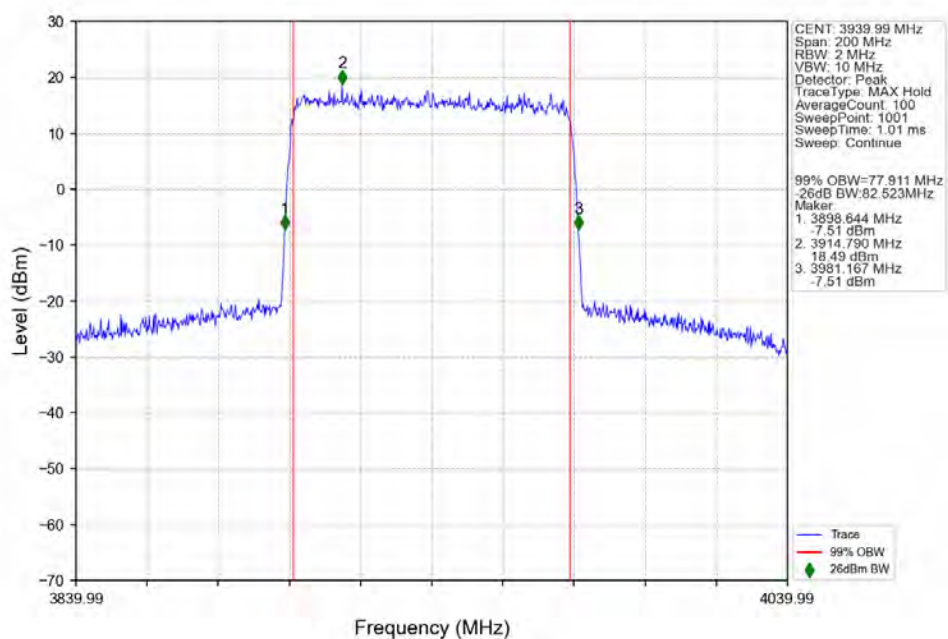
n77a_30kHz_SISO_NTNV_80MHz_CP-OFDM_64_QAM_3939.99MHz_Outer_Full_Ant1
