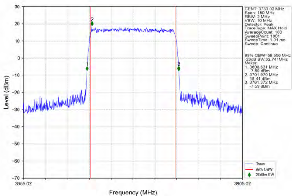
n77a_30kHz_SISO_NTNV_60MHz_CP-OFDM_QPSK_3730.02MHz_Outer_Full_Ant1
