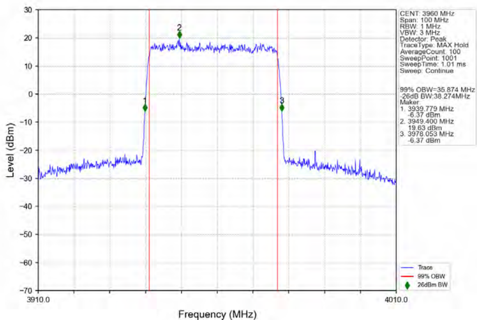
n77a_30kHz_SISO_NTNV_40MHz_DFT-s-OFDM_64_QAM_3960MHz_Outer_Full_Ant1
