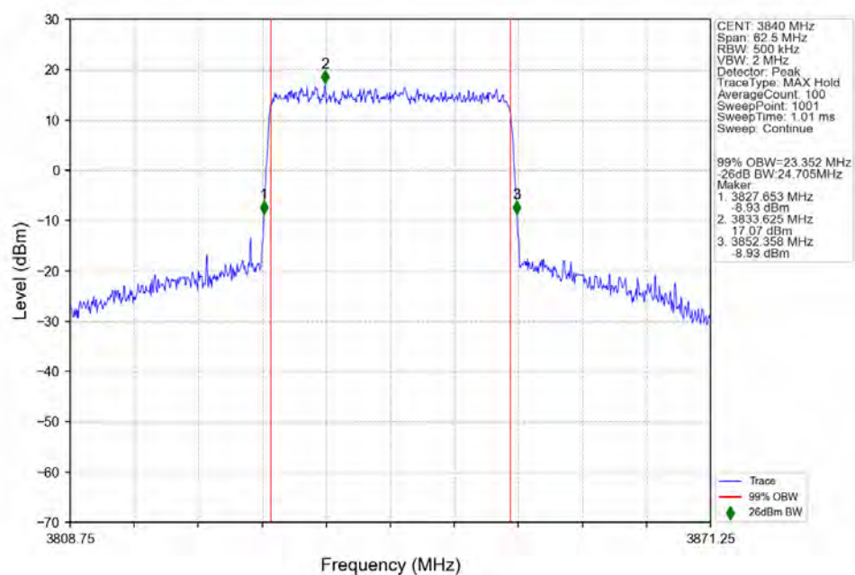
n77a_30kHz_SISO_NTNV_25MHz_CP-OFDM_16_QAM_3840MHz_Outer_Full_Ant1
