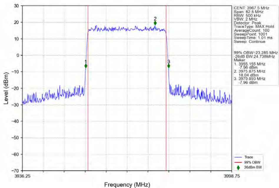
n77a_30kHz_SISO_NTNV_25MHz_CP-OFDM_QPSK_3967.5MHz_Outer_Full_Ant1
