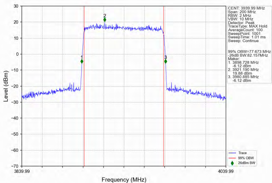
n77a_30kHz_SISO_NTNV_80MHz_DFT-s-OFDM_64_QAM_3939.99MHz_Outer_Full_Ant1
