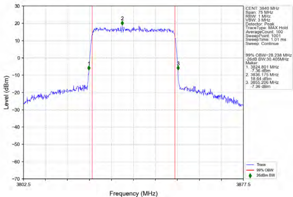
n77a_30kHz_SISO_NTNV_30MHz_CP-OFDM_16_QAM_3840MHz_Outer_Full_Ant1
