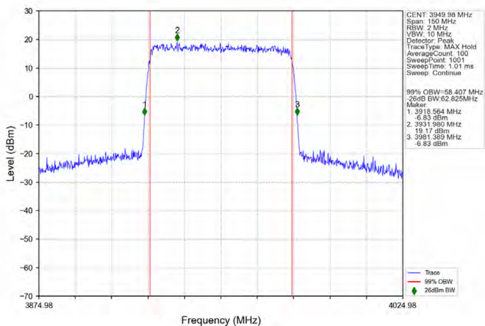
n77a_30kHz_SISO_NTNV_60MHz_CP-OFDM_64_QAM_3949.98MHz_Outer_Full_Ant1
