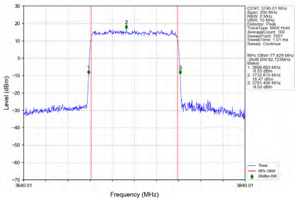
n77a_30kHz_SISO_NTNV_80MHz_CP-OFDM 64 QAM 3740.01MHz_Outer_Full_Ant1
