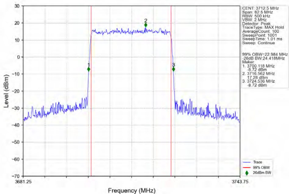
n77a_30kHz_SISO_NTNV_25MHz_DFT-s-OFDM_64_QAM_3712.5MHz_Outer_Full_Ant1
