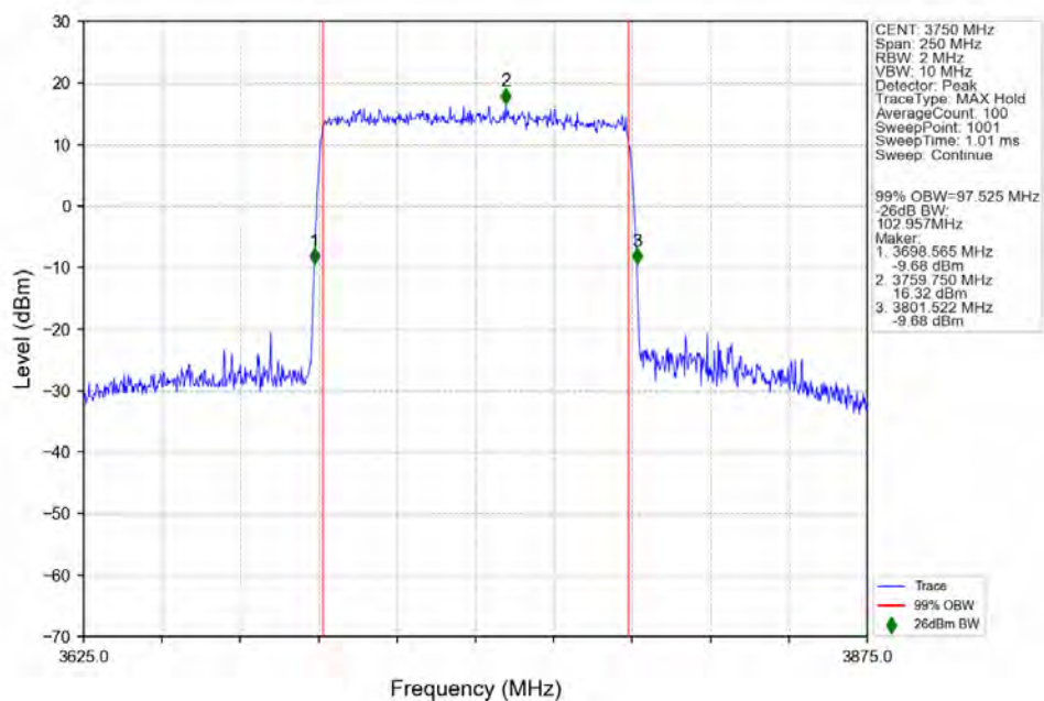
n77a_30kHz_SISO_NTNV_100MHz_CP-OFDM_QPSK_3750MHz_Outer_Full_Ant1
