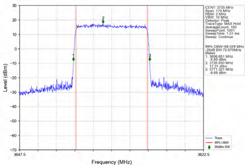
n77a_30kHz_SISO_NTNV_70MHz_CP-OFDM_QPSK_3735MHz_Outer_Full_Ant1
