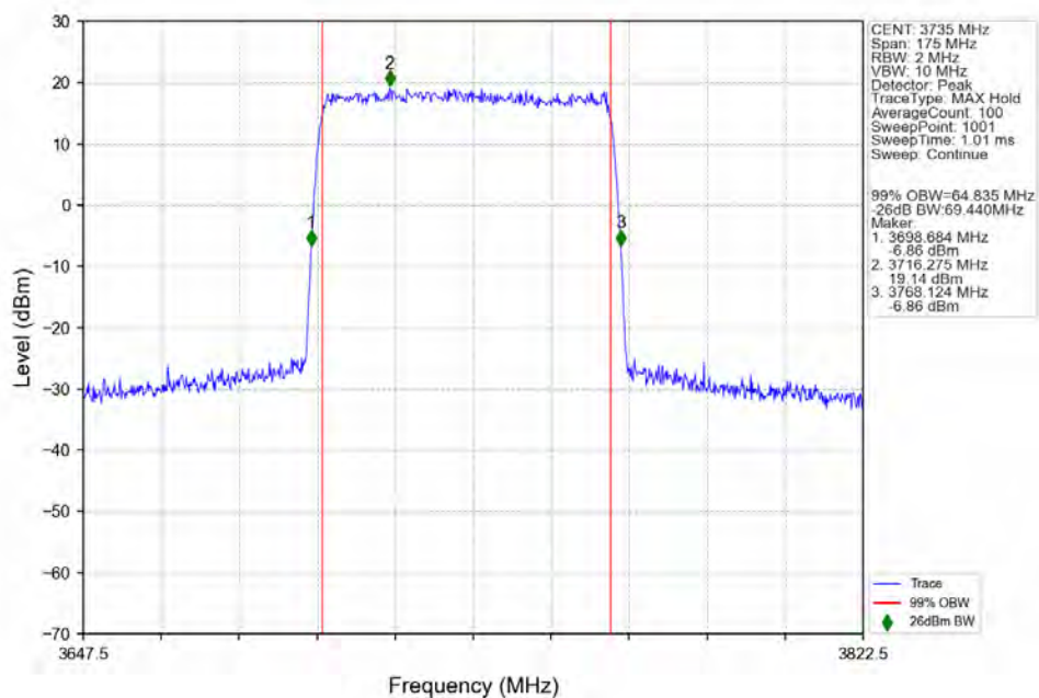
n77a_30kHz_SISO_NTNV_70MHz_DFT-s-OFDM_QPSK_3735MHz_Outer_Full_Ant1
