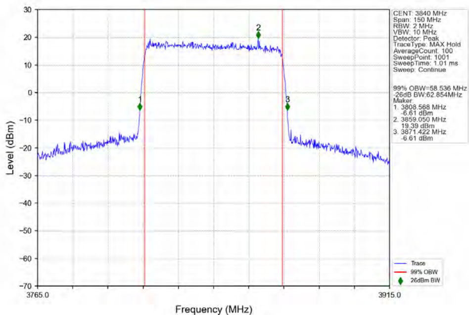
n77a_30kHz_SISO_NTNV_60MHz_CP-OFDM_16_QAM_3840MHz_Outer_Full_Ant1
