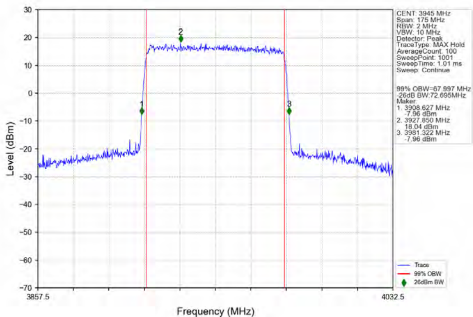
n77a_30kHz_SISO_NTNV_70MHz_CP-OFDM_64_QAM_3945MHz_Outer_Full_Ant1
