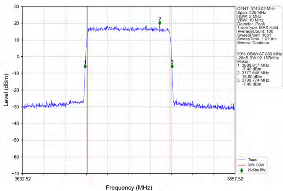
n77a_30kHz_SISO_NTNV_90MHz_DFT-s-OFDM QPSK_3745.02MHz_Outer_Full_Ant1
