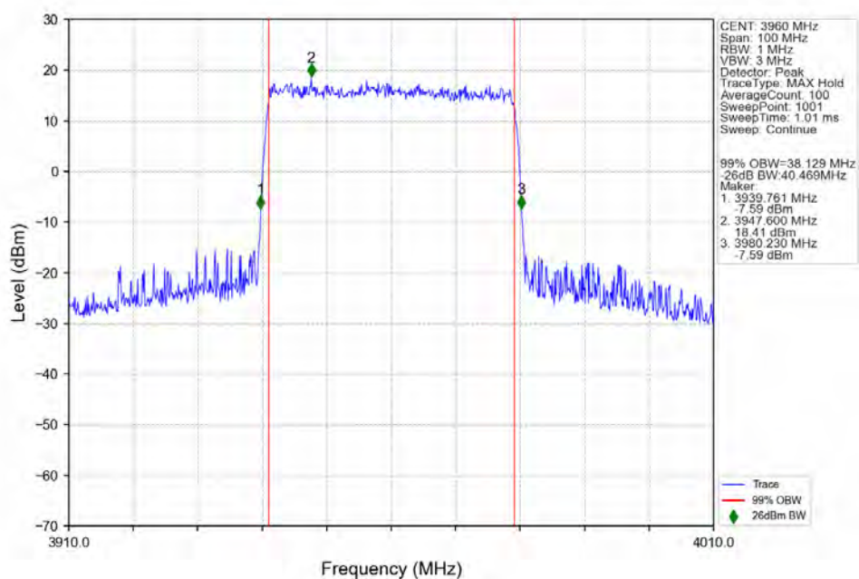
n77a_30kHz_SISO_NTNV_40MHz_CP-OFDM_QPSK_3960MHz_Outer_Full_Ant1
