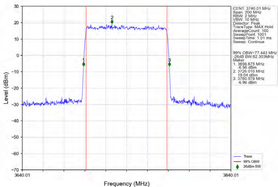
n77a_30kHz_SISO_NTNV_80MHz_DFT-s-OFDM_QPSK_3740.01MHz_Outer_Full_Ant1
