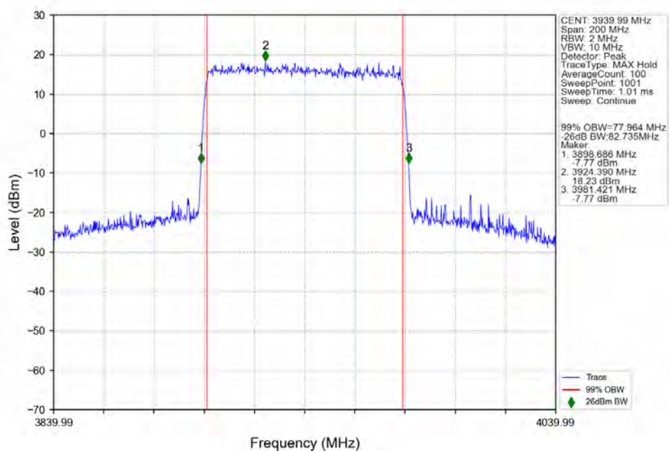
n77a_30kHz_SISO_NTNV_80MHz_CP-OFDM_QPSK_3939.99MHz_Outer_Full_Ant1
