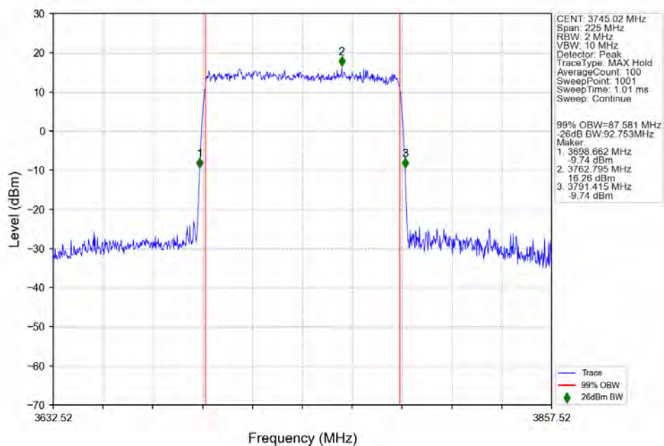
n77a_30kHz_SISO_NTNV_90MHz_CP-OFDM 64 QAM 3745.02MHz_Outer_Full_Ant1
