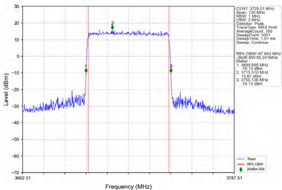
n77a_30kHz_SISO_NTNV_50MHz_CP-OFDM_QPSK_3725.01MHz_Outer_Full_Ant1
