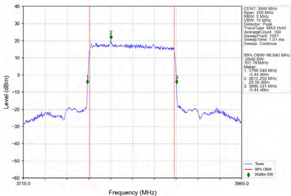
n77a_30kHz_SISO_NTNV_100MHz_DFT-s-OFDM PI/2 BPSK_3840MHz_Outer_Full_Ant1
