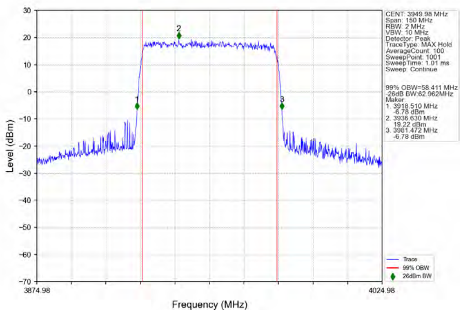
n77a_30kHz_SISO_NTNV_60MHz_CP-OFDM_QPSK_3949.98MHz_Outer_Full_Ant1
