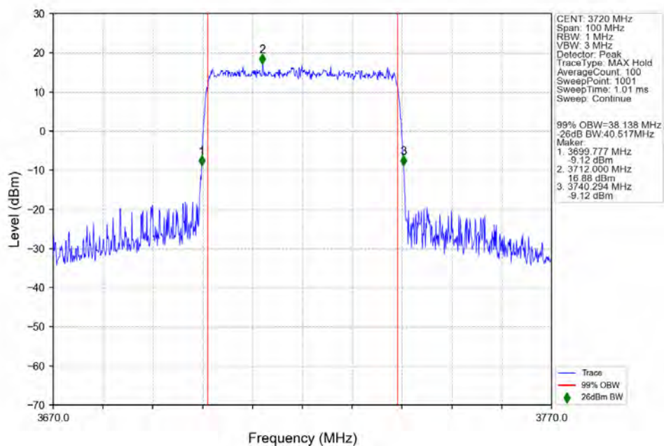
n77a_30kHz_SISO_NTNV_40MHz_CP-OFDM_QPSK_3720MHz_Outer_Full_Ant1
