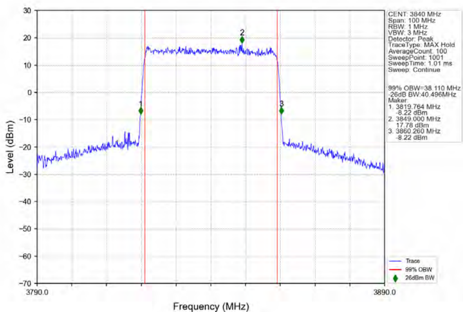
n77a_30kHz_SISO_NTNV_40MHz_CP-OFDM_16_QAM_3840MHz_Outer_Full_Ant1
