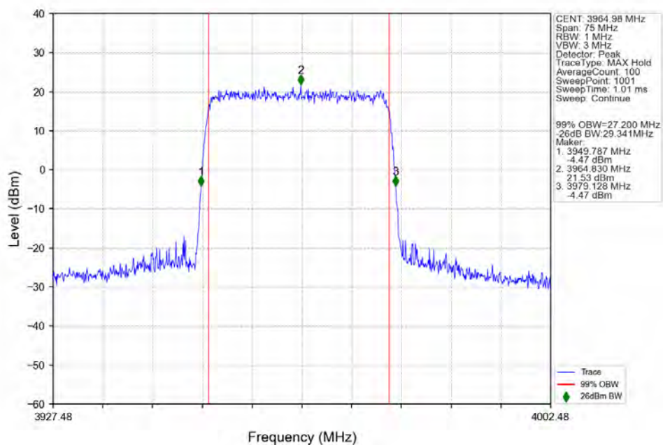
n77a_30kHz_SISO_NTNV_30MHz_DFT-s-OFDM_QPSK_3964.98MHz_Outer_Full_Ant1
