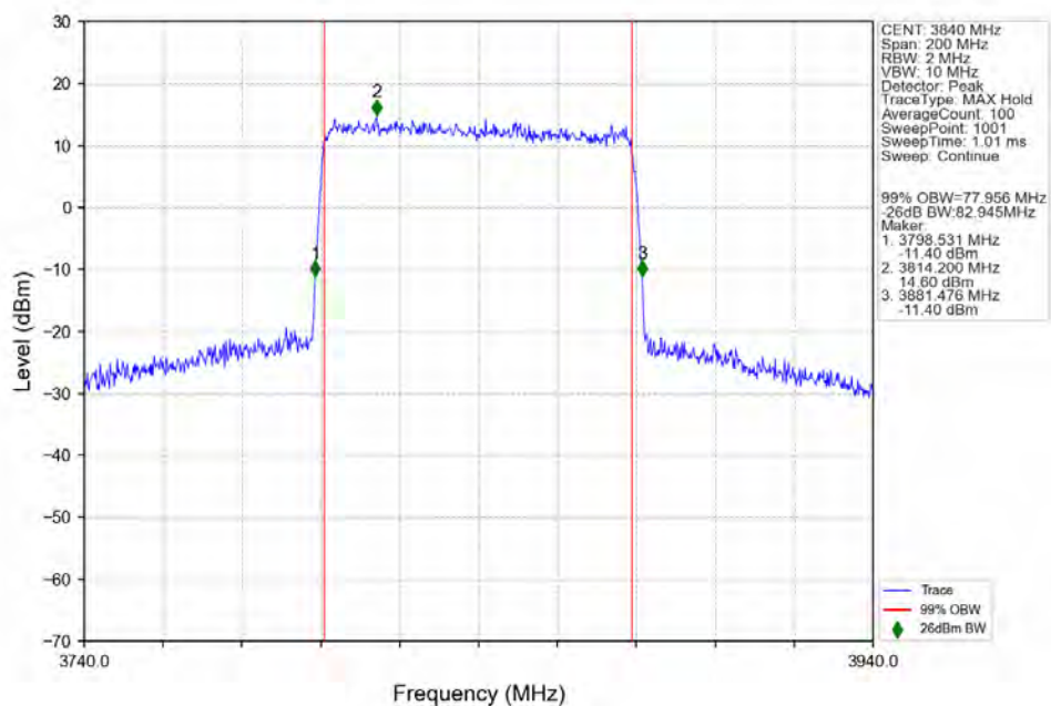
n77a_30kHz_SISO_NTNV_80MHz_CP-OFDM_256_QAM_3840MHz_Outer_Full_Ant1
