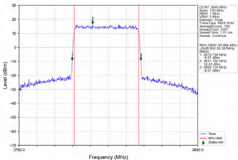
n77a_30kHz_SISO_NTNV_40MHz_DFT-s-OFDM_256_QAM_3840MHz_Outer_Full_Ant1
