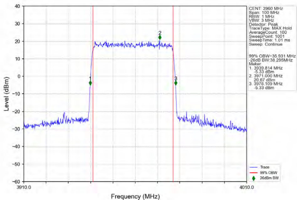
n77a_30kHz_SISO_NTNV_40MHz_DFT-s-OFDM_QPSK_3960MHz_Outer_Full_Ant1
