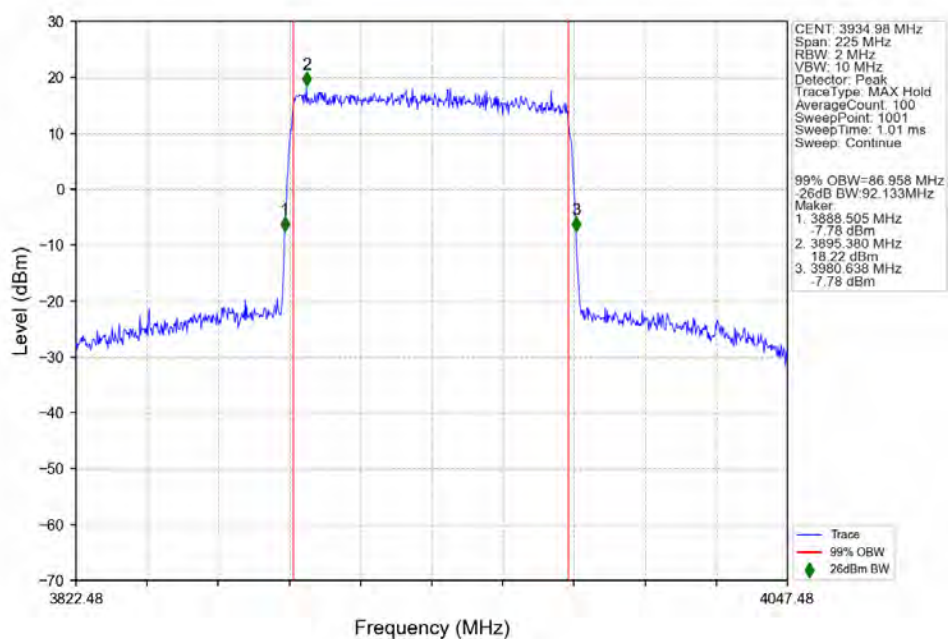
n77a_30kHz_SISO_NTNV_90MHz_DFT-s-OFDM_64_QAM_3934.98MHz_Outer_Full_Ant1
