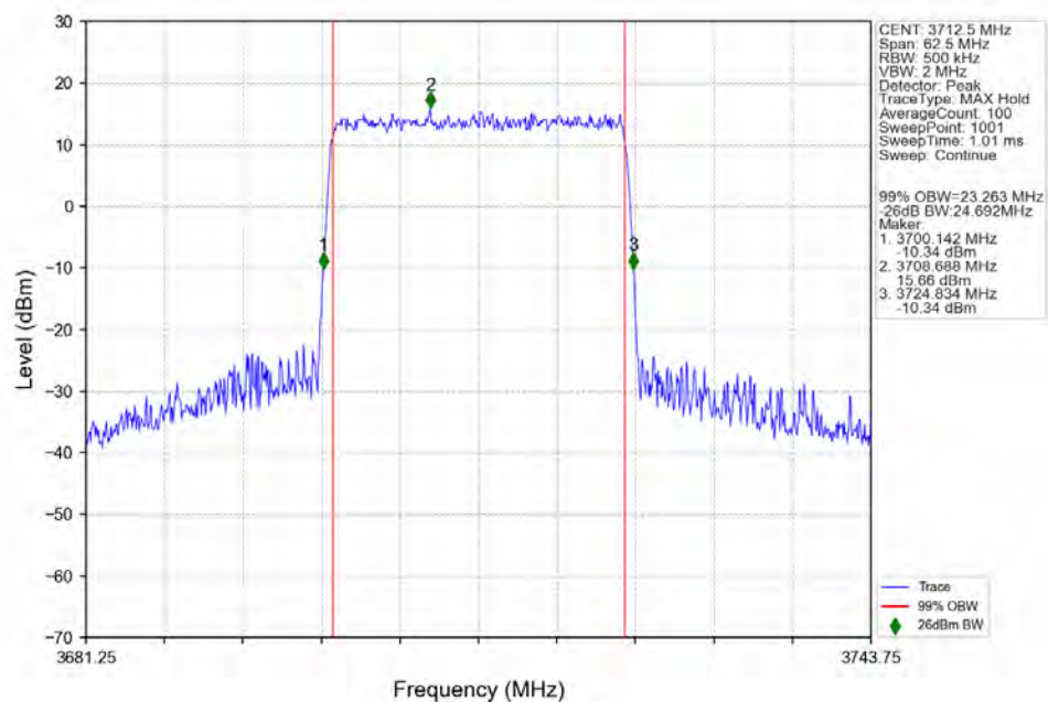
n77a_30kHz_SISO_NTNV_25MHz_CP-OFDM_64_QAM_3712.5MHz_Outer_Full_Ant1
