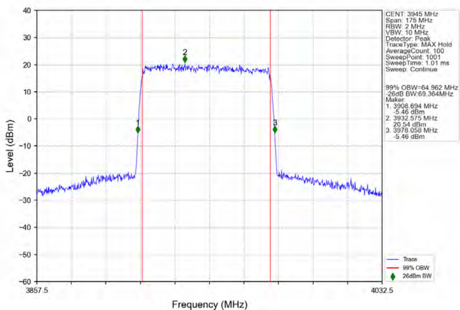
n77a_30kHz_SISO_NTNV_70MHz_DFT-s-OFDM_QPSK_3945MHz_Outer_Full_Ant1
