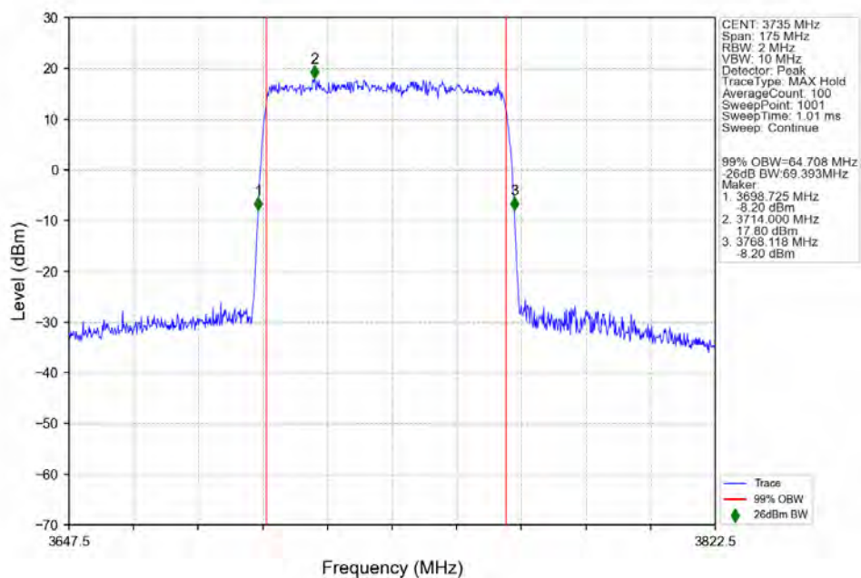
n77a_30kHz_SISO_NTNV_70MHz_DFT-s-OFDM_64_QAM_3735MHz_Outer_Full_Ant1
