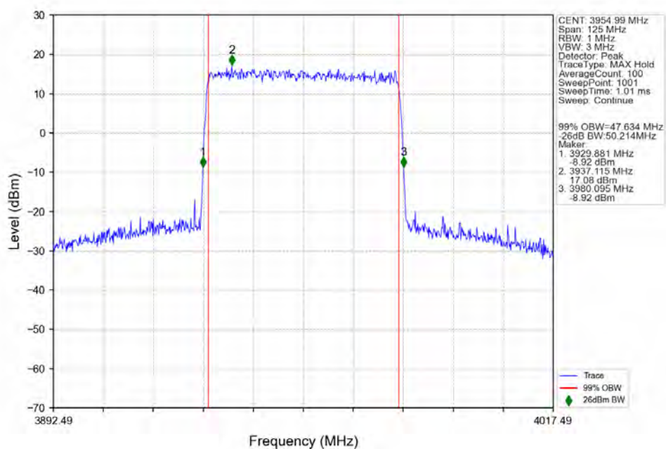
n77a_30kHz_SISO_NTNV_50MHz_CP-OFDM_QPSK_3954.99MHz_Outer_Full_Ant1
