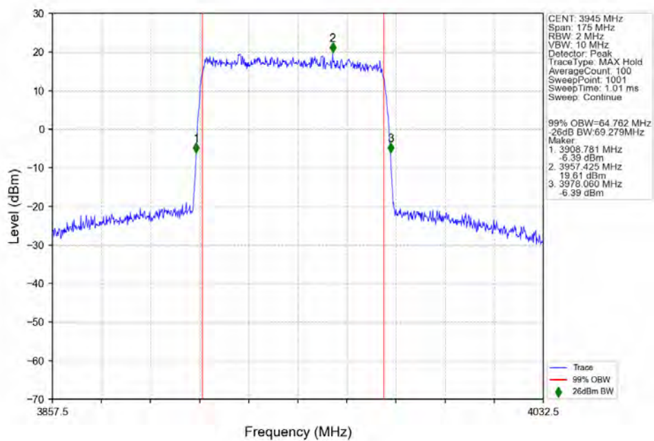
n77a_30kHz_SISO_NTNV_70MHz_DFT-s-OFDM_64_QAM_3945MHz_Outer_Full_Ant1
