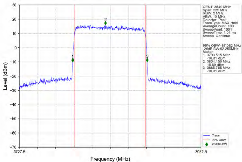
n77a_30kHz_SISO_NTNV_90MHz_DFT-s-OFDM_256_QAM_3840MHz_Outer_Full_Ant1
