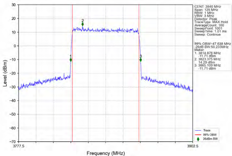
n77a_30kHz_SISO_NTNV_50MHz_CP-OFDM_256_QAM_3840MHz_Outer_Full_Ant1
