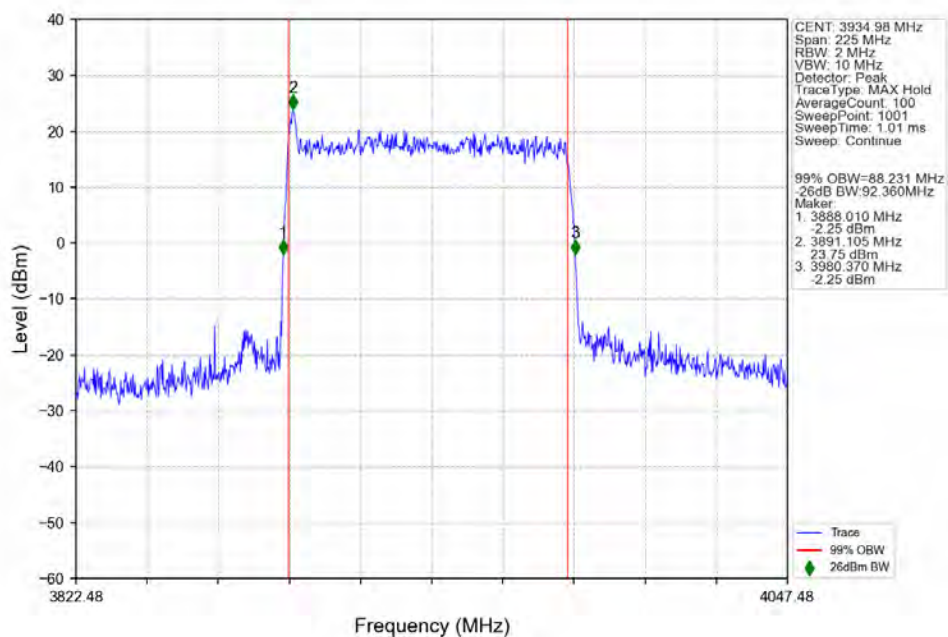
n77a_30kHz_SISO_NTNV_90MHz_DFT-s-OFDM_QPSK_3934.98MHz_Outer_Full_Ant1
