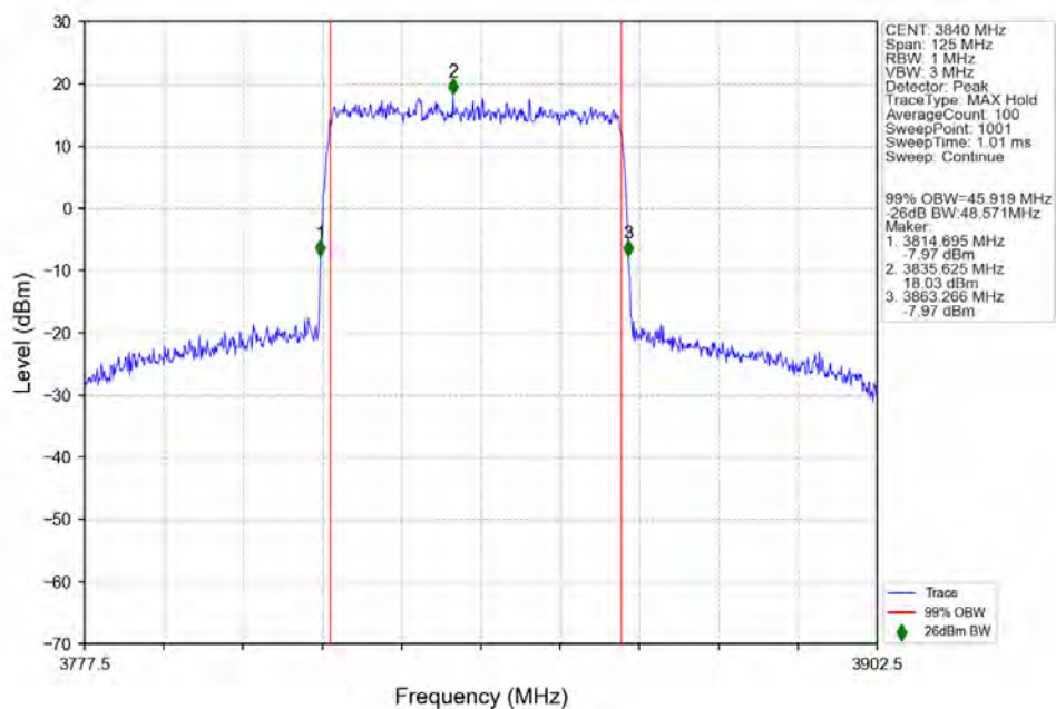
n77a_30kHz_SISO_NTNV_50MHz_DFT-s-OFDM_16_QAM_3840MHz_Outer_Full_Ant1
