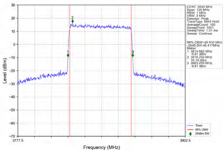
n77a_30kHz_SISO_NTNV_50MHz_DFT-s-OFDM_256_QAM_3840MHz_Outer_Full_Ant1
