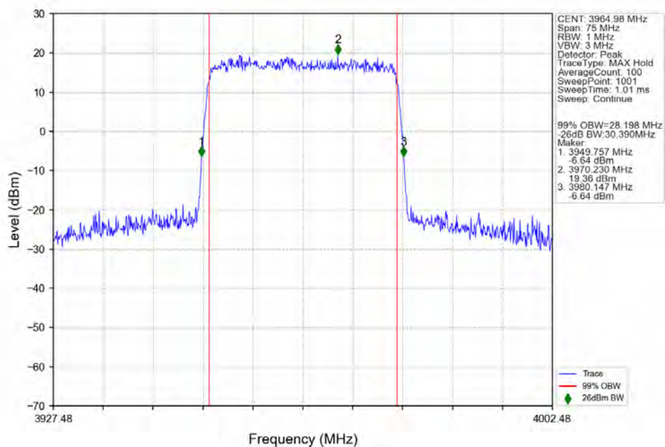
n77a_30kHz_SISO_NTNV_30MHz_CP-OFDM_64_QAM_3964.98MHz_Outer_Full_Ant1
