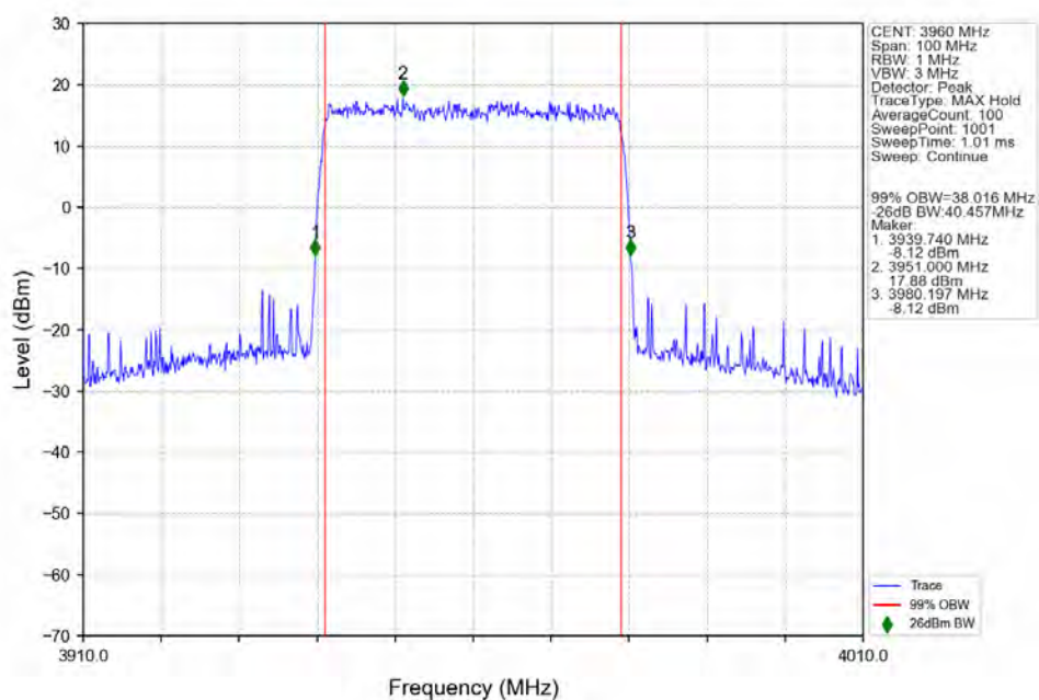
n77a_30kHz_SISO_NTNV_40MHz_CP-OFDM_64_QAM_3960MHz_Outer_Full_Ant1
