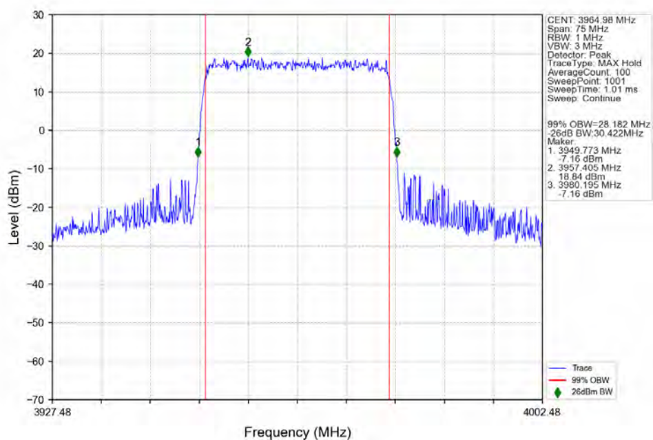
n77a_30kHz_SISO_NTNV_30MHz_CP-OFDM_QPSK_3964.98MHz_Outer_Full_Ant1
