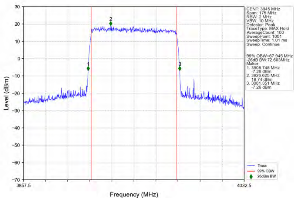
n77a_30kHz_SISO_NTNV_70MHz_CP-OFDM_QPSK_3945MHz_Outer_Full_Ant1
