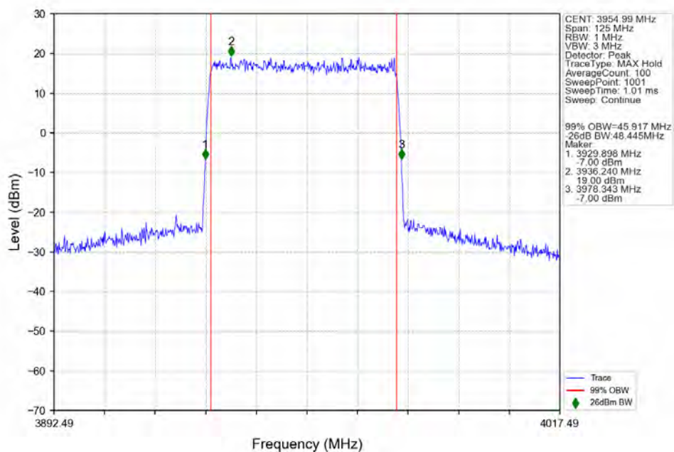
n77a_30kHz_SISO_NTNV_50MHz_DFT-s-OFDM_QPSK_3954.99MHz_Outer_Full_Ant1
