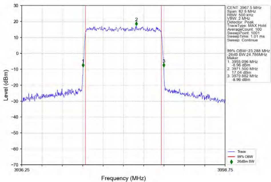
n77a_30kHz_SISO_NTNV_25MHz_CP-OFDM_64_QAM_3967.5MHz_Outer_Full_Ant1
