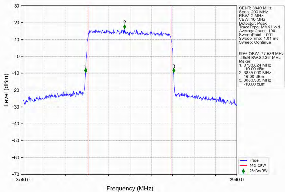
n77a_30kHz_SISO_NTNV_80MHz_DFT-s-OFDM_256_QAM_3840MHz_Outer_Full_Ant1
