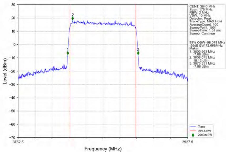
n77a_30kHz_SISO_NTNV_70MHz_CP-OFDM_16_QAM_3840MHz_Outer_Full_Ant1
