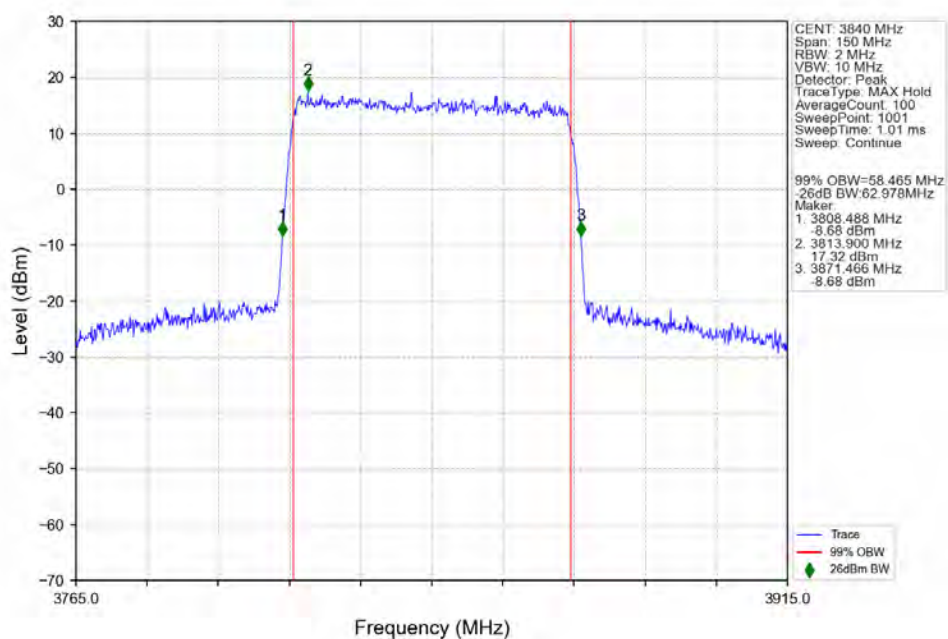
n77a_30kHz_SISO_NTNV_60MHz_DFT-s-OFDM_256_QAM_3840MHz_Outer_Full_Ant1
