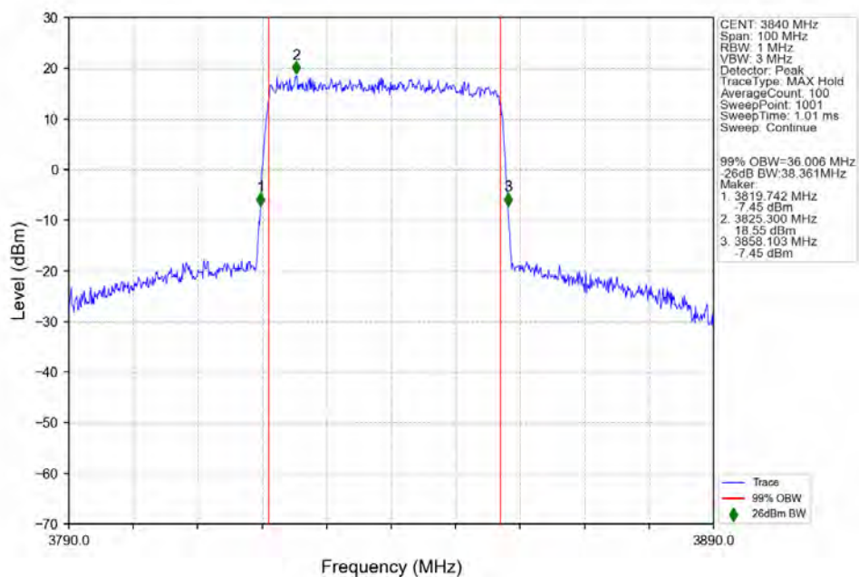
n77a_30kHz_SISO_NTNV_40MHz_DFT-s-OFDM_16_QAM_3840MHz_Outer_Full_Ant1
