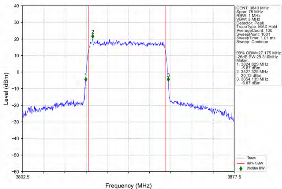
n77a_30kHz_SISO_NTNV_30MHz_DFT-s-OFDM_16_QAM_3840MHz_Outer_Full_Ant1
