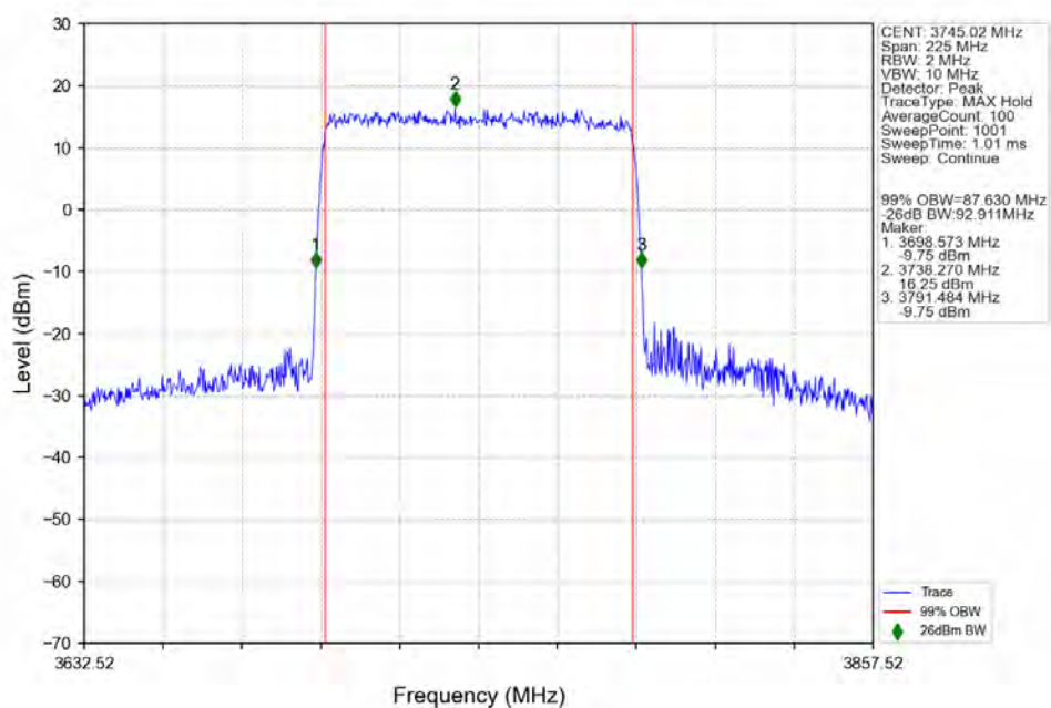
n77a_30kHz_SISO_NTNV_90MHz_CP-OFDM_QPSK_3745.02MHz_Outer_Full_Ant1
