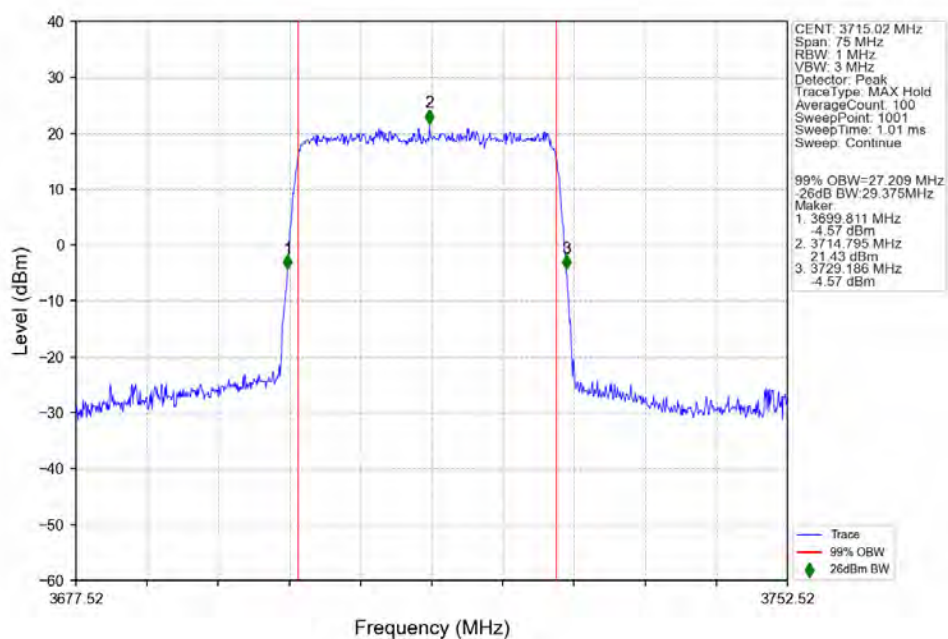
n77a_30kHz_SISO_NTNV_30MHz_DFT-s-OFDM QPSK_3715.02MHz_Outer_Full_Ant1
