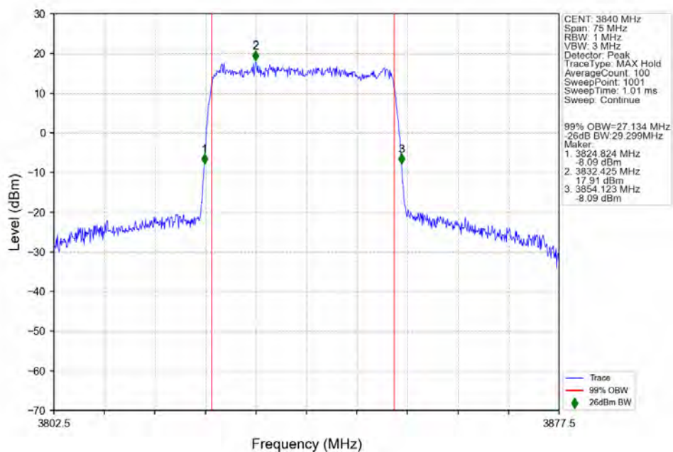
n77a_30kHz_SISO_NTNV_30MHz_DFT-s-OFDM_256_QAM_3840MHz_Outer_Full_Ant1
