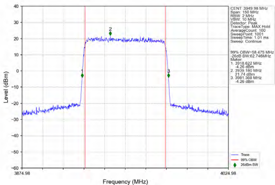
n77a_30kHz_SISO_NTNV_60MHz_DFT-s-OFDM_QPSK_3949.98MHz_Outer_Full_Ant1
