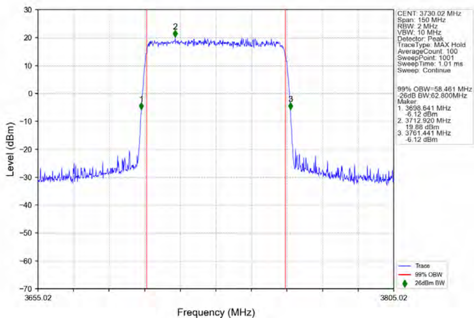
n77a_30kHz_SISO_NTNV_60MHz_DFT-s-OFDM_QPSK_3730.02MHz_Outer_Full_Ant1
