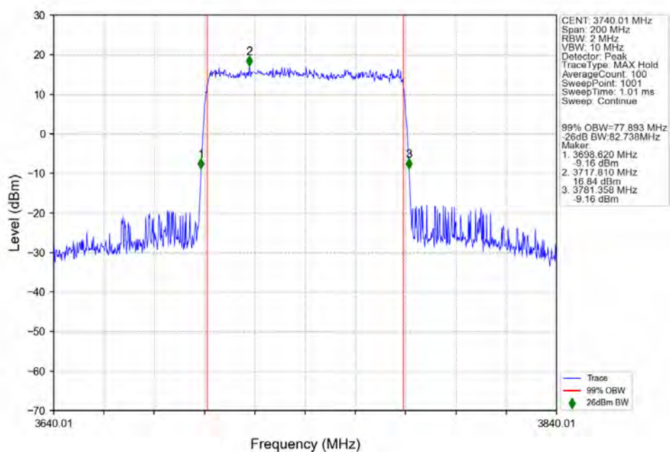
n77a_30kHz_SISO_NTNV_80MHz_CP-OFDM_QPSK_3740.01MHz_Outer_Full_Ant1
