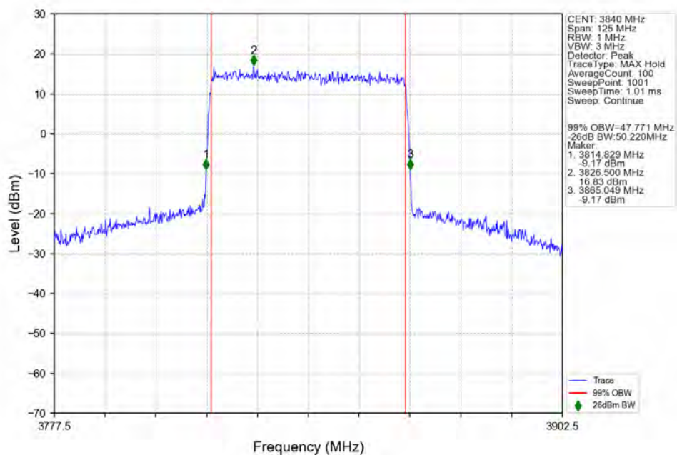
n77a_30kHz_SISO_NTNV_50MHz_CP-OFDM_16_QAM_3840MHz_Outer_Full_Ant1
