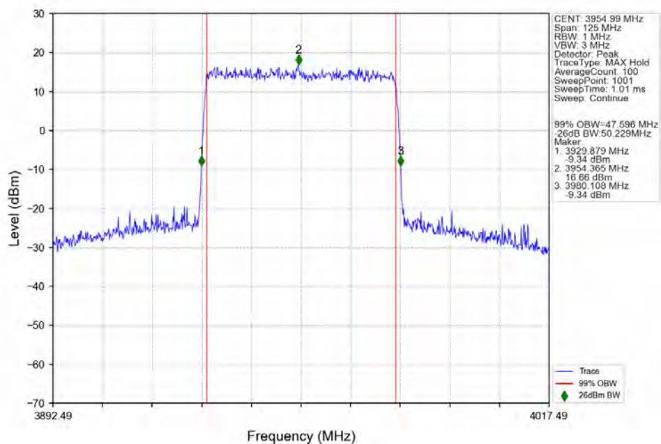
n77a_30kHz_SISO_NTNV_50MHz_CP-OFDM_64_QAM_3954.99MHz_Outer_Full_Ant1
