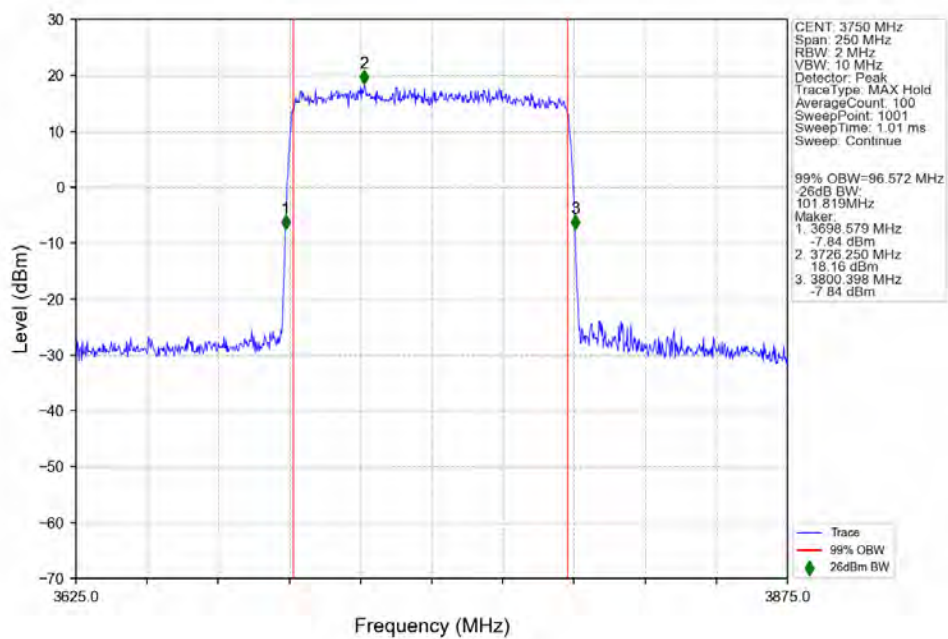
n77a_30kHz_SISO_NTNV_100MHz_DFT-s-OFDM_QPSK_3750MHz_Outer_Full_Ant1
