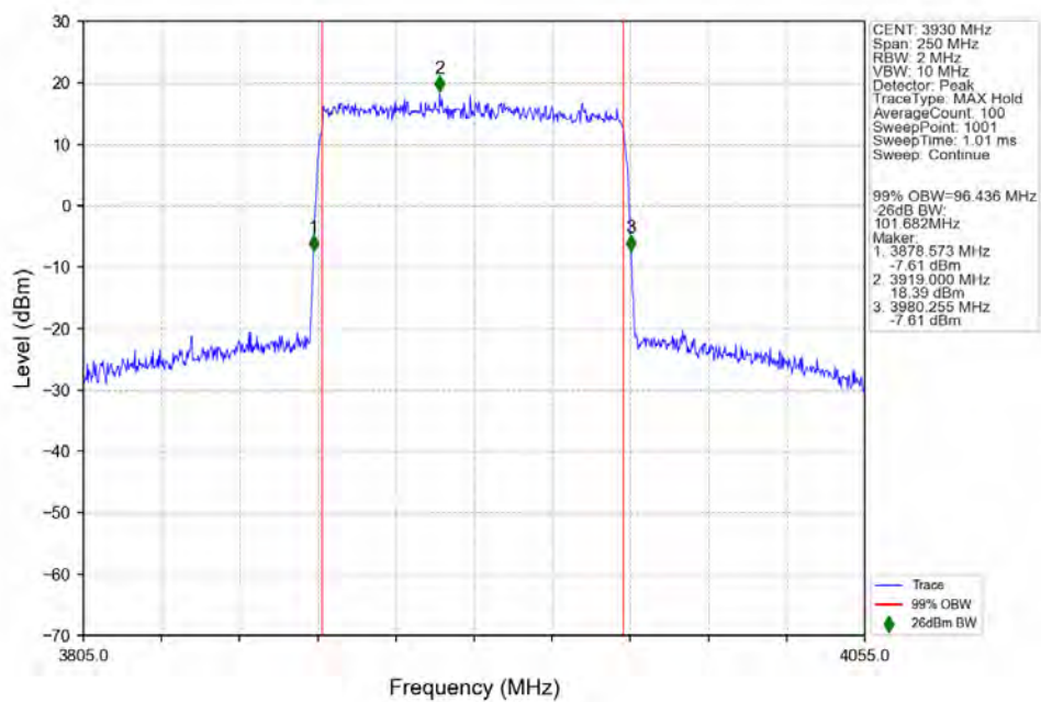
n77a_30kHz_SISO_NTNV_100MHz_DFT-s-OFDM_64_QAM_3930MHz_Outer_Full_Ant1
