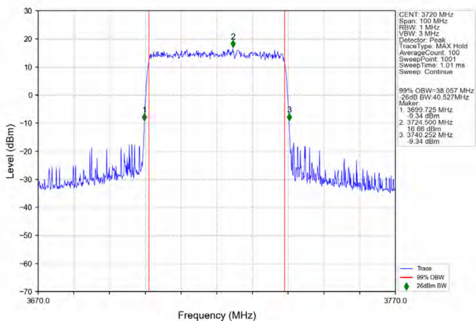
n77a_30kHz_SISO_NTNV_40MHz_CP-OFDM_64 QAM_3720MHz_Outer_Full_Ant1
