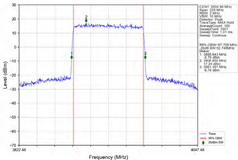
n77a_30kHz_SISO_NTNV_90MHz_CP-OFDM_64_QAM_3934.98MHz_Outer_Full_Ant1
