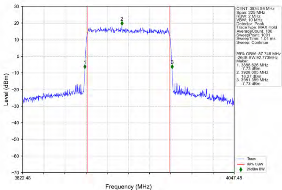
n77a_30kHz_SISO_NTNV_90MHz_CP-OFDM_QPSK_3934.98MHz_Outer_Full_Ant1
