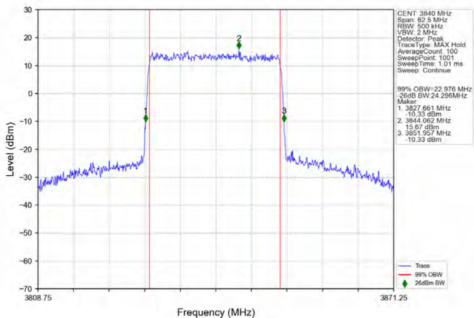
n77a_30kHz_SISO_NTNV_25MHz_DFT-s-OFDM_256_QAM_3840MHz_Outer_Full_Ant1
