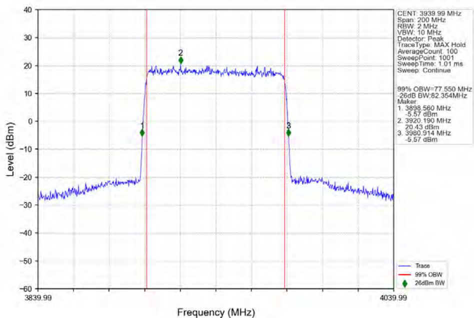
n77a_30kHz_SISO_NTNV_80MHz_DFT-s-OFDM_QPSK_3939.99MHz_Outer_Full_Ant1
