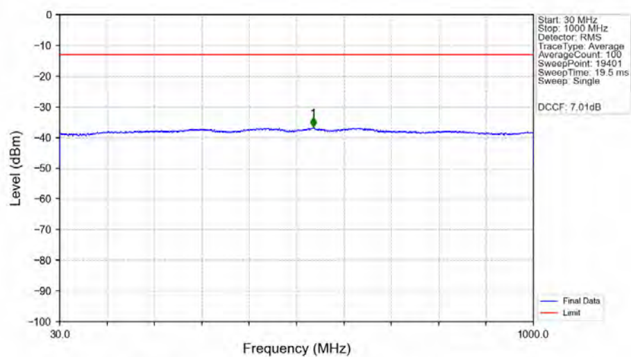
n77a_30kHz_SISO_NTNV_50MHz_CP-OFDM_QPSK_3840MHz_Edge_1RB_Left_Ant1
