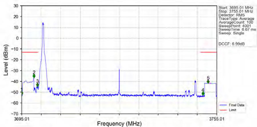
n77a_30kHz_SISO_NTNV_50MHz_CP-OFDM_QPSK_3725.01MHz_Inner_1RB_Left_Ant1
