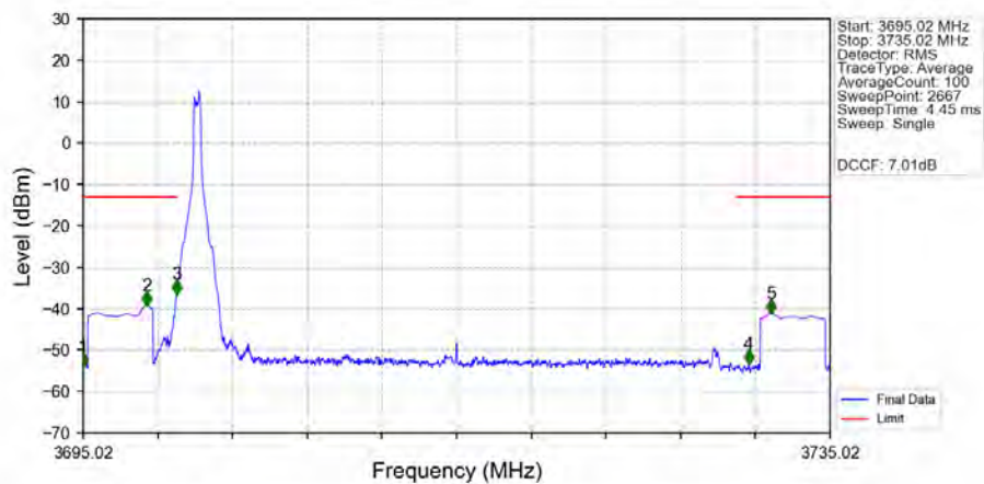
n77a_30kHz_SISO_NTNV_30MHz_DFT-s-OFDM PI/2 BPSK_3715.02MHz_Edge_1RB_Left_Ant1
