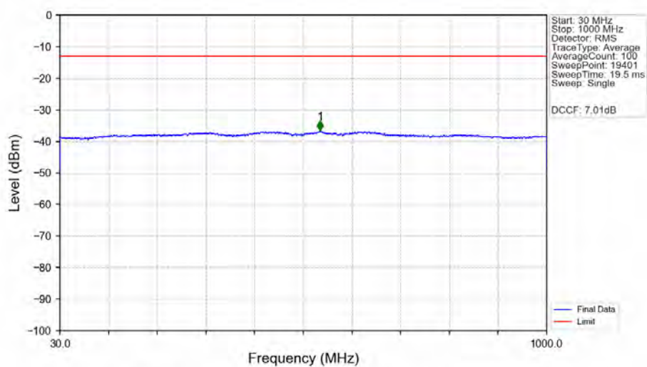
n77a_30kHz_SISO_NTNV_80MHz_DFT-s-OFDM_PI/2_BPSK_3840MHz_Edge_1RB_Left_Ant1
