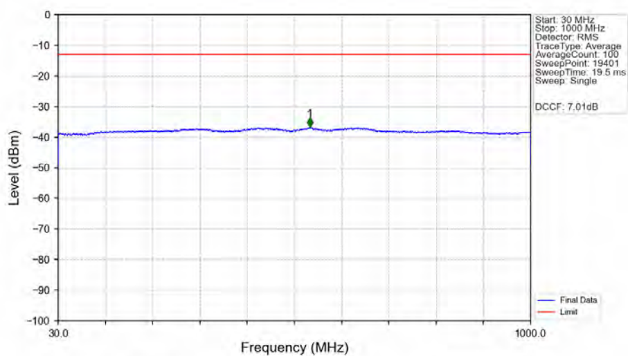
n77a_30kHz_SISO_NTNV_50MHz_DFT-s-OFDM_PI/2_BPSK_3840MHz_Edge_1RB_Left_Ant1
