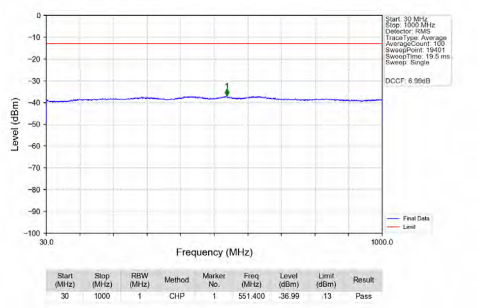
n77a_30kHz_SISO_NTNV_80MHz_CP-OFDM_QPSK_3740.01MHz_Edge_1RB_Left_Ant1
