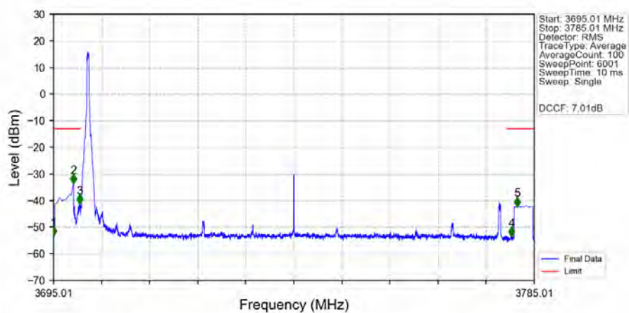
n77a_30kHz_SISO_NTNV_80MHz_DFT-s-OFDM_PI/2_BPSK_3740.01MHz_Inner_1RB_Left_Ant1
