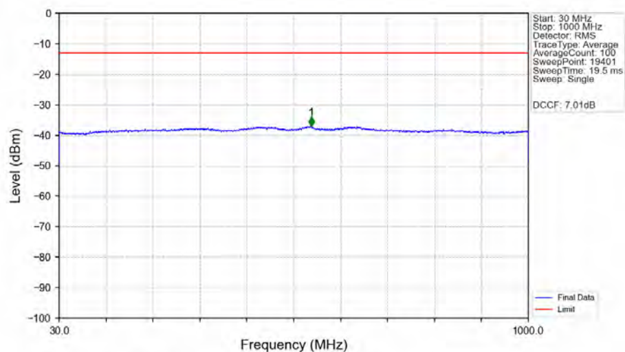
n77a_30kHz_SISO_NTNV_30MHz_DFT-s-OFDM PI/2 BPSK_3715.02MHz_Edge_1RB_Left_Ant1
