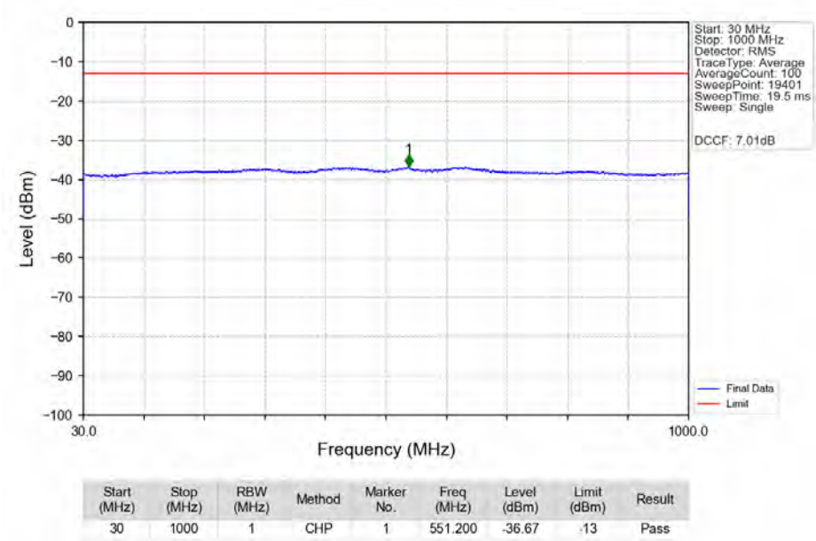
n77a_30kHz_SISO_NTNV_70MHz_CP-OFDM_QPSK_3840MHz_Edge_1RB_Left_Ant1
