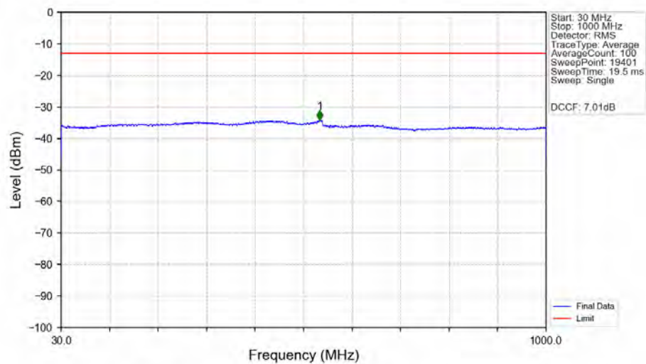
n78e_30kHz_MIMO_NTNV_90MHz_DFT-s-OFDM PI/2 BPSK_3495MHz_Edge_1RB_Left_Ant1
