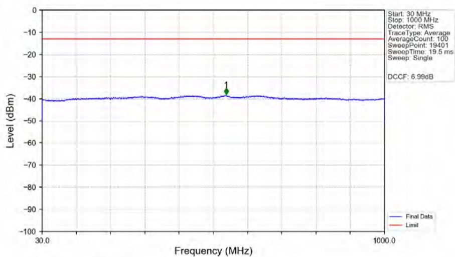
n78e_30kHz_SISO_NTNV_30MHz_DFT-s-OFDM_QPSK_3534.99MHz_Edge_1RB_Right_Ant1
