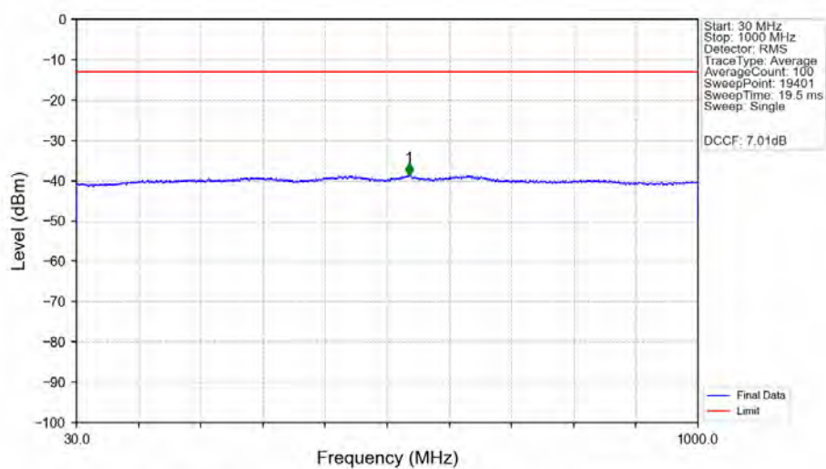
n78e_30kHz_SISO_NTNV_30MHz_DFT-s-OFDM_PI/2_BPSK_3500.01MHz_Edge_1RB_Left_Ant1
