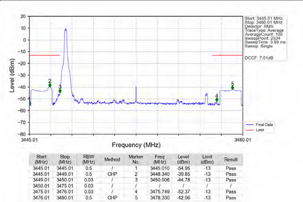
n78e_30kHz_SISO_NTNV_25MHz_CP-OFDM_QPSK_3462.51MHz_Edge_1RB_Left_Ant1
