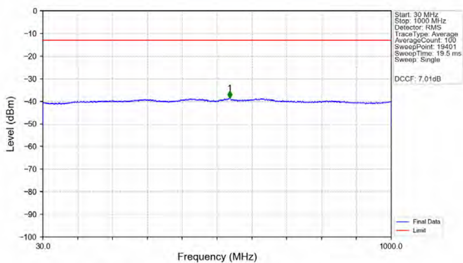
n78e_30kHz_SISO_NTNV_15MHz_DFT-s-OFDM_QPSK_3500.01MHz_Edge_1RB_Left_Ant1
