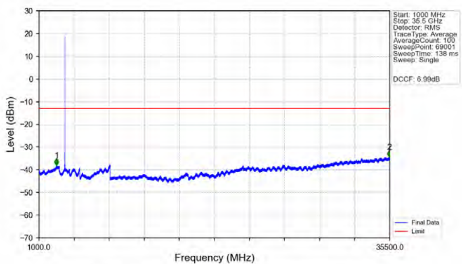
n78e_30kHz_SISO_NTNV_15MHz_CP-OFDM_QPSK_3542.49MHz_Edge_1RB_Right_Ant1
