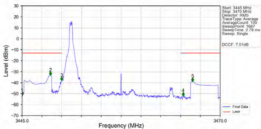
n78e_30kHz_SISO_NTNV_15MHz_DFT-s-OFDM_QPSK_3457.5MHz_Inner_1RB_Left_Ant1
