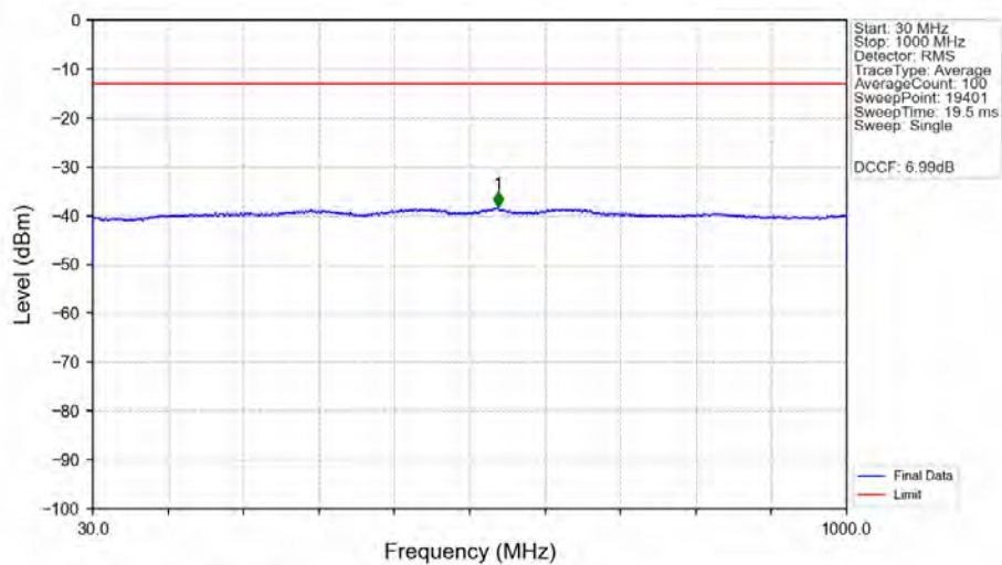
n78e_30kHz_SISO_NTNV_15MHz_CP-OFDM_QPSK_3542.49MHz_Edge_1RB_Right_Ant1
