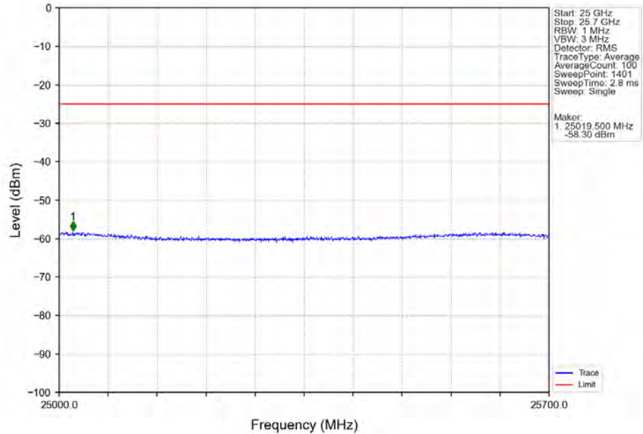
Band7_5MHz_64QAM_LCH_2502.5MHz_RB_1_0_NTNV
