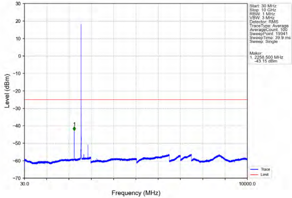
Band7_5MHz_256QAM_HCH_2567.5MHz_RB_1_0_NTNV
