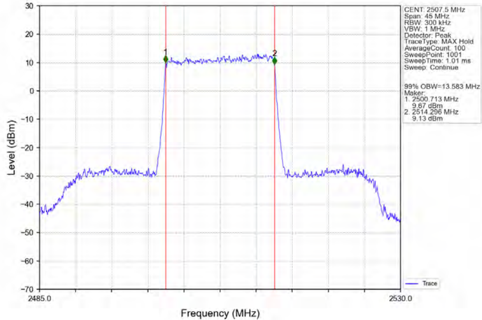
Band7_15MHz_256QAM_LCH_2507.5MHz_RB_75_0_NTNV
