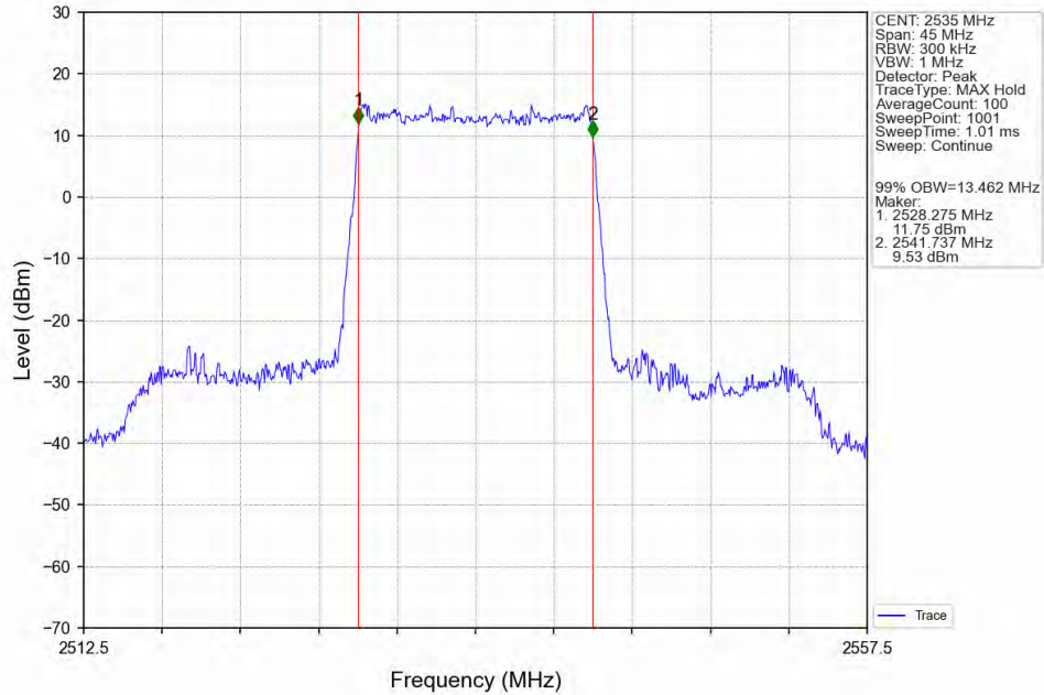
Band7_15MHz_64QAM_MCH_2535MHz_RB_75_0_NTNV
