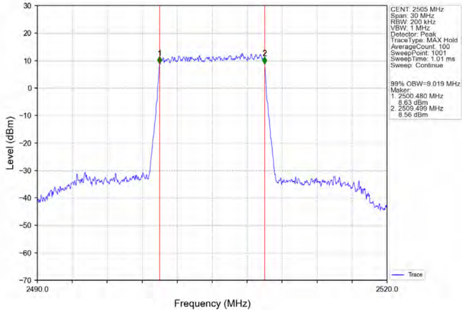
Band7_10MHz_256QAM_LCH_2505MHz_RB_50_0_NTNV
