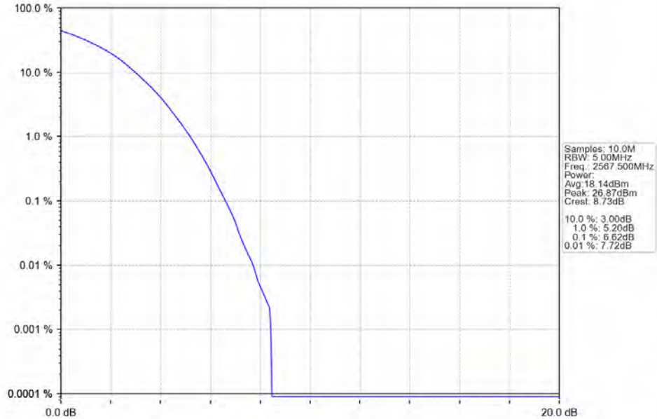
Band7_5MHz_256QAM_HCH_2567.5MHz_RB_25_0_NTNV
