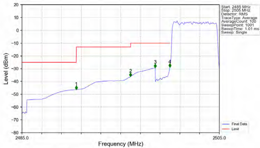
Band7_5MHz_64QAM_LCH_2502.5MHz_RB_25_0_NTNV
