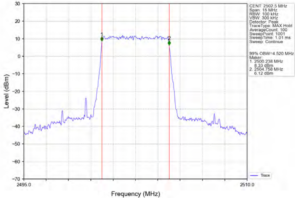
Band7_5MHz_256QAM_LCH_2502.5MHz_RB_25_0_NTNV
