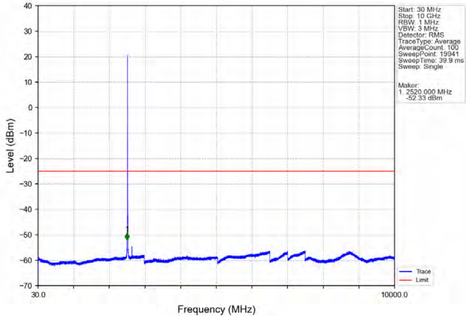
Band7_5MHz_64QAM_MCH_2535MHz_RB_1_0_NTNV
