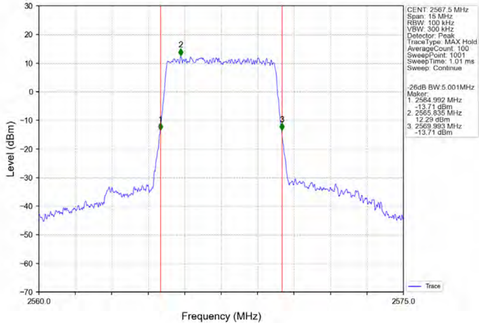
Band7_5MHz_256QAM_HCH_2567.5MHz_RB_25_0_NTNV
