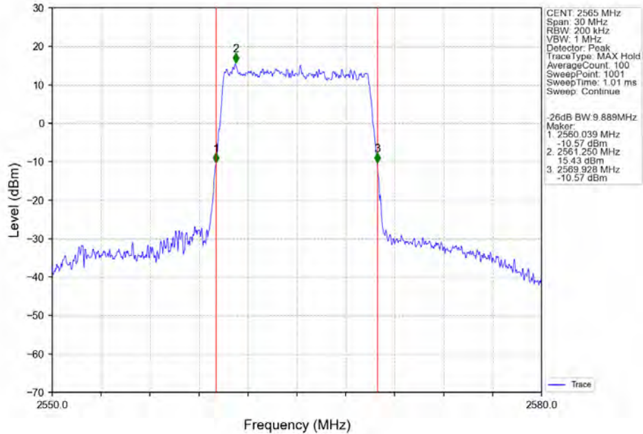
Band7_10MHz_16QAM_HCH_2565MHz_RB_50_0_NTNV
