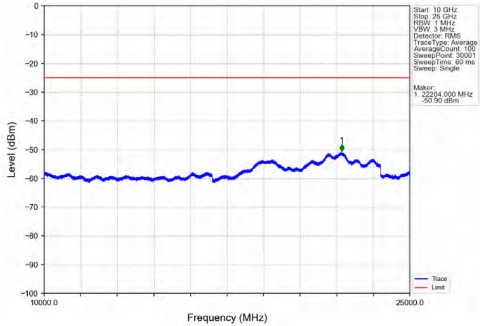
Band7_5MHz_256QAM_MCH_2535MHz_RB_1_0_NTNV
