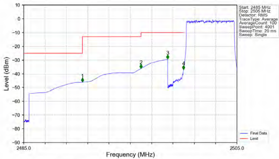
Band7 5MHz 64QAM LCH 2502.5MHz RB 1 0 NTNV
