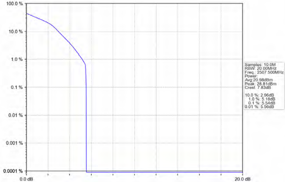
Band7_15MHz_16QAM_LCH_2507.5MHz_RB_75_0_NTNV
