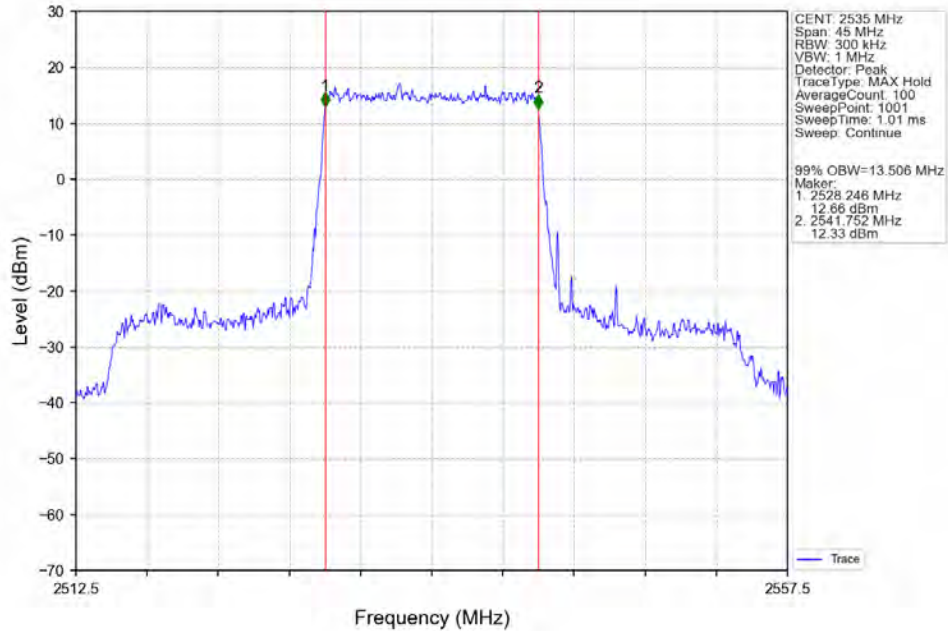
Band7_15MHz_QPSK_MCH_2535MHz_RB_75_0_NTNV
