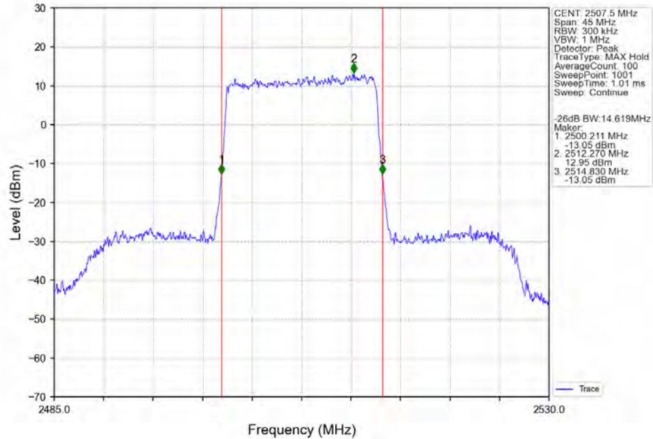
Band7_15MHz_256QAM_LCH_2507.5MHz_RB_75_0_NTNV
