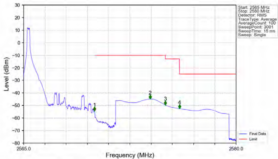
Band7_5MHz_16QAM_HCH_2567.5MHz_RB_1_24_NTNV
