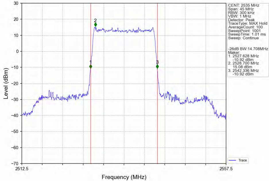
Band7_15MHz_64QAM_MCH_2535MHz_RB_75_0_NTNV
