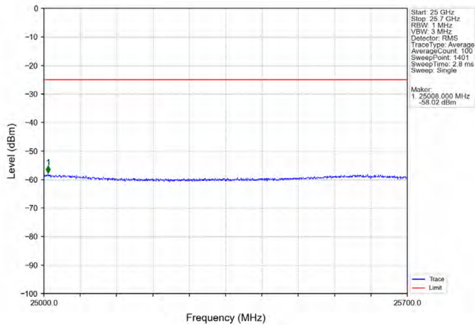
Band7_5MHz_64QAM_HCH_2567.5MHz_RB_1_24_NTNV
