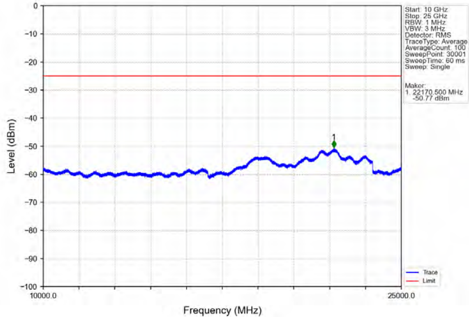
Band7_5MHz_256QAM_LCH_2502.5MHz_RB_1_0_NTNV
