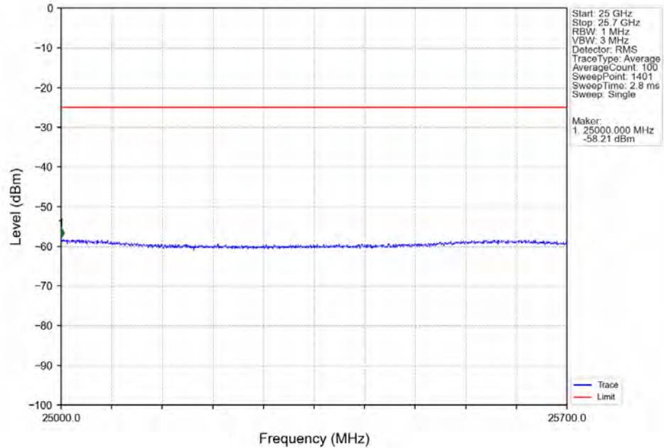
Band7_5MHz_16QAM_HCH_2567.5MHz_RB_1_0_NTNV
