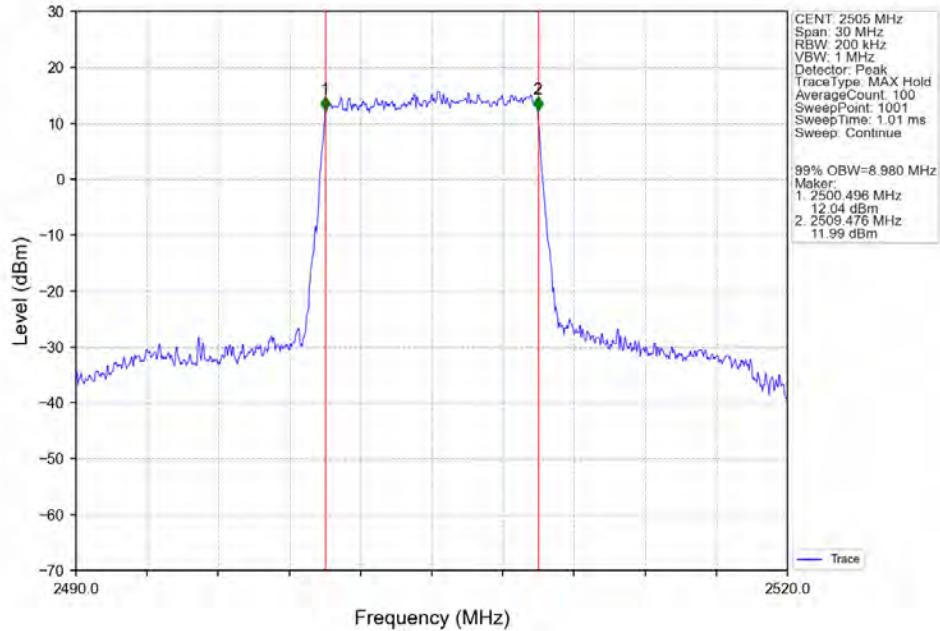
Band7_10MHz_16QAM_LCH_2505MHz_RB_50_0_NTNV
