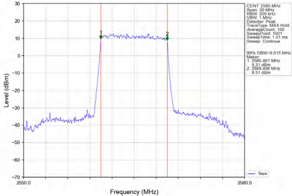
Band7_10MHz_256QAM_HCH_2565MHz_RB_50_0_NTNV
