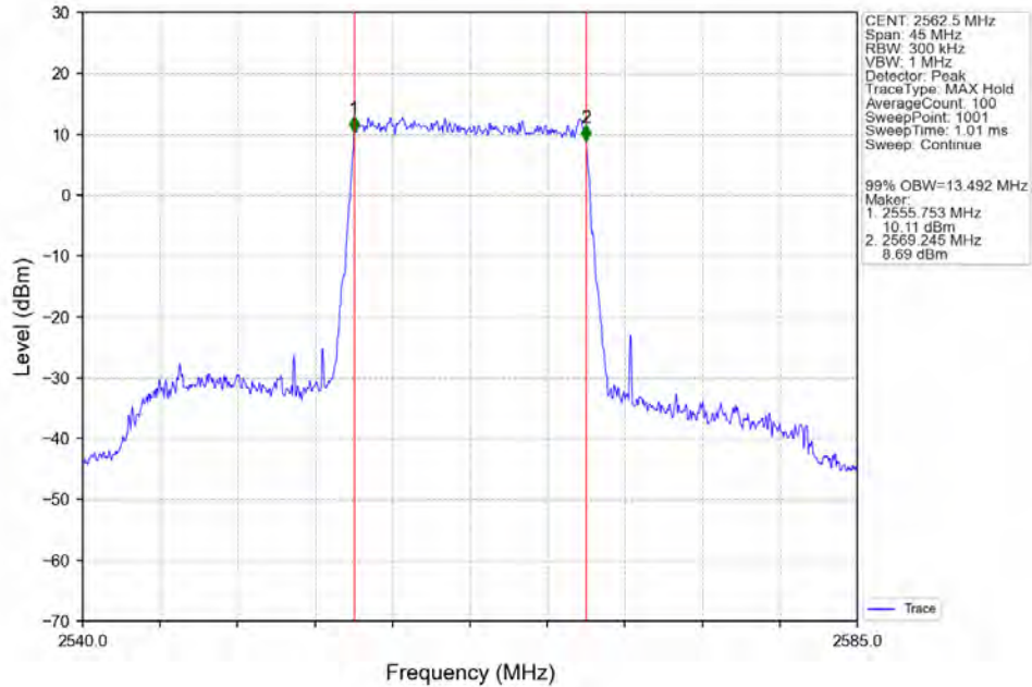
Band7_15MHz_256QAM_HCH_2562.5MHz_RB_75_0_NTNV
