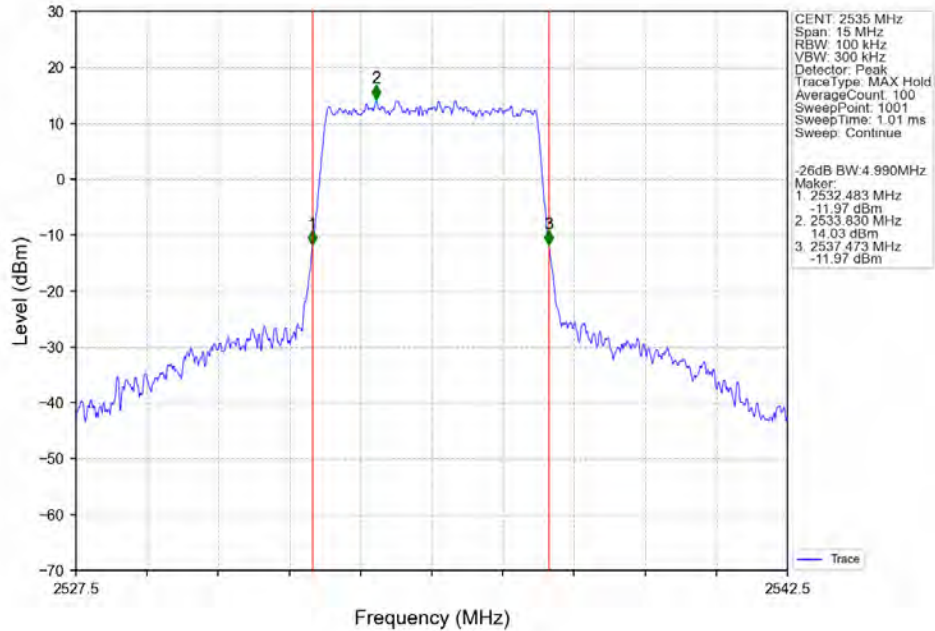
Band7_5MHz_64QAM_MCH_2535MHz_RB_25_0_NTNV
