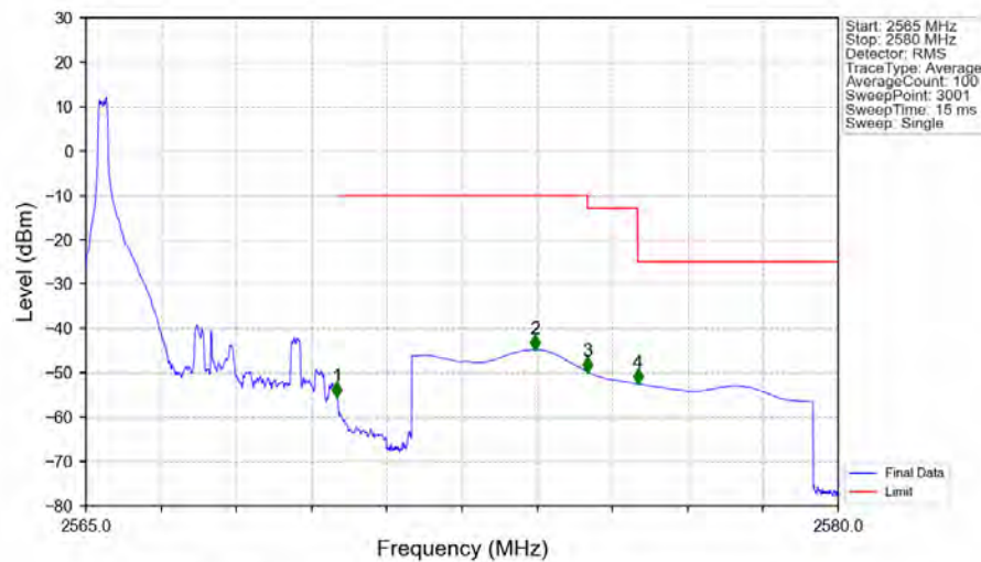
Band7_5MHz_64QAM_HCH_2567.5MHz_RB_1_24_NTNV
