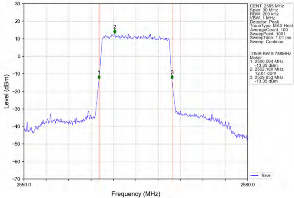
Band7_10MHz_256QAM_HCH_2565MHz_RB_50_0_NTNV
