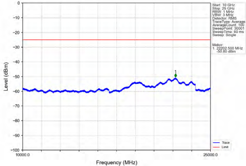
Band7_5MHz_64QAM_HCH_2567.5MHz_RB_1_0_NTNV
