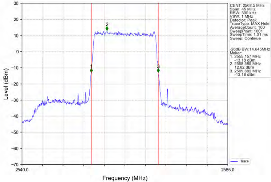
Band7_15MHz_256QAM_HCH_2562.5MHz_RB_75_0_NTNV
