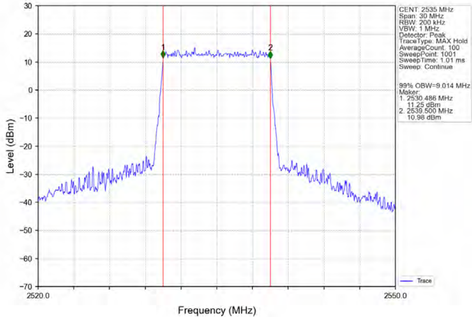
Band7_10MHz_64QAM_MCH_2535MHz_RB_50_0_NTNV
