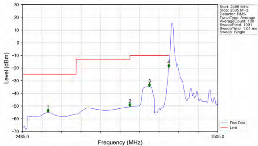
Band7_5MHz_256QAM_LCH_2502.5MHz_RB_25_0_NTNV
