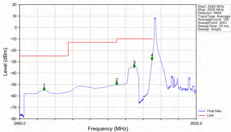
Band7_5MHz_256QAM_LCH_2502.5MHz_RB_1_0_NTNV
