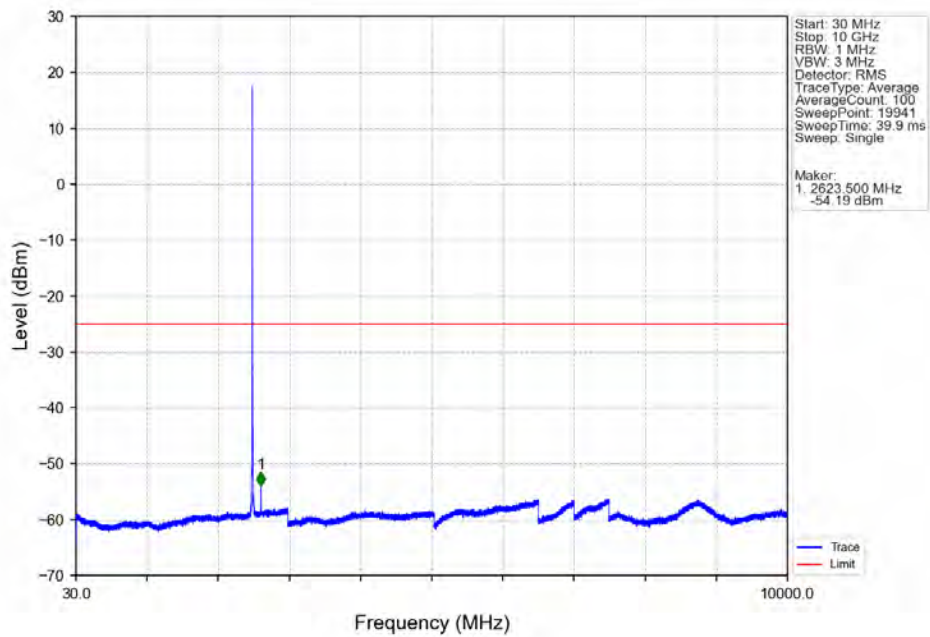
Band7_5MHz_256QAM_LCH_2502.5MHz_RB_1_0_NTNV
