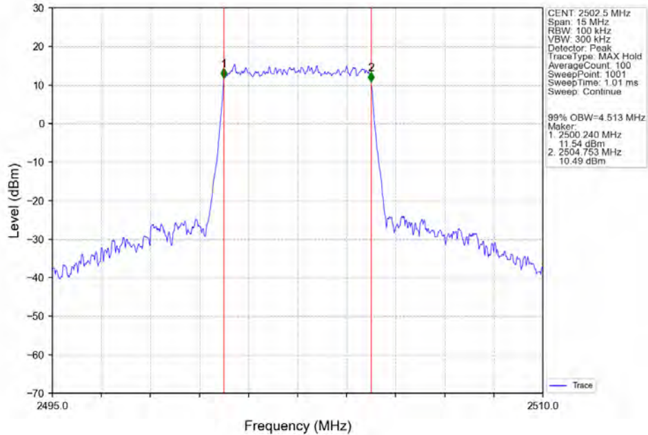
Band7_5MHz_16QAM_LCH_2502.5MHz_RB_25_0_NTNV
