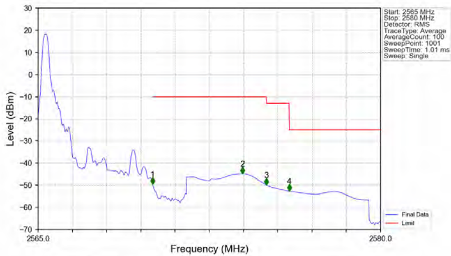
Band7_5MHz_64QAM_HCH_2567.5MHz_RB_25_0_NTNV
