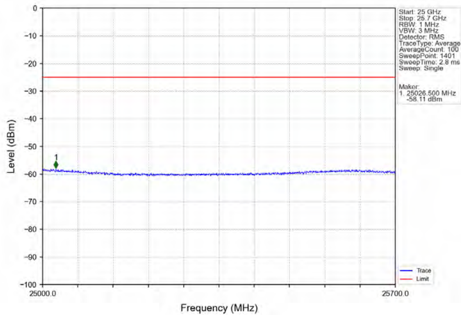
Band7_5MHz_256QAM_LCH_2502.5MHz_RB_25_0_NTNV
