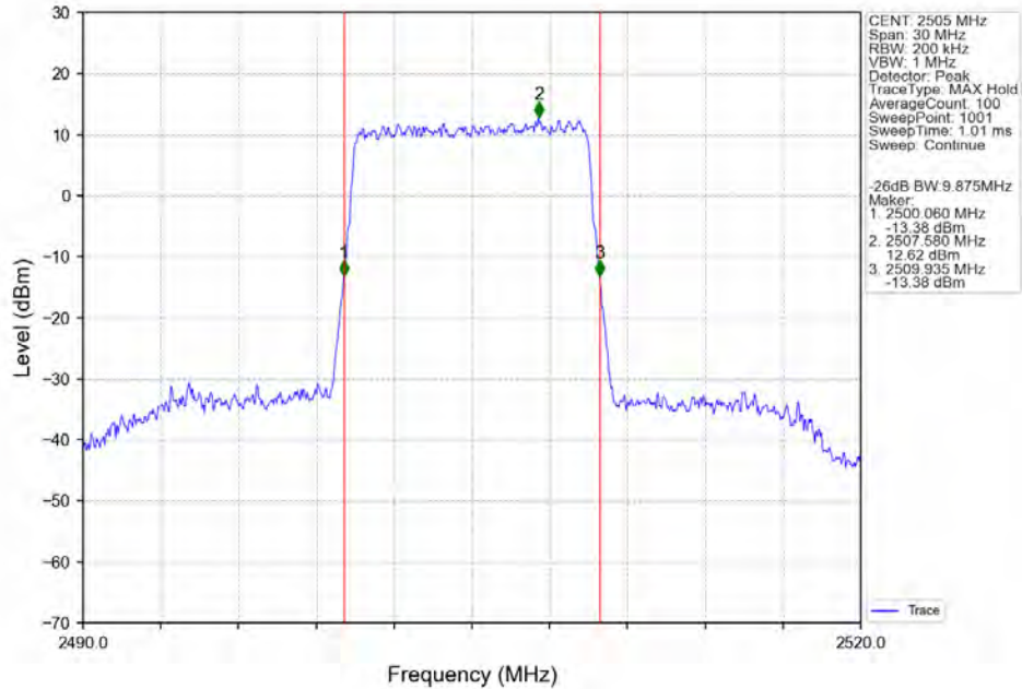
Band7_10MHz_256QAM_LCH_2505MHz_RB_50_0_NTNV
