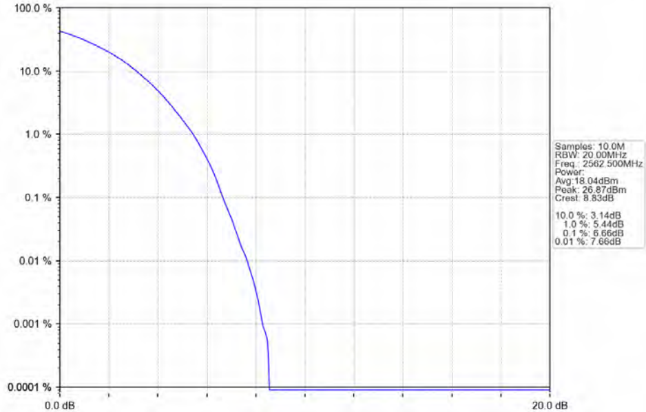
Band7_15MHz_256QAM_HCH_2562.5MHz_RB_75_0_NTNV
