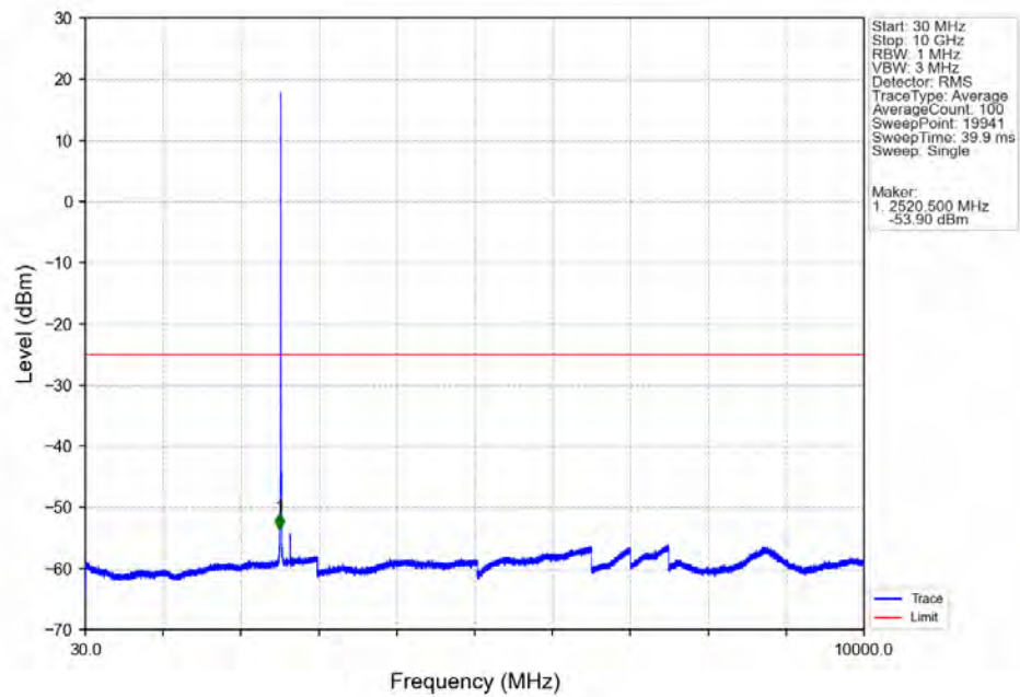
Band7_5MHz_256QAM_MCH_2535MHz_RB_1_0_NTNV
