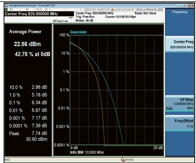
Band26(824-849)-10MHz-16QAM-26840-50RB#0-PASS
