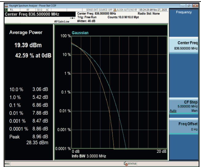
Band26(824-849)-3MHz-256QAM-26915-15RB#0-PASS
