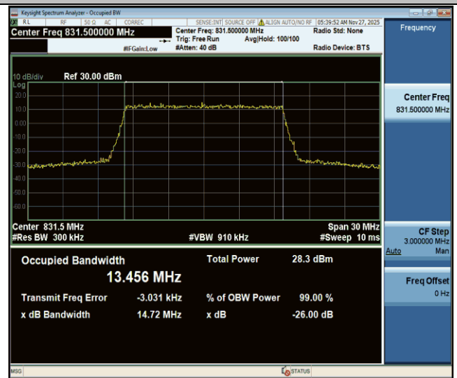
Band26(824-849)-15MHz-256QAM-26865-75RB#0-PASS
