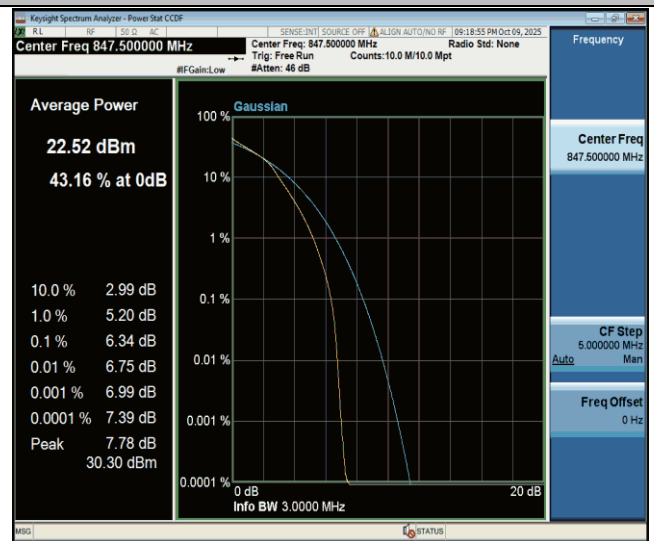
Band26(824-849)-3MHz-16QAM-27025-15RB#0-PASS
