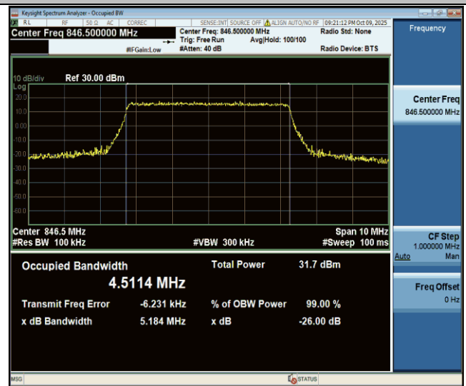
Band26(824-849)-5MHz-16QAM-27015-25RB#0-PASS
