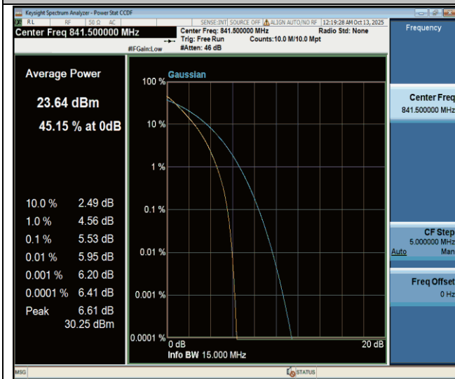
Band26(824-849)-15MHz-QPSK-26965-75RB#0-PASS
