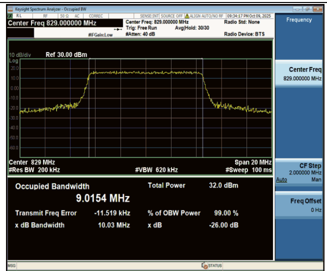
Band26(824-849)-10MHz-16QAM-26840-50RB#0-PASS
