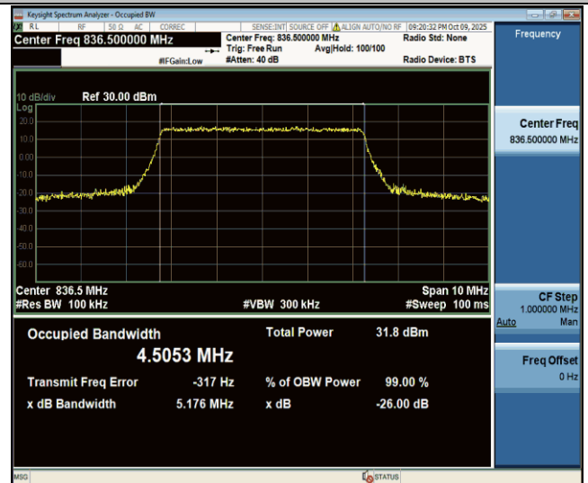
Band26(824-849)-5MHz-16QAM-26915-25RB#0-PASS
