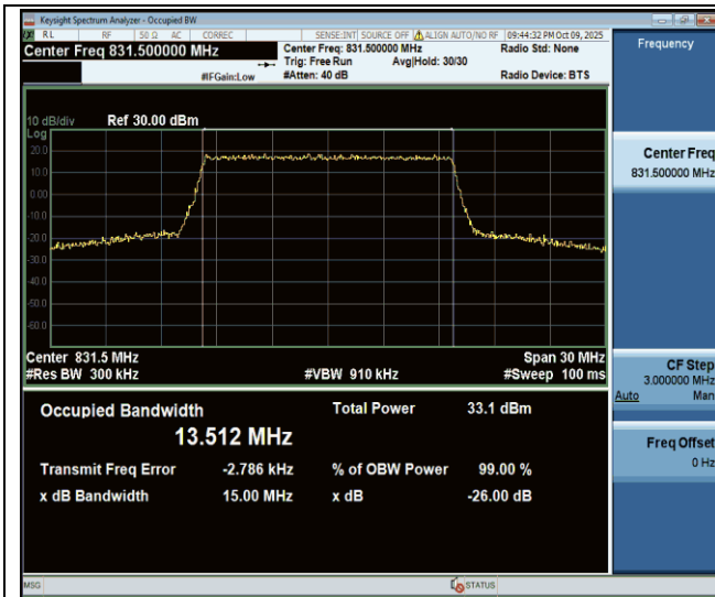
Band26(824-849)-15MHz-QPSK-26865-75RB#0-PASS
