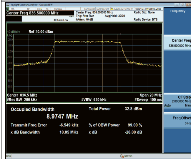
Band26(824-849)-10MHz-QPSK-26915-50RB#0-PASS
