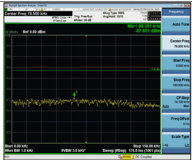
Band26(824-849)-15MHz-QPSK-26915-1RB#0-0.009~0.15-PASS
