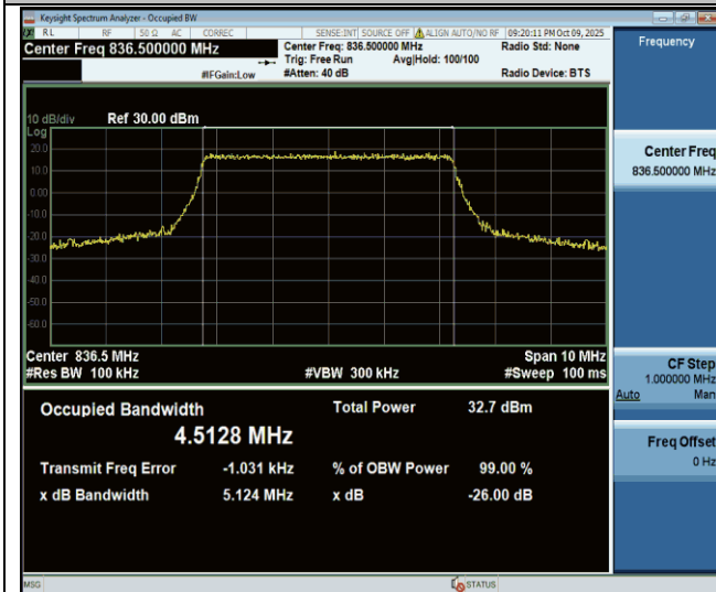
Band26(824-849)-5MHz-QPSK-26915-25RB#0-PASS
