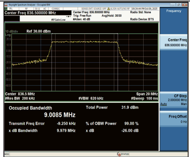
Band26(824-849)-10MHz-16QAM-26915-50RB#0-PASS
