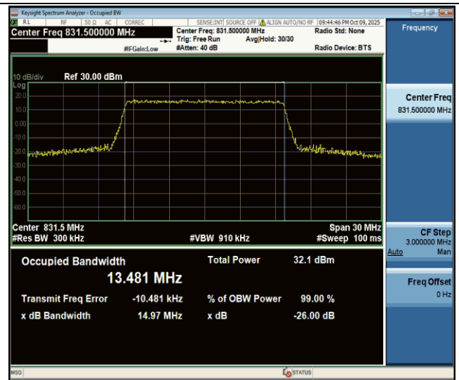
Band26(824-849)-15MHz-16QAM-26865-75RB#0-PASS
