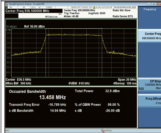
Band26(824-849)-15MHz-QPSK-26915-75RB#0-PASS
