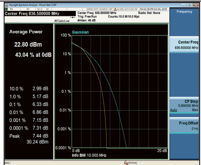
Band26(824-849)-10MHz-16QAM-26915-50RB#0-PASS
