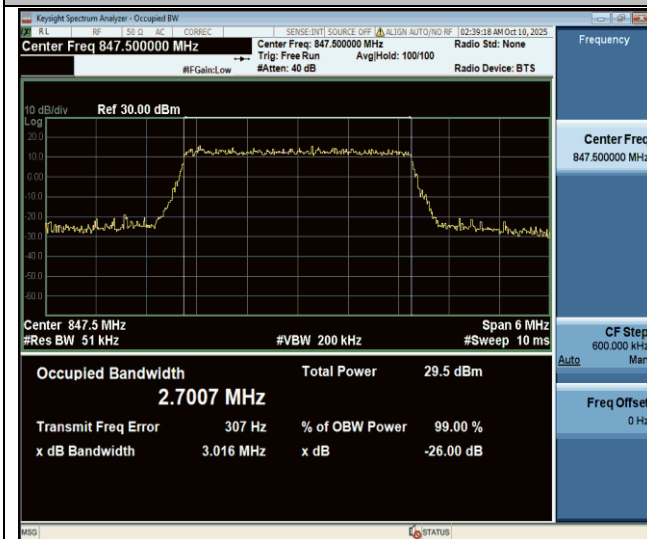
Band26(824-849)-3MHz-64QAM-27025-15RB#0-PASS
