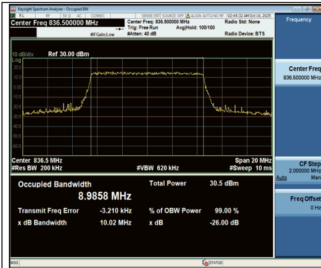
Band26(824-849)-10MHz-64QAM-26915-50RB#0-PASS
