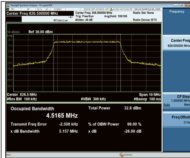
Band26(824-849)-5MHz-QPSK-26815-25RB#0-PASS
