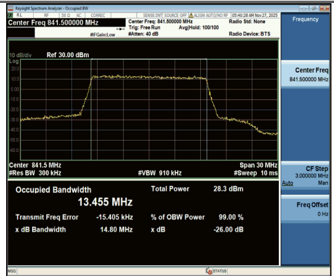
Band26(824-849)-15MHz-256QAM-26965-75RB#0-PASS
