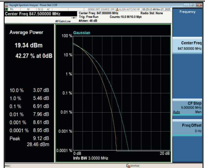
Band26(824-849)-3MHz-256QAM-27025-15RB#0-PASS
