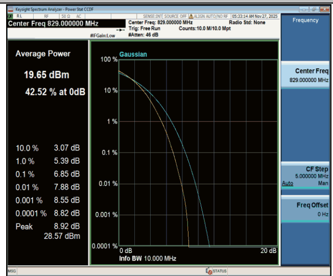
Band26(824-849)-10MHz-256QAM-26840-50RB#0-PASS
