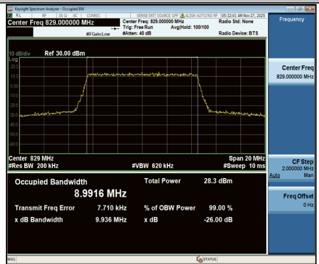
Band26(824-849)-10MHz-256QAM-26840-50RB#0-PASS
