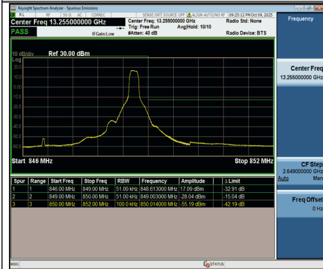
Band26(824-849)-5MHz-QPSK-27015-1RB#24-PASS
