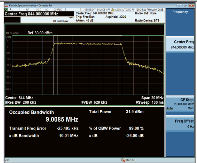
Band26(824-849)-10MHz-16QAM-26990-50RB#0-PASS
