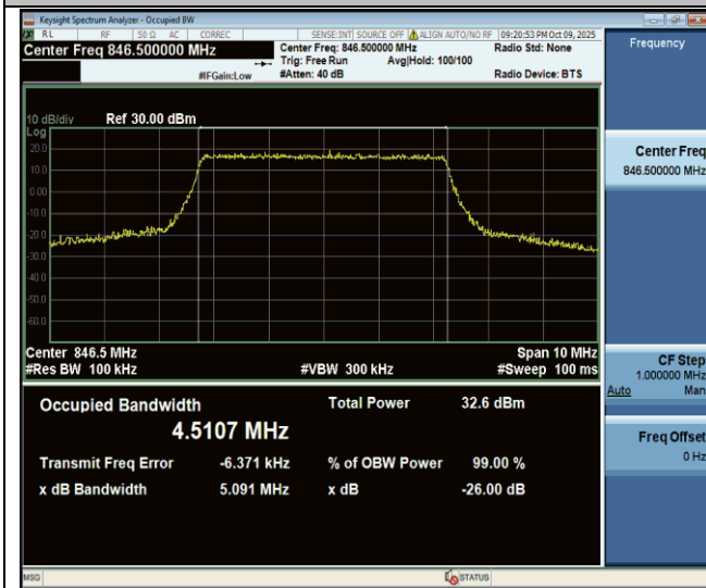
Band26(824-849)-5MHz-QPSK-27015-25RB#0-PASS
