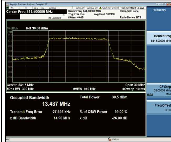
Band26(824-849)-15MHz-64QAM-26965-75RB#0-PASS
