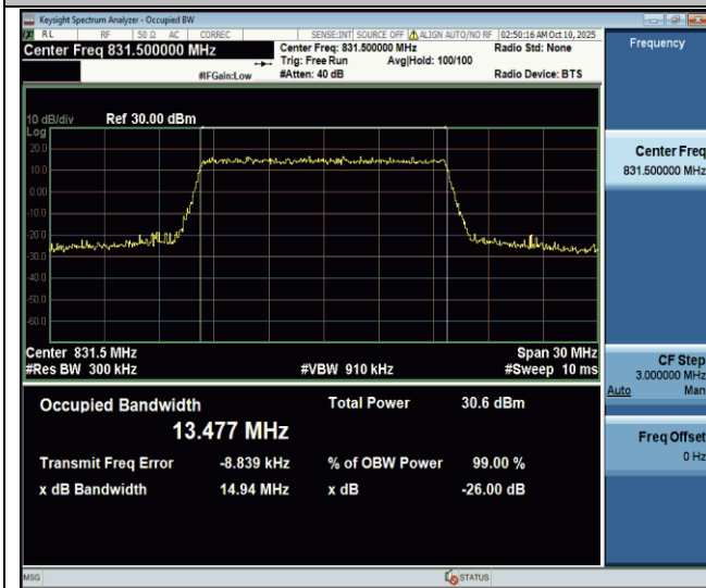
Band26(824-849)-15MHz-64QAM-26865-75RB#0-PASS
