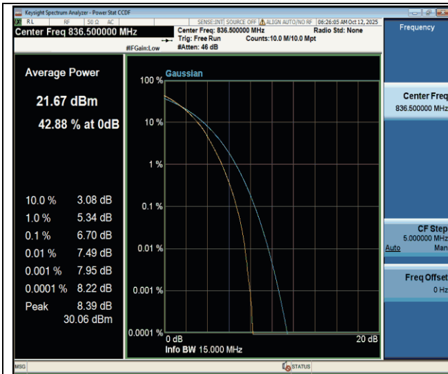
Band26(824-849)-15MHz-64QAM-26915-75RB#0-PASS
