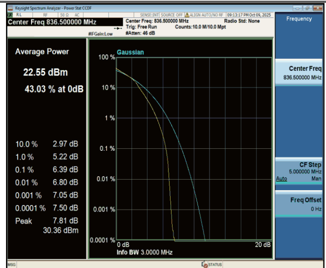
Band26(824-849)-3MHz-16QAM-26915-15RB#0-PASS
