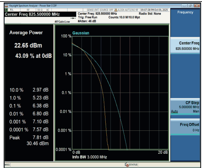
Band26(824-849)-3MHz-16QAM-26805-15RB#0-PASS
