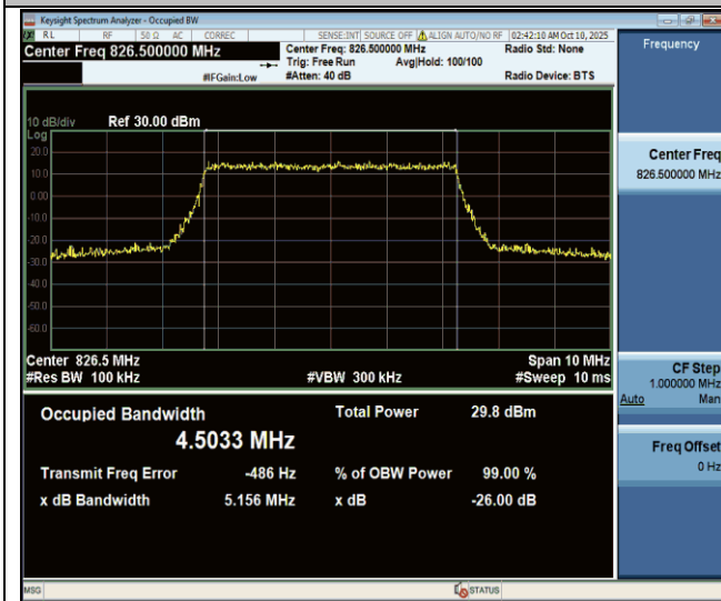
Band26(824-849)-5MHz-64QAM-26815-25RB#0-PASS
