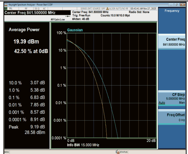
Band26(824-849)-15MHz-256QAM-26965-75RB#0-PASS
