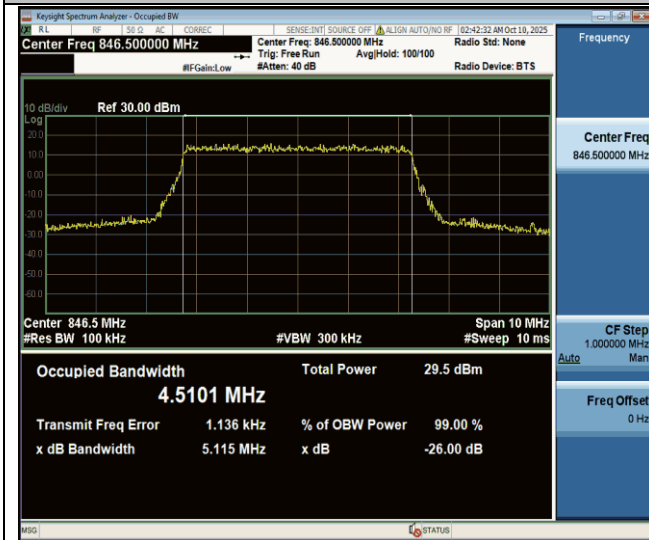
Band26(824-849)-5MHz-64QAM-27015-25RB#0-PASS
