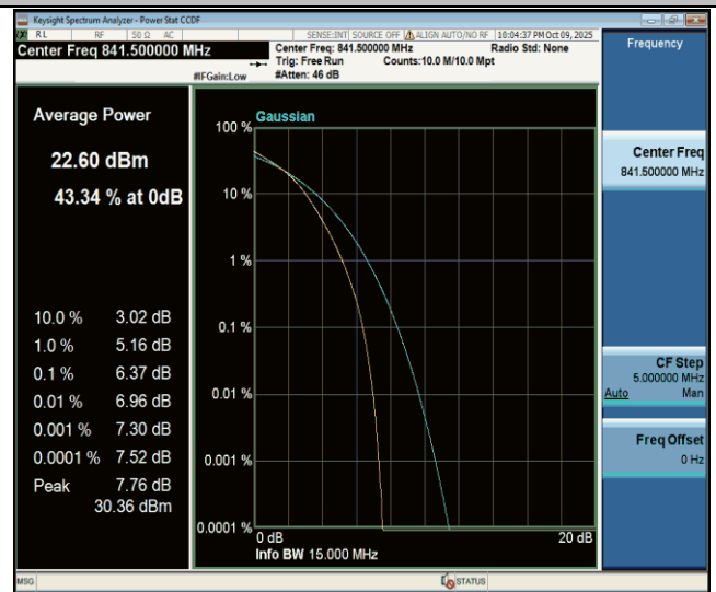
Band26(824-849)-15MHz-16QAM-26965-75RB#0-PASS
