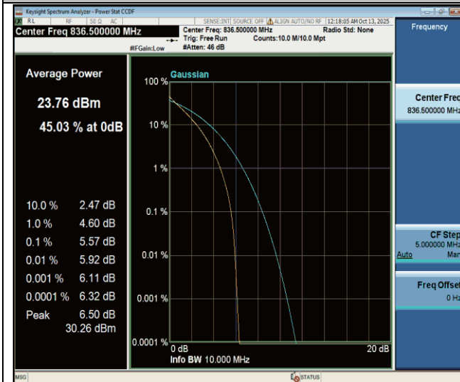
Band26(824-849)-10MHz-QPSK-26915-50RB#0-PASS
