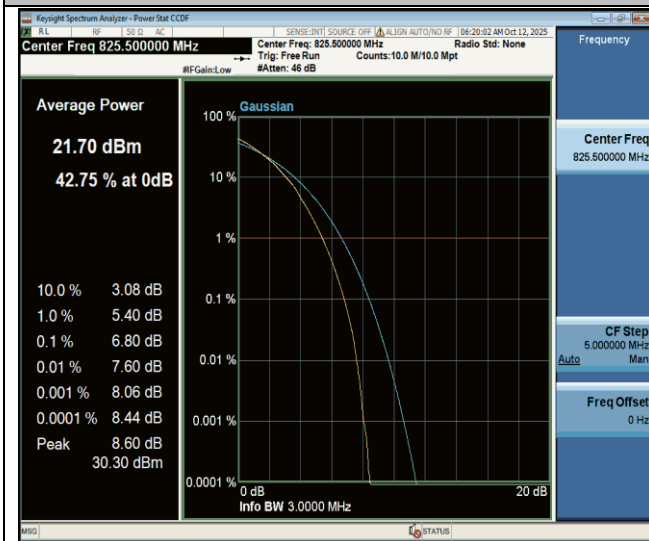
Band26(824-849)-3MHz-64QAM-26805-15RB#0-PASS
