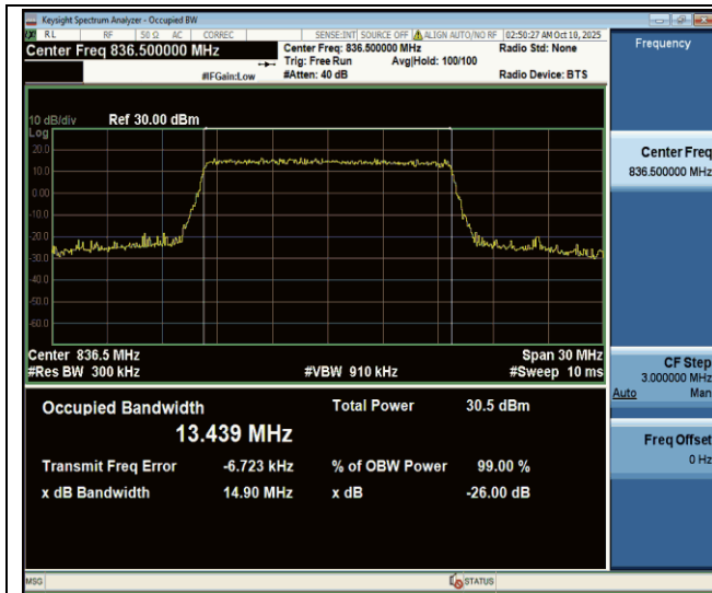
Band26(824-849)-15MHz-64QAM-26915-75RB#0-PASS
