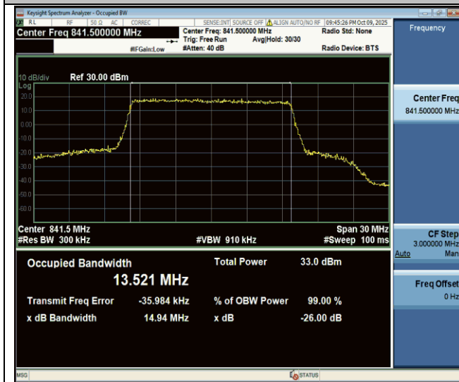
Band26(824-849)-15MHz-QPSK-26965-75RB#0-PASS
