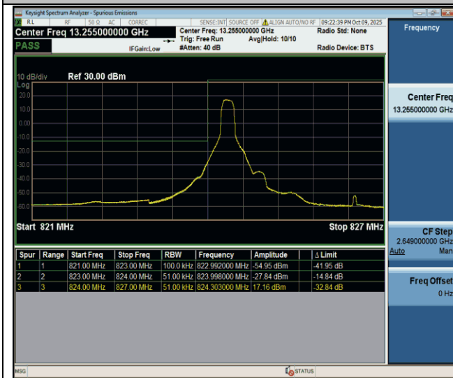
Band26(824-849)-5MHz-QPSK-26815-1RB#0-PASS
