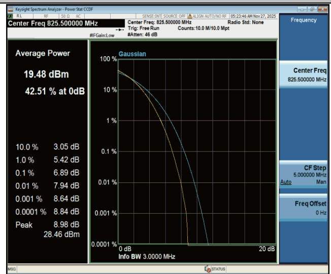
Band26(824-849)-3MHz-256QAM-26805-15RB#0-PASS
