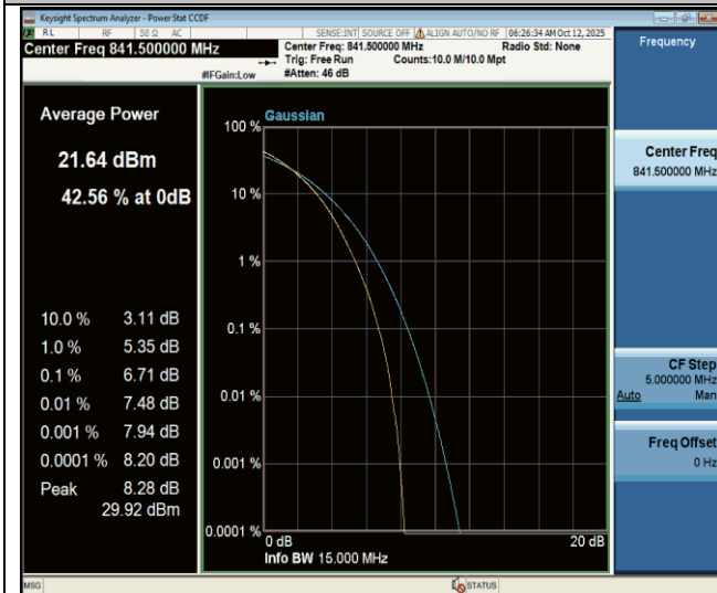
Band26(824-849)-15MHz-64QAM-26965-75RB#0-PASS
