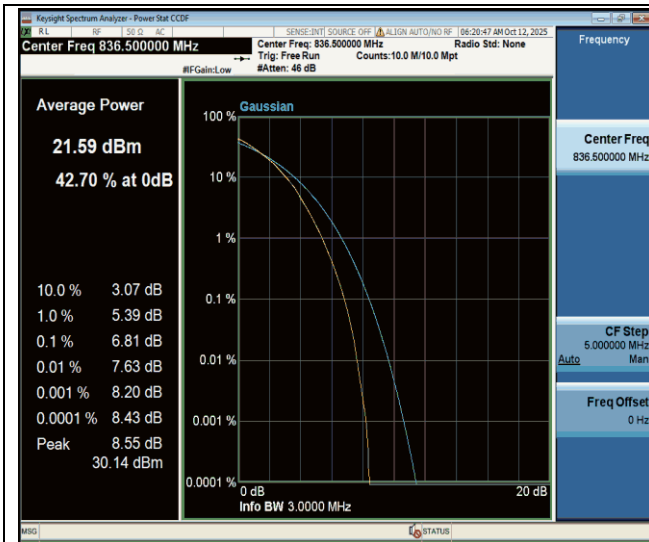
Band26(824-849)-3MHz-64QAM-26915-15RB#0-PASS
