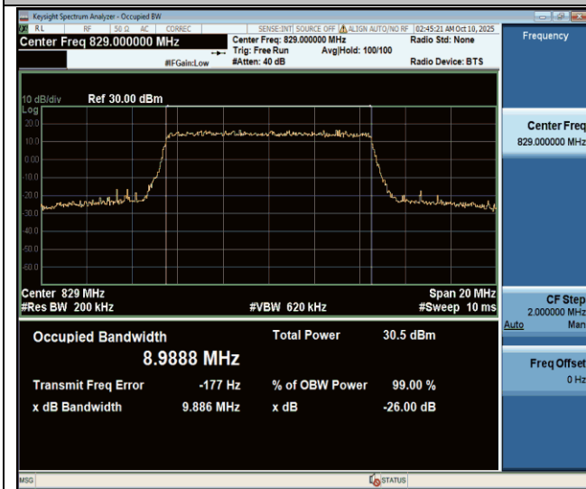
Band26(824-849)-10MHz-64QAM-26840-50RB#0-PASS
