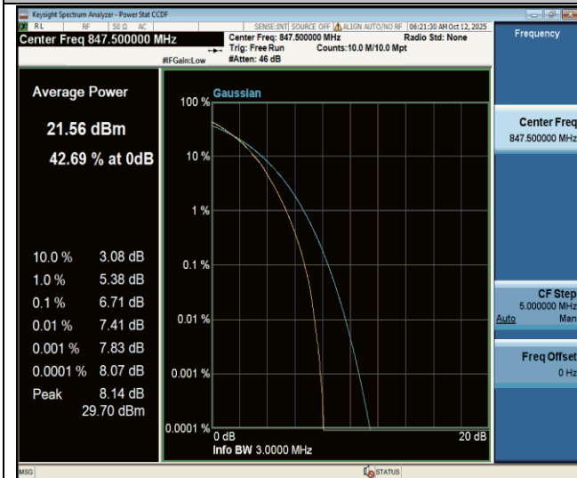
Band26(824-849)-3MHz-64QAM-27025-15RB#0-PASS
