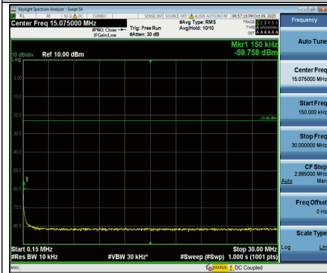
Band26(824-849)-15MHz-QPSK-26915-1RB#0-0.15~30-PASS
