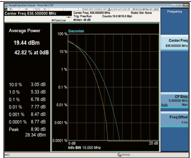
Band26(824-849)-15MHz-256QAM-26915-75RB#0-PASS
