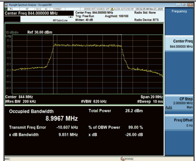
Band26(824-849)-10MHz-256QAM-26990-50RB#0-PASS
