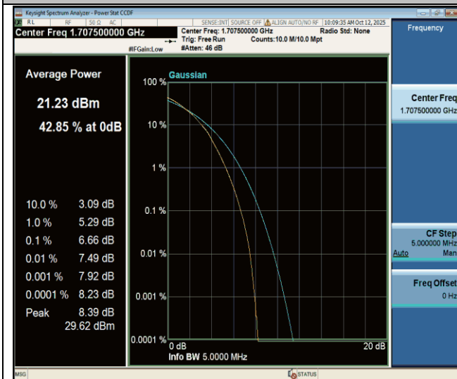
Band70-5MHz-64QAM-133097-25RB#0-PASS
