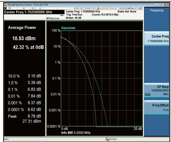
Band70-5MHz-256QAM-133047-25RB#0-PASS
