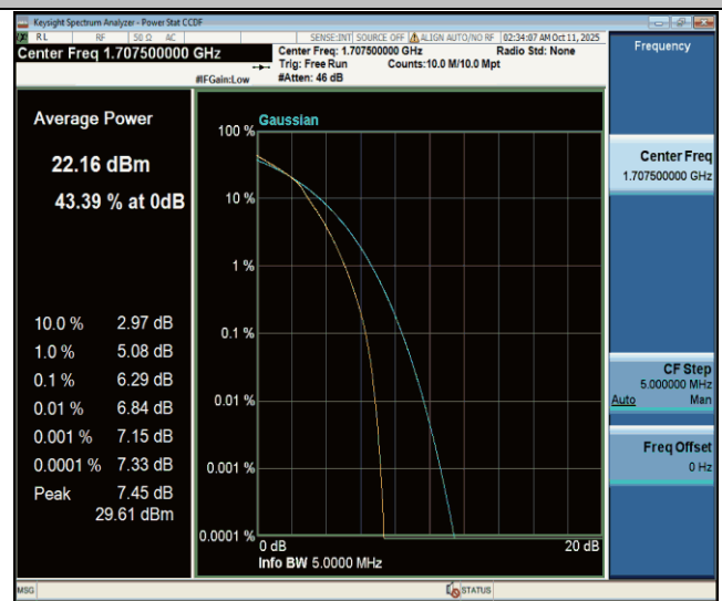
Band70-5MHz-16QAM-133097-25RB#0-PASS
