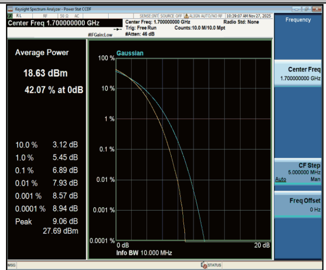
Band70-10MHz-256QAM-133022-50RB#0-PASS
