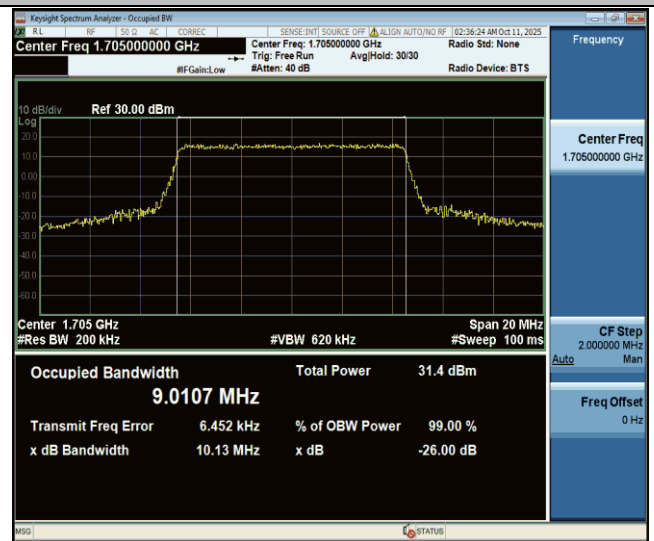
Band70-10MHz-256QAM-133072-50RB#0-PASS
