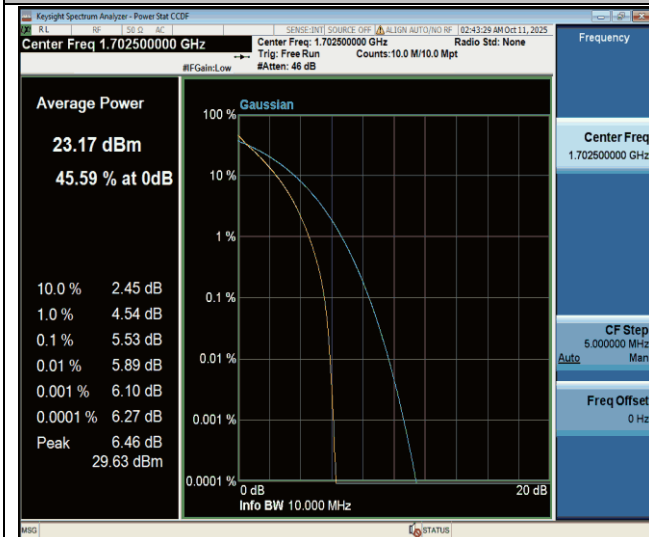
Band70-10MHz-QPSK-133047-50RB#0-PASS
