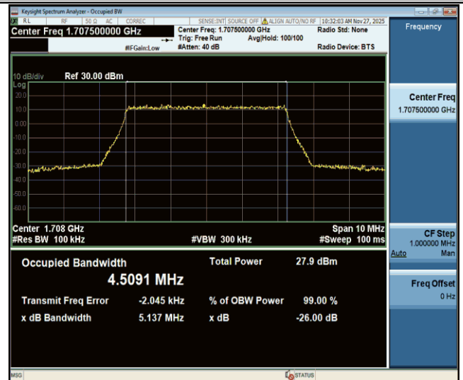
Band70-5MHz-256QAM-133097-25RB#0-PASS
