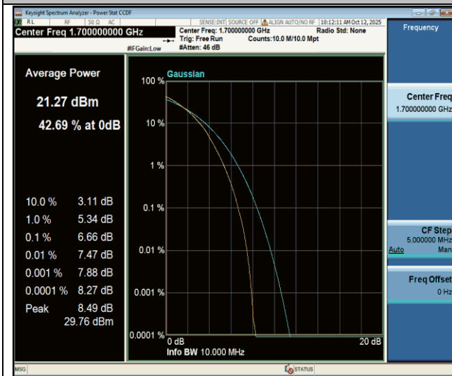
Band70-10MHz-64QAM-133022-50RB#0-PASS
