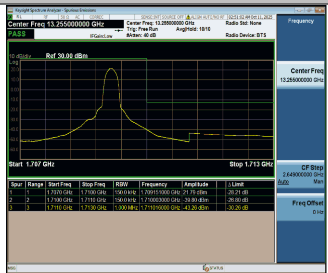
Band70-15MHz-QPSK-133047-1RB#74-PASS
