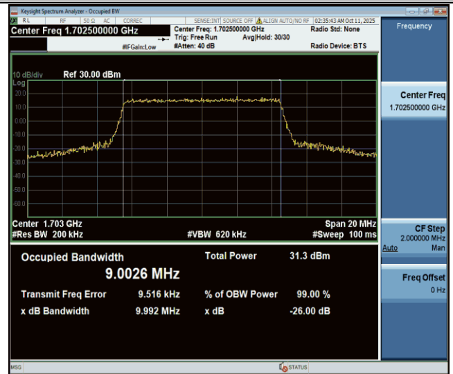
Band70-10MHz-16QAM-133047-50RB#0-PASS
