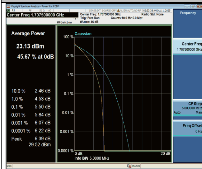
Band70-5MHz-QPSK-133097-25RB#0-PASS
