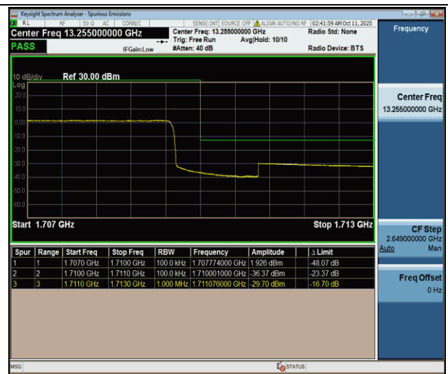
Band70-10MHz-QPSK-133072-50RB#0-PASS
