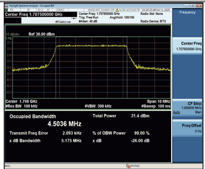
Band70-5MHz-16QAM-133097-25RB#0-PASS
