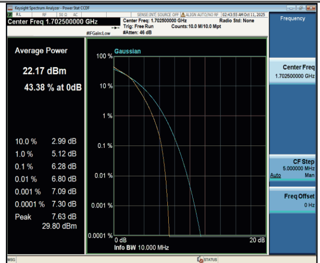
Band70-10MHz-16QAM-133047-50RB#0-PASS
