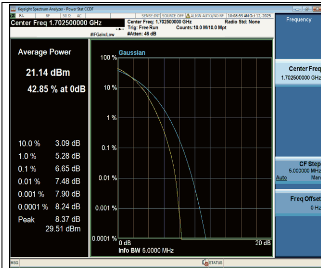
Band70-5MHz-64QAM-133047-25RB#0-PASS
