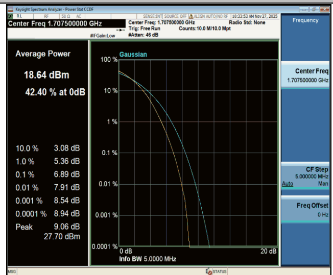
Band70-5MHz-256QAM-133097-25RB#0-PASS
