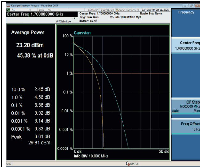
Band70-10MHz-QPSK-133022-50RB#0-PASS
