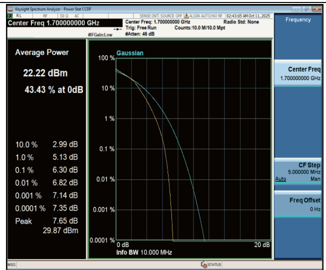
Band70-10MHz-16QAM-133022-50RB#0-PASS
