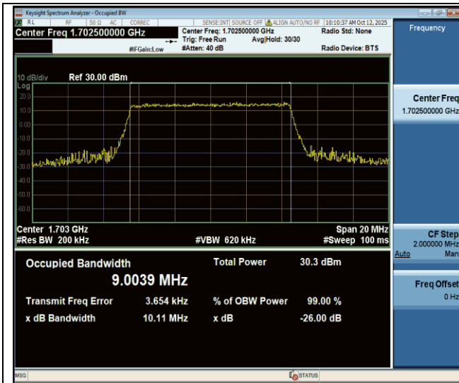
Band70-10MHz-64QAM-133047-50RB#0-PASS
