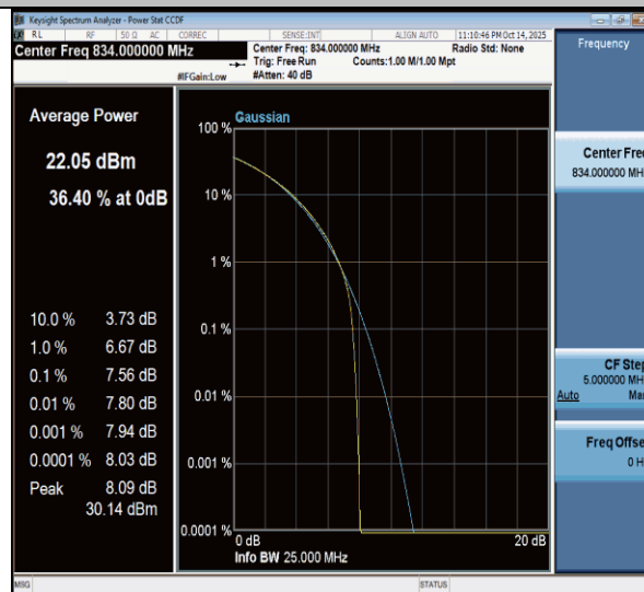
NTNV-n26(824-849)-PC3-15-20-L-CP-16QAM-Outer_Full-PASS
