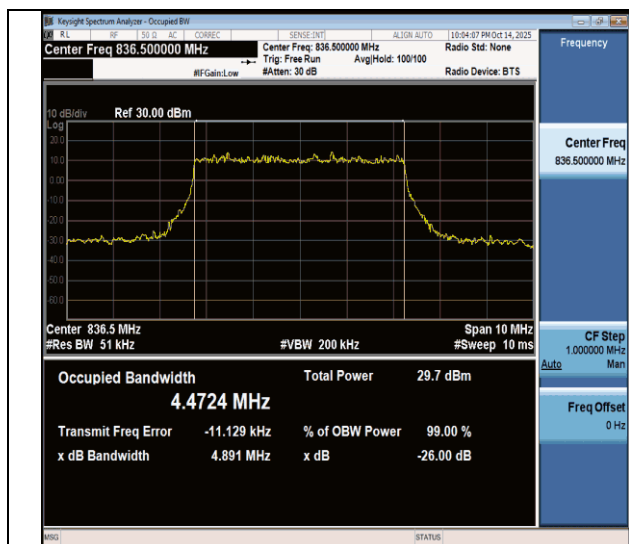
NTNV-n26(824-849)-PC3-15-5-M-DFT-QPSK-Outet_Full-Ant1- PASS
