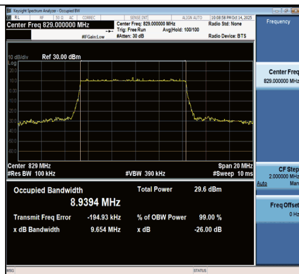
NTNV-n26(824-849)-PC3-15-10-L-DFT-16QAM-Outet_Full-Ant1- PASS
