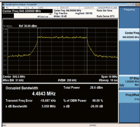
NTNV-n26(824-849)-PC3-15-5-H-DFT-16QAM-Outer_Full-Ant1- PASS
