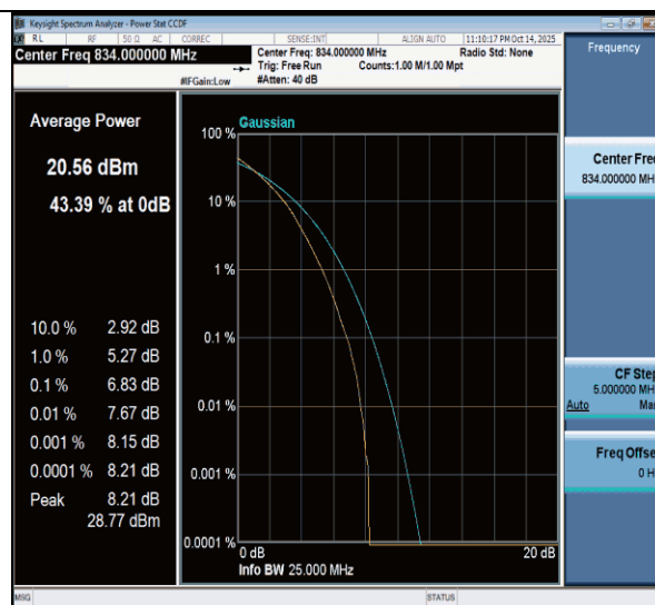
NTNV-n26(824-849)-PC3-15-20-L-DFT-256QAM-Outer_Full-PASS
