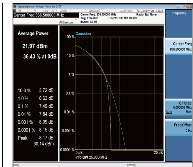
NTNV-n26(824-849)-PC3-15-20-M-CP-16QAM-Outer_Full-PASS
