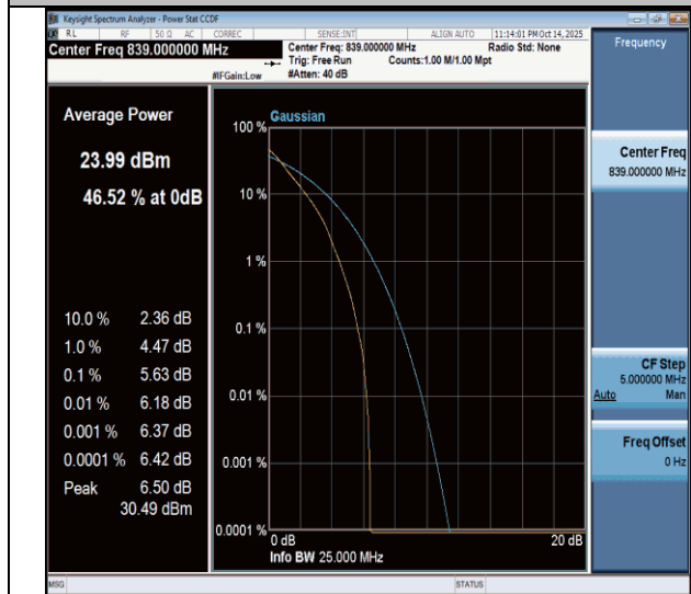
NTNV-n26(824-849)-PC3-15-20-H-DFT-QPSK-Outer_Full-PASS
