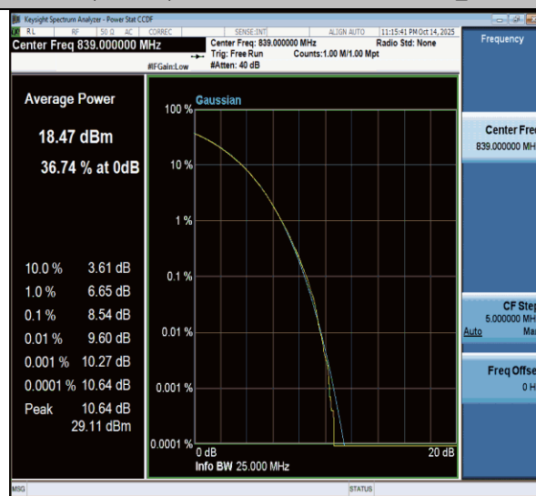
NTNV-n26(824-849)-PC3-15-20-H-CP-256QAM-Outer_Full-PASS
