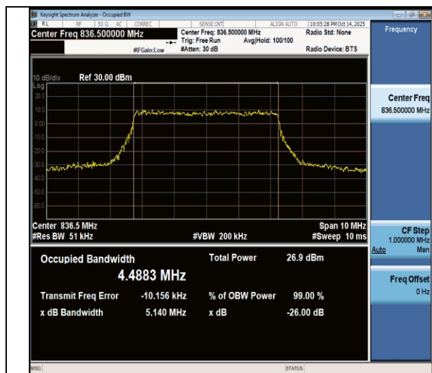
NTNV-n26(824-849)-PC3-15-5-M-CP-64QAM-Outer_Full-Ant1- PASS
