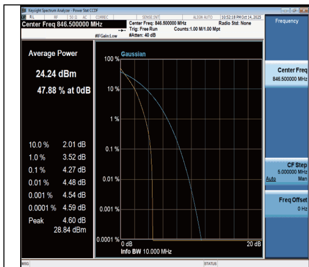
NTNV-n26(824-849)-PC3-15-5-H-DFT-BPSK-Outer_Full-PASS
