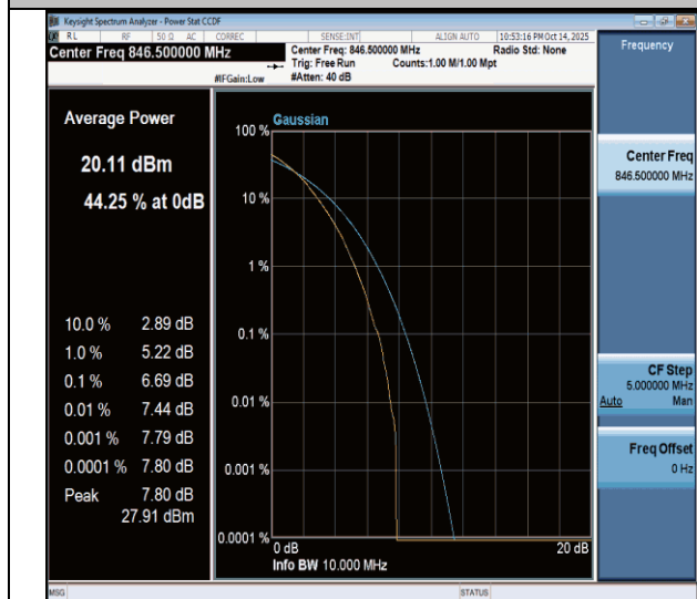
NTNV-n26(824-849)-PC3-15-5-H-DFT-256QAM-Outer_Full-PASS
