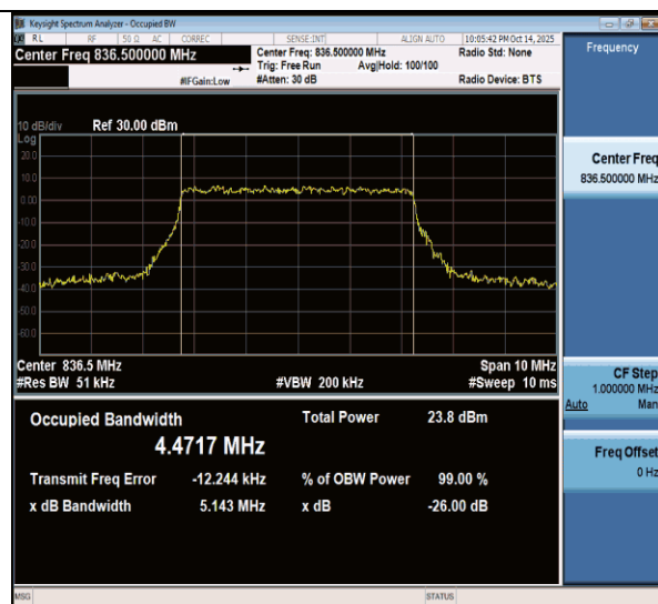
NTNV-n26(824-849)-PC3-15-5-M-CP-256QAM-Outer_Full-Ant1- PASS
