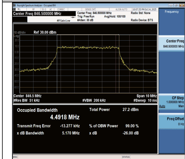
NTNV-n26(824-849)-PC3-15-5-H-CP-16QAM-Outer_Full-Ant1- PASS
