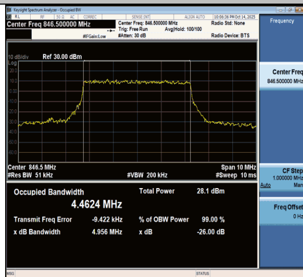
NTNV-n26(824-849)-PC3-15-5-H-DFT-64QAM-Outer_Full-Ant1- PASS
