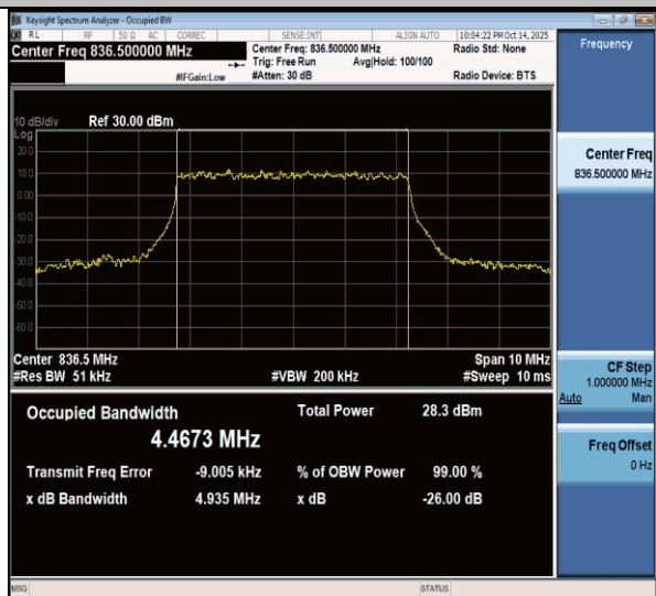
NTNV-n26(824-849)-PC3-15-5-M-DFT-64QAM-Outet_Full-Ant1- PASS
