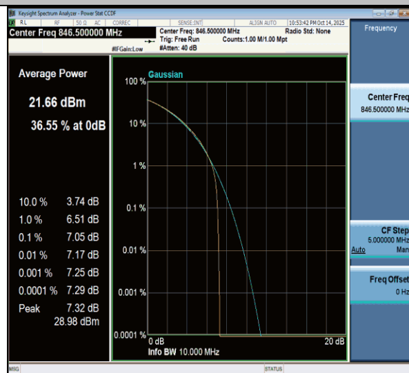
NTNV-n26(824-849)-PC3-15-5-H-CP-QPSK-Outer_Full-PASS
