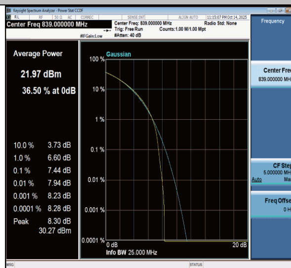
NTNV-n26(824-849)-PC3-15-20-H-CP-16QAM-Outer_Full-PASS
