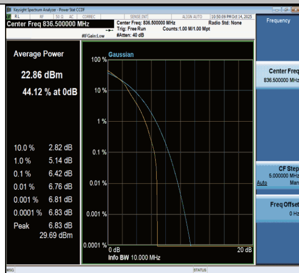
NTNV-n26(824-849)-PC3-15-5-M-DFT-16QAM-Outet_Full-PASS
