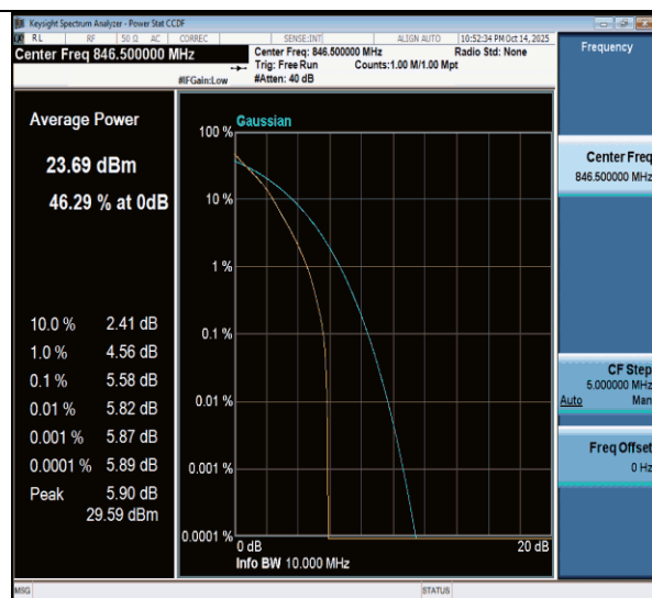
NTNV-n26(824-849)-PC3-15-5-H-DFT-QPSK-Outer_Full-PASS
