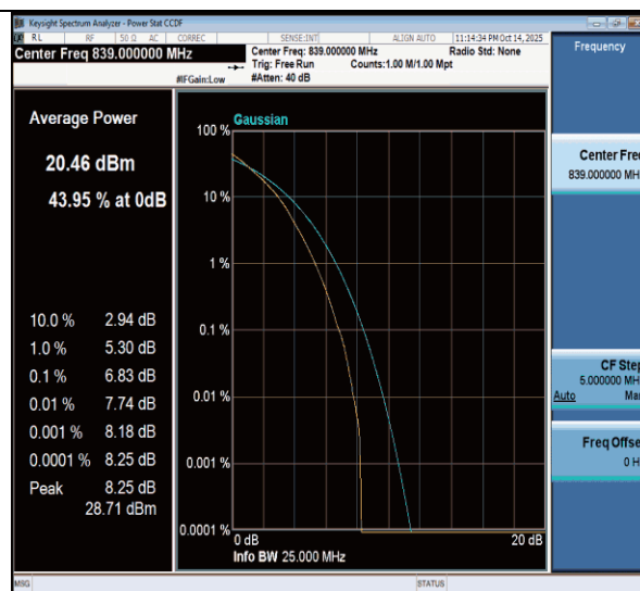
NTNV-n26(824-849)-PC3-15-20-H-DFT-256QAM-Outer_Full-PASS
