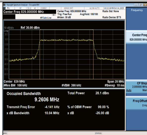
NTNV-n26(824-849)-PC3-15-10-L-CP-16QAM-Outet_Full-Ant1- PASS
