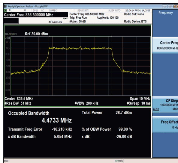
NTNV-n26(824-849)-PC3-15-5-M-DFT-16QAM-Outet_Full-Ant1- PASS
