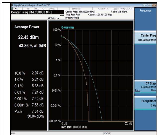
NTNV-n26(824-849)-PC3-15-10-H-DFT-64QAM-Outer_Full-PASS
