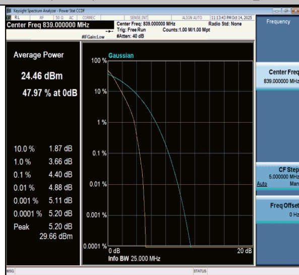
NTNV-n26(824-849)-PC3-15-20-H-DFT-BPSK-Outer_Full-PASS
