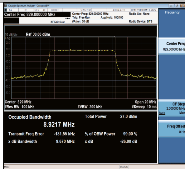
NTNV-n26(824-849)-PC3-15-10-L-DFT-256QAM-Outet_Full-Ant1- PASS
