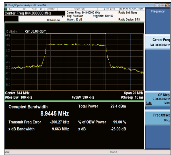
NTNV-n26(824-849)-PC3-15-10-H-DFT-16QAM-Outet_Full-Ant1- PASS
