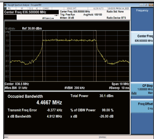
NTNV-n26(824-849)-PC3-15-5-M-DFT-BPSK-Outet_Full-Ant1- PASS
