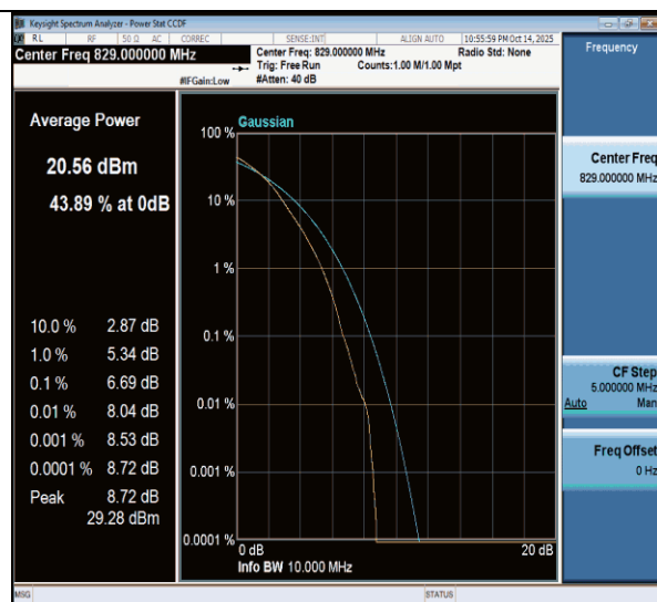
NTNV-n26(824-849)-PC3-15-10-L-DFT-256QAM-Outer_Full-PASS
