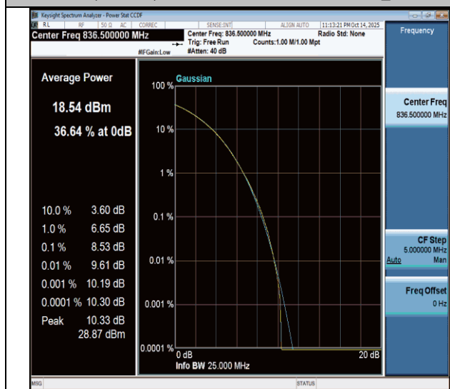
NTNV-n26(824-849)-PC3-15-20-M-CP-256QAM-Outer_Full-PASS
