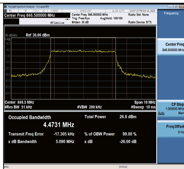
NTNV-n26(824-849)-PC3-15-5-H-CP-QPSK-Outer_Full-Ant1- PASS
