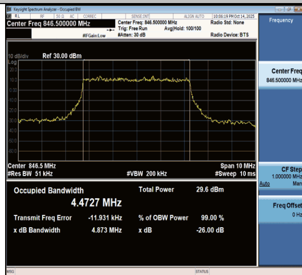
NTNV-n26(824-849)-PC3-15-5-H-DFT-QPSK-Outer_Full-Ant1- PASS
