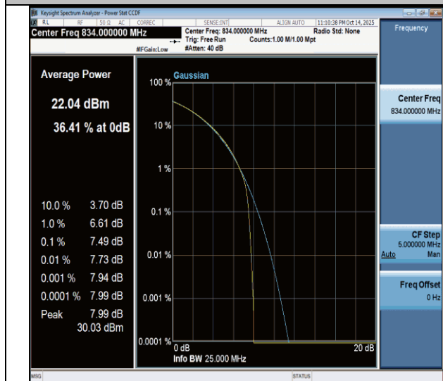
NTNV-n26(824-849)-PC3-15-20-L-CP-QPSK-Outer_Full-PASS
