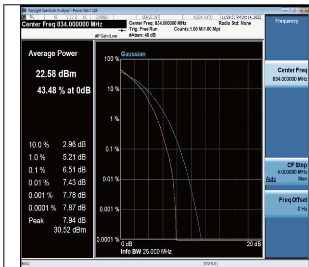
NTNV-n26(824-849)-PC3-15-20-L-DFT-64QAM-Outer_Full-PASS
