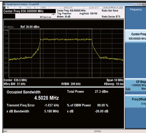
NTNV-n26(824-849)-PC3-15-5-M-CP-16QAM-Outet_Full-Ant1- PASS
