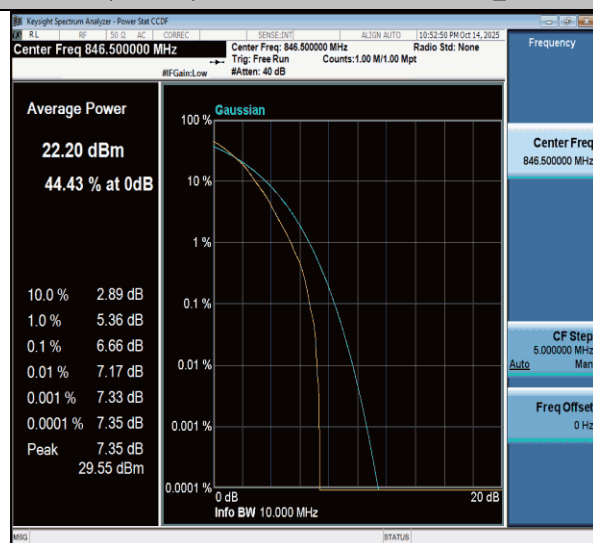
NTNV-n26(824-849)-PC3-15-5-H-DFT-64QAM-Outer_Full-PASS
