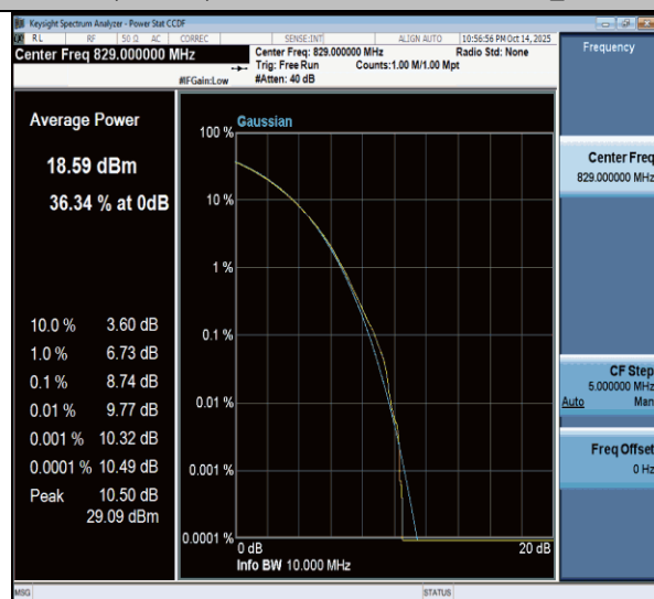
NTNV-n26(824-849)-PC3-15-10-L-CP-256QAM-Outer_Full-PASS
