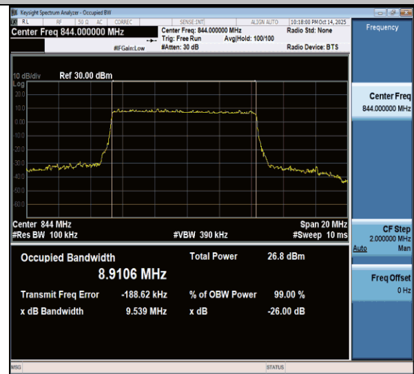
NTNV-n26(824-849)-PC3-15-10-H-DFT-256QAM-Outet_Full-Ant1-PASS
