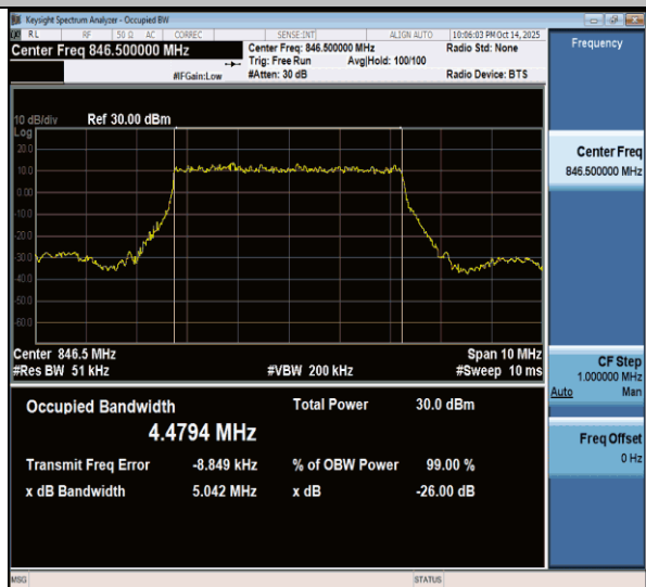
NTNV-n26(824-849)-PC3-15-5-H-DFT-BPSK-Outer_Full-Ant1- PASS
