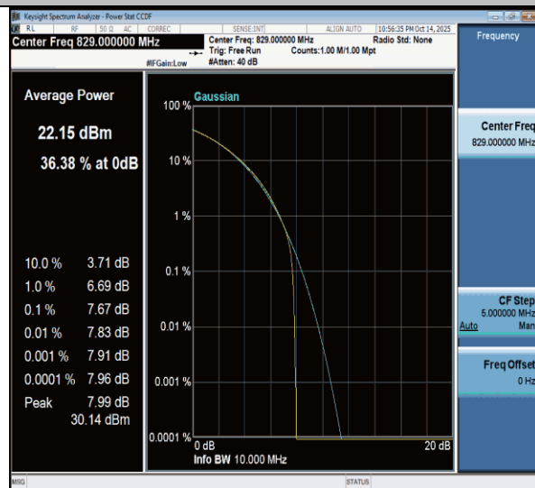
NTNV-n26(824-849)-PC3-15-10-L-CP-16QAM-Outer_Full-PASS
