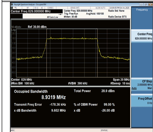
NTNV-n26(824-849)-PC3-15-10-L-DFT-64QAM-Outet_Full-Ant1- PASS
