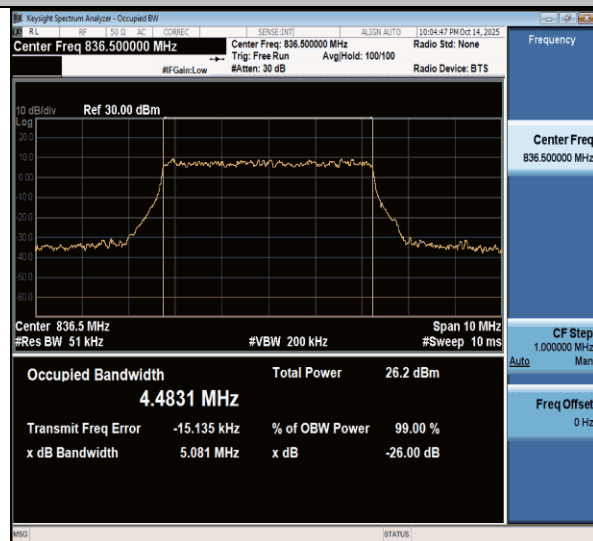
NTNV-n26(824-849)-PC3-15-5-M-DFT-256QAM-Outet_Full-Ant1- PASS
