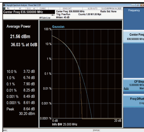
NTNV-n26(824-849)-PC3-15-20-M-CP-64QAM-Outer_Full-PASS
