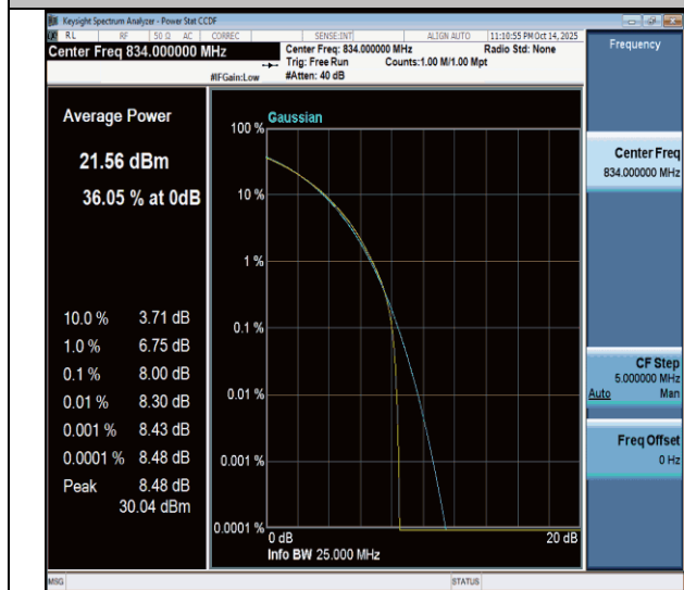
NTNV-n26(824-849)-PC3-15-20-L-CP-64QAM-Outer_Full-PASS
