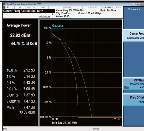
NTNV-n26(824-849)-PC3-15-20-H-DFT-16QAM-Outer_Full-PASS
