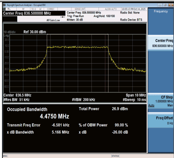
NTNV-n26(824-849)-PC3-15-5-M-CP-QPSK-Outet_Full-Ant1- PASS
