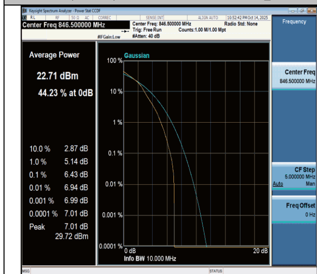
NTNV-n26(824-849)-PC3-15-5-H-DFT-16QAM-Outer_Full-PASS
