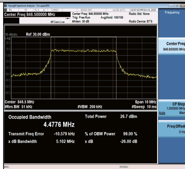
NTNV-n26(824-849)-PC3-15-5-H-CP-64QAM-Outer_Full-Ant1- PASS
