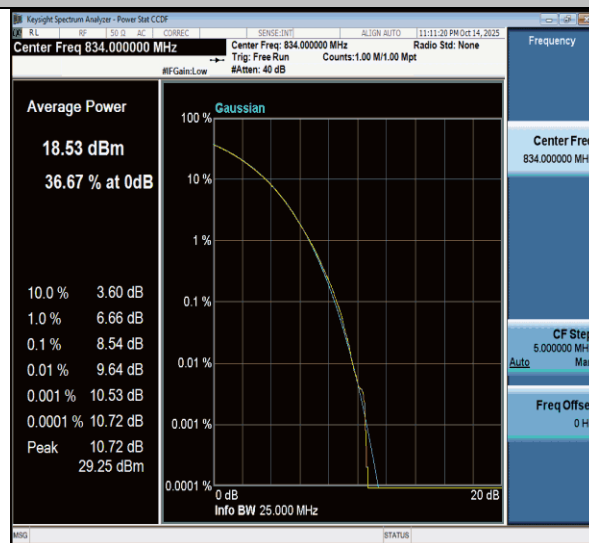
NTNV-n26(824-849)-PC3-15-20-L-CP-256QAM-Outer_Full-PASS
