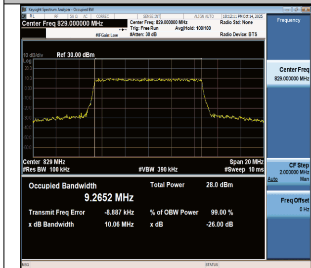
NTNV-n26(824-849)-PC3-15-10-L-CP-QPSK-Outet_Full-Ant1- PASS
