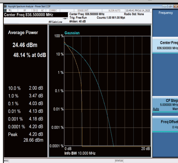
NTNV-n26(824-849)-PC3-15-5-M-DFT-BPSK-Outet_Full-PASS
