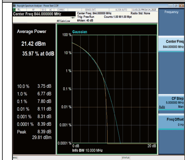
NTNV-n26(824-849)-PC3-15-10-H-CP-64QAM-Outer_Full-PASS
