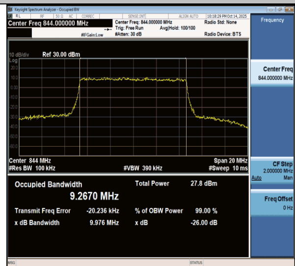
NTNV-n26(824-849)-PC3-15-10-H-CP-16QAM-Outet_Full-Ant1- PASS
