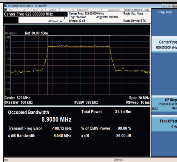
NTNV-n26(824-849)-PC3-15-10-L-DFT-BPSK-Outer_Full-Ant1- PASS
