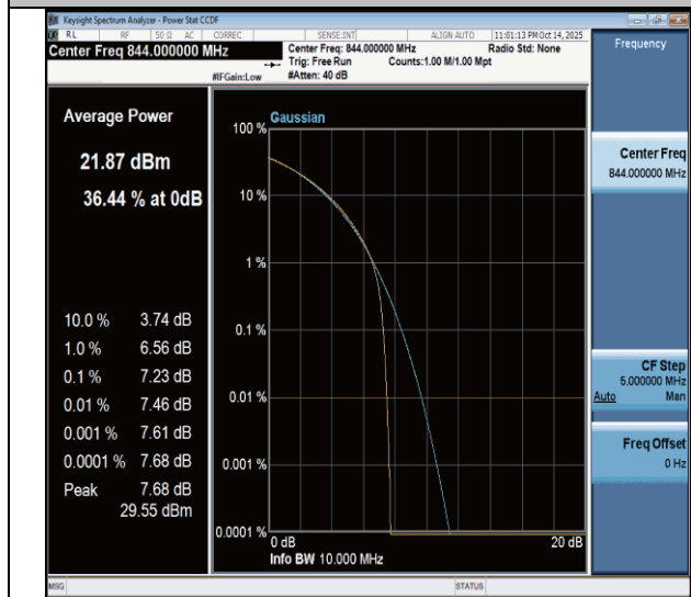
NTNV-n26(824-849)-PC3-15-10-H-CP-QPSK-Outer_Full-PASS
