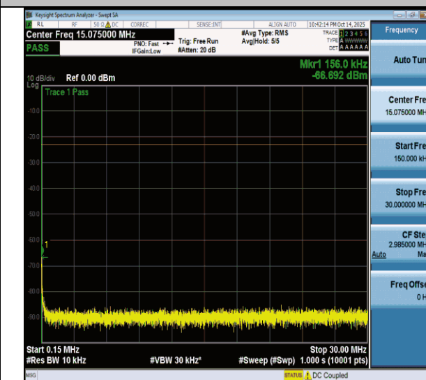
NTNV-n26(824-849)-PC3-15-20-M-DFT-BPSK-Edge_1RB_Left- 0.15-30-PASS
