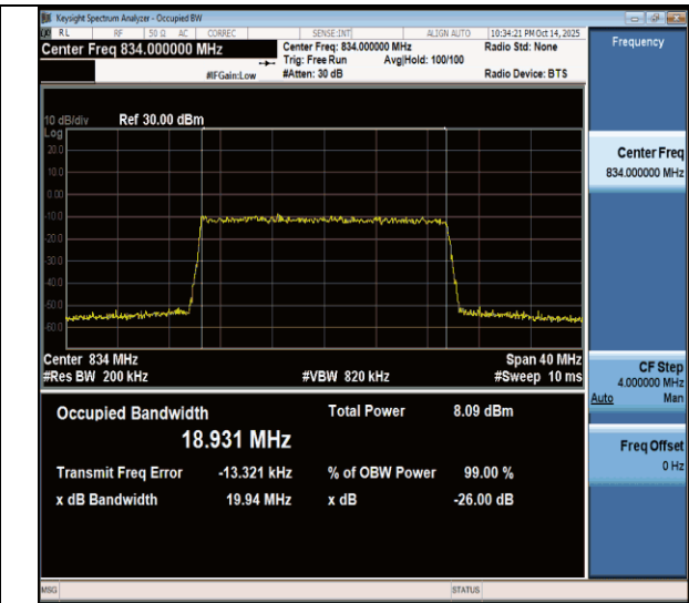
NTNV-n26(824-849)-PC3-15-20-L-CP-256QAM-Outer_Full-Ant1- PASS
