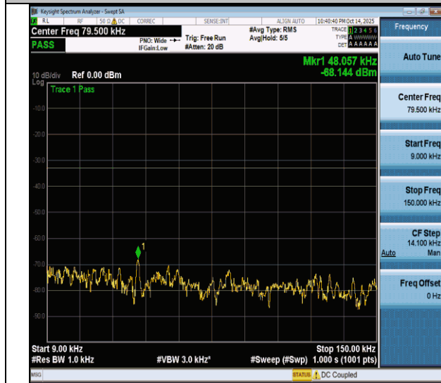
NTNV-n26(824-849)-PC3-15-20-L-CP-QPSK-Edge_1RB_Left- 0.009-0.15-PASS
