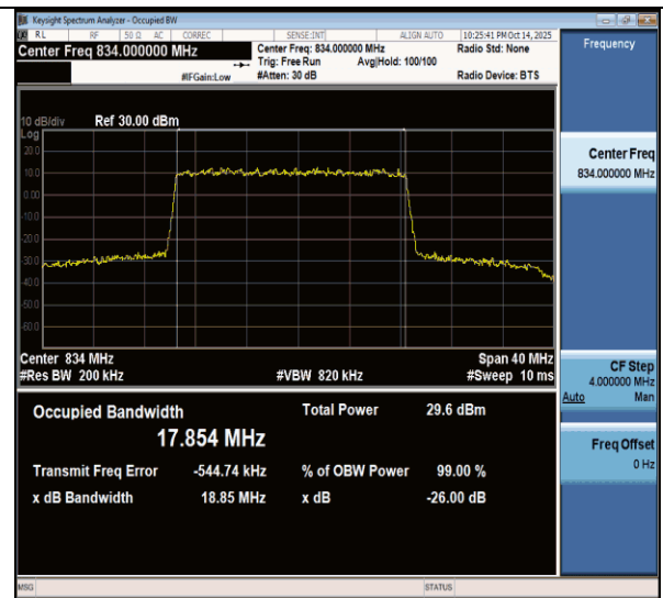
NTNV-n26(824-849)-PC3-15-20-L-DFT-16QAM-Outer_Full-Ant1- PASS
