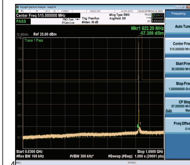
NTNV-n26(824-849)-PC3-15-20-M-DFT-BPSK-Edge_1RB_Left- 30-1000-PASS
