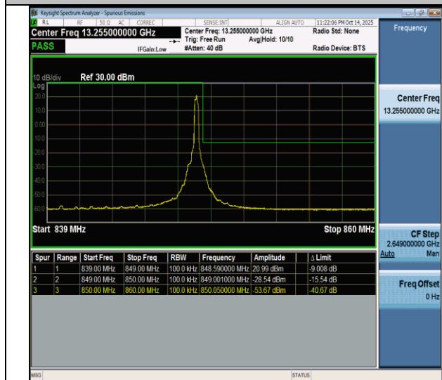
NTNV-n26(824-849)-PC3-15-10-H-DFT-BPSK-Edge_1RB_Right-PASS
