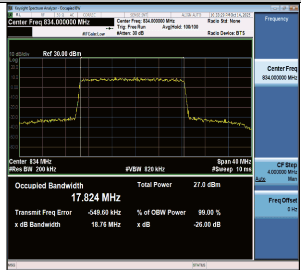
NTNV-n26(824-849)-PC3-15-20-L-DFT-256QAM-Outer_Full-Ant1- PASS
