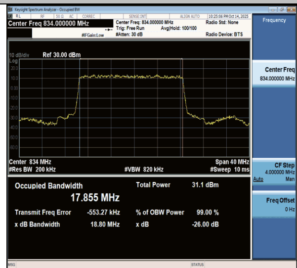
NTVN-n26(824-849)-PC3-15-20-L-DFT-BPSK-Outet_Full-Ant1-PASS
