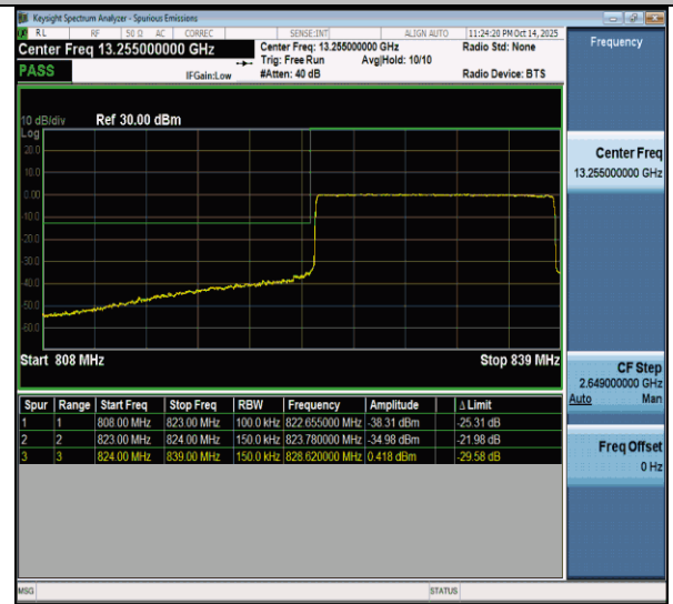
NTNV-n26(824-849)-PC3-15-15-L-CP-QPSK-Outer_Full-PASS
