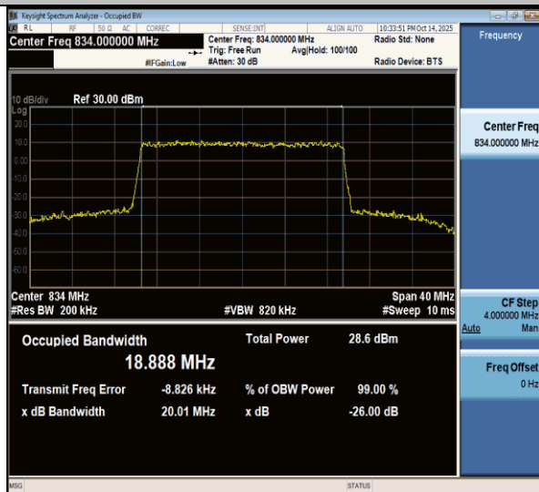
NTNV-n26(824-849)-PC3-15-20-L-CP-QPSK-Outer_Full-Ant1- PASS
