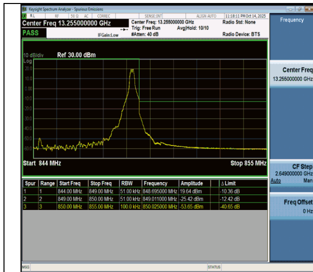
NTNV-n26(824-849)-PC3-15-5-H-DFT-BPSK-Edge_1RB_Right-PASS
