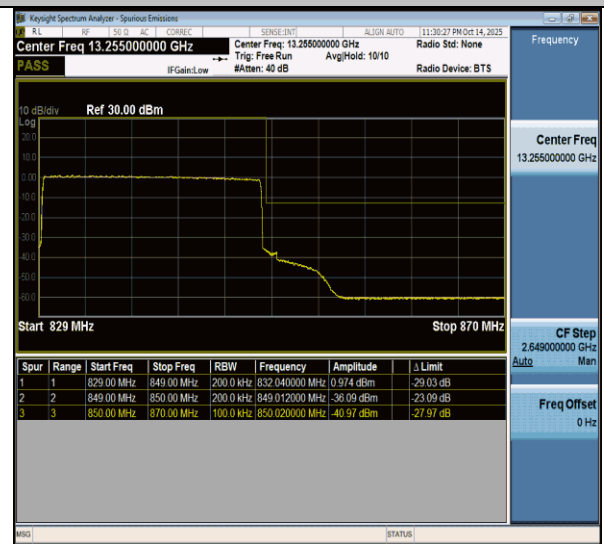
NTNV-n26(824-849)-PC3-15-20-H-CP-QPSK-Outer_Full-PASS
