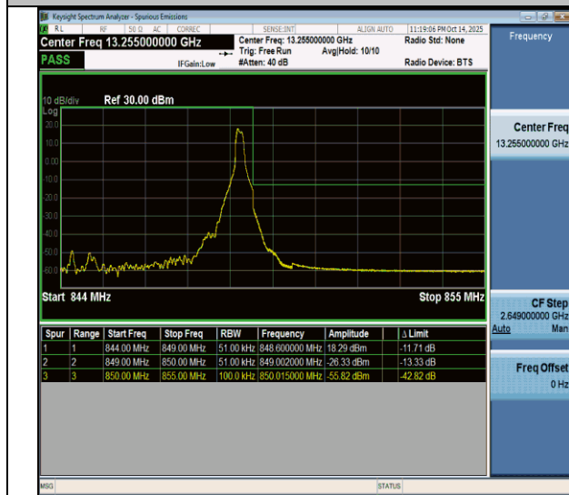
NTNV-n26(824-849)-PC3-15-5-H-CP-QPSK-Edge_1RB_Right-PASS
