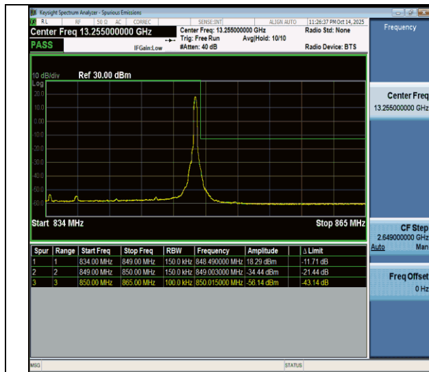
NTNV-n26(824-849)-PC3-15-15-H-CP-QPSK-Edge_1RB_Right-PASS
