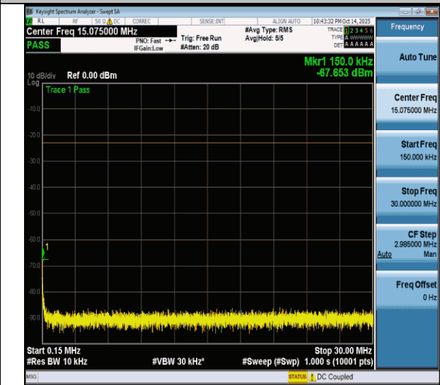
NTNV-n26(824-849)-PC3-15-20-M-CP-QPSK-Edge_1RB_Left- 0.15-30-PASS
