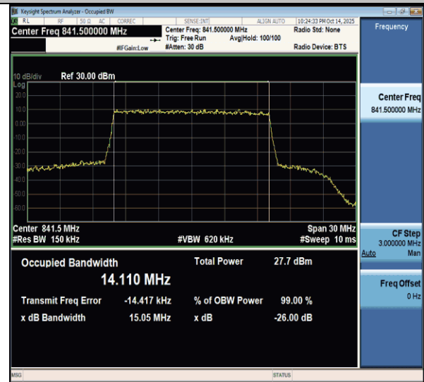
NTVN-n26(824-849)-PC3-15-15-H-CP-64QAM-Outet_Full-Ant1-PASS
