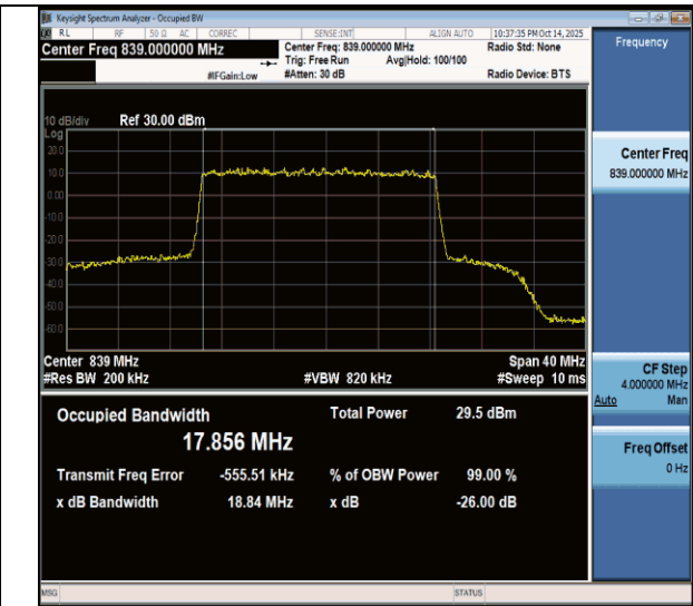
NTNV-n26(824-849)-PC3-15-20-H-DFT-16QAM-Outet_Full-Ant1- PASS
