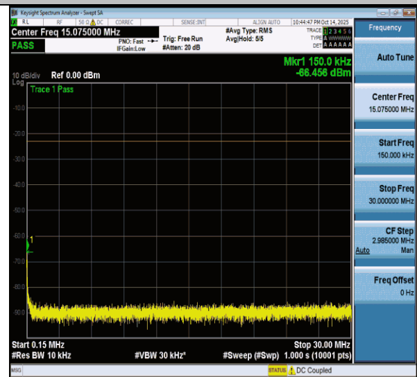
NTNV-n26(824-849)-PC3-15-20-H-DFT-BPSK-Edge_1RB_Left- 0.15-30-PASS
