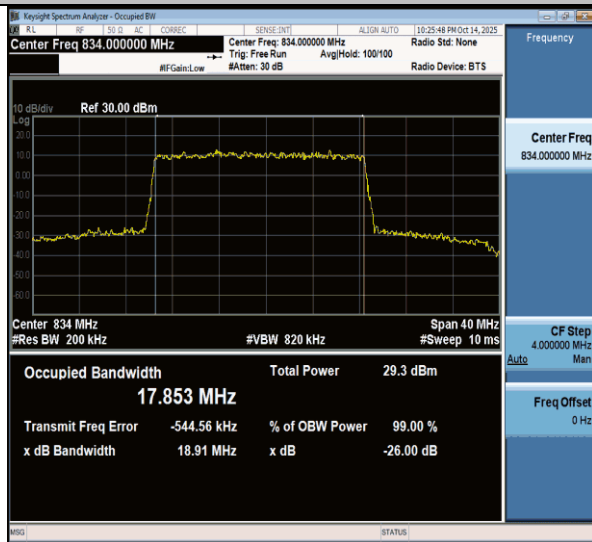
NTNV-n26(824-849)-PC3-15-20-L-DFT-64QAM-Outer_Full-Ant1- PASS
