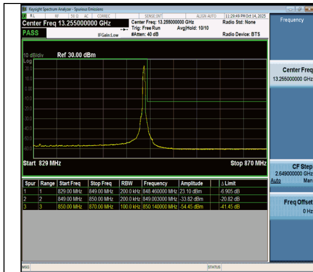
NTNV-n26(824-849)-PC3-15-20-H-DFT-BPSK-Edge_1RB_Right- PASS
