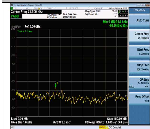
NTNV-n26(824-849)-PC3-15-20-M-DFT-BPSK-Edge_1RB_Left- 0.009-0.15-PASS
