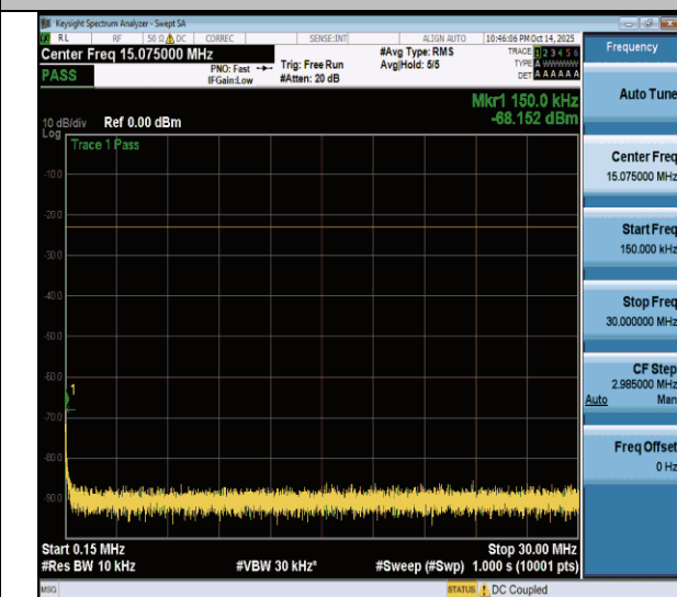
NTNV-n26(824-849)-PC3-15-20-H-CP-QPSK-Edge_1RB_Left- 0.15-30-PASS
