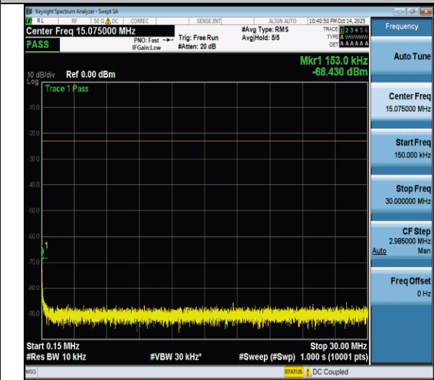
NTNV-n26(824-849)-PC3-15-20-L-CP-QPSK-Edge_1RB_Left- 0.15-30-PASS
