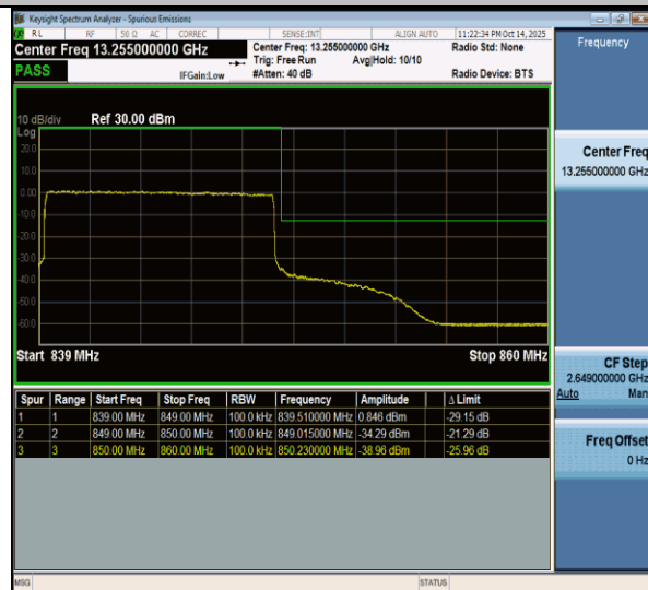
NTNV-n26(824-849)-PC3-15-10-H-CP-QPSK-Outer_Full-PASS
