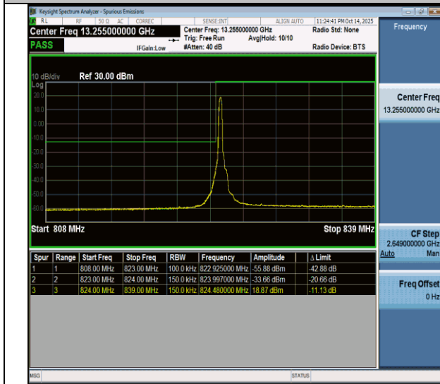
NTNV-n26(824-849)-PC3-15-15-L-CP-QPSK-Edge_1RB_Left-PASS
