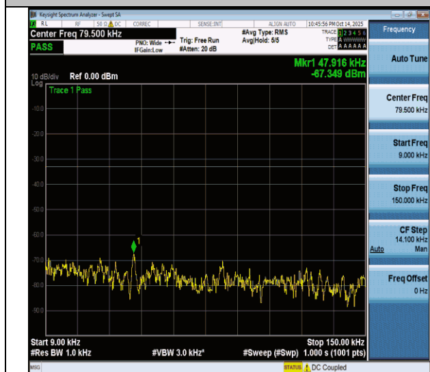
NTNV-n26(824-849)-PC3-15-20-H-CP-QPSK-Edge_1RB_Left- 0.009-0.15-PASS
