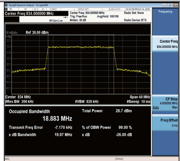
NTNV-n26(824-849)-PC3-15-20-L-CP-16QAM-Outer_Full-Ant1- PASS
