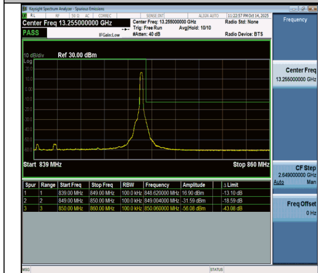
NTNV-n26(824-849)-PC3-15-10-H-CP-QPSK-Edge_1RB_Right-PASS
