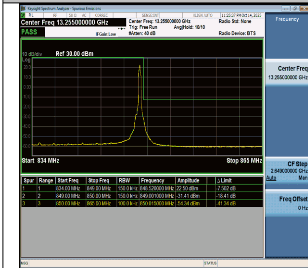
NTNV-n26(824-849)-PC3-15-15-H-DFT-BPSK-Edge_1RB_Right-PASS
