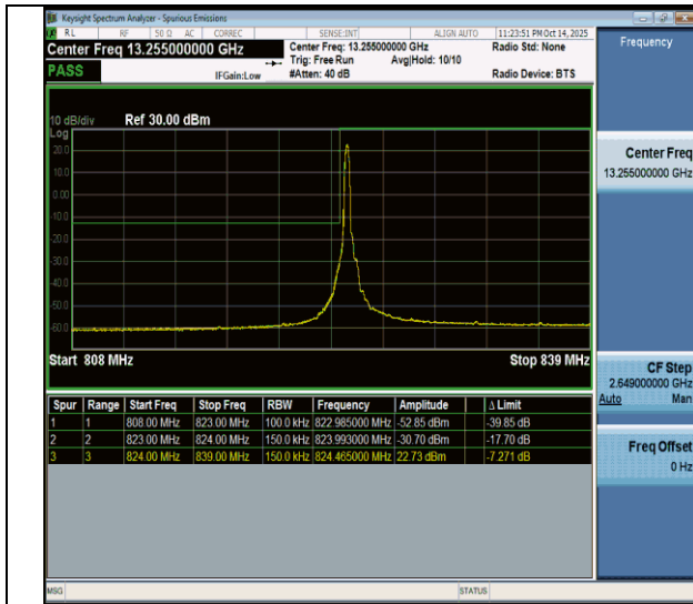
NTNV-n26(824-849)-PC3-15-15-L-DFT-BPSK-Edge_1RB_Left-PASS
