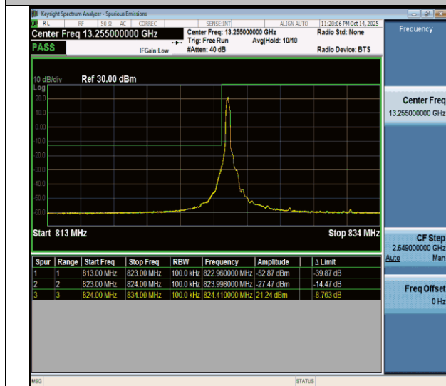
NTNV-n26(824-849)-PC3-15-10-L-DFT-BPSK-Edge_1RB_Left-PASS
