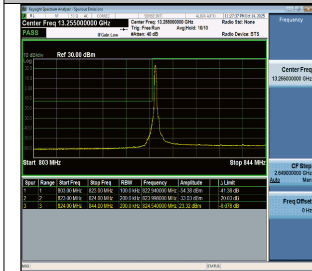
NTNV-n26(824-849)-PC3-15-20-L-DFT-BPSK-Edge_1RB_Left-PASS
