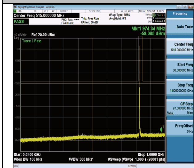
NTNV-n26(824-849)-PC3-15-20-H-CP-QPSK-Edge_1RB_Left-30- 1000-PASS
