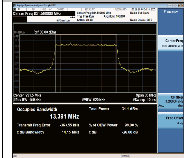
NTNV-n26(824-849)-PC3-15-15-L-DFT-BPSK-Outer_Full-Ant1- PASS
