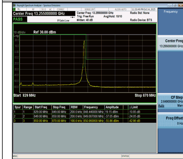
NTNV-n26(824-849)-PC3-15-20-H-CP-QPSK-Edge_1RB_Right- PASS
