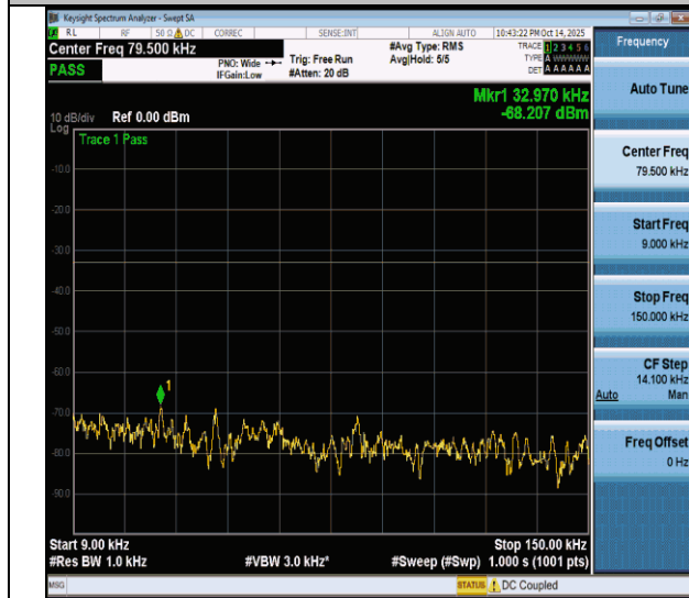
NTNV-n26(824-849)-PC3-15-20-M-CP-QPSK-Edge_1RB_Left- 0.009-0.15-PASS
