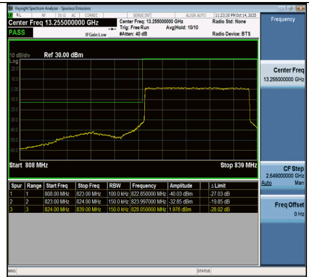
NTNV-n26(824-849)-PC3-15-15-L-DFT-BPSK-Outer_Full-PASS
