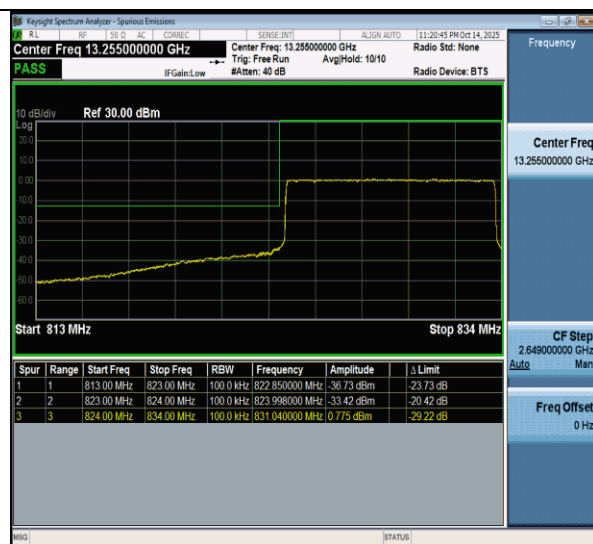
NTNV-n26(824-849)-PC3-15-10-L-CP-QPSK-Outer_Full-PASS
