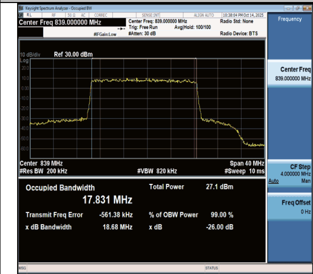
NTNV-n26(824-849)-PC3-15-20-H-DFT-256QAM-Outet_Full-Ant1-PASS
