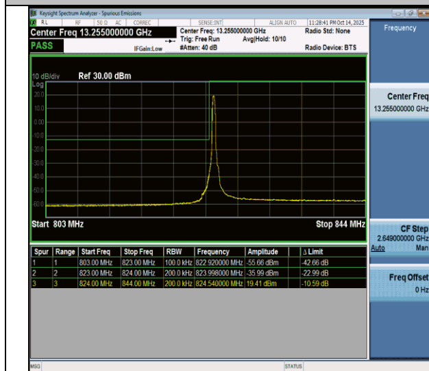
NTNV-n26(824-849)-PC3-15-20-L-CP-QPSK-Edge_1RB_Left-PASS
