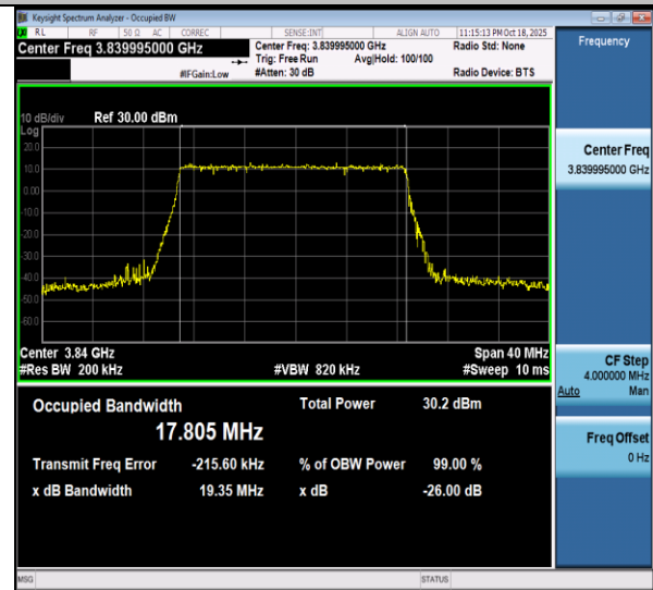
NTVN-n77(3700-3980)-PC3-30-20-M-DFT-256QAM-Outet_Full-Ant1-PASS
