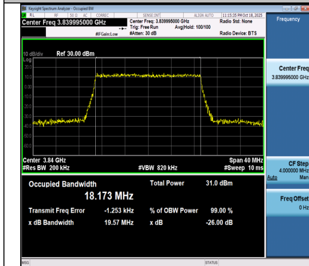
NTVN-n77(3700-3980)-PC3-30-20-M-CP-QPSK-Outet_Full-Ant1-PASS
