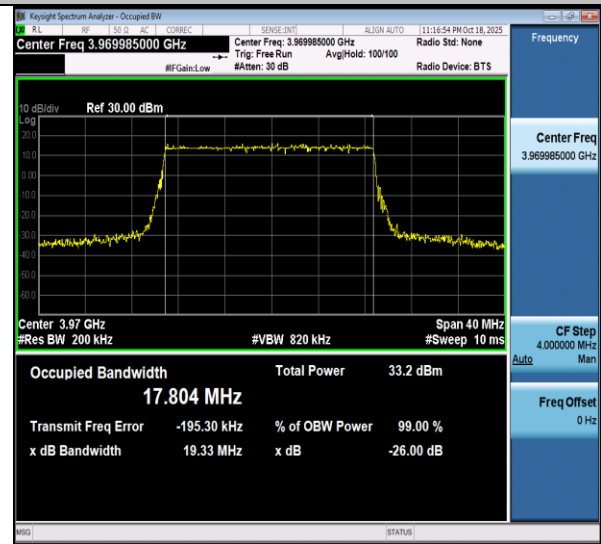
NTNV-n77(3700-3980)-PC3-30-20-H-DFT-QPSK-Outer_Full-Ant1-PASS
