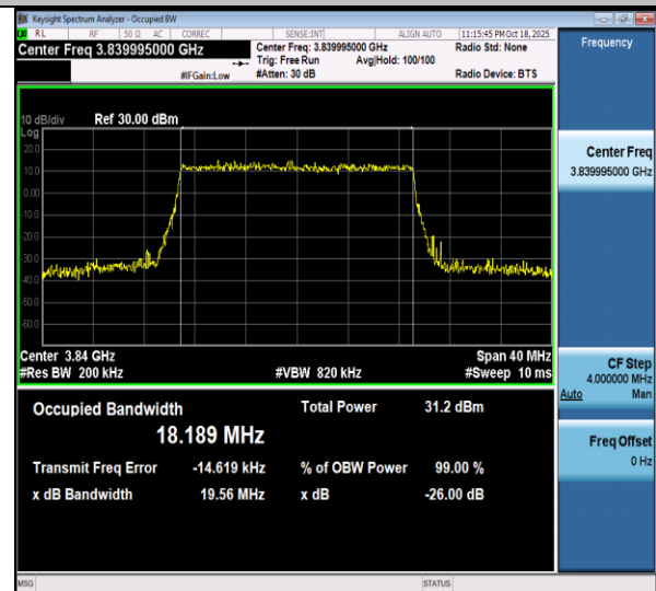
NTVN-n77(3700-3980)-PC3-30-20-M-CP-16QAM-Outet_Full-Ant1-PASS
