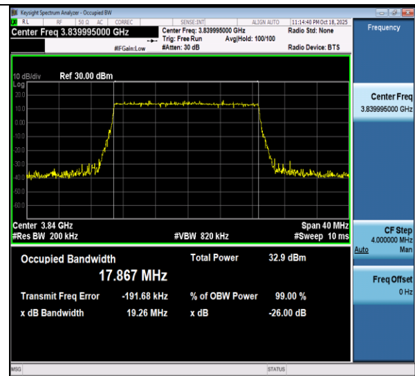
NTVN-n77(3700-3980)-PC3-30-20-M-DFT-16QAM-Outet_Full-Ant1-PASS
