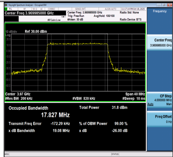
NTNV-n77(3700-3980)-PC3-30-20-H-DFT-64QAM-Outer_Full-Ant1-PASS
