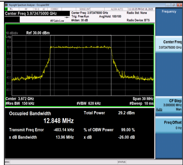
NTNV-n77(3700-3980)-PC3-30-15-H-DFT-256QAM-Outet_Full-Ant1-PASS
