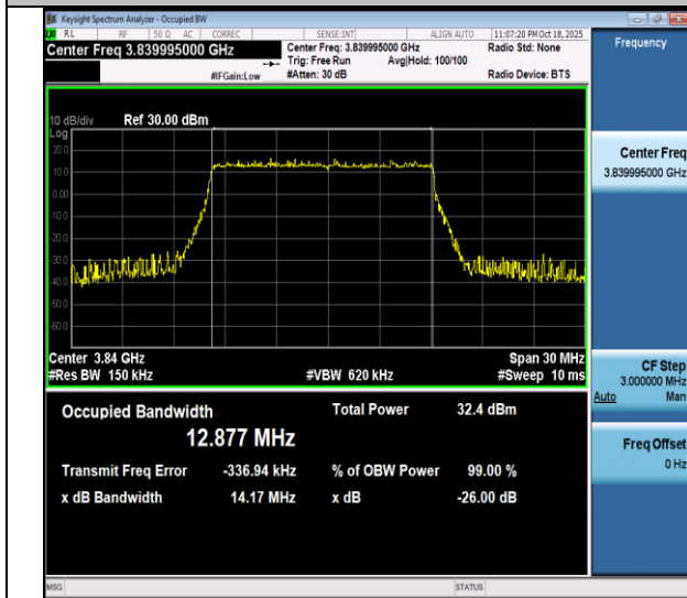
NTNV-n77(3700-3980)-PC3-30-15-M-DFT-16QAM-Outet_Full- Ant1-PASS
