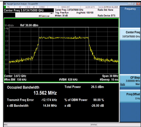
NTVN-n77(3700-3980)-PC3-30-15-H-CP-256QAM-Outer_Full-Ant1-PASS
