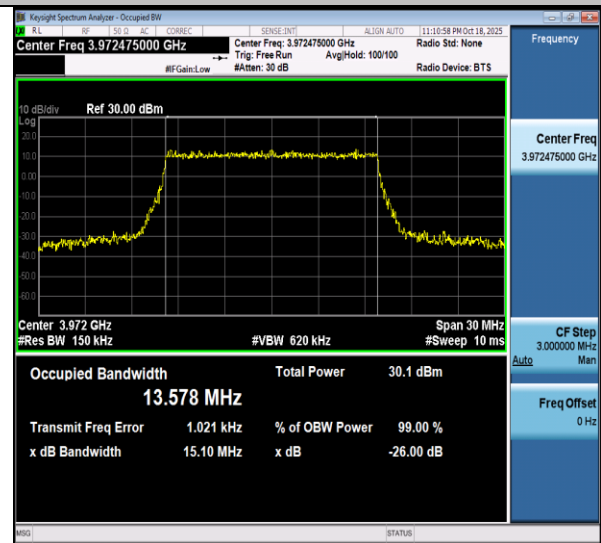
NTNV-n77(3700-3980)-PC3-30-15-H-CP-16QAM-Outet_Full-Ant1-PASS
