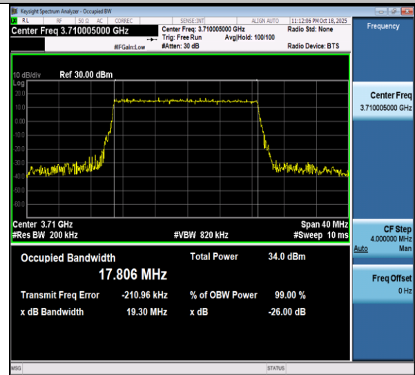
NTVN-n77(3700-3980)-PC3-30-20-L-DFT-QPSK-Outer_Full-Ant1-PASS
