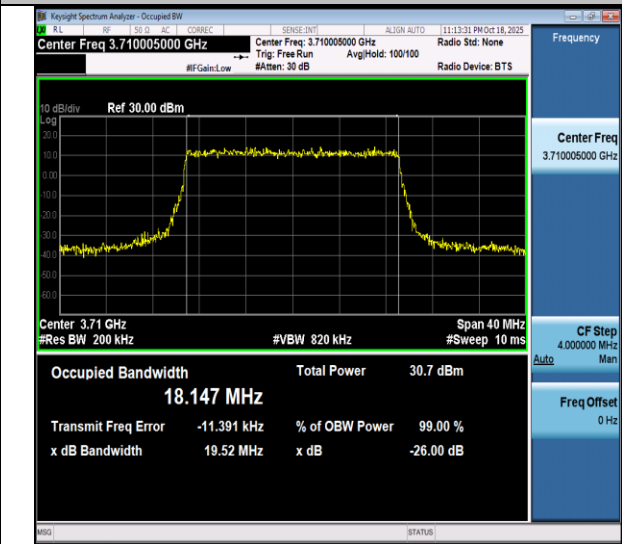
NTNV-n77(3700-3980)-PC3-30-20-L-CP-64QAM-Outer_Full-Ant1-PASS
