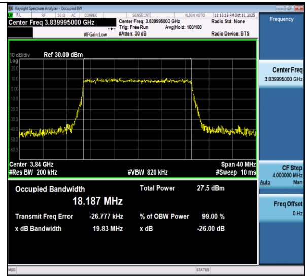
NTNV-n77(3700-3980)-PC3-30-20-M-CP-256QAM-Outer_Full-Ant1-PASS
