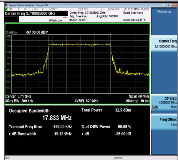
NTVN-n77(3700-3980)-PC3-30-20-L-DFT-64QAM-Outer_Full-Ant1-PASS
