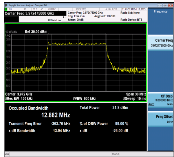
NTNV-n77(3700-3980)-PC3-30-15-H-DFT-16QAM-Outet_Full-Ant1-PASS
