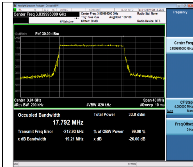
NTVN-n77(3700-3980)-PC3-30-20-M-DFT-QPSK-Outet_Full-Ant1-PASS
