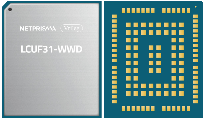
Figure 42: Top and Bottom Views
