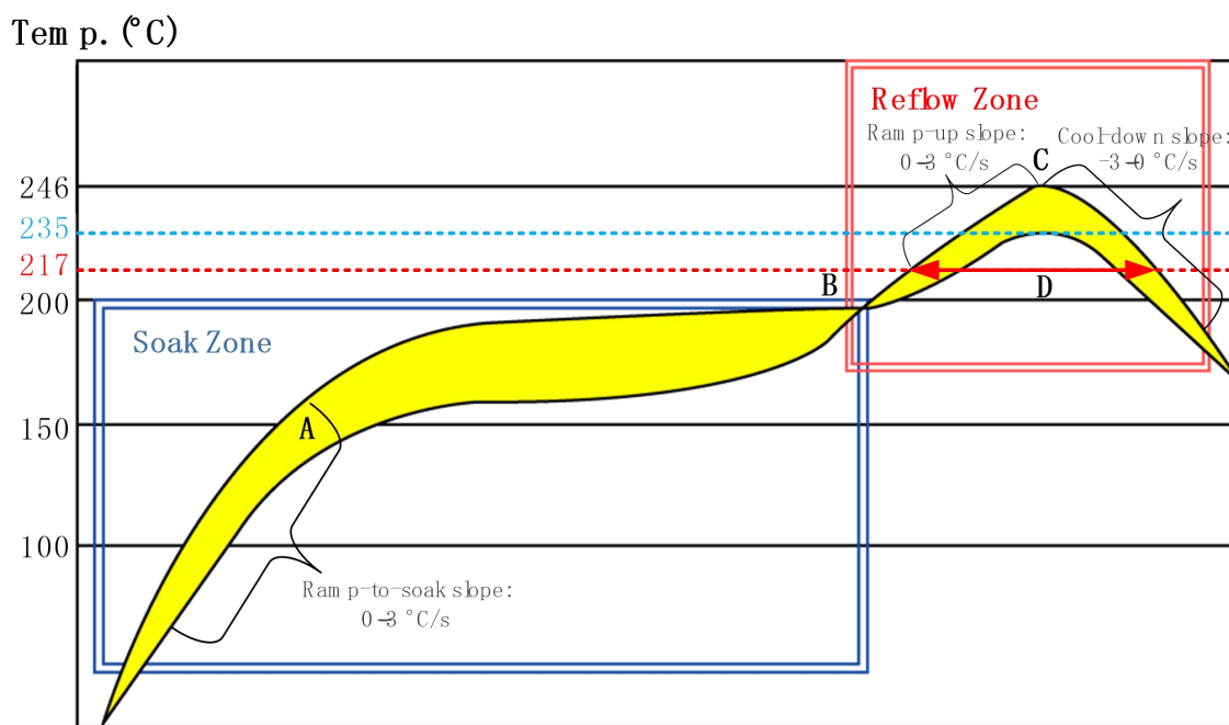
Figure 43: Recommended Reflow Soldering Thermal Profile
