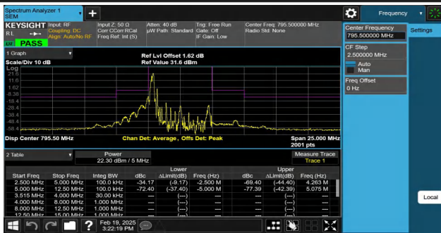
NTNV-Band14-5MHz-QPSK-23355-1RB#0--12.50--5.00-PASS
