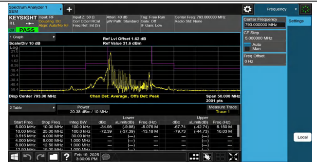
NTNV-Band14-10MHz-16QAM-23330-1RB#0--25.00--10.00-PASS
