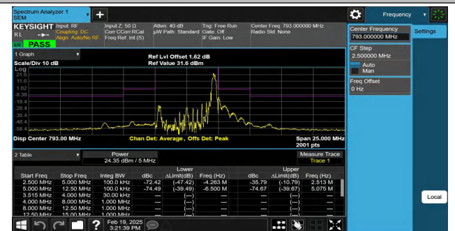
NTNV-Band14-5MHz-QPSK-23330-1RB#24-5.00-12.50-PASS
