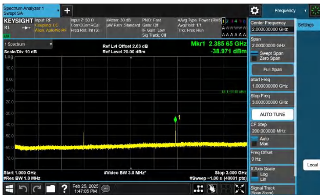
Band14-5MHz-QPSK-23330-1RB#24-1000~3000-PASS
