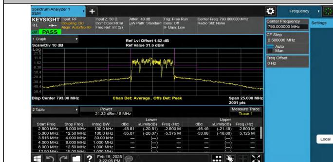
NTNV-Band14-5MHz-16QAM-23330-25RB#0--12.50--5.00-PASS
