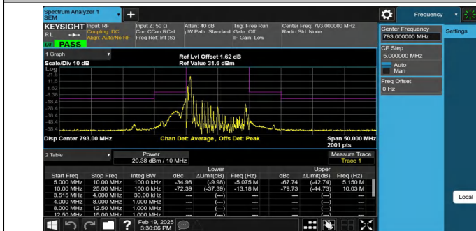
NTNV-Band14-10MHz-16QAM-23330-1RB#0-10.00-25.00-PASS
