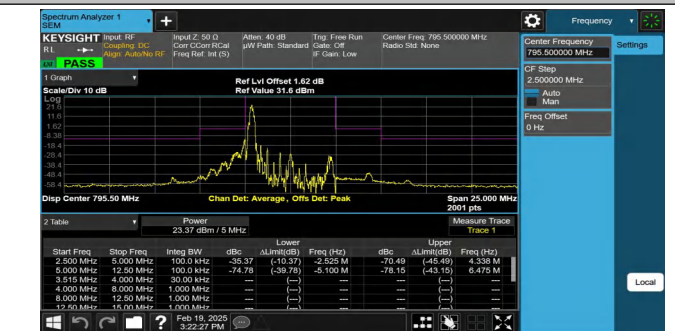
NTNV-Band14-5MHz-16QAM-23355-1RB#0-5.00-12.50-PASS
