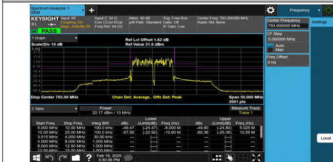
NTNV-Band14-10MHz-QPSK-23330-50RB#0-10.00-25.00-PASS
