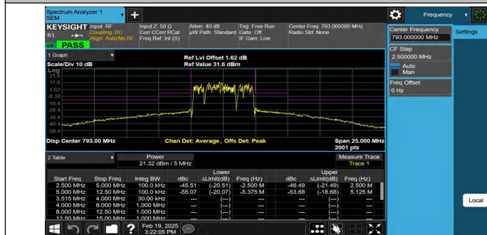
NTNV-Band14-5MHz-16QAM-23330-25RB#0--2.50-2.50-PASS
