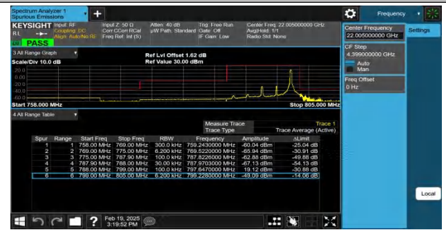
Band14-5MHz-QPSK-23355-1RB#24-PASS
