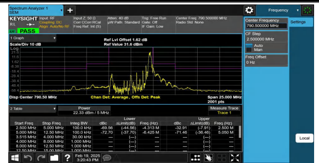
NTNV-Band14-5MHz-QPSK-23305-1RB#24--5.00--2.50-PASS
