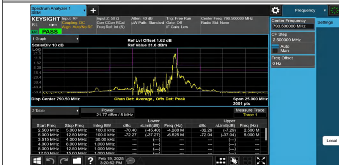
NTNV-Band14-5MHz-16QAM-23305-1RB#24-2.50-2.50-PASS
