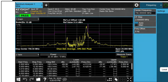
NTNV-Band14-5MHz-QPSK-23305-1RB#24--12.50--5.00-PASS
