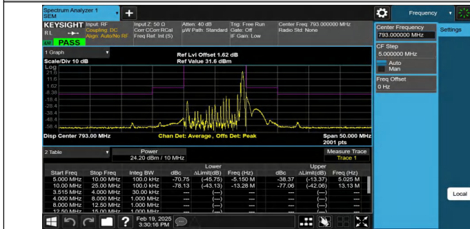
NTNV-Band14-10MHz-QPSK-23330-1RB#49-10.00-25.00-PASS
