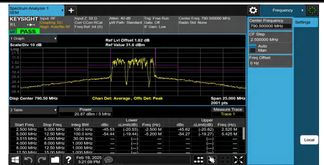
NTNV-Band14-5MHz-16QAM-23305-25RB#0--5.00--2.50-PASS
