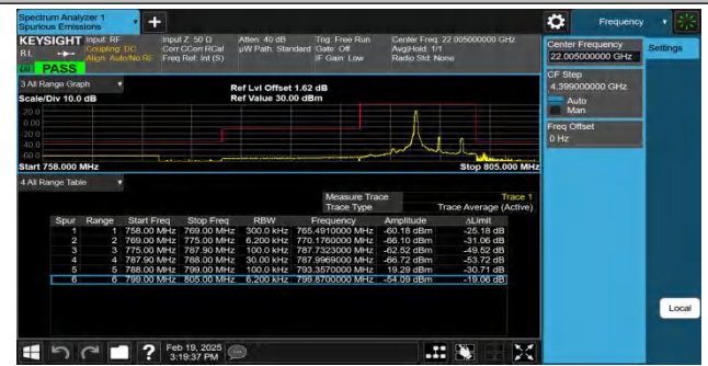
Band14-5MHz-QPSK-23355-1RB#0-PASS
