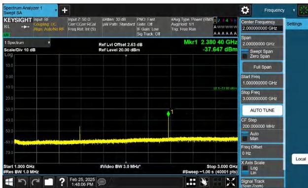
Band14-5MHz-QPSK-23355-1RB#0-1000~3000-PASS
