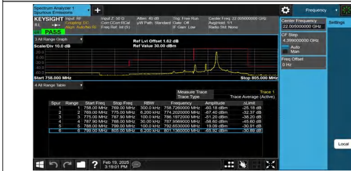
Band14-5MHz-QPSK-23305-1RB#24-PASS
