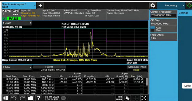
NTNV-Band14-10MHz-16QAM-23330-1RB#49-10.00-25.00-PASS
