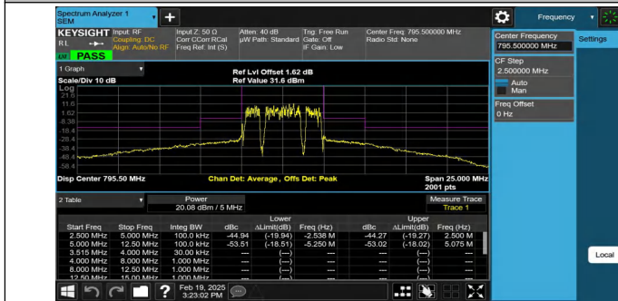
NTNV-Band14-5MHz-16QAM-23355-25RB#0--2.50--2.50-PASS
