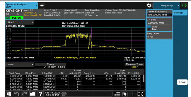
NTNV-Band14-5MHz-QPSK-23330-25RB#0-5.00-12.50-PASS
