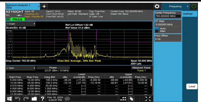
NTNV-Band14-10MHz-QPSK-23330-1RB#0--5.00-5.00-PASS
