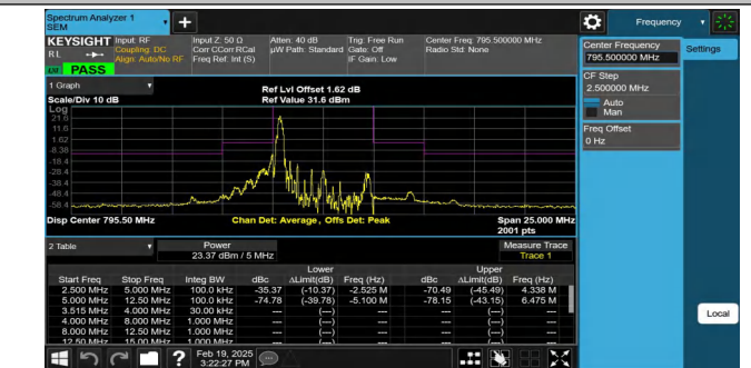
NTNV-Band14-5MHz-16QAM-23355-1RB#0--5.00--2.50-PASS
