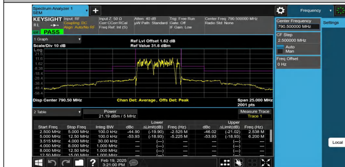
NTNV-Band14-5MHz-QPSK-23305-25RB#0-2.50-5.00-PASS
