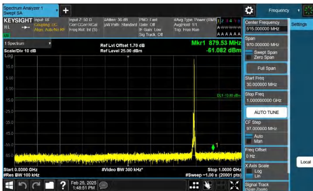
Band14-5MHz-QPSK-23355-1RB#24-30~1000-PASS
