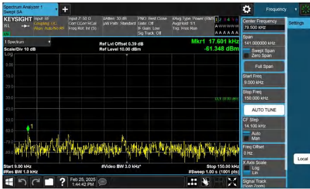
Band14-5MHz-QPSK-23305-1RB#24-0.009~0.15-PASS
