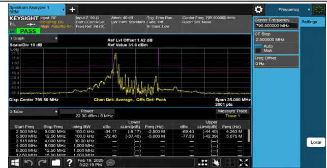
NTNV-Band14-5MHz-QPSK-23355-1RB#0-5.00-12.50-PASS
