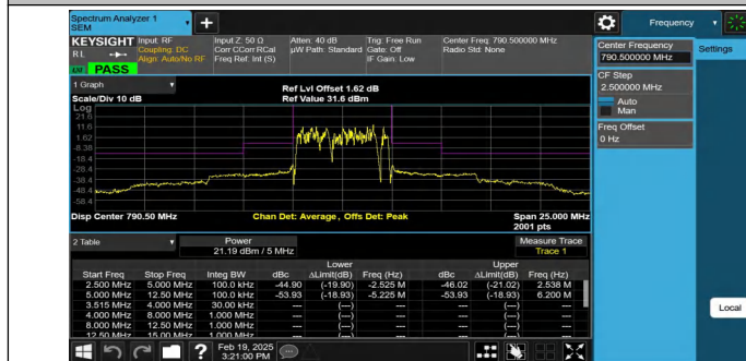
NTNV-Band14-5MHz-QPSK-23305-25RB#0--12.50--5.00-PASS
