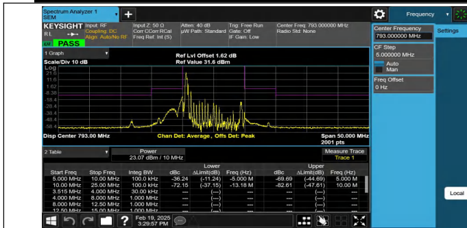
NTNV-Band14-10MHz-QPSK-23330-1RB#0--10.00--5.00-PASS
