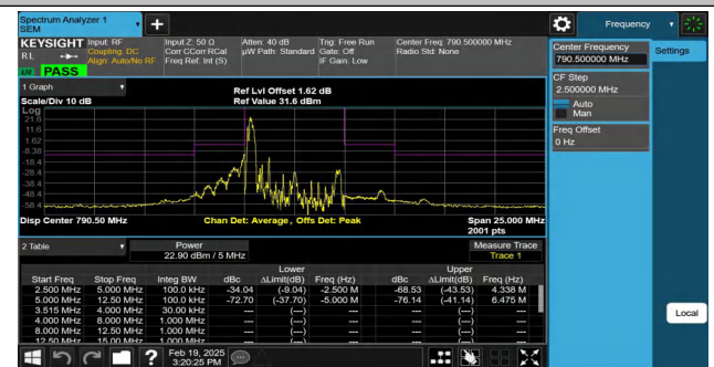
NTNV-Band14-5MHz-QPSK-23305-1RB#0-5.00-12.50-PASS
