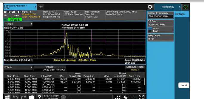
NTNV-Band14-5MHz-16QAM-23330-1RB#0-5.00-12.50-PASS
