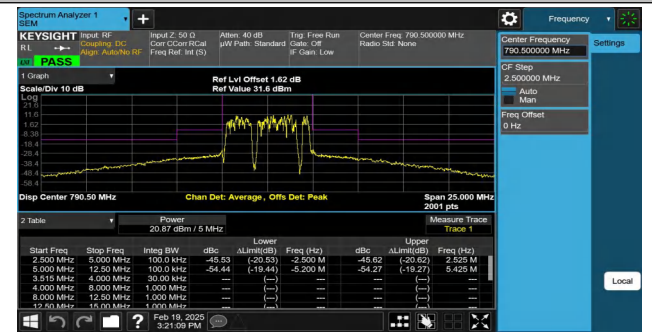
NTNV-Band14-5MHz-16QAM-23305-25RB#0-5.00-12.50-PASS
