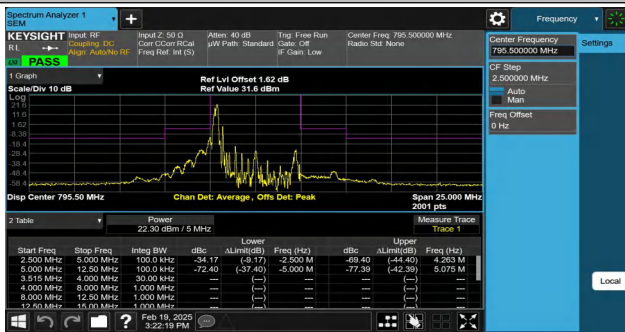
NTNV-Band14-5MHz-QPSK-23355-1RB#0-2.50-5.00-PASS
