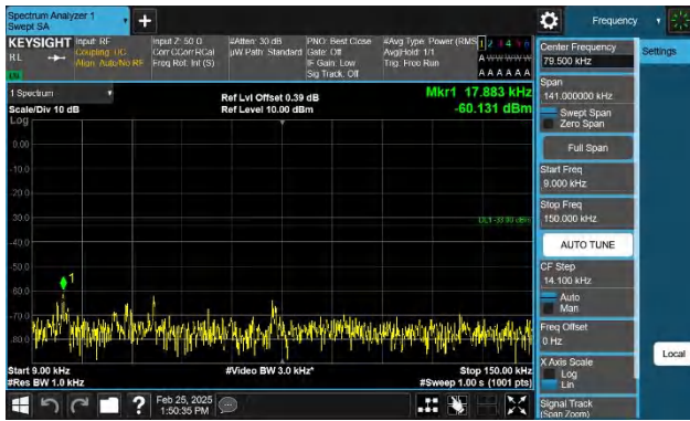
Band14-10MHz-QPSK-23330-1RB#49-0.009~0.15-PASS
