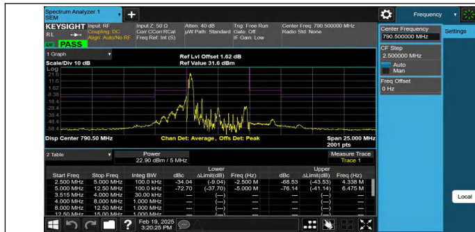
NTNV-Band14-5MHz-QPSK-23305-1RB#0--12.50--5.00-PASS
