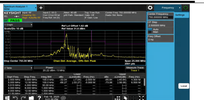
NTNV-Band14-5MHz-16QAM-23330-1RB#0--5.00--2.50-PASS
