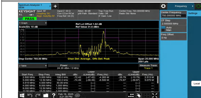
NTNV-Band14-5MHz-QPSK-23330-1RB#24-2.50-5.00-PASS
