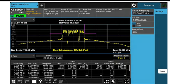
NTNV-Band14-5MHz-16QAM-23355-25RB#0--5.00--2.50-PASS
