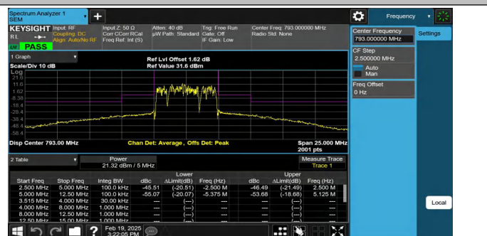
NTNV-Band14-5MHz-16QAM-23330-25RB#0--5.00--2.50-PASS
