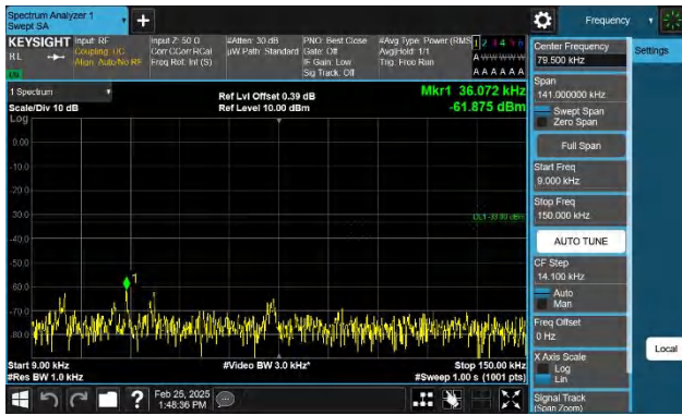
Band14-5MHz-QPSK-23355-1RB#24-0.009~0.15-PASS
