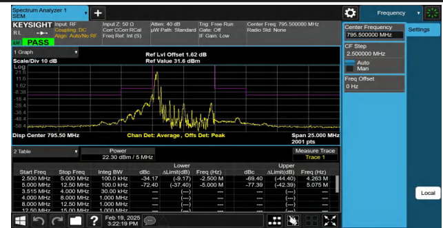
NTNV-Band14-5MHz-QPSK-23355-1RB#0--5.00--2.50-PASS
