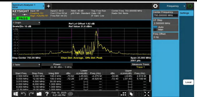
NTNV-Band14-5MHz-16QAM-23330-1RB#24--5.00--2.50-PASS
