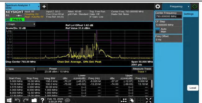
NTNV-Band14-10MHz-16QAM-23330-1RB#49--25.00--10.00-PASS
