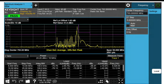
NTNV-Band14-10MHz-QPSK-23330-1RB#49-5.00-10.00-PASS
