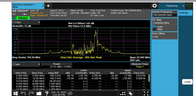
NTNV-Band14-5MHz-16QAM-23355-1RB#24--5.00--2.50-PASS
