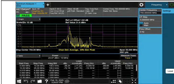
NTNV-Band14-10MHz-QPSK-23330-1RB#0-5.00-10.00-PASS
