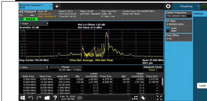
NTNV-Band14-5MHz-16QAM-23330-1RB#24--12.50--5.00-PASS
