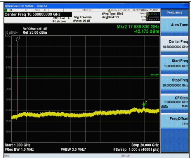
Band IV-1413-1000~20000MHz-PASS
