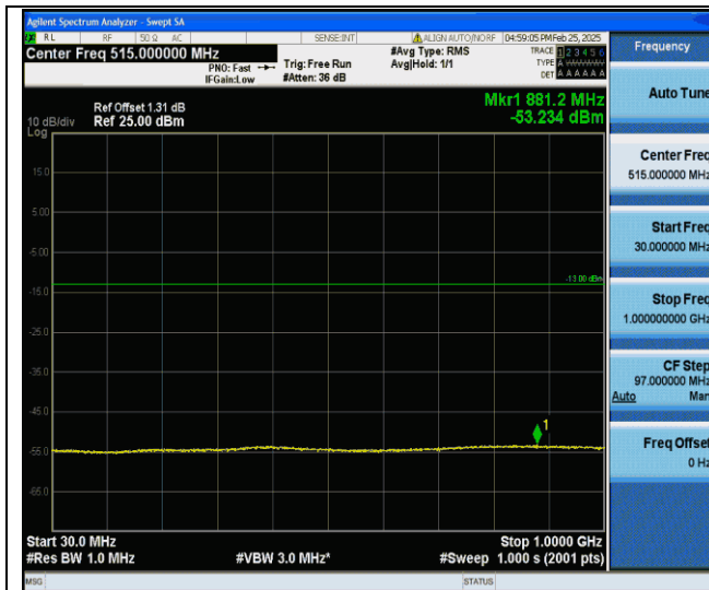
Band IV-1413-30~1000MHz-PASS
