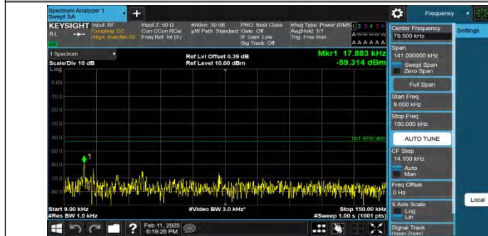
Band25-10MHz-QPSK-26090-1RB#0-0.009~0.15-PASS
