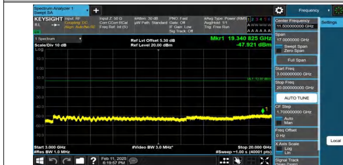
Band25-10MHz-QPSK-26090-1RB#0-3000~20000-PASS
