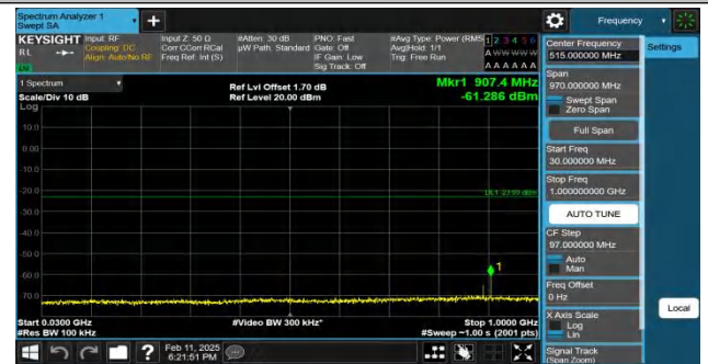
Band25-10MHz-QPSK-26365-1RB#49-30~1000-PASS
