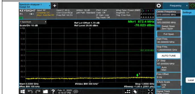
Band25-10MHz-QPSK-26090-1RB#0-30~1000-PASS
