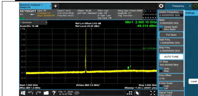
Band25-5MHz-QPSK-26665-1RB#24-1000~3000-PASS
