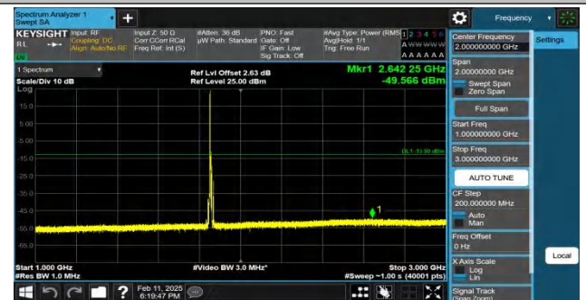
Band25-10MHz-QPSK-26090-1RB#0-1000~3000-PASS
