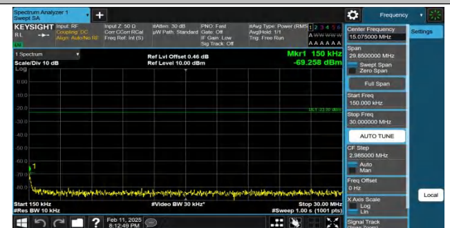
Band26(824-849)-15MHz-QPSK-26965-1RB#0-0.15~30-PASS
