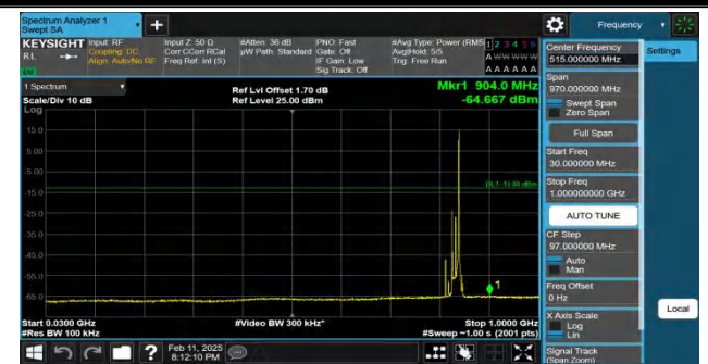
Band26(824-849)-15MHz-QPSK-26915-1RB#74-30~1000-PASS
