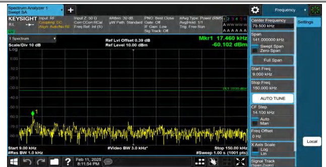
Band26(824-849)-15MHz-QPSK-26915-1RB#74-0.009~0.15-PASS
