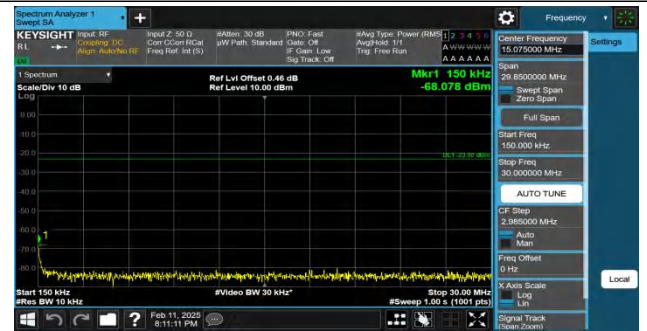
Band26(824-849)-15MHz-QPSK-26915-1RB#0-0.15~30-PASS
