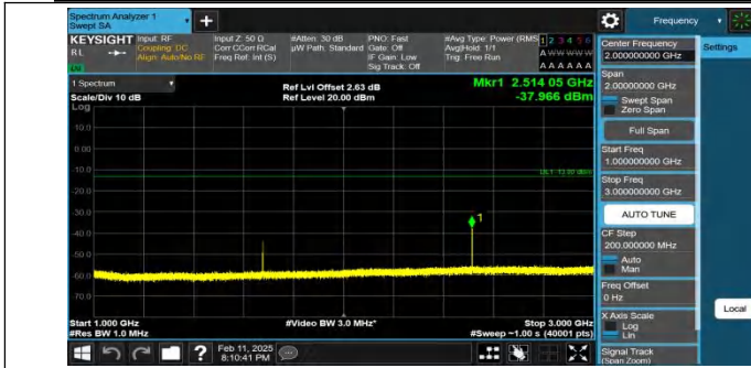
Band26(824-849)-15MHz-QPSK-26865-1RB#74-1000~3000-PAS
