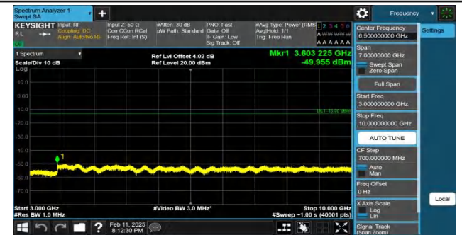
Band26(824-849)-15MHz-QPSK-26915-1RB#74-3000~10000-PAS
