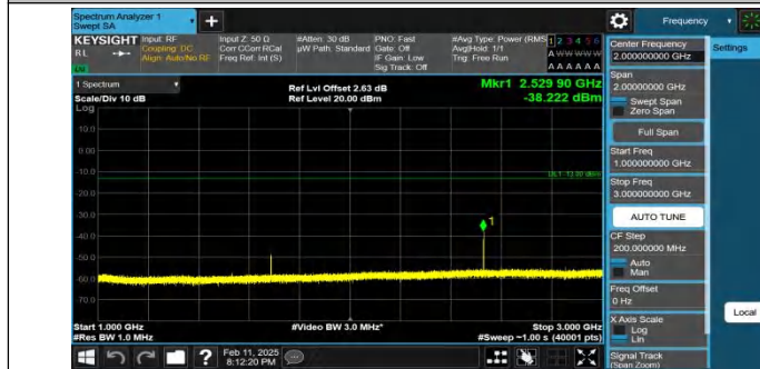
Band26(824-849)-15MHz-QPSK-26915-1RB#74-1000~3000-PAS
