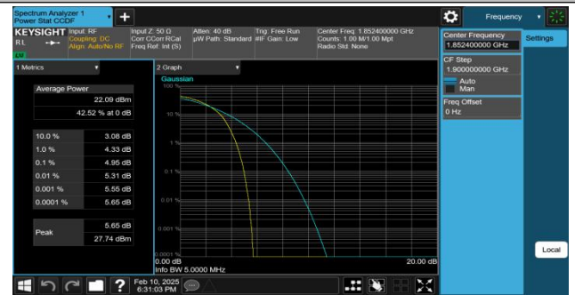
Band2-9262-4-PASS
