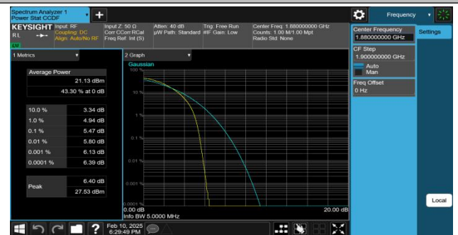
Band2-9400-3-PASS
