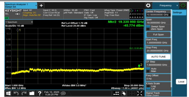
Band2-9538-1000~20000MHz-PASS
