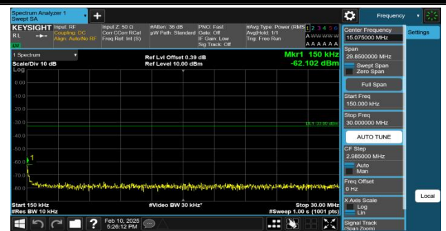
Band2-9538-0.15~30MHz-PASS
