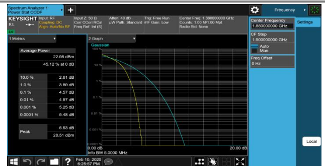
Band2-9400-1-PASS
