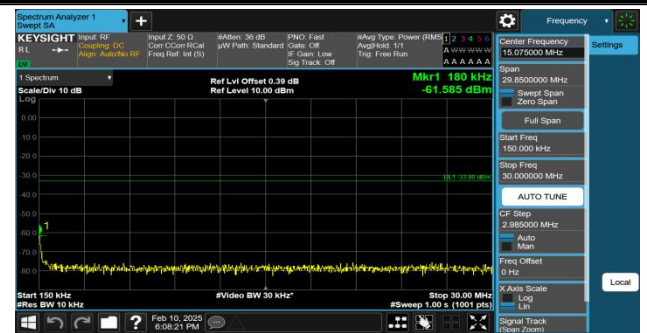
Band2-9262-1-0.15~30MHz-PASS
