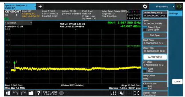
Band4-3MHz-QPSK-20175-1RB#14-3000~20000-PASS
