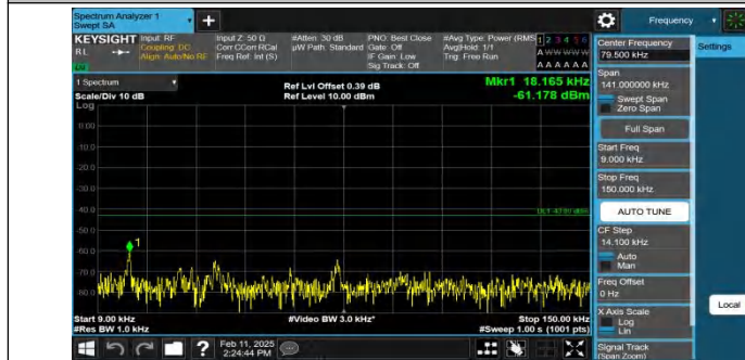
Band4-3MHz-QPSK-20385-1RB#0-0.009~0.15-PASS
