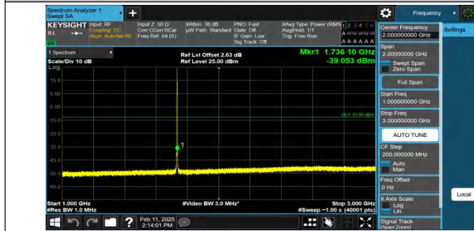
Band4-1.4MHz-QPSK-20175-1RB#5-1000~3000-PASS
