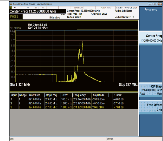
Band5_Stand-Alone_0.18_QPSK_20402_1@11_15kHz
