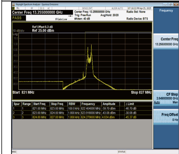
Band5_Stand-Alone_0.18_BPSK_20402_1@11_15kHz
