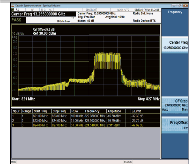
Band5_5MHz_QPSK_20425_6_Low
