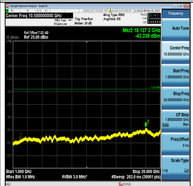
Band2-20MHz-QPSK-18900-PASS_1_Low
