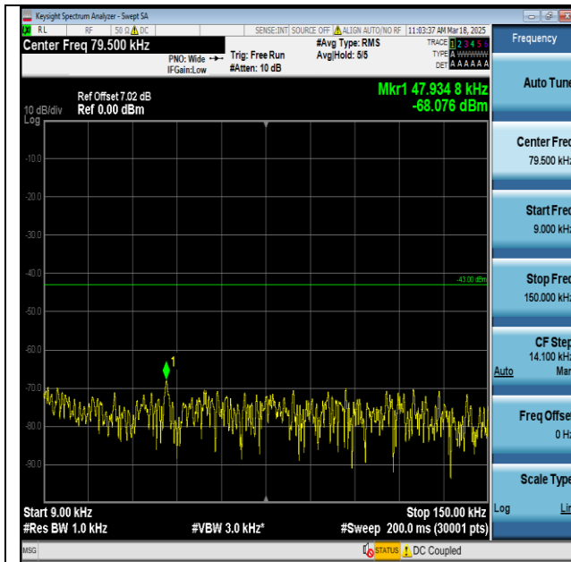
Band2-20MHz-QPSK-18900-PASS_1_Low
