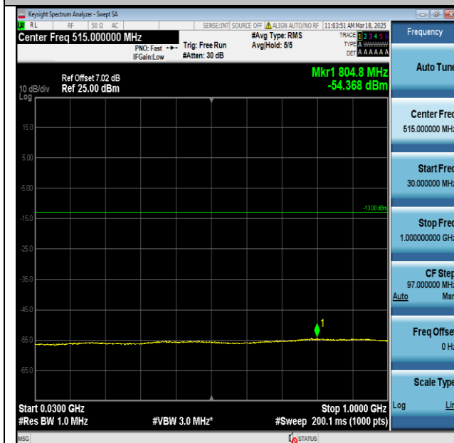
Band2-20MHz-QPSK-18900-PASS_1_Low
