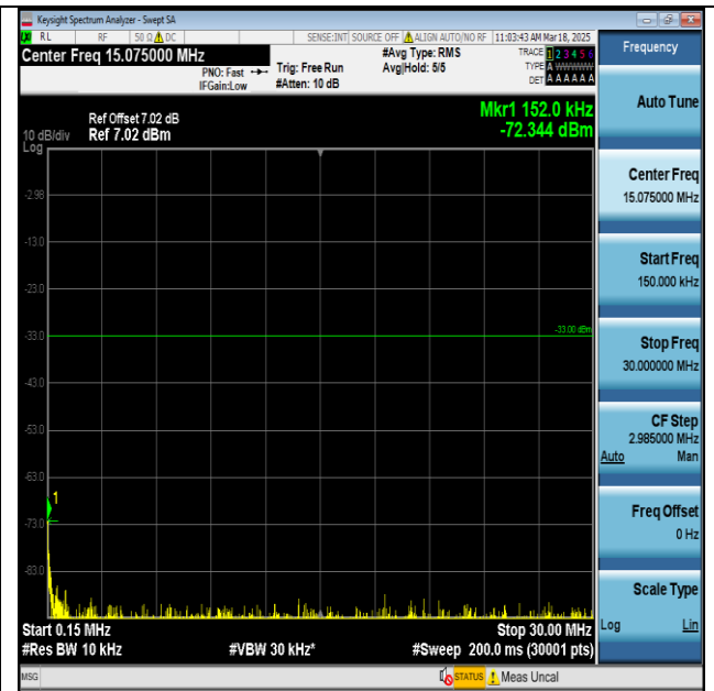
Band2-20MHz-QPSK-18900-PASS_1_Low
