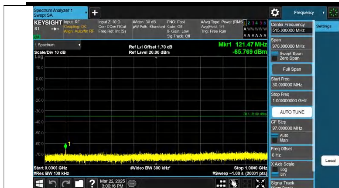
Band7-10MHz-QPSK-20800-1RB#0-30~1000-PASS
