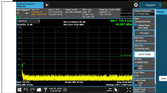
Band7-20MHz-QPSK-20850-1RB#99-0.15~30-PASS
