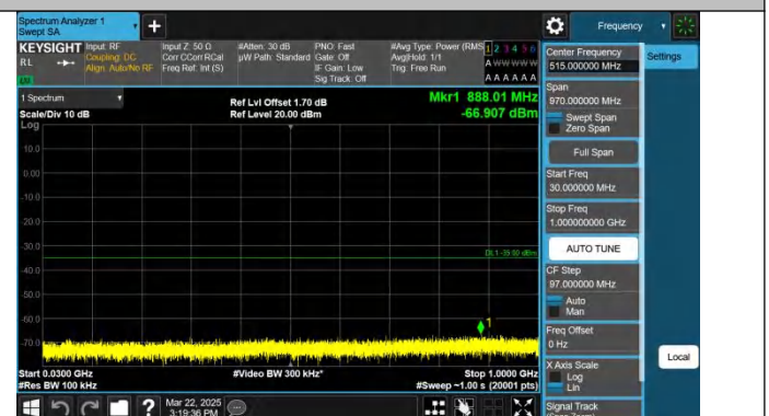
Band7-15MHz-QPSK-21375-1RB#74-30~1000-PASS
