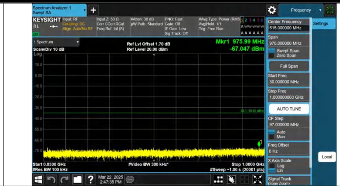
Band7-5MHz-QPSK-21100-1RB#24-30~1000-PASS
