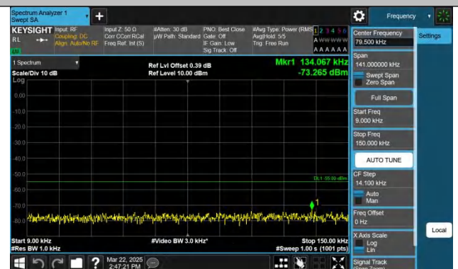
Band7-5MHz-QPSK-21100-1RB#24-0.009~0.15-PASS
