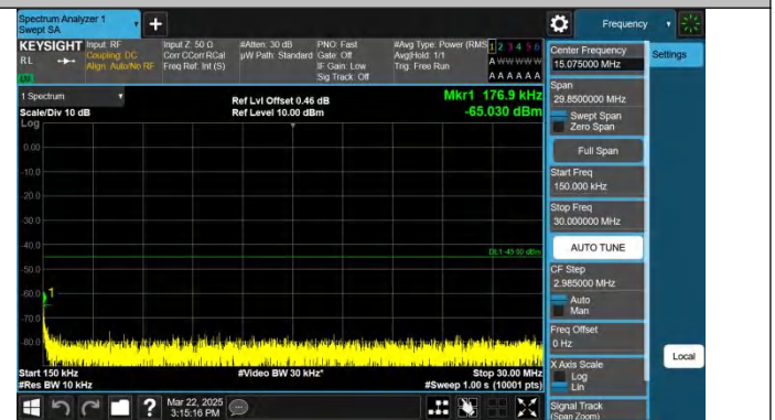
Band7-15MHz-QPSK-20825-1RB#0-0.15~30-PASS
