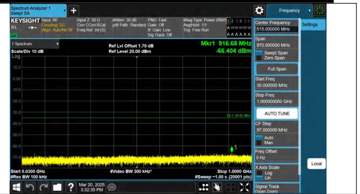
Band7-20MHz-QPSK-20850-1RB#99-30~1000-PASS
