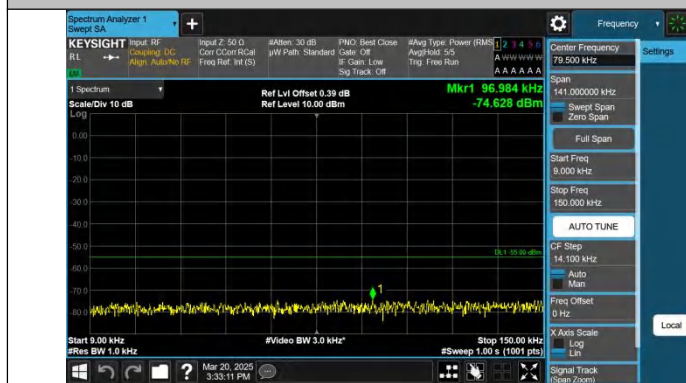
Band7-20MHz-QPSK-21100-1RB#0-0.009~0.15-PASS
