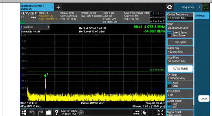
Band7-5MHz-QPSK-21425-1RB#0-0.15~30-PASS
