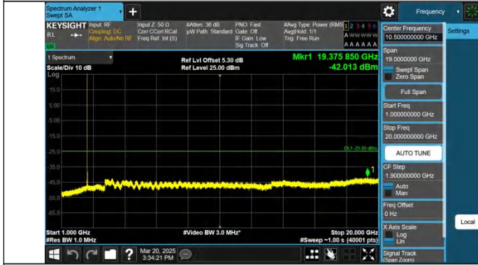
Band7-20MHz-QPSK-21100-1RB#99-1000~20000-PASS
