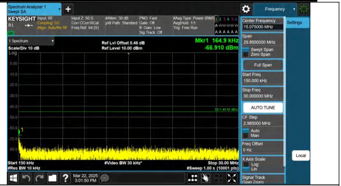
Band7-10MHz-QPSK-21100-1RB#0-0.15~30-PASS
