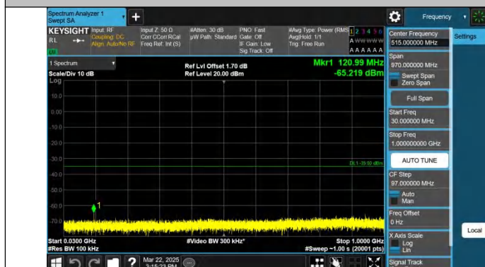
Band7-15MHz-QPSK-20825-1RB#0-30~1000-PASS
