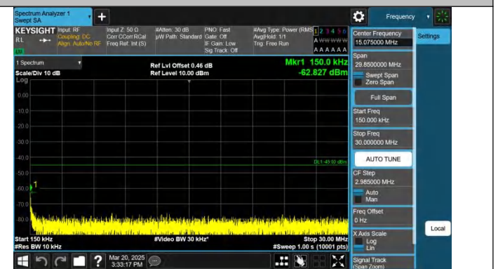
Band7-20MHz-QPSK-21100-1RB#0-0.15~30-PASS
