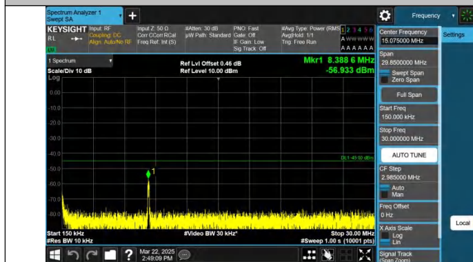
Band7-5MHz-QPSK-21425-1RB#24-0.15~30-PASS
