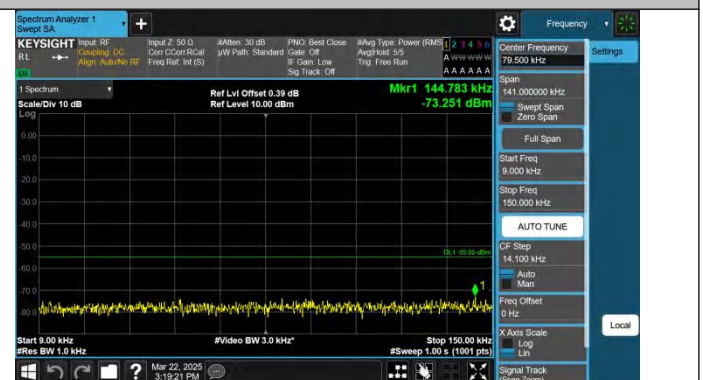
Band7-15MHz-QPSK-21375-1RB#74-0.009~0.15-PASS
