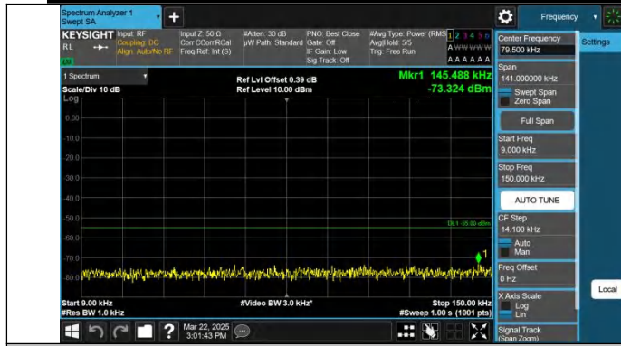
Band7-10MHz-QPSK-21100-1RB#0-0.009~0.15-PASS
