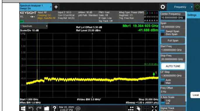
Band7-5MHz-QPSK-21425-1RB#24-1000~20000-PASS
