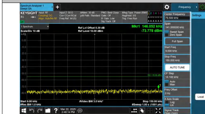
Band7-5MHz-QPSK-21425-1RB#0-0.009~0.15-PASS
