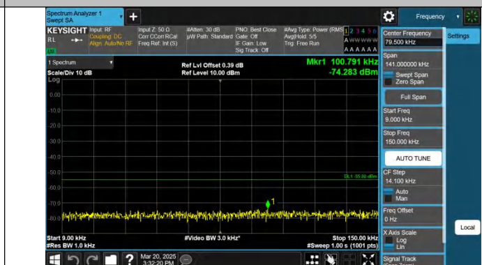
Band7-20MHz-QPSK-20850-1RB#99-0.009~0.15-PASS
