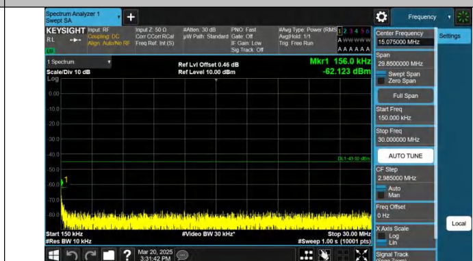
Band7-20MHz-QPSK-20850-1RB#0-0.15~30-PASS
