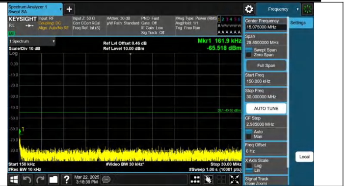
Band7-15MHz-QPSK-21375-1RB#0-0.15~30-PASS
