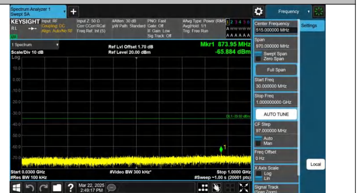
Band7-5MHz-QPSK-21425-1RB#24-30~1000-PASS
