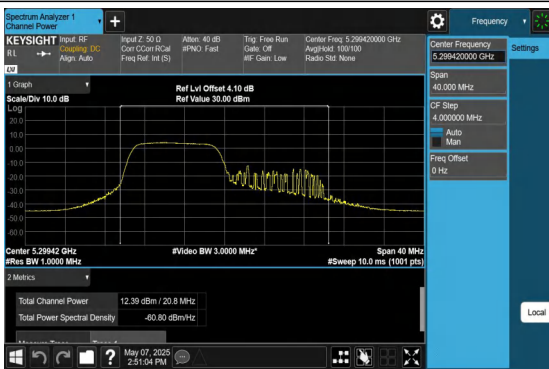
11AX20MIMO-Ant1-5300-TPC_L-106Tone-RU53-PASS
