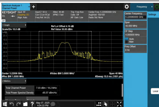
11AX20MIMO-Ant1-5220-52Tone-RU39-PASS
