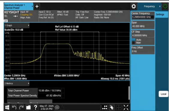
11AX20MIMO-Ant2-5300-TPC_L-106Tone-RU53-PASS
