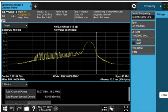
11AX20MIMO-Ant1-5320-TPC_L-26Tone-RU8-PASS
