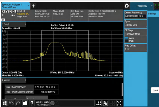
11AX20MIMO-Ant1-5300-TPC_H-106Tone-RU53-PASS
