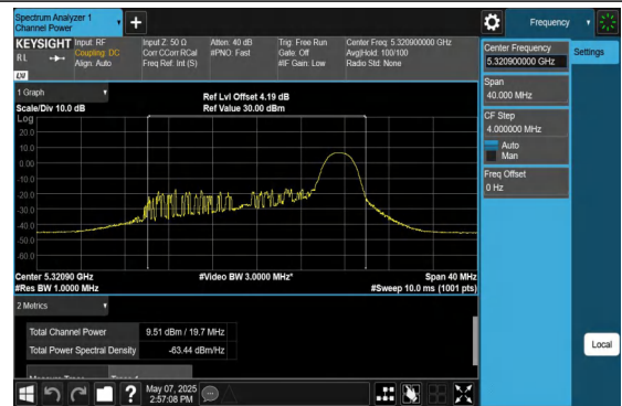
11AX20MIMO-Ant2-5320-TPC_L-26Tone-RU8-PASS
