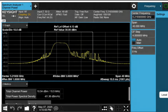
11AX20MIMO-Ant1-5220-106Tone-RU53-PASS
