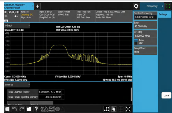
11AX20MIMO-Ant2-5300-TPC_H-106Tone-RU53-PASS
