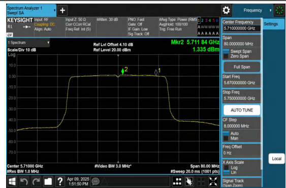
11AX40MIMO-Ant2-5710_UNII-3-PASS
