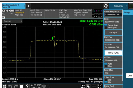
11AX160MIMO-Ant1-5250_UNII-2A-PASS
