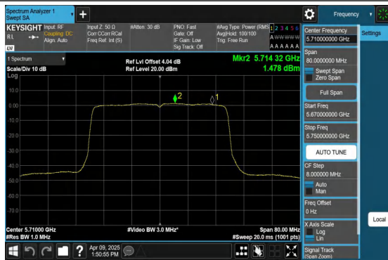
11AX40MIMO-Ant1-5710_UNII-3-PASS
